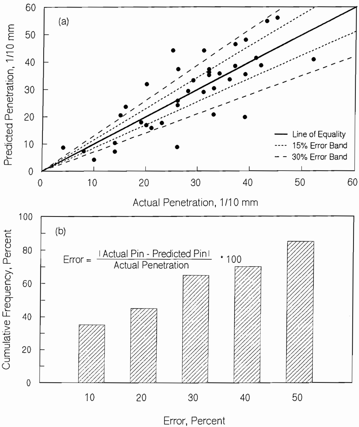
Figure F.2 Comparison of Actual and Predicted Penetration Values Using Equation 5.5 for Austin Data (without Outliers) a) Scatter Plot, b) Cumulative Percent Error.
