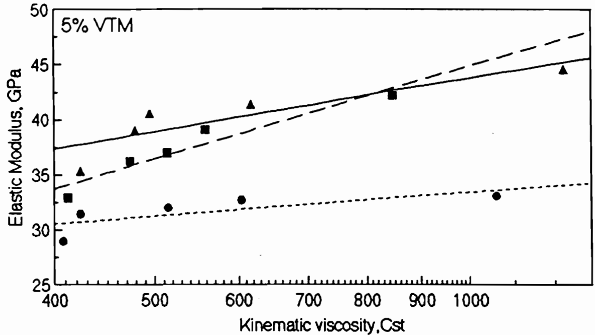
E.1 Effect of Asphalt Content on the Relationship between Elastic Modulus and Kinematic Viscosity for El Paso Mix.
