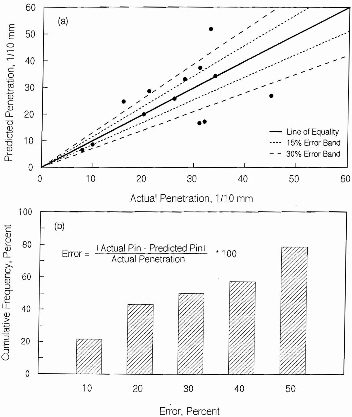
Figure F.10 Comparison of Actual and Predicted Penetration Values Using Equation 5.1 for Austin Data with 5 percent AC Content (without Outliers) a) Scatter Plot, b) Cumulative Percent Error.
