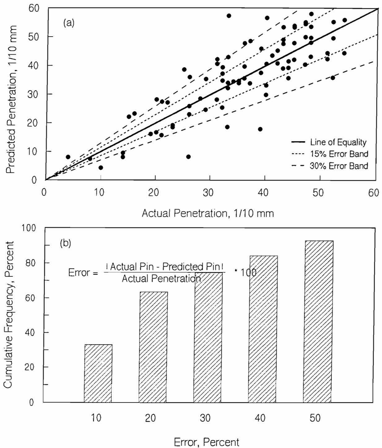
Figure F.5 Comparison of Actual and Predicted Penetration Values Using Equation 5.5 for All Data (without Outliers) a) Scatter Plot, b) Cumulative Percent Error.
