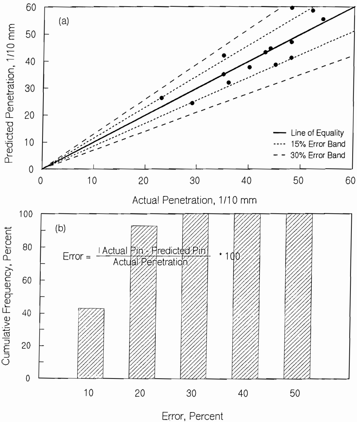
Figure F.16 Comparison of Actual and Predicted Penetration Values Using Equation 5.1 for El Paso Data with 5 percent VTM (without Outliers) a) Scatter Plot, b) Cumulative Percent Error.
