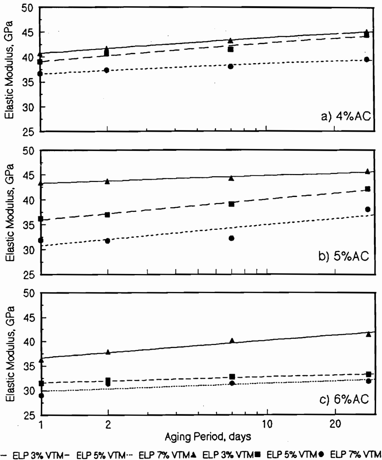
Figure 4.1 - Typical Variation in Elastic Modulus with Aging Period for El Paso Mix.
