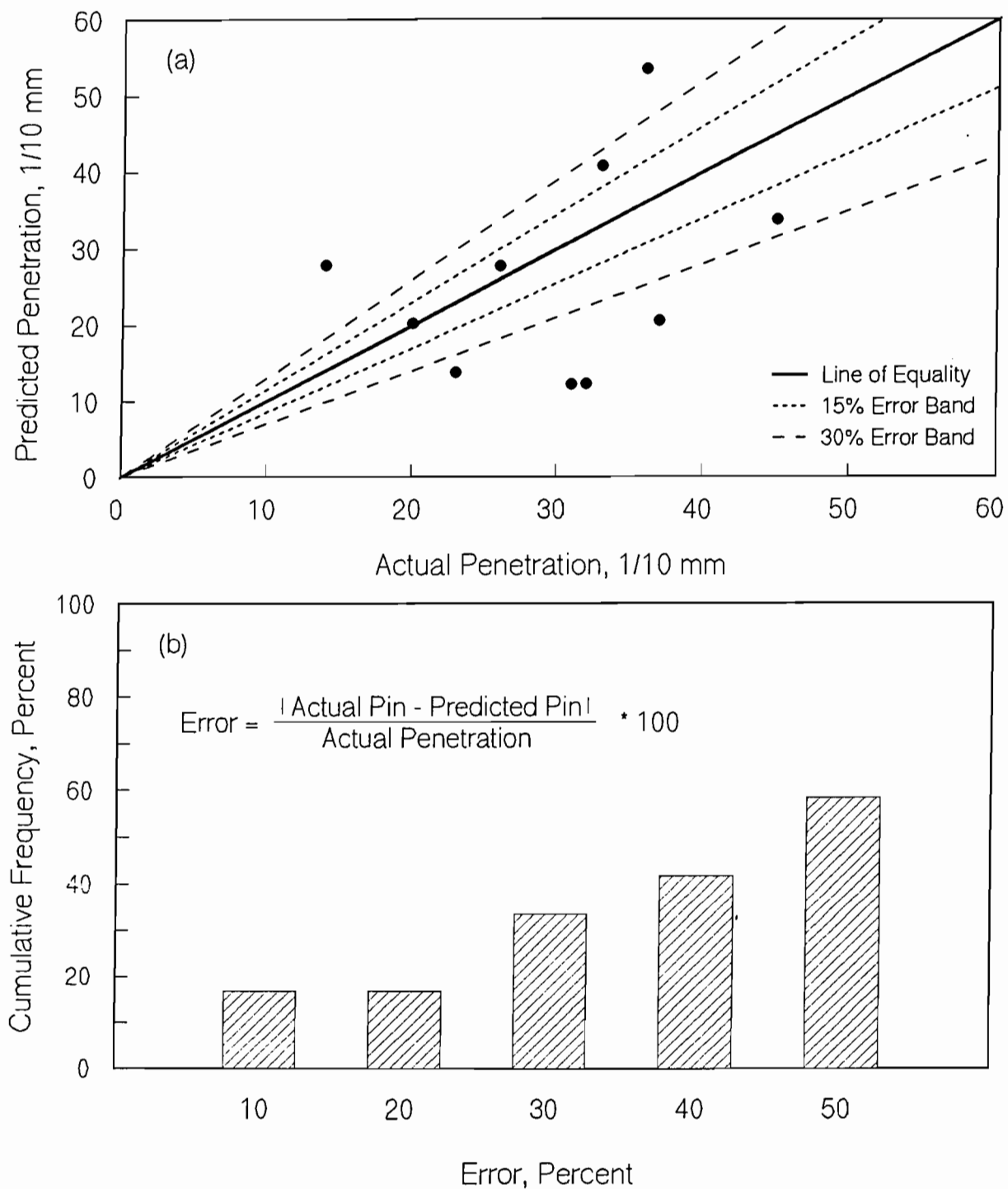
Figure F.14 Comparison of Actual and Predicted Penetration Values Using Equation 5.1 for Austin Data with 5 percent VTM (without Outliers) a) Scatter Plot, b) Cumulative Percent Error.
