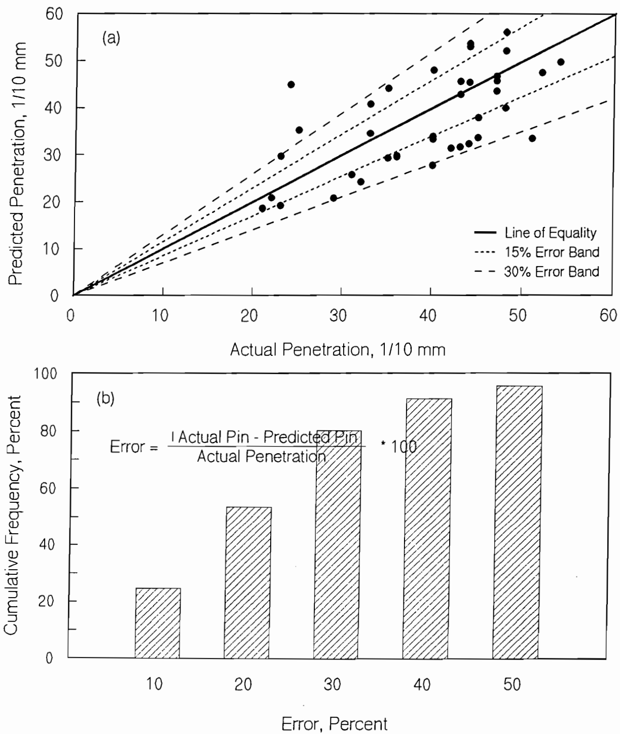
Figure F.8 Comparison of Actual and Predicted Penetration Values Using Equation 5.1 for El Paso Data a) Scatter Plot, b) Cumulative Percent Error.
