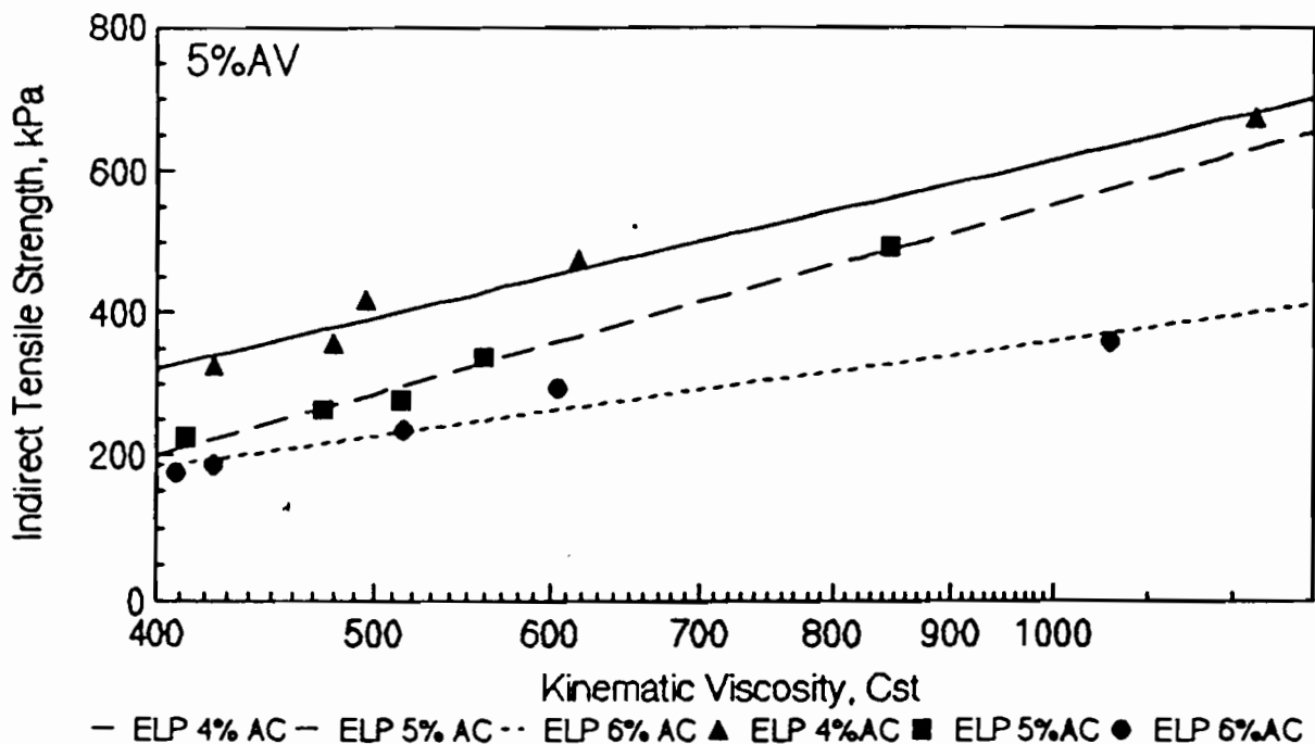
E.4 Effect of Asphalt Content on the Relationship between IDT Strength and Kinematic Viscosity for El Paso Mix.
