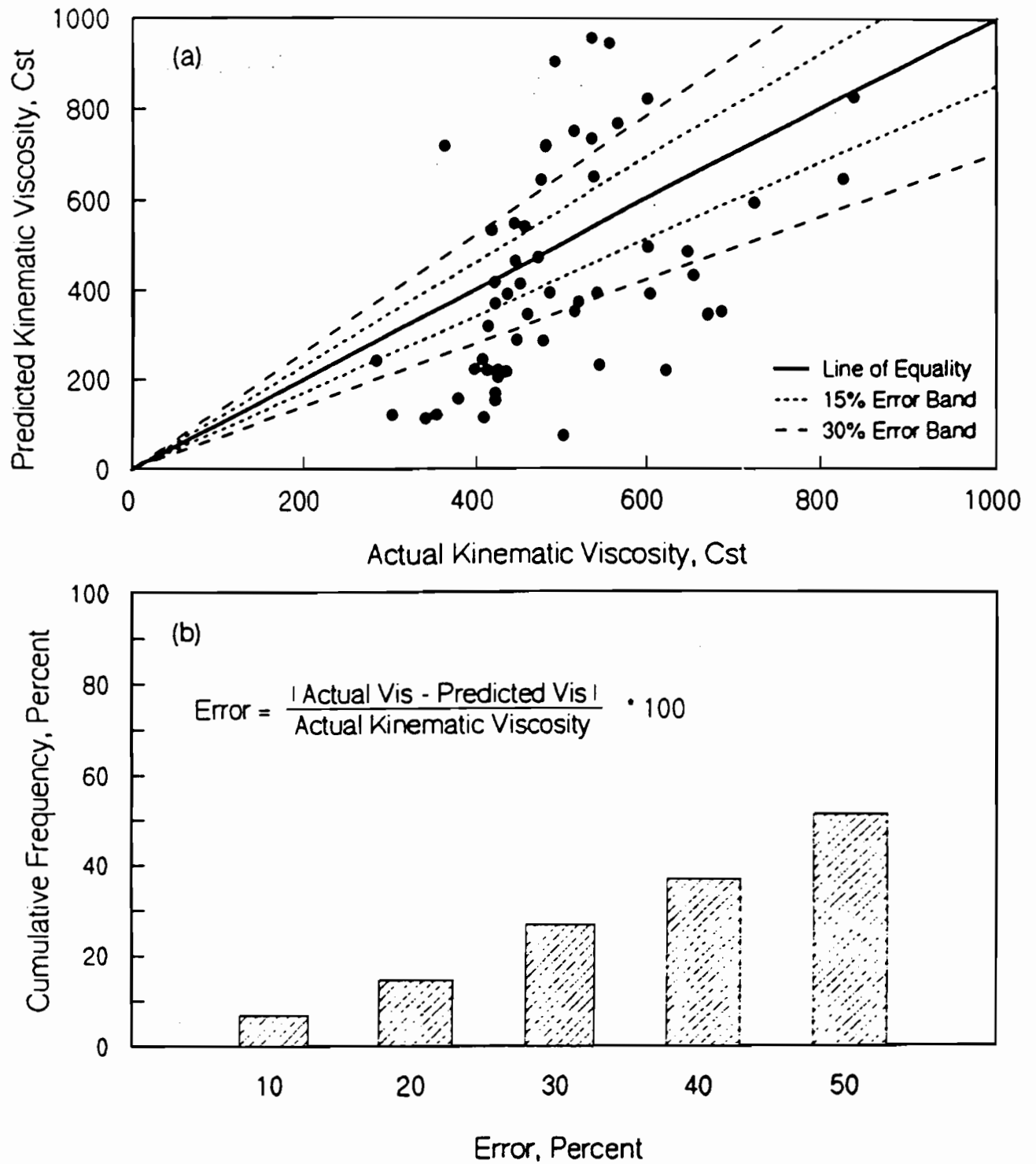
Figure 5.3 - Comparison of Actual and Predicted Kinematic Viscosity Values Using Equation 5.2 for All Data a) Scatter Plot b) Cumulative Error.
