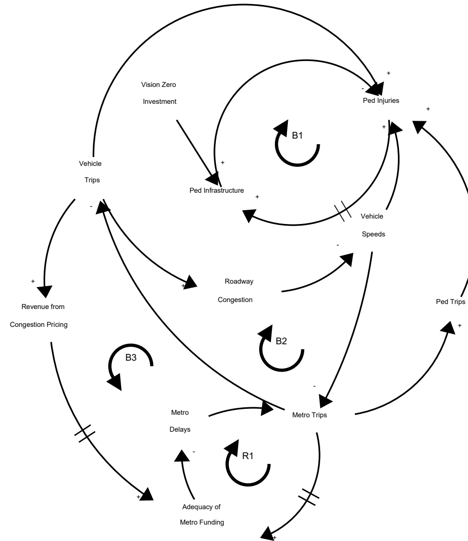
FIGURE. Causal loop diagram of feedback structure contributing to potential congestion pricing policy impacts on pedestrian injury
