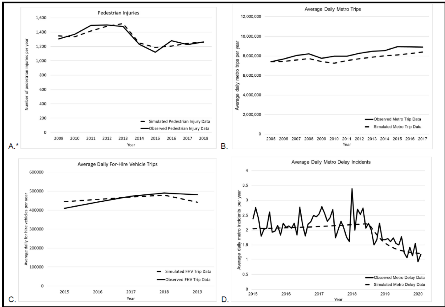
FIGURE 2. Observed vs. simulated data in congestion pricing policy-related system dynamics model
