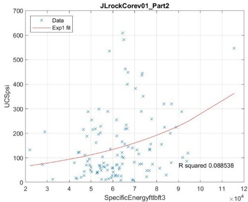
Figure 11. Single parameter exponential regression correlation results for UCS versus (a) depth, (b) down pressure, (c) torque, (d) rotation speed (e) moving speed and (f) specific energy. R^2 values are tabulated in Table 10.
