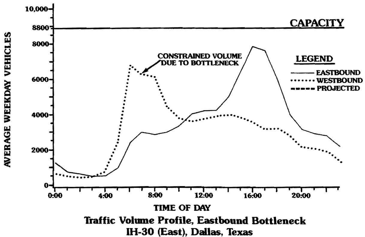
Figure 1. Daily Traffic Volume Profiles
