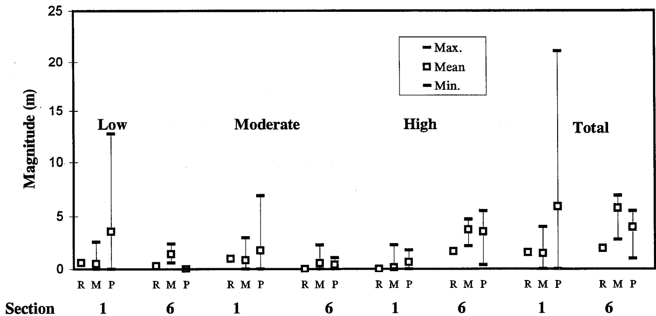
Figure 326. Spalling of Transverse Joints (Meters) - PCC Pavements: Reference, Minimum, Mean, and Maximum Values of Individual Surveys for Manual and PASCO/PADIAS.
