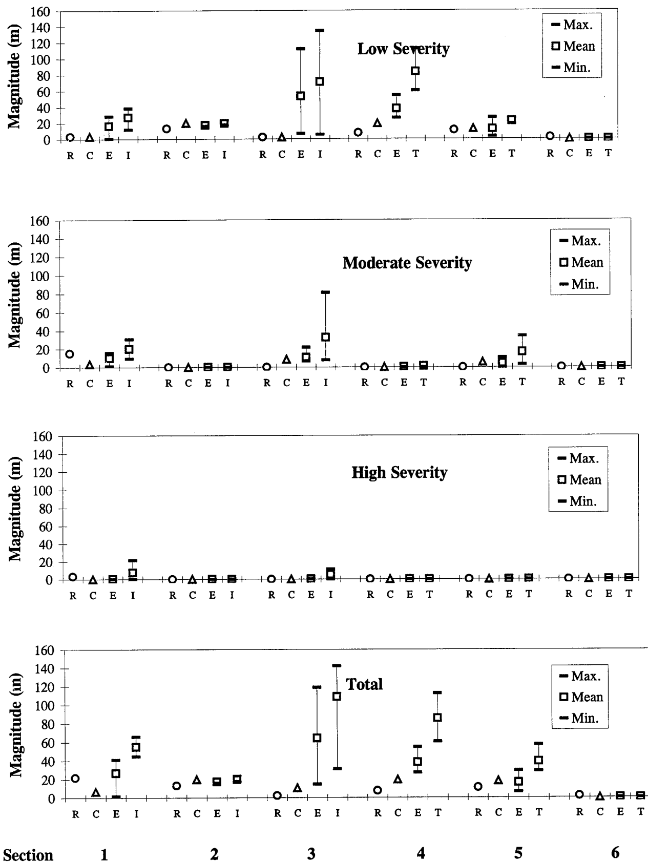
Figure 176. Longitudinal Cracking WP (Meters) - AC Pavements, PASCO/PADIAS: Reference, Consensus, Experts, Individuals, & Teams.
