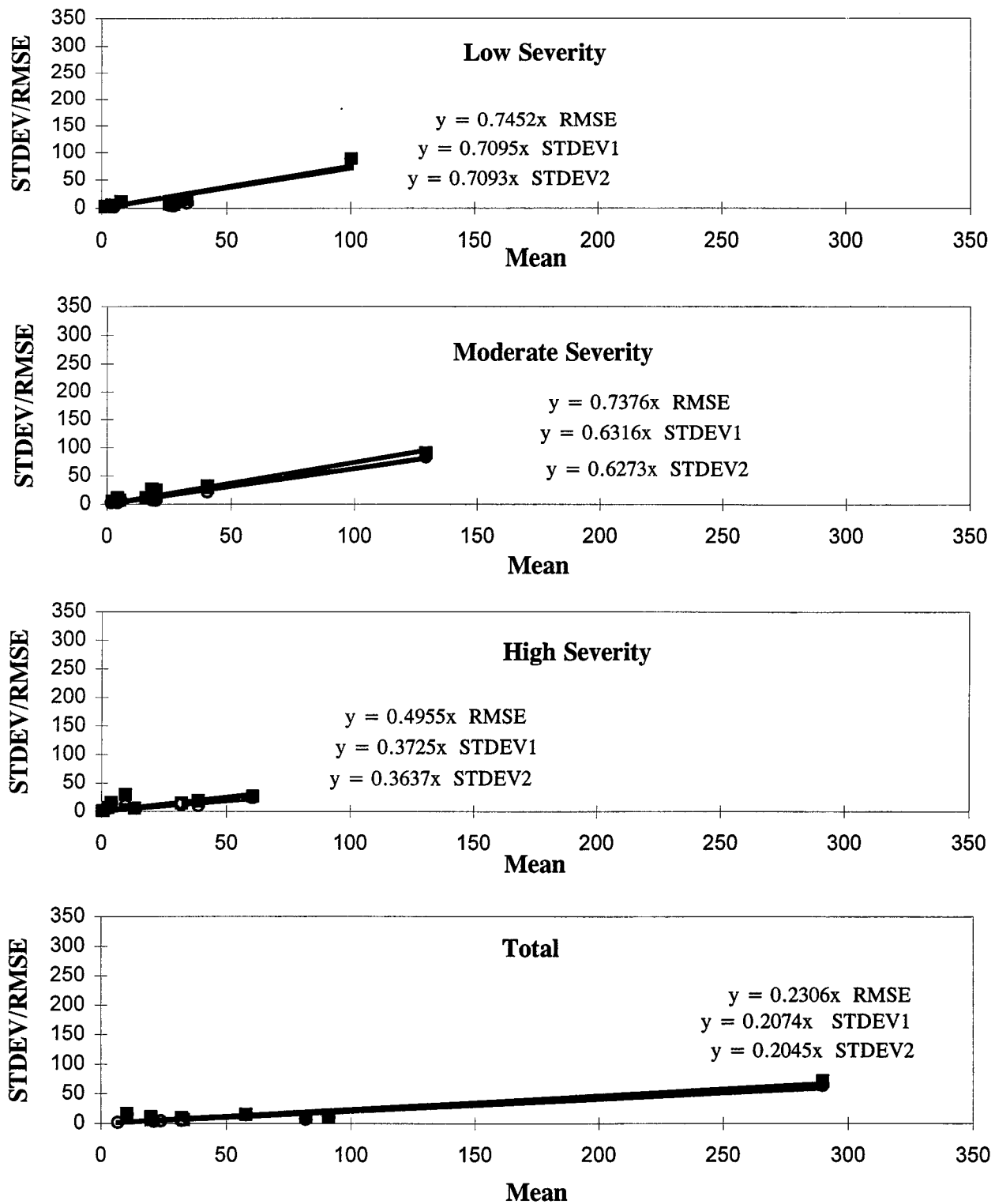
Figure 24. Longitudinal Cracking NWP (Meters) - AC Pavements, Manual Surveys: Standard Deviation/RMSE Vs. Mean.
