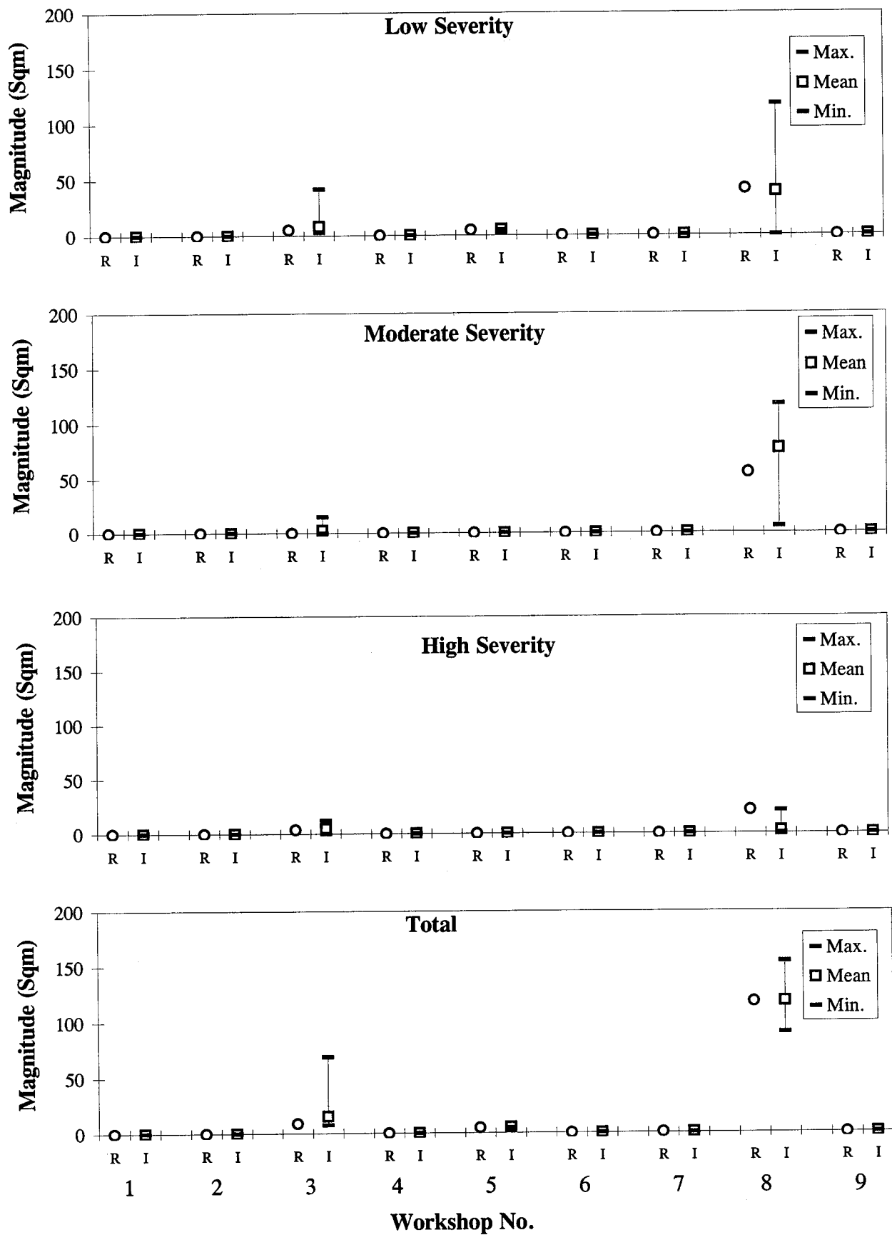
Figure 21. Patch/Patch Deterioration Rigid (Sq. Meters) - PCC Pavements, Manual Surveys: Reference and Individual Minimum, Mean, and Maximum Values.
