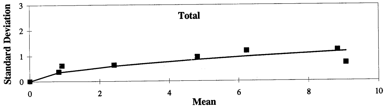
Figure 39. Corner Breaks (No.) - PCC Pavements, Manual Surveys: Standard Deviation Vs. Mean.
