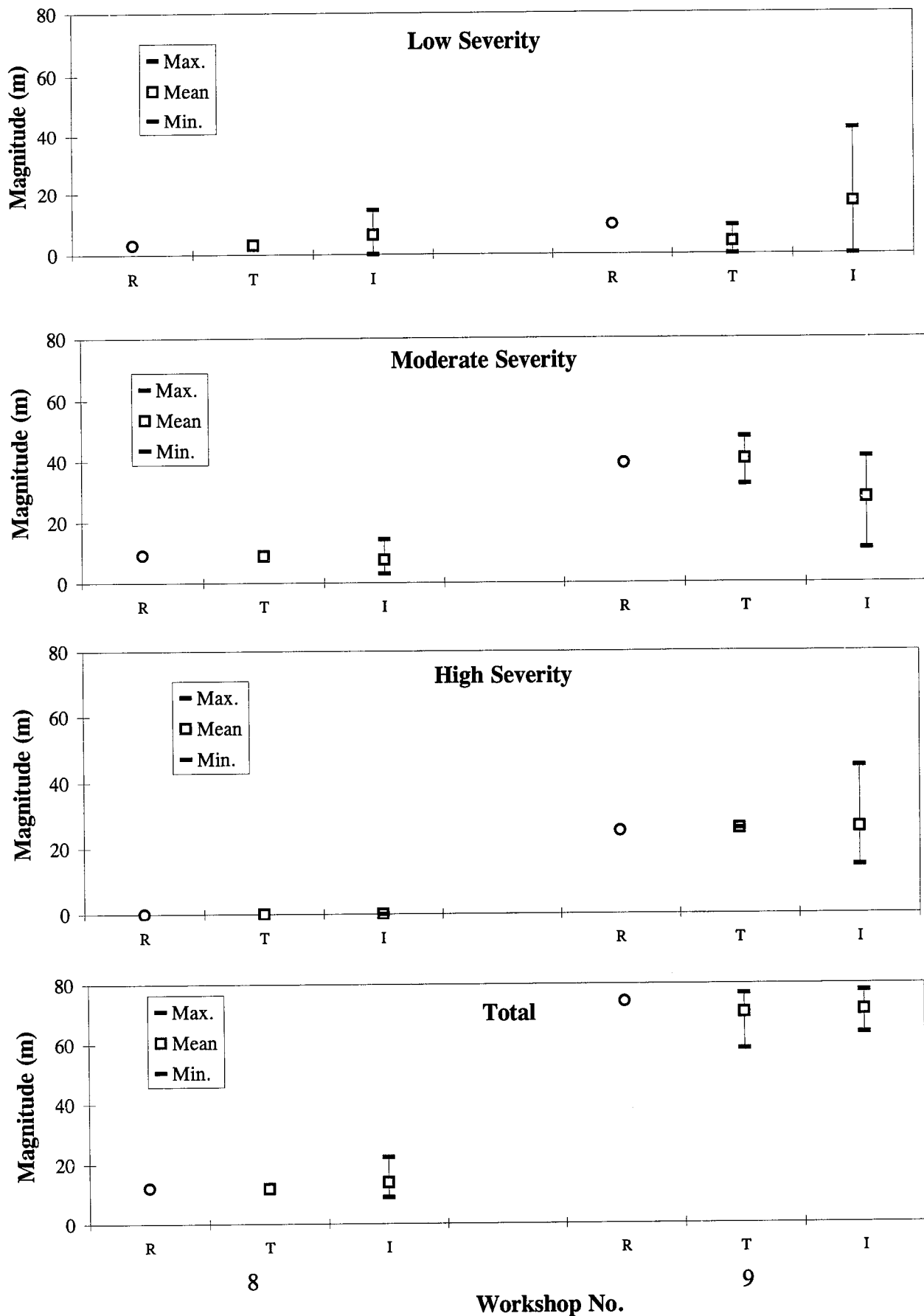
Figure 58. Transverse Cracking (Meters) - PCC Pavements, Manual Surveys: Reference, Team, and Individual Values.
