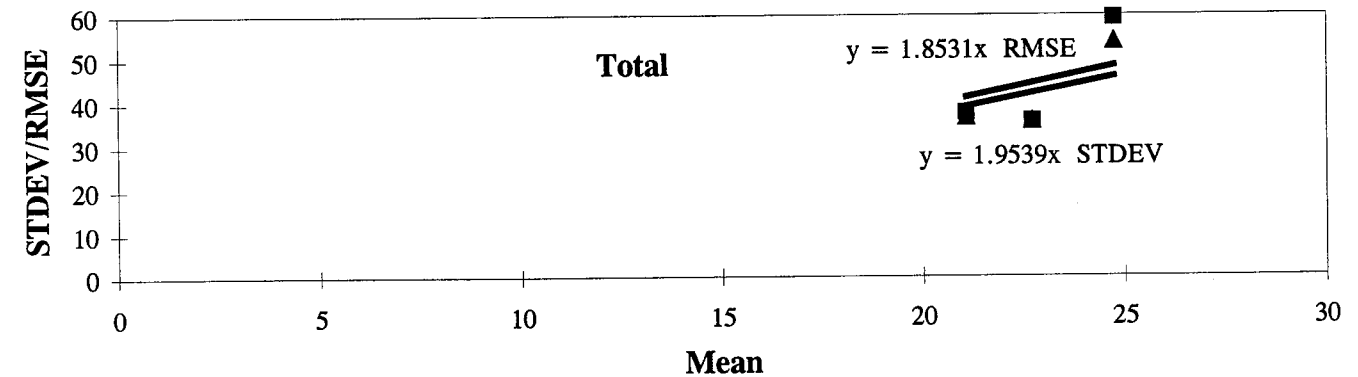
Figure 227. Longitudinal Cracking (Meters) - PCC Pavements, Individual Raters, PASCO Method: Standard Deviation/RMSE Vs. Mean.
