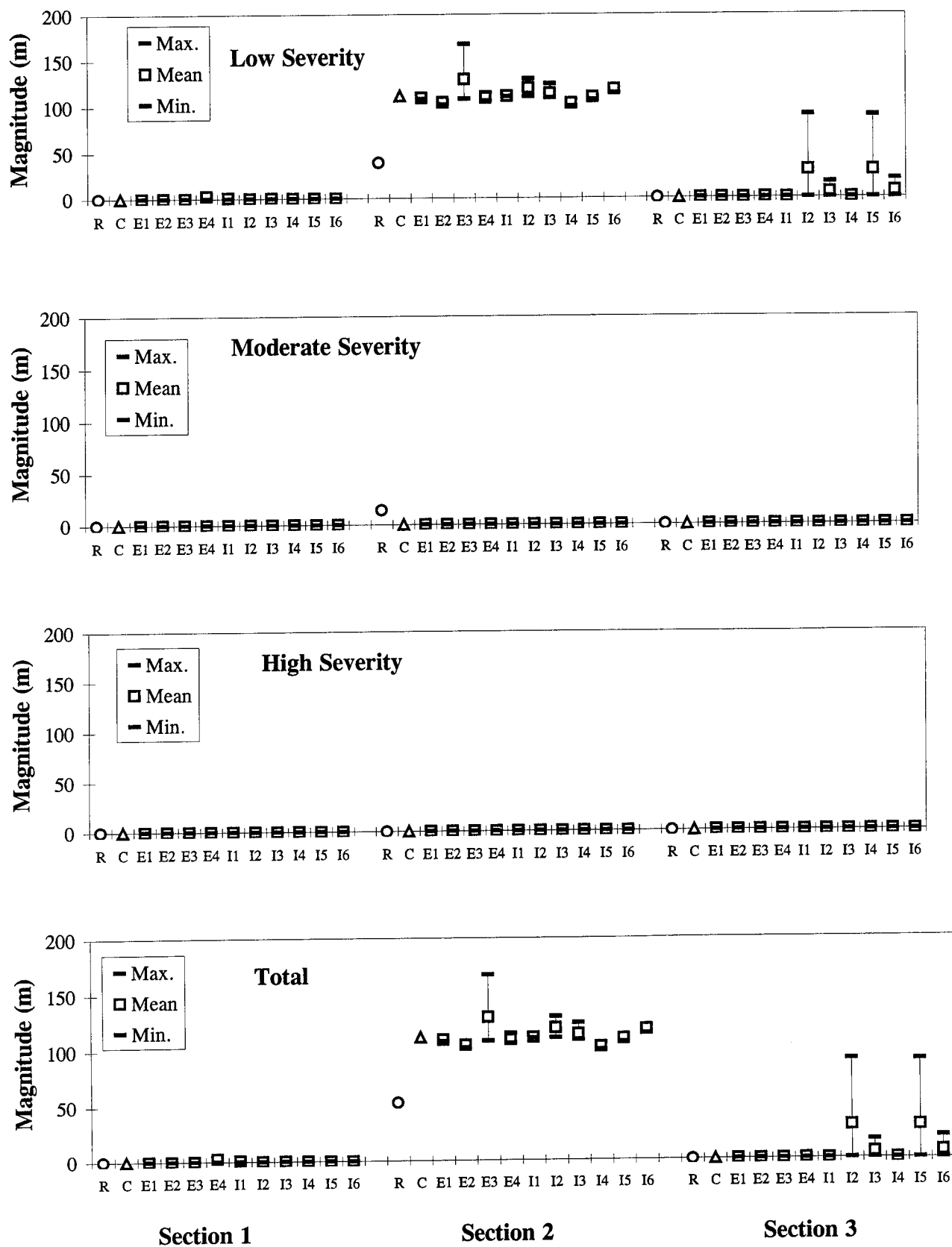
Figure 84. Transverse Cracking, Sealed (Meters) - AC Pavements, PASCO/PADIAS: Reference, Consensus, and Minimum, Mean, and Maximum Values for Experts and Individual Raters for Three Repetitions.
