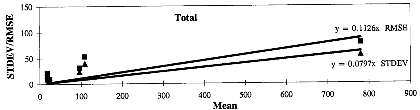
Figure 222. Transverse Cracking (Meters) - PCC Pavements, Expert Raters, PASCO Method: Standard Deviation/RMSE Vs. Mean.
