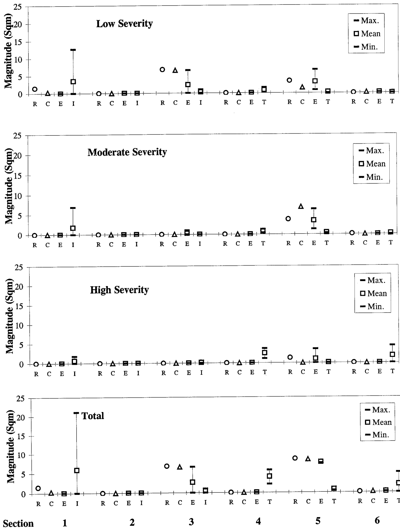
Figure 184. Patch/Patch Deterioration (Sq. Meters) - AC Pavements, PASCO/PADIAS: Reference, Consensus, Experts, Individuals, & Teams.
