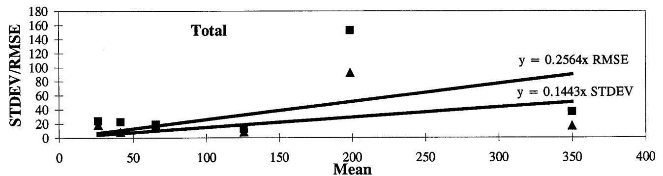
Figure 205. Longitudinal Cracking NWP (Meters) - AC Pavements, Experts, PASCO Method: Standard Deviation/RMSE Vs. Mean.
