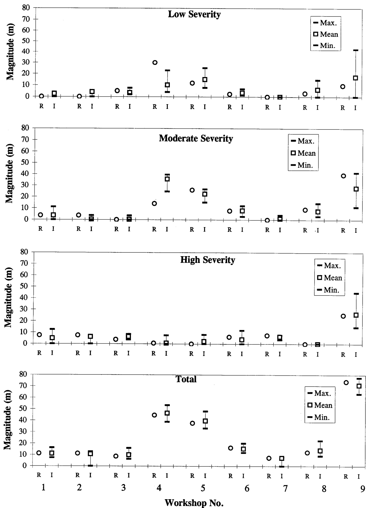
Figure 10. Transverse Cracking (Meters) - PCC Pavements, Manual Surveys: Reference and Individual Minimum, Mean, and Maximum Values.
