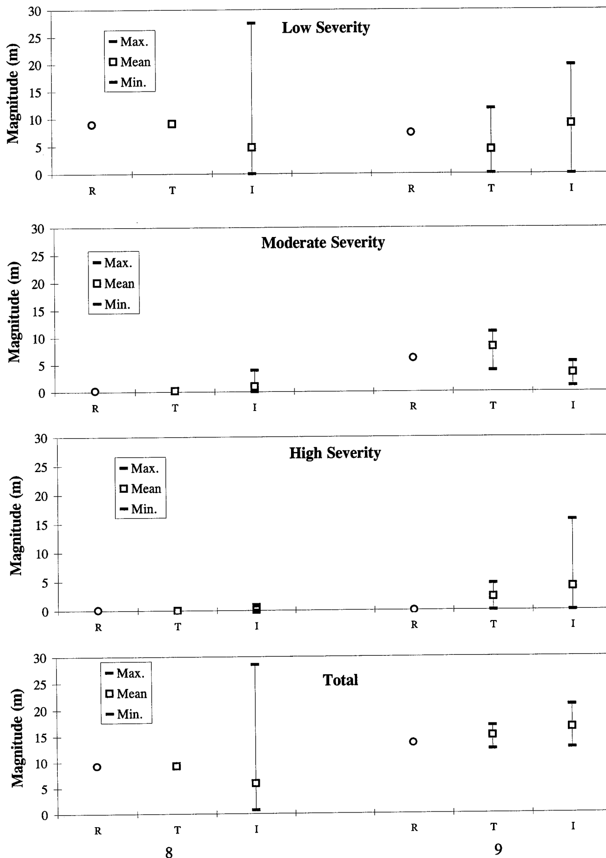
Workshop No. Figure 62. Spalling of Longitudinal Joints (Meters) - PCC Pavements, Manual Surveys: Reference, Team, and Individual Values.
