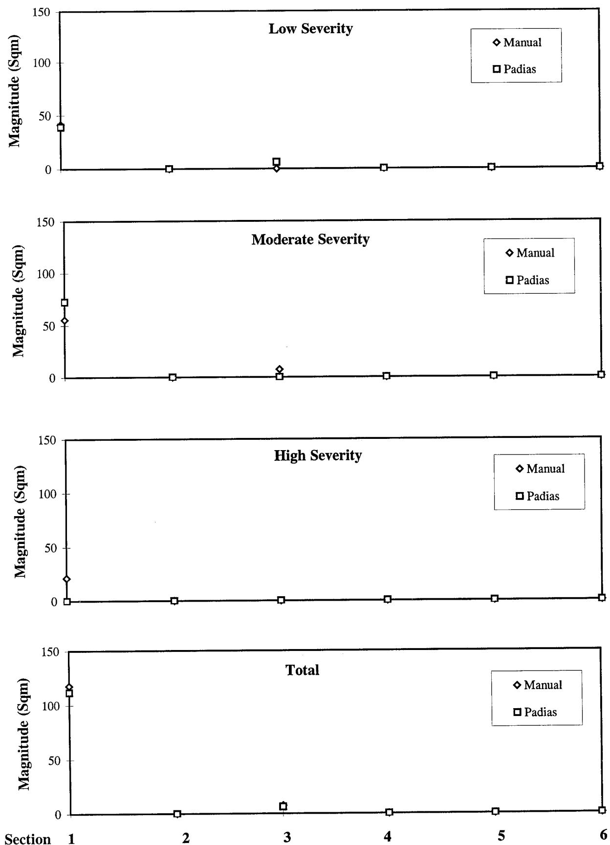
Figure 358. Patch/Patch Deterioration, Rigid (Sq. Meters) - PCC Pavements: Manual (Reference) and PASCO/PADIAS (Consensus).
