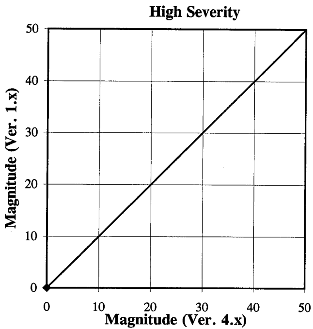
Figure 262. Comparison of PADIAS v1.x and v4.x - JPC Pavements, PCC Patch (Sq. Meters).
