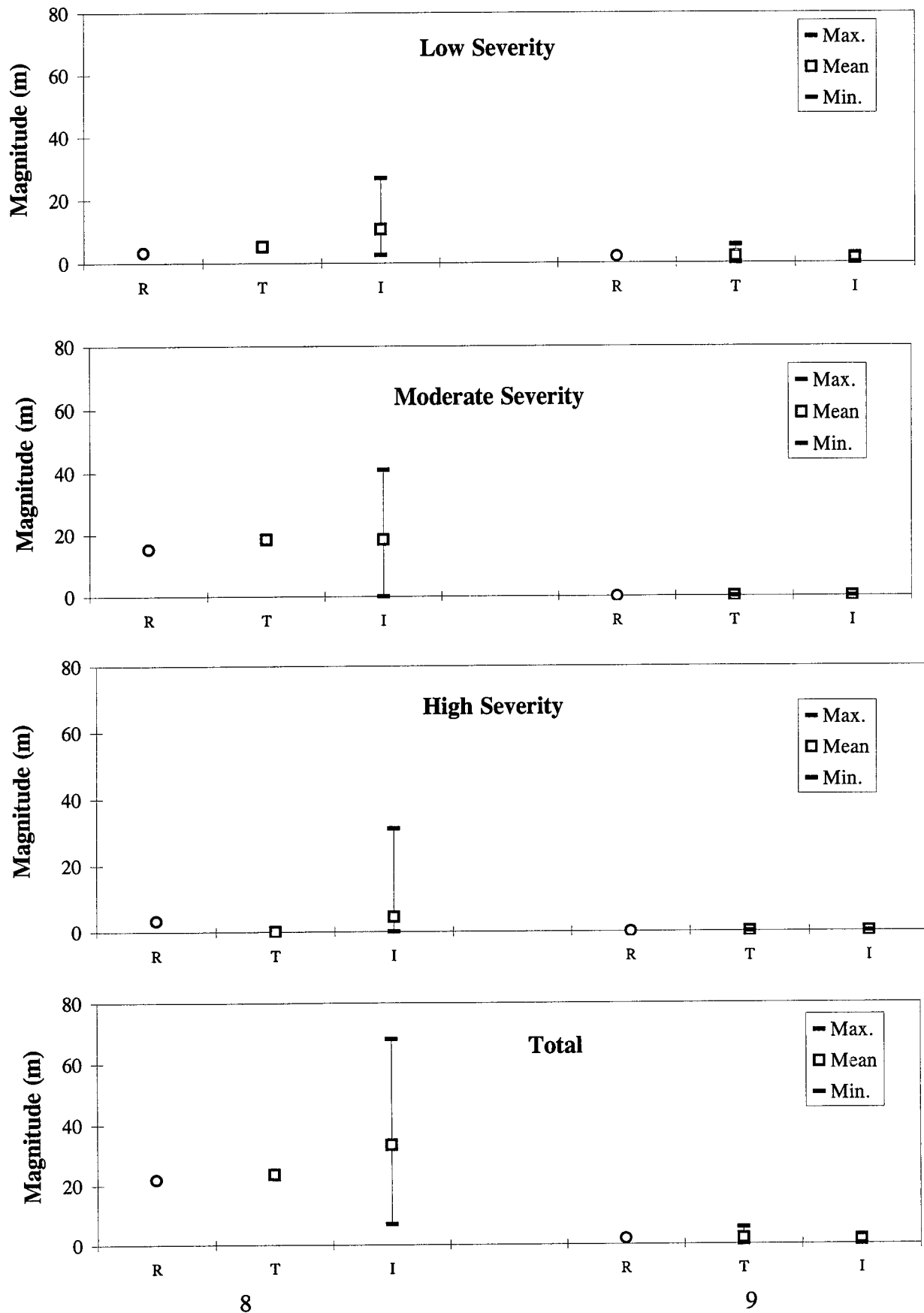
Workshop No. Figure 47. Longitudinal Cracking WP (Meters) - AC Pavements, Manual Surveys: Reference, Team, and Individual Values.
