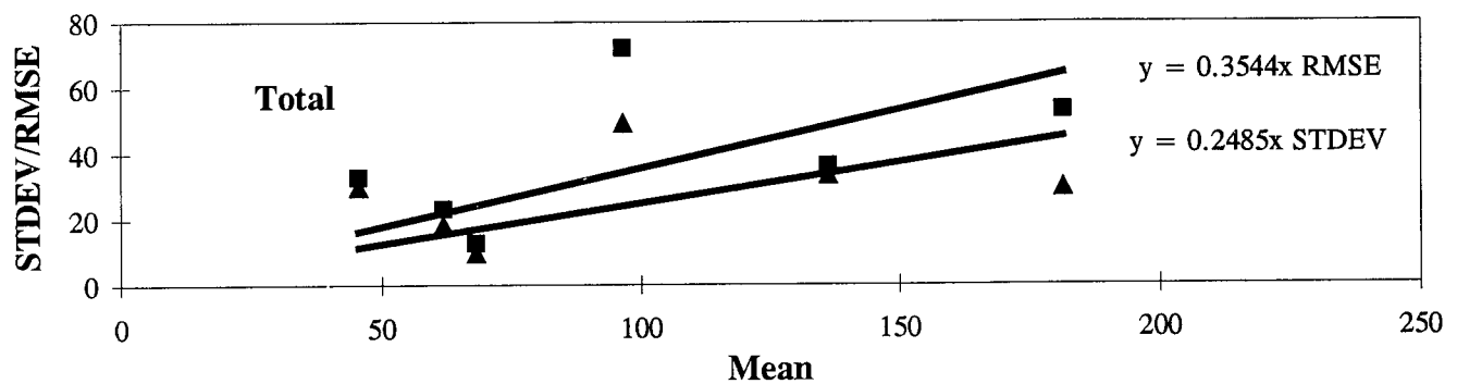
Figure 208. Transverse Cracking (Meters) - AC Pavements, Experts, PASCO Method: Standard Deviation/RMSE Vs. Mean.
