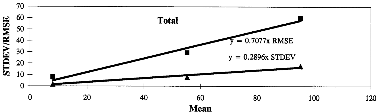
Figure 217. Transverse Cracking (No.) - AC Pavements, Teams: Standard Deviation/RMSE Vs. Mean.
