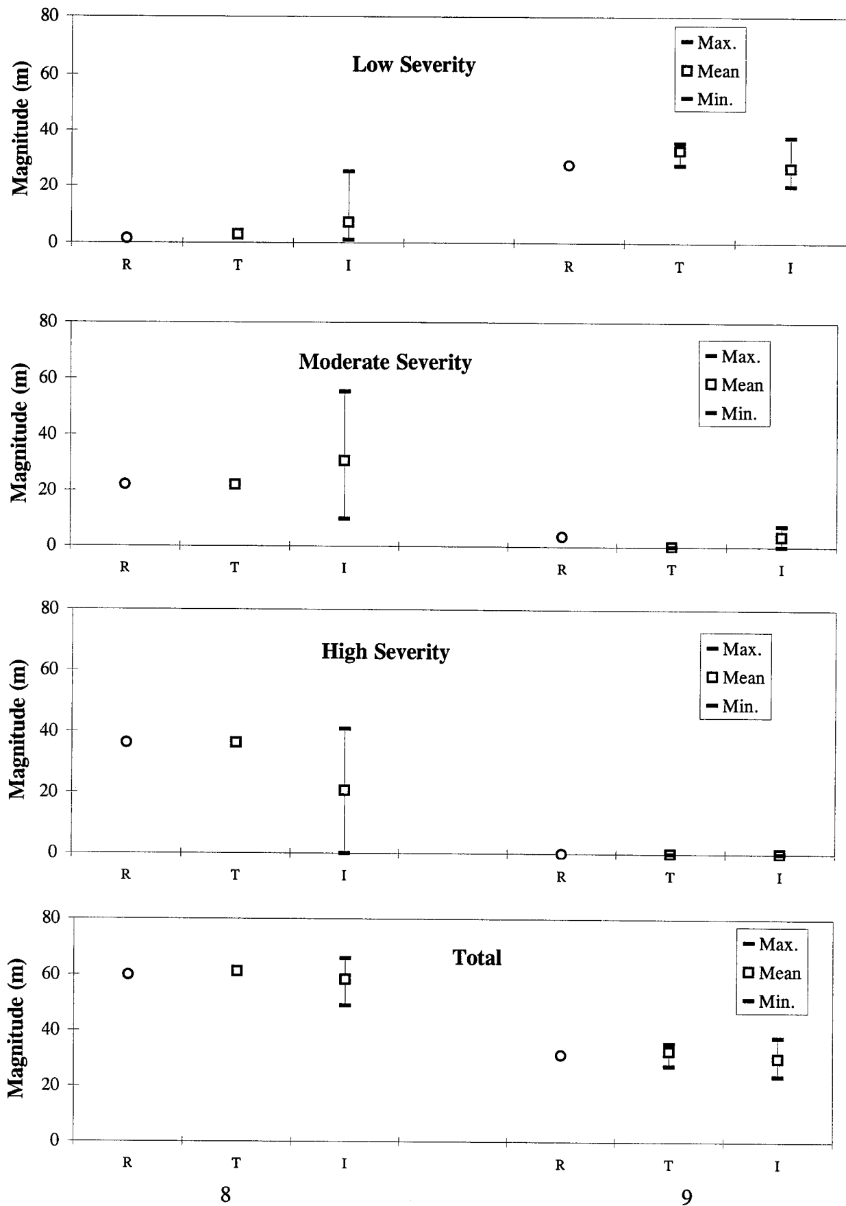
Workshop No. 8 9 Figure 50. Transverse Cracking (Meters) - AC Pavements, Manual Surveys: Reference, Team, and Individual Values.
