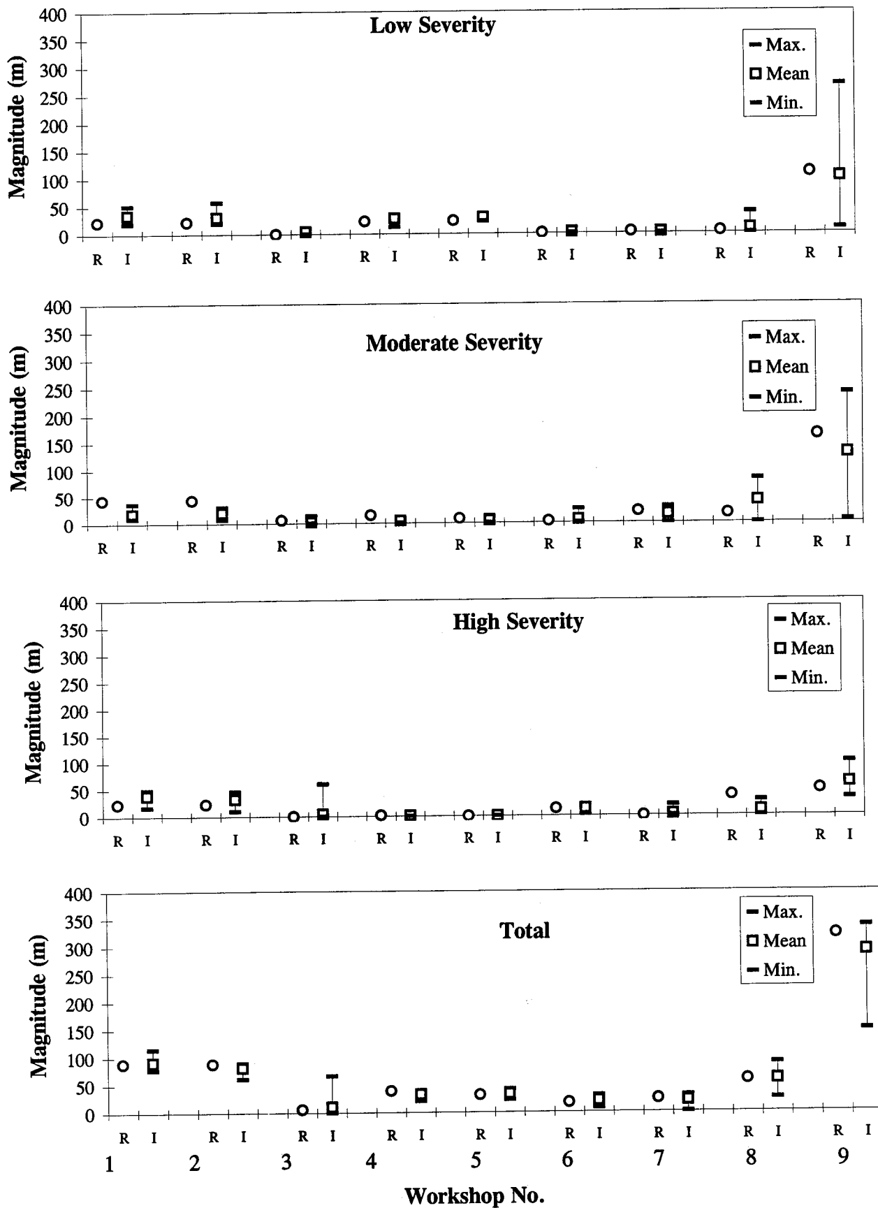
Figure 3. Longitudinal Cracking NWP (Meters) - AC Pavements, Manual Surveys: Reference and Individual Minimum, Mean, and Maximum Values.
