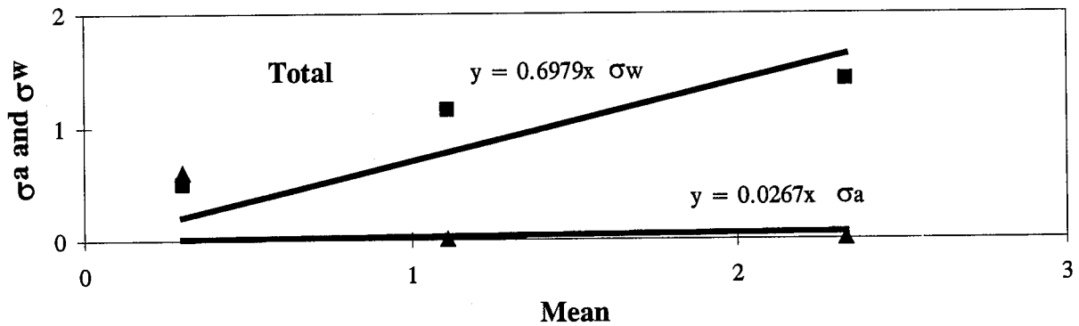
Figure 172. Spalling of Transverse Joints (No.) - PCC Pavements, Teams, PASCO Method: \sigma_a and \sigma_w Vs. Mean.
