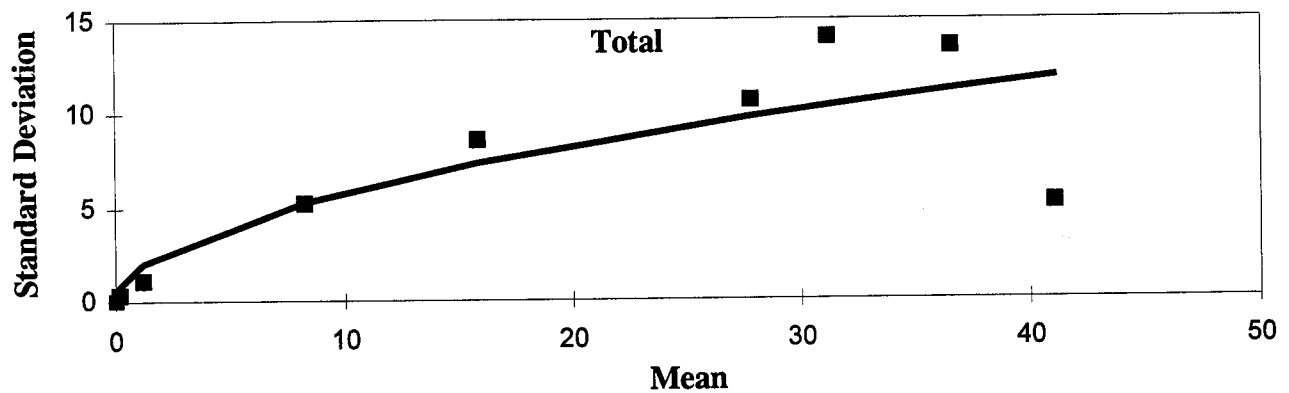
Figure 35. Longitudinal Cracking WP (Meters) - AC Pavements, Manual Surveys: Standard Deviation Vs. Mean.
