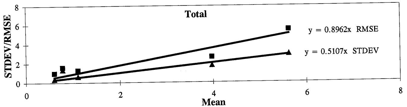
Figure 225. Spalling of Transverse Joints (Meters) - PCC Pavements, Expert Raters, PASCO Method: Standard Deviation/RMSE Vs. Mean.
