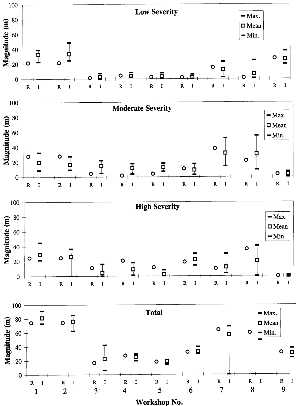
Figure 5. Transverse Cracking (Meters) - AC Pavements, Manual Surveys: Reference and Individual Minimum, Mean, and Maximum Values.
