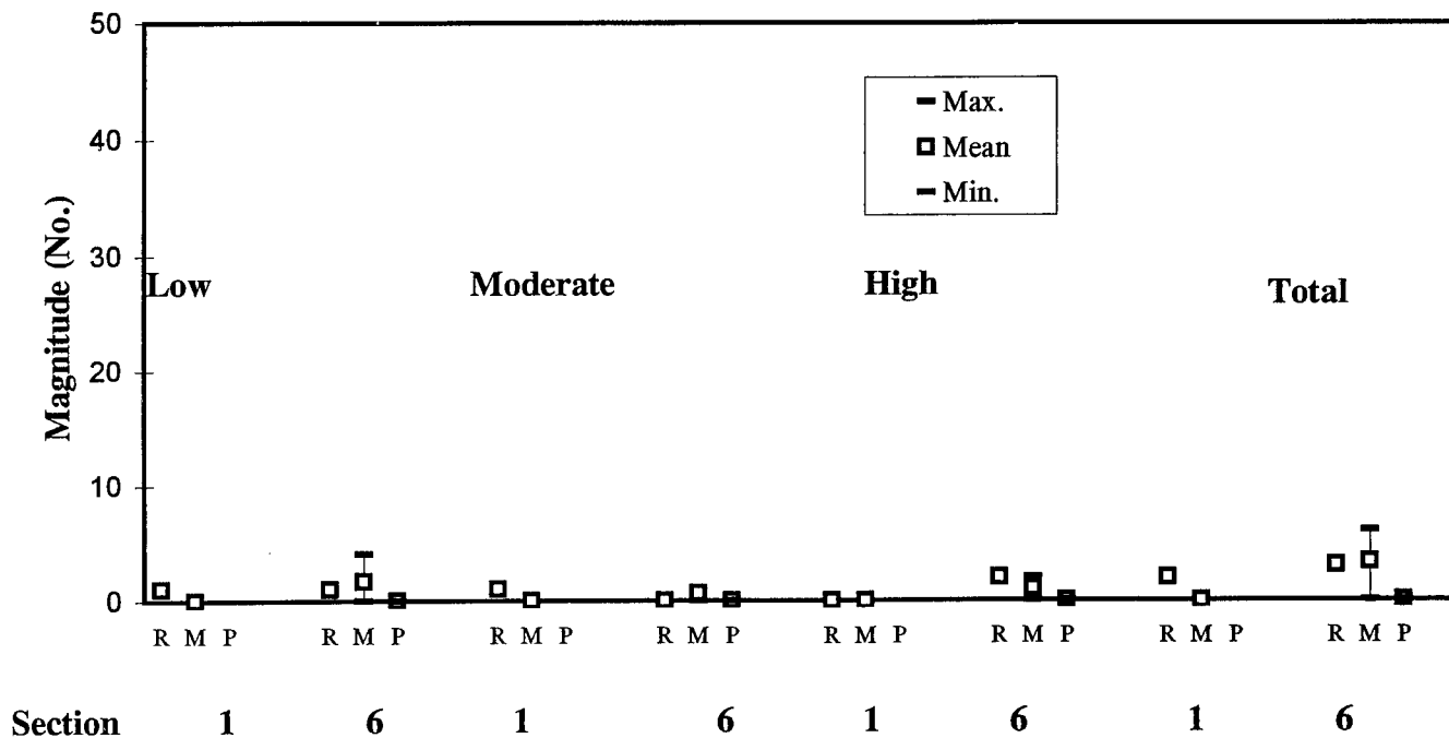
Figure 325. Spalling of Transverse Joints (No.) - PCC Pavements: Reference, Minimum, Mean, and Maximum Values of Team Surveys for Manual and PASCO/PADIAS.
