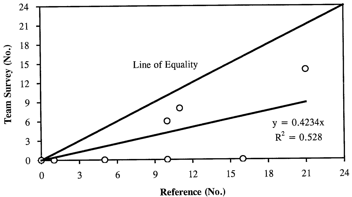
Figure 293. Team Survey Vs. Reference and Consensus: Corner Break of PCC Pavement, PASCO's Production Procedure.
