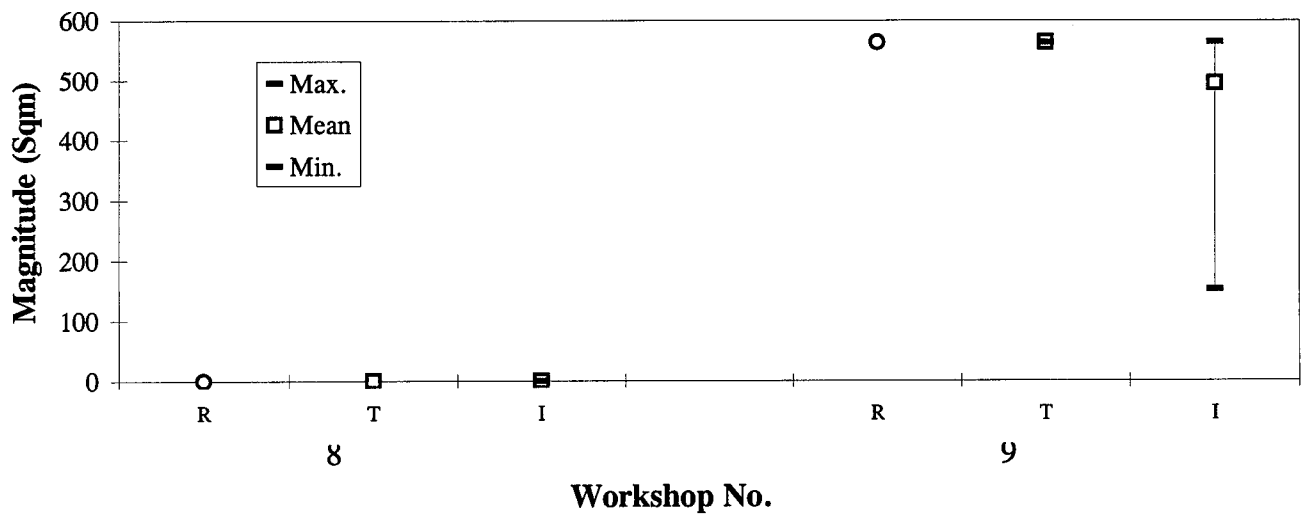
Figure 66. Map Cracking (Sq. Meters) - PCC Pavements, Manual Surveys: Reference, Team, and Individual Values.
