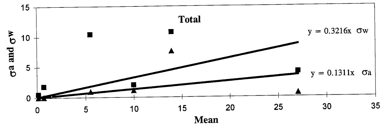
Figure 154. Longitudinal Cracking (Meters) - PCC Pavements, Experts, PASCO Method: \sigma_a and \sigma_w Vs. Mean.
