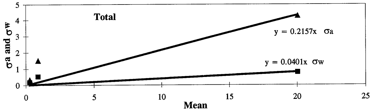
Figure 168. Longitudinal Cracking (Meters) - PCC Pavements, Teams, PASCO Method: \sigma_a and \sigma_w Vs. Mean.
