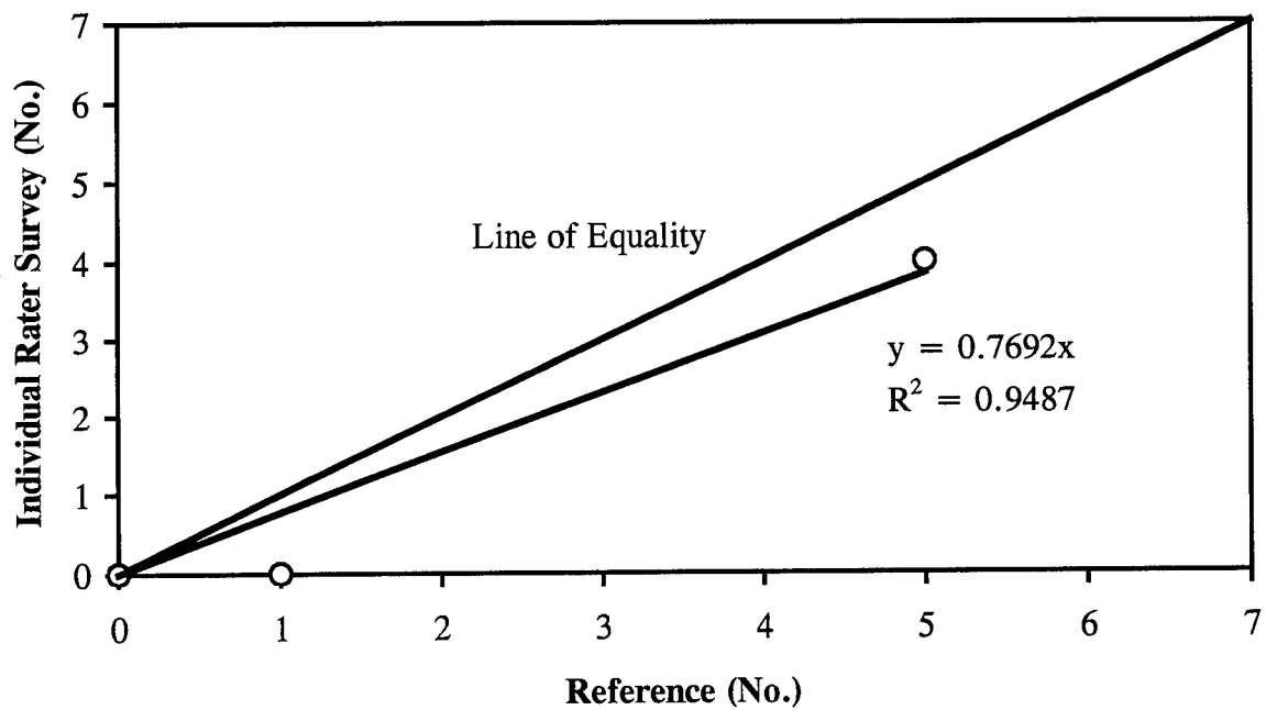
Figure 286. Individual Survey Vs. Reference and Consensus: Corner Break of PCC Pavement, PASCO's Production Procedure.
