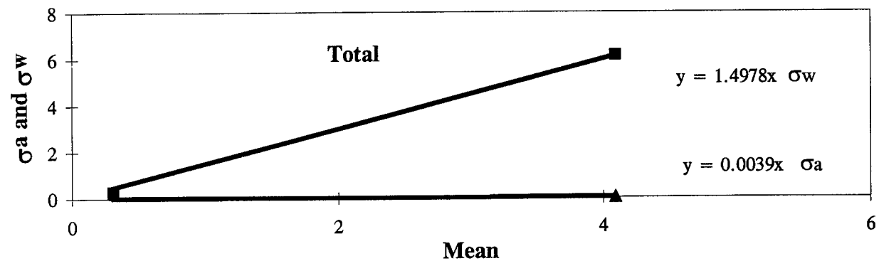
Figure 166. Spalling of Transverse Joints (Meters) - PCC Pavements, Individuals, PASCO Method: \sigma_a and \sigma_w Vs. Mean.
