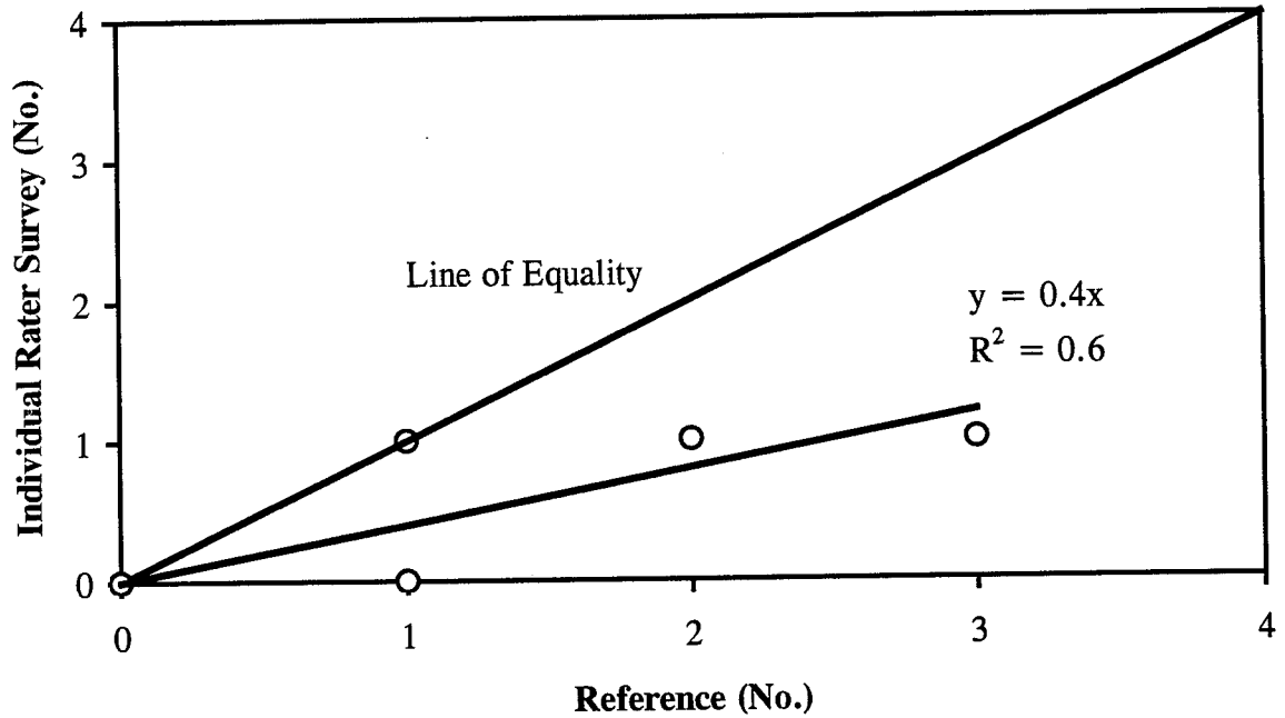
Figure 291. Individual Survey Vs. Reference and Consensus: Spalling of Transverse Joints (No.) of PCC Pavement, PASCO's Production Procedure.
