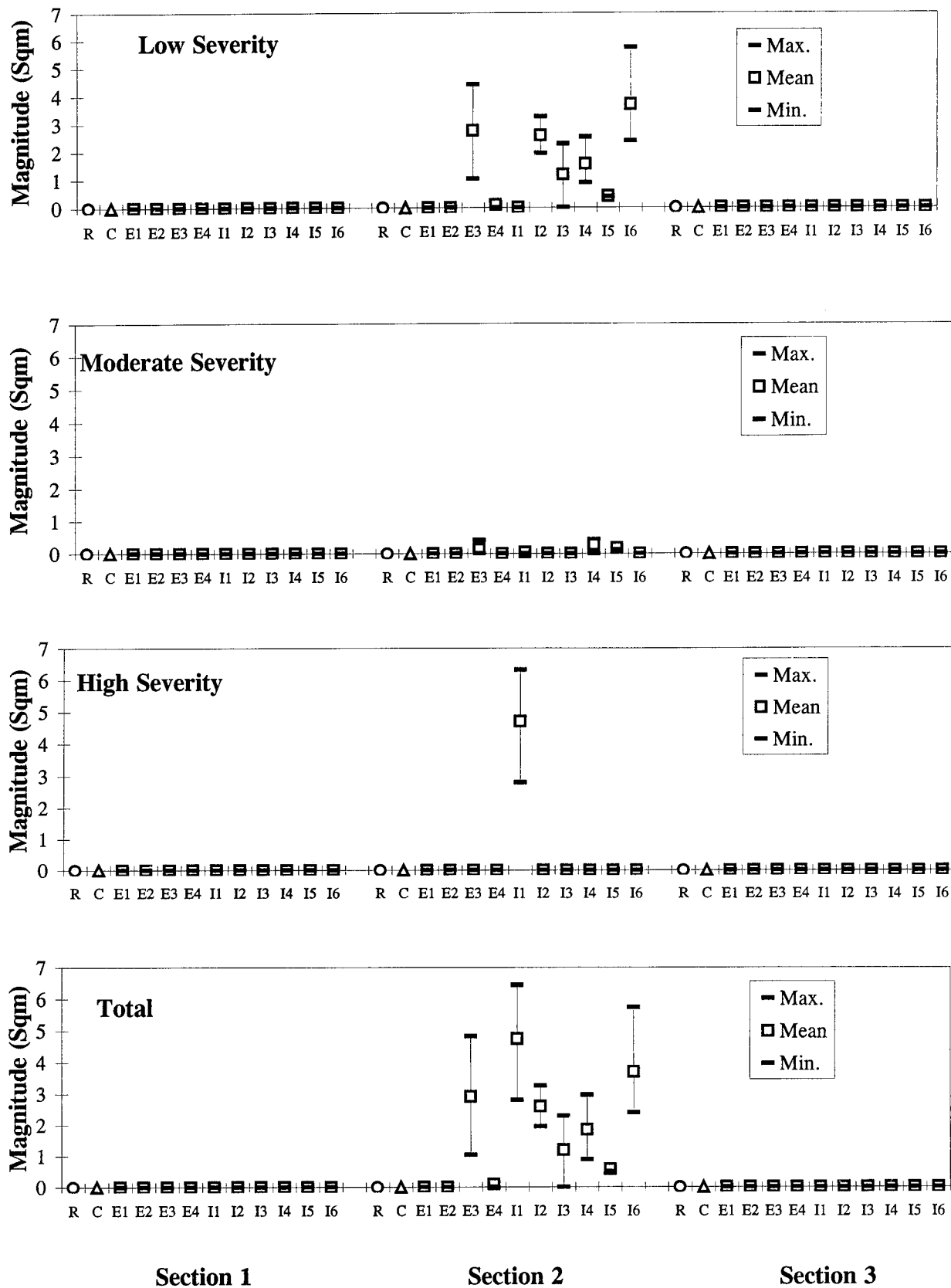
Figure 117. Patch/Patch Deterioration Flexible (Sq. Meters) - PCC Pavements, PASCO/ PADIAS: Reference, Consensus, and Minimum, Mean, and Maximum Values for Experts and Individual Raters for Three Repetitions.
