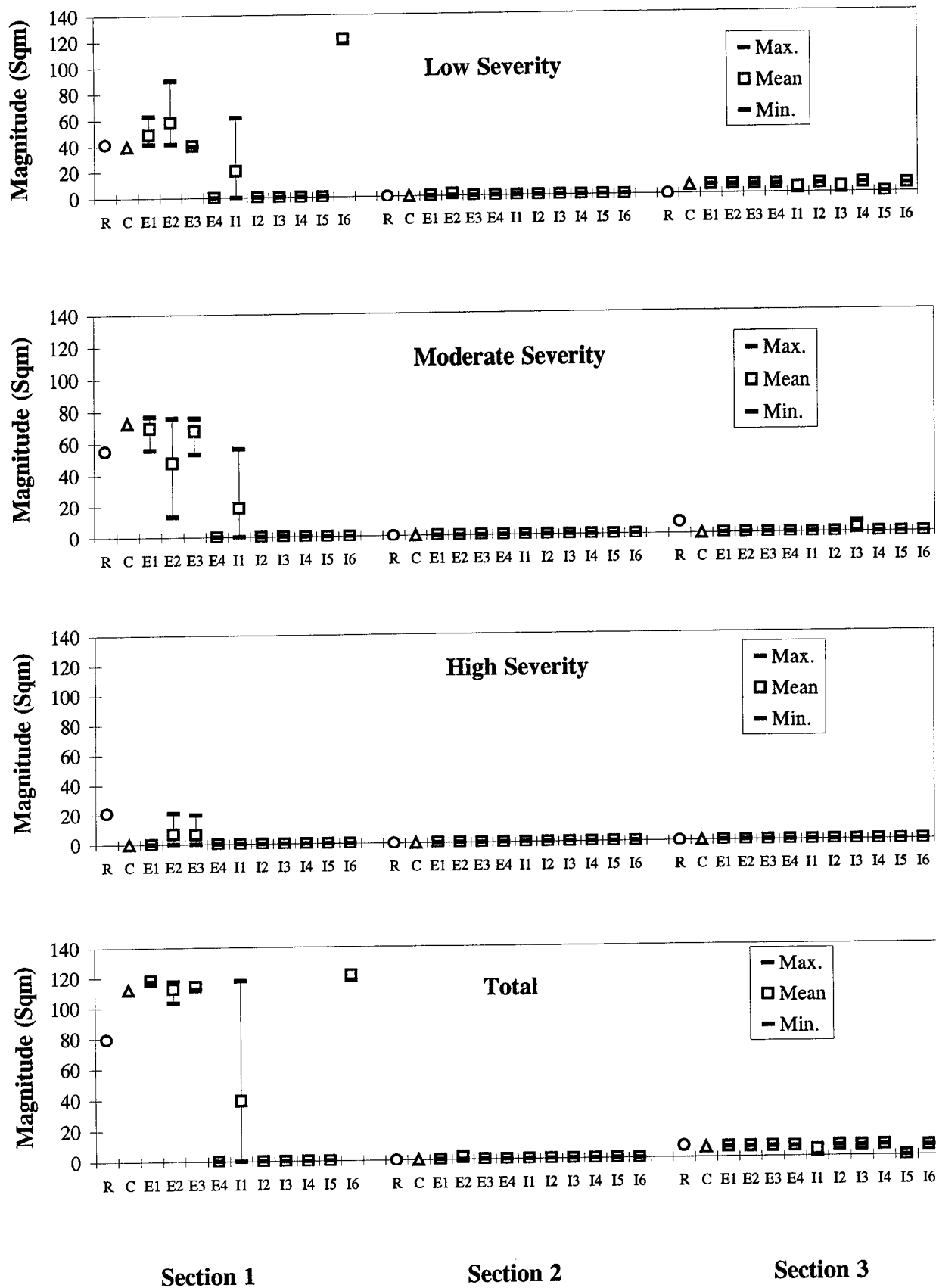
Figure 119. Patch/Patch Deterioration Rigid (Sq. Meters) - PCC Pavements, PASCO/PADIAS: Reference, Consensus, and Minimum, Mean, and Maximum Values for Experts and Individual Raters for Three Repetitions.
