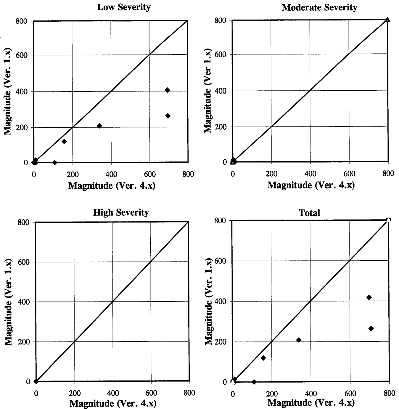
Figure 241. Comparison of PADIAS v1.x and v4.x - AC Pavements, Longitudinal Cracking (Meters).
