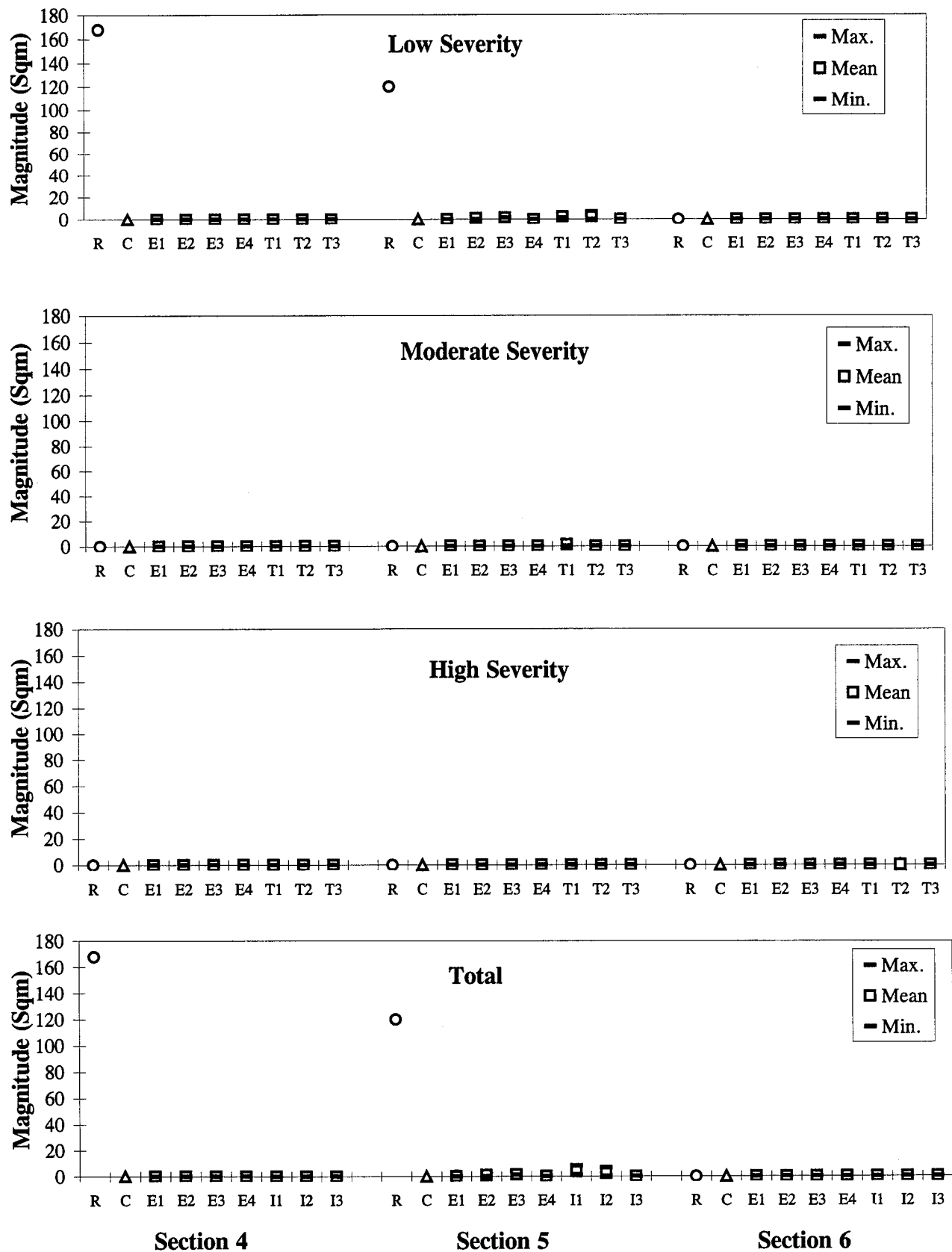
Figure 99. Bleeding (Sq. Meters) - AC Pavements, PASCO/PADIAS: Reference, Consensus, and Minimum, Mean, and Maximum Values for Experts and Teams for Three Repetitions.
