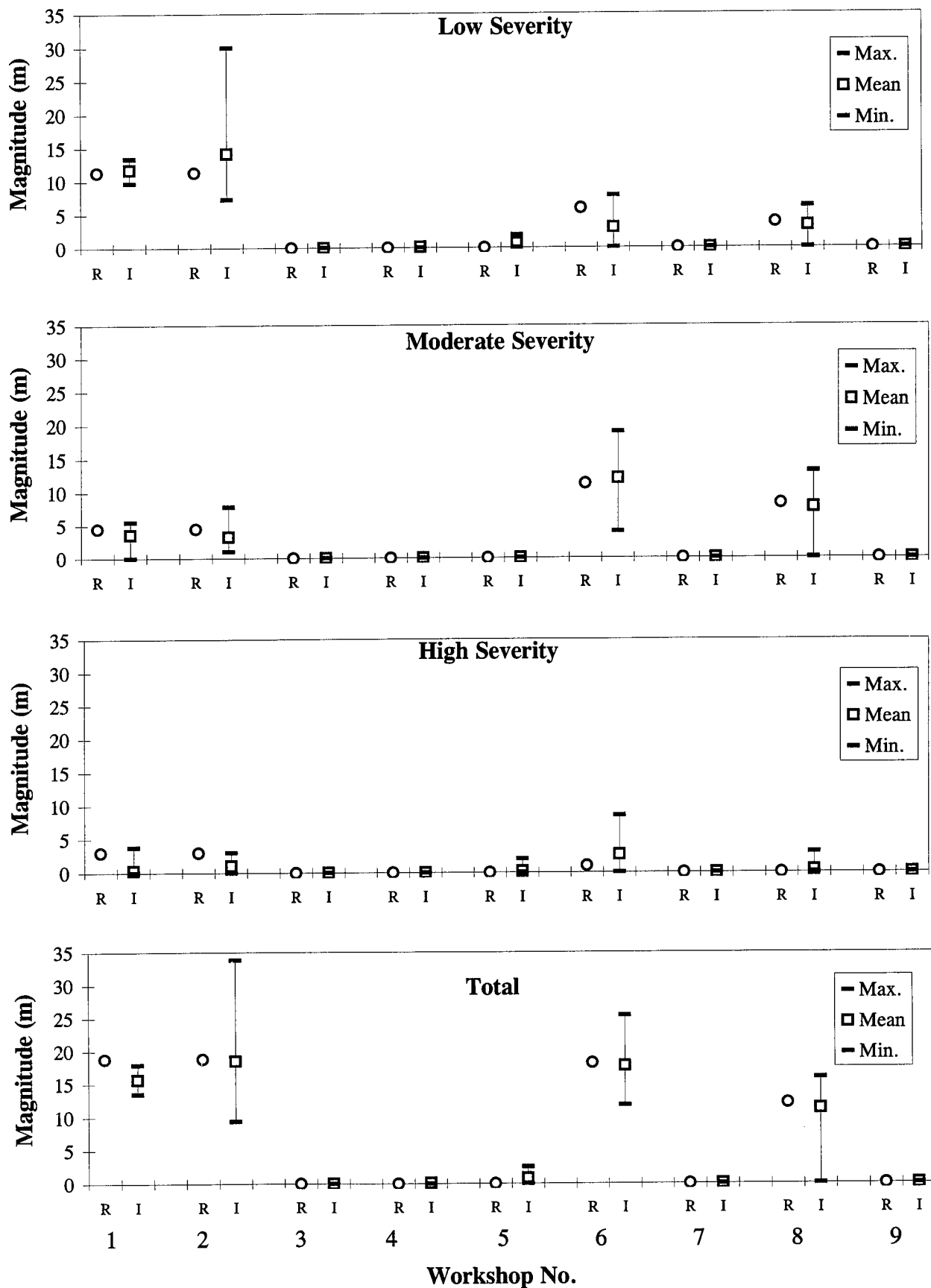
Figure 7. Longitudinal Cracking (Meters) - PCC Pavements, Manual Surveys: Reference and Individual Minimum, Mean, and Maximum Values.
