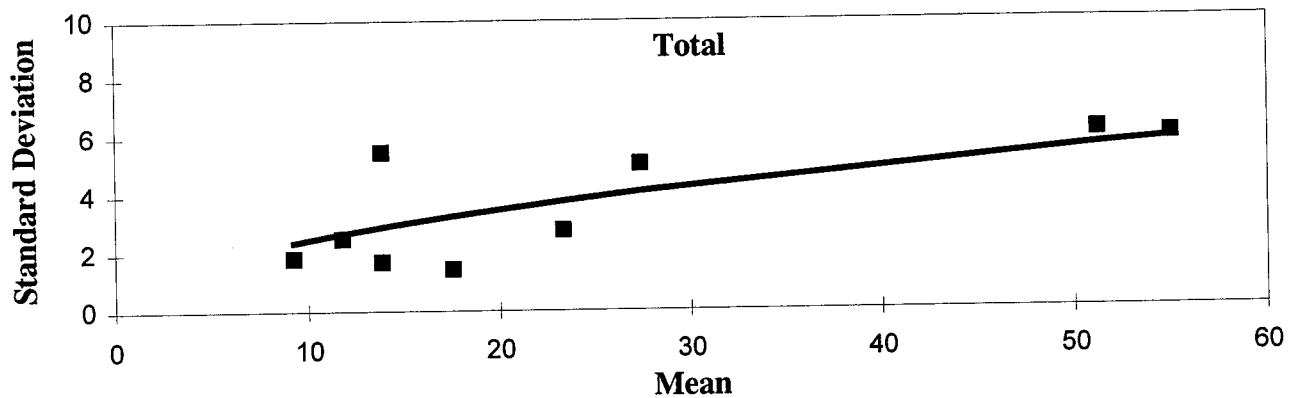
Figure 37. Transverse Cracking (No.) - AC Pavements, Manual Surveys: Standard Deviation Vs. Mean.
