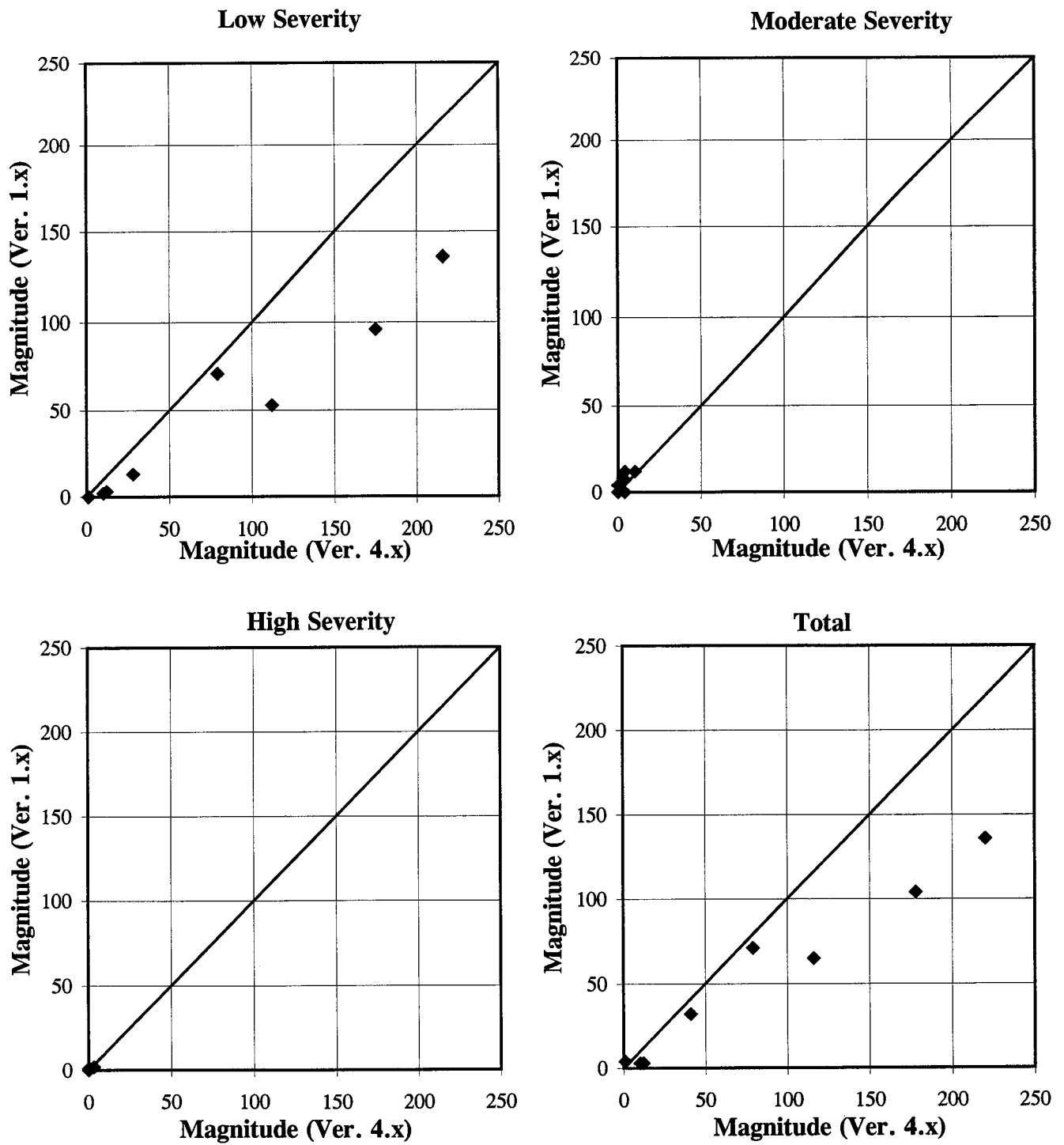
Figure 243. Comparison of PADIAS v1.x and v4.x - AC Pavements, Transverse Cracking (No.).
