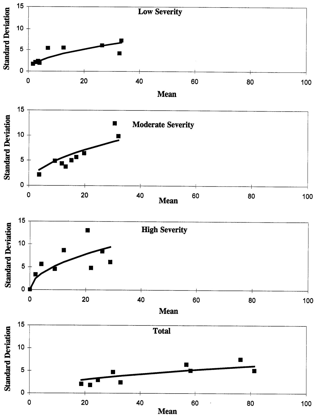
Figure 38. Transverse Cracking (Meters) - AC Pavements, Manual Surveys: Standard Deviation Vs. Mean.
