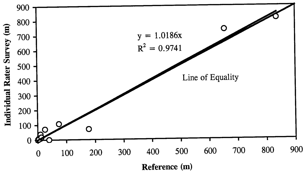
Figure 289. Individual Survey Vs. Reference and Consensus: Transverse Cracking (Meters) of PCC Pavement, PASCO's Production Procedure.
