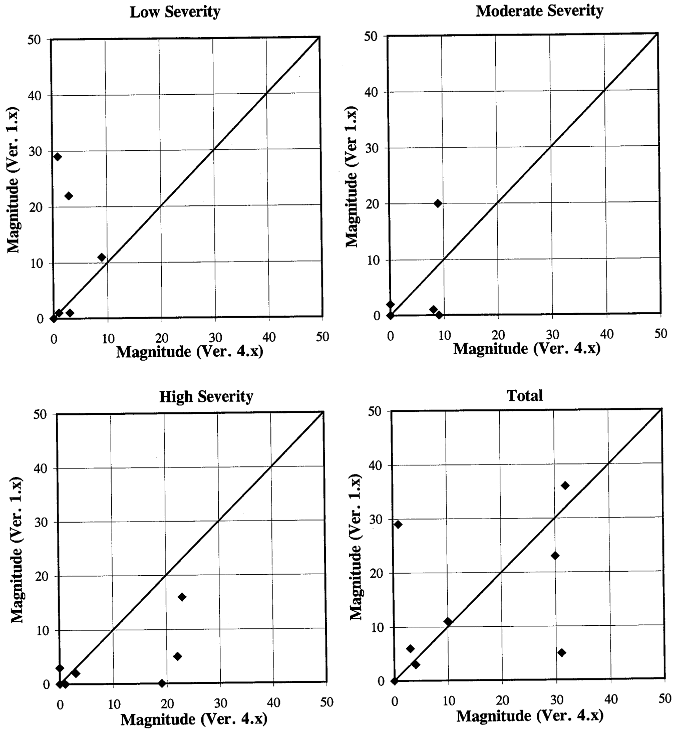
Figure 257. Comparison of PADIAS v1.x and v4.x - JPC Pavements, Spalling of Transverse Joints (No.).
