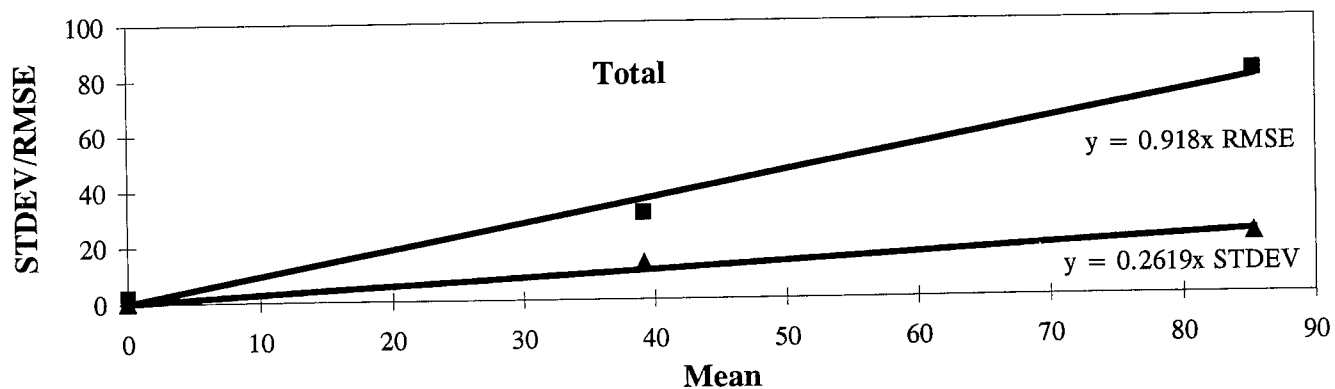
Figure 216. Longitudinal Cracking WP (Meters) - AC Pavements, Teams: Standard Deviation/RMSE Vs. Mean.
