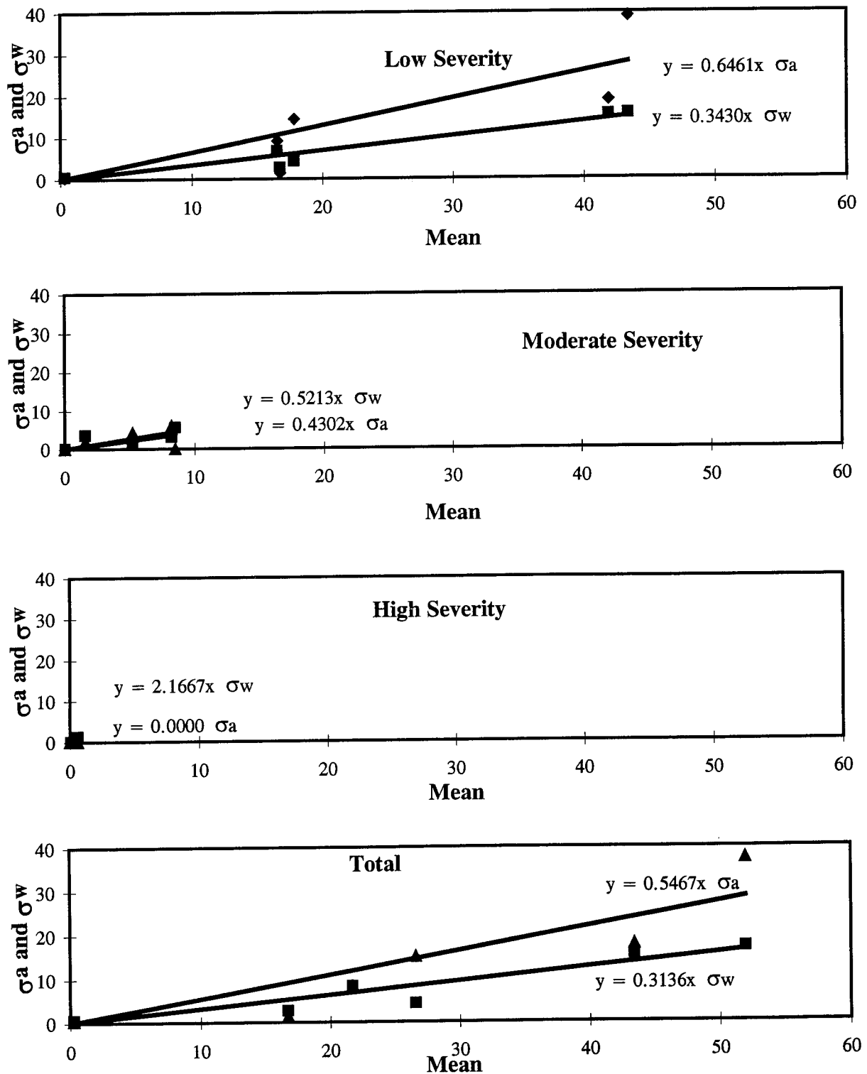
Figure 23. Longitudinal Cracking WP (Meters) - AC Pavements, Experts, PASCO Method: \sigma_a and \sigma_w Vs. Mean.
