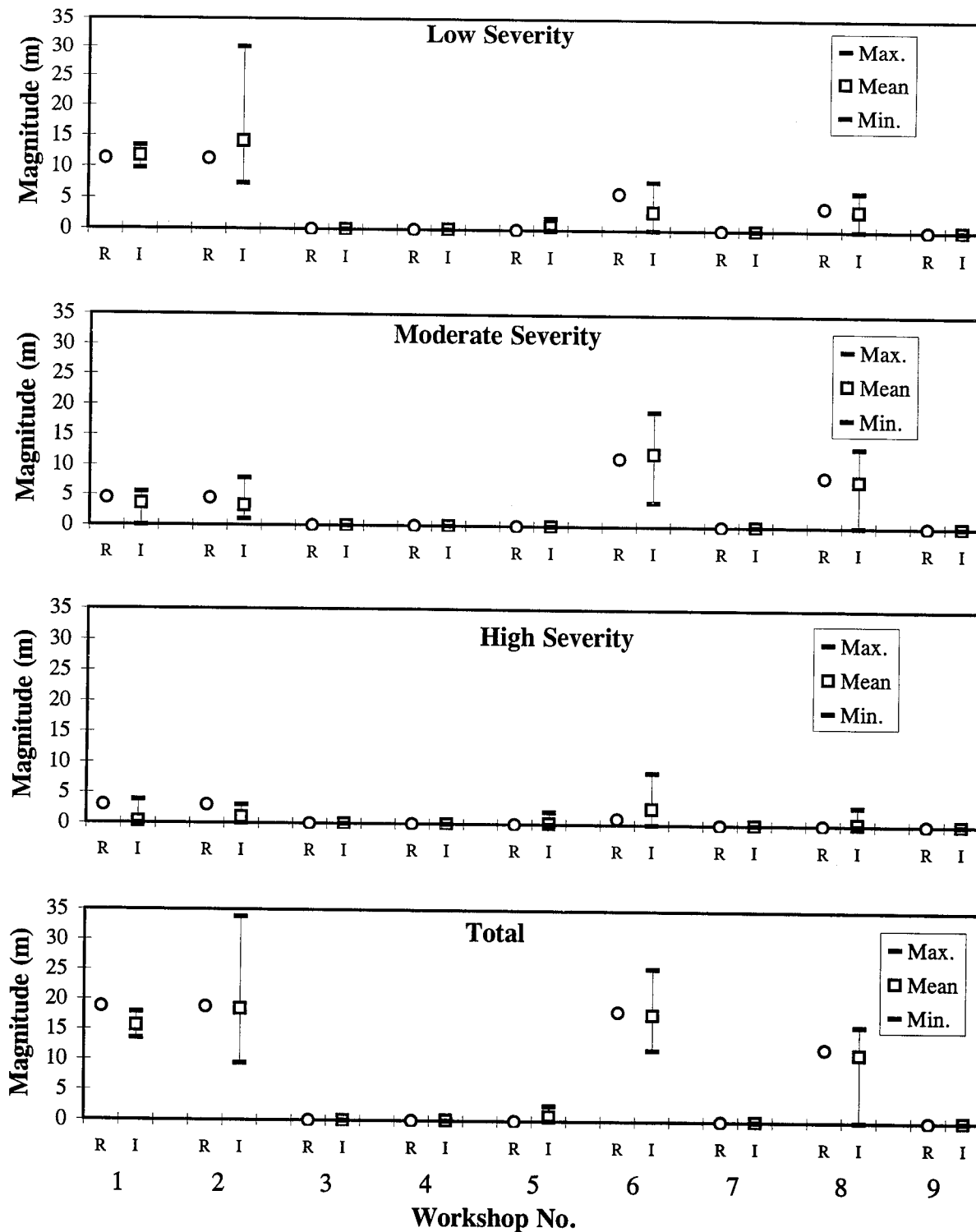
Figure 4. Longitudinal Cracking (Meters) - PCC Pavements, Manual Surveys: Reference and Individual Minimum, Mean, and Maximum Values.
