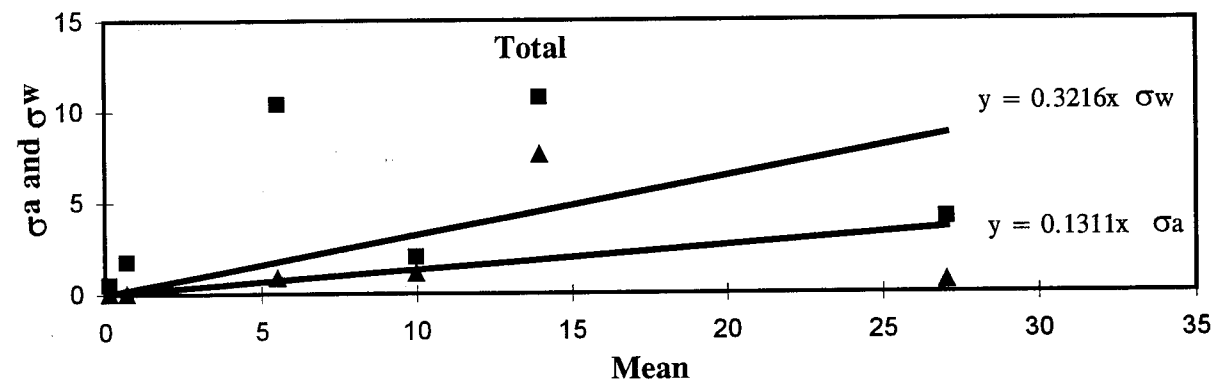
Figure 25. Longitudinal Cracking (Meters) - PCC Pavements, Experts PASCO Method: \sigma_a and \sigma_w Vs. Mean.
