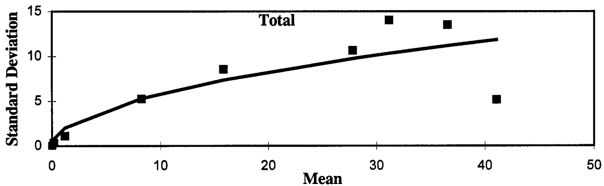
Figure 11. Longitudinal Cracking WP (Meters) - AC Pavements, Manual Surveys: Standard Deviation Vs. Mean.
