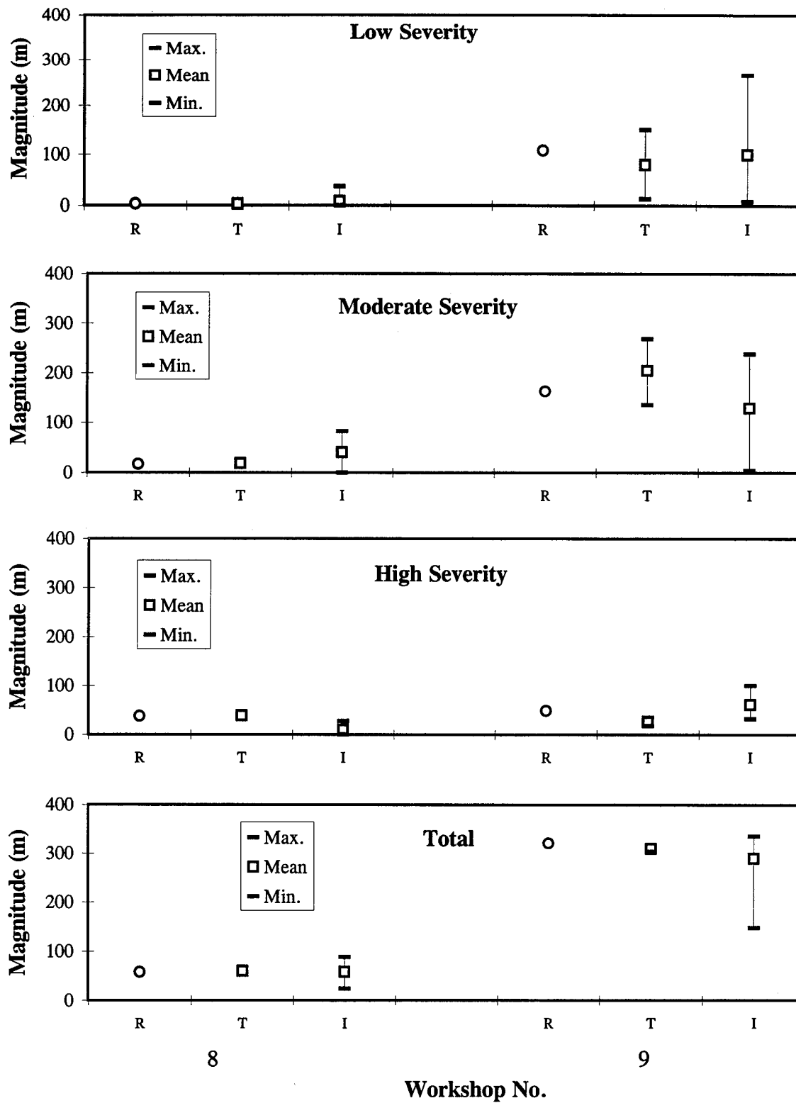
Figure 15. Longitudinal Cracking NWP (Meters) - AC Pavements, Manual Surveys: Reference, Team, and Individual Values.
