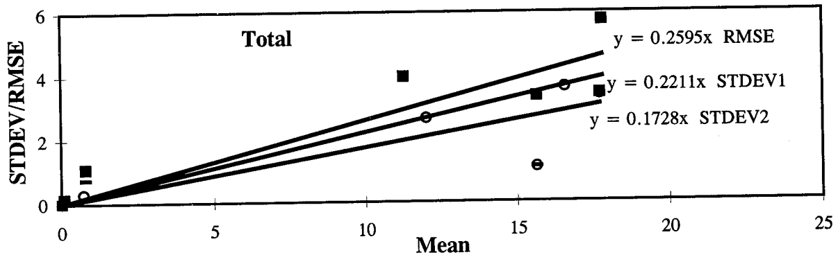
Figure 9. Longitudinal Cracking (Meters) - PCC Pavements, Manual Surveys: Standard Deviation/RMSE Vs. Mean.
