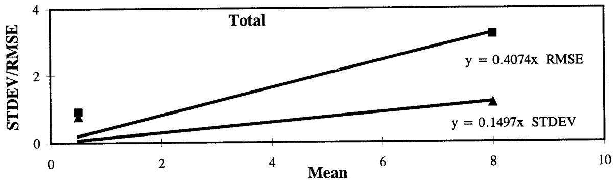
Figure 34. Corner Breaks (No.) - PCC Pavements, Individual Raters, PASCO Method: Standard Deviation/RMSE Vs. Mean.
