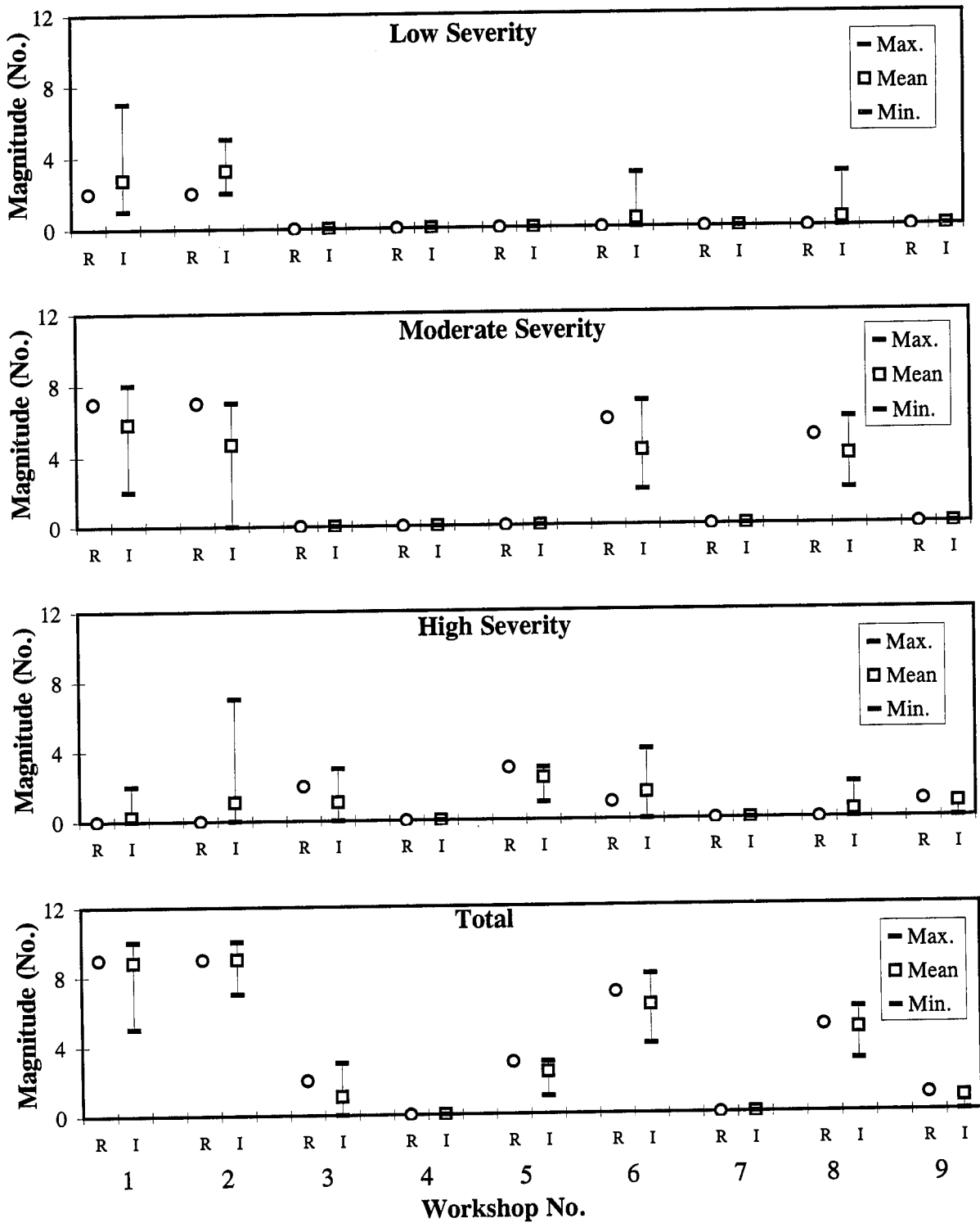
Figure 3. Corner Breaks (No.) - PCC Pavements, Manual Surveys: Reference and Individual Minimum, Mean, and Maximum Values.
