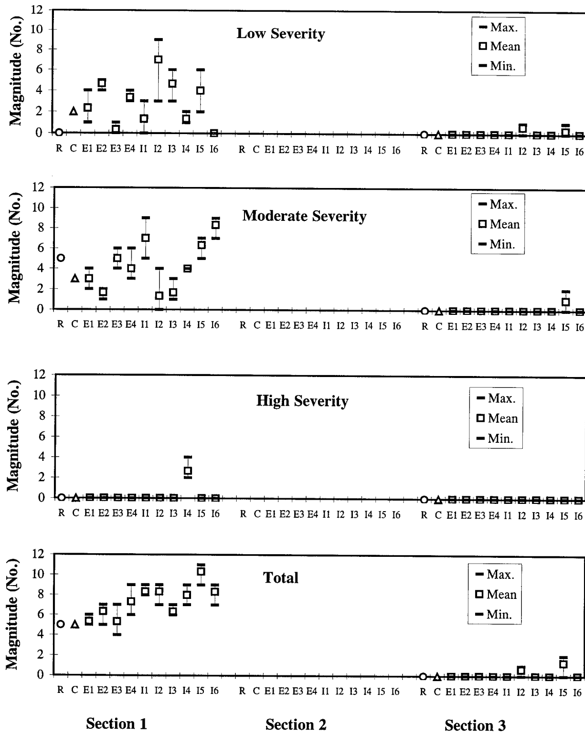
Figure 20. Corner Breaks (No.) - PCC Pavements, PASCO/PADIAS: Reference, Consensus, and Minimum, Mean, and Maximum Values for Experts and Individual Raters for Three Repetitions.
