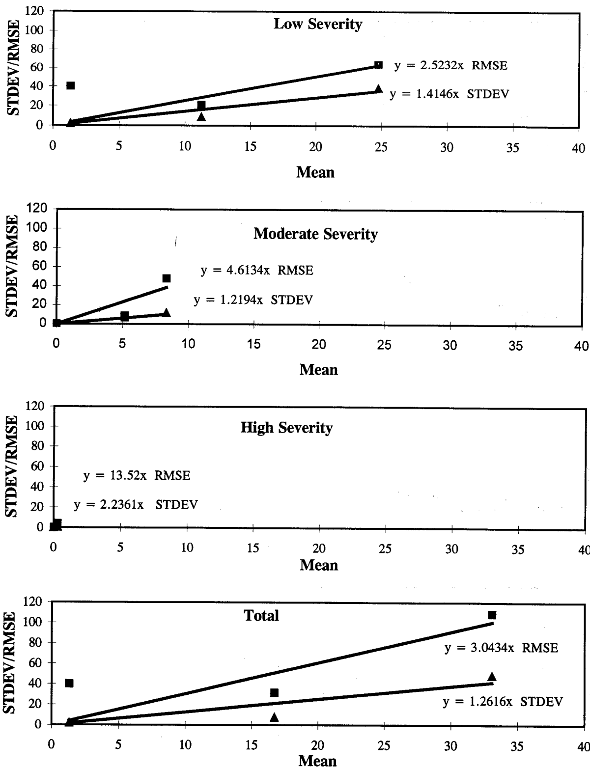
Figure 31. Fatigue Cracking (Sq. Meters) - AC Pavements, Individual Raters, PASCO Method: Standard Deviation/RMSE Vs. Mean.
