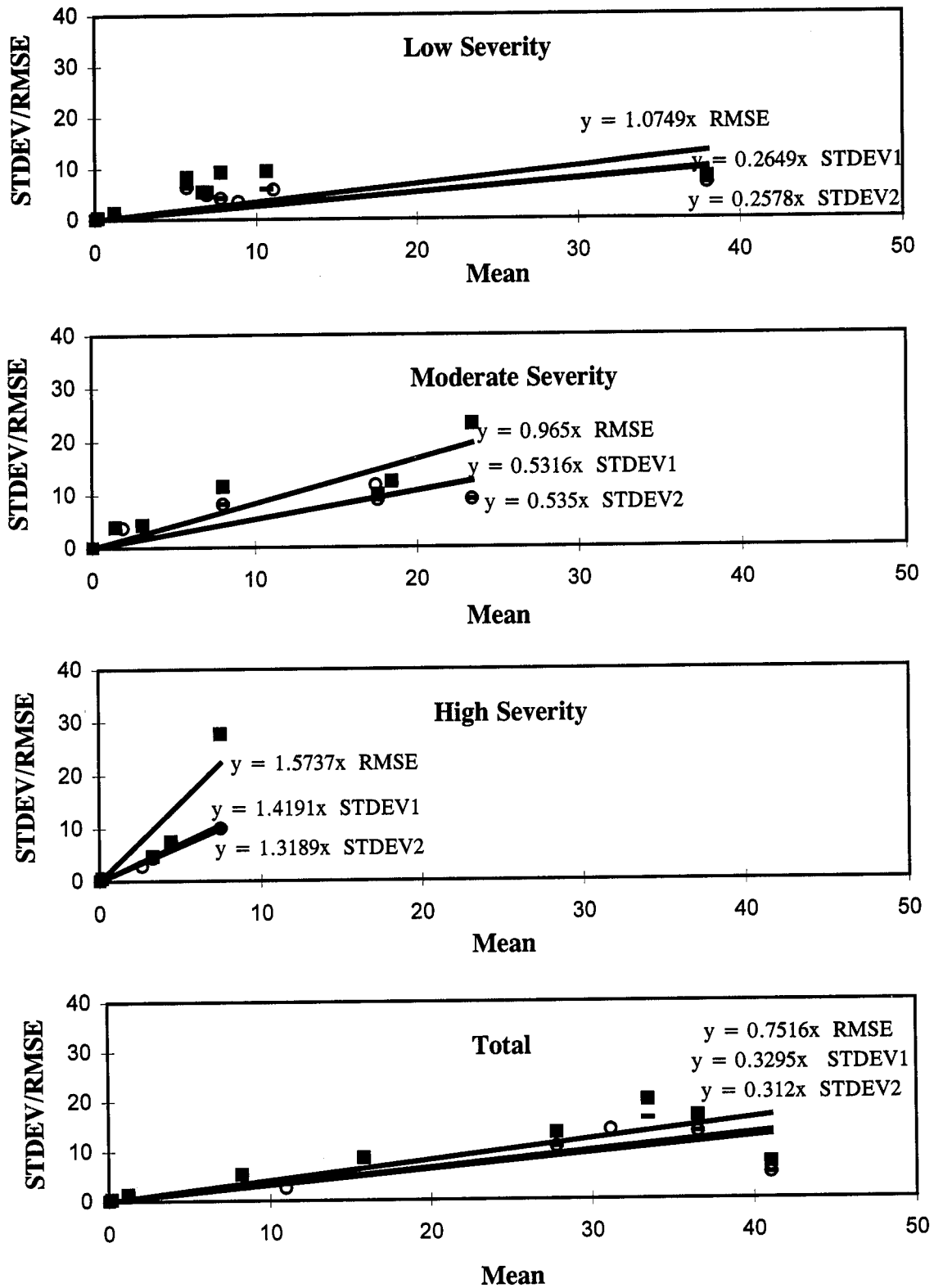
Figure 7. Longitudinal Cracking WP (Meters) - AC Pavements, Manual Surveys: Standard Deviation/RMSE Vs. Mean.
