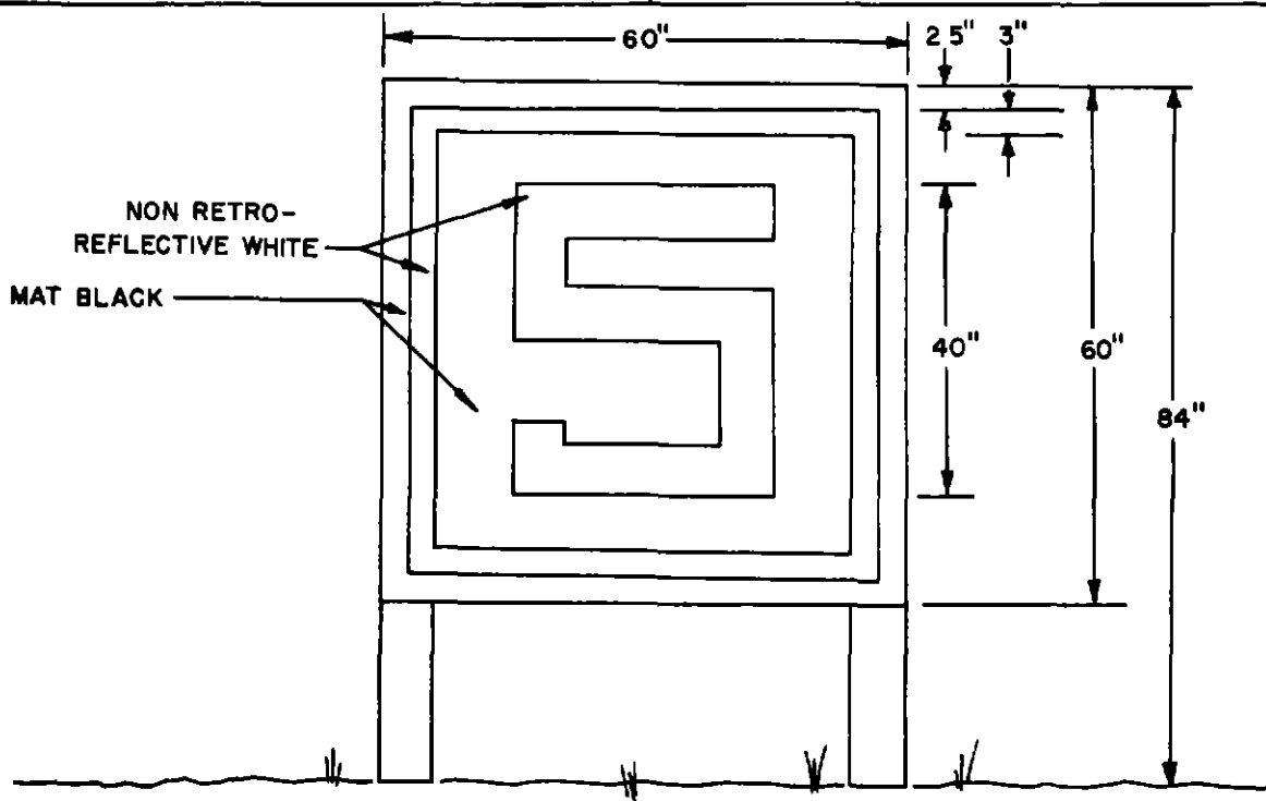
RUNWAY DISTANCE REMAINING SIGN
