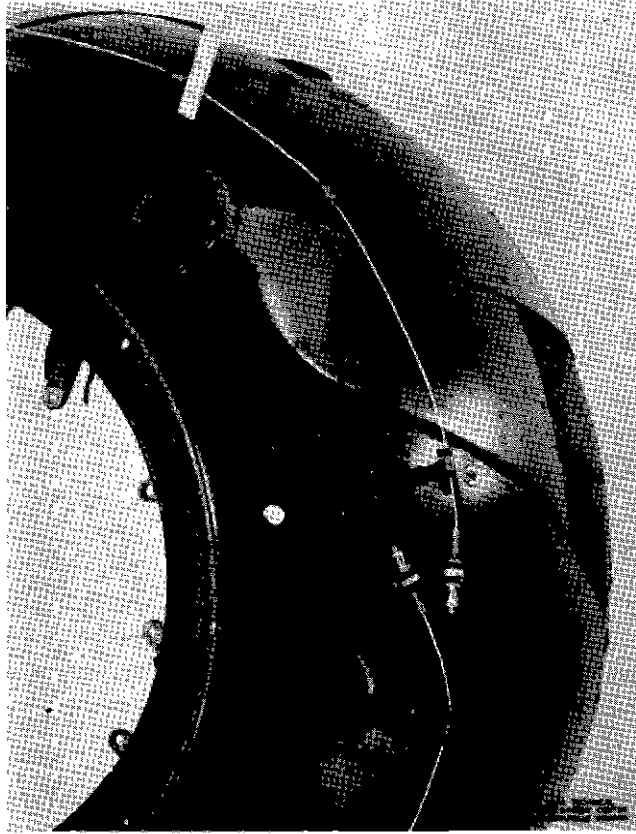
Fig. 8 Mounting Details for Afterbody Loop
