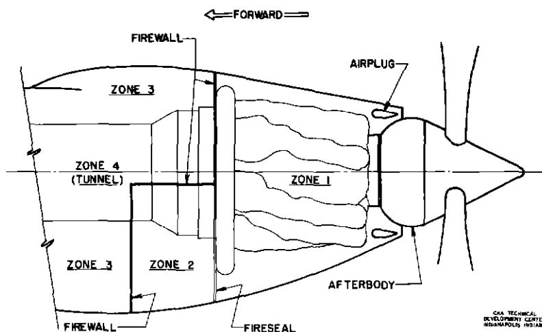
Fig. 3 Major Zones in the B-36 Nacelle
