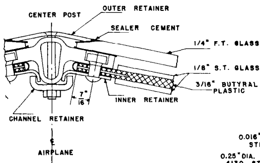
VERTICAL SECTION
