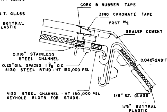
HORIZONTAL SECTION
