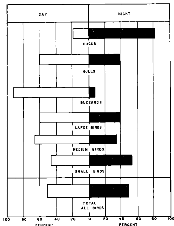
Fig 11 Distribution of Strikes Involving Identified Bird Types According to Occurrence During Daylight or Darkness
