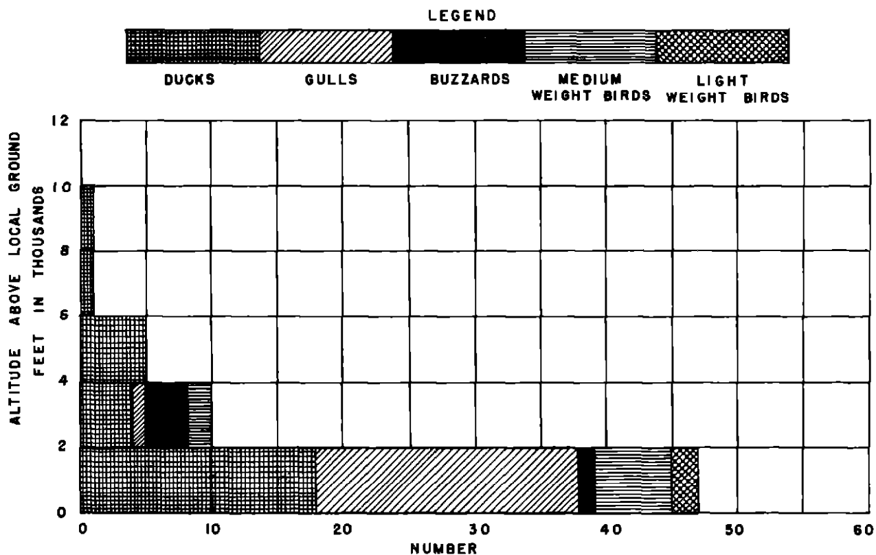
Fig 6 Identified Bird Types Struck at Various Altitudes Above Local Ground Level
