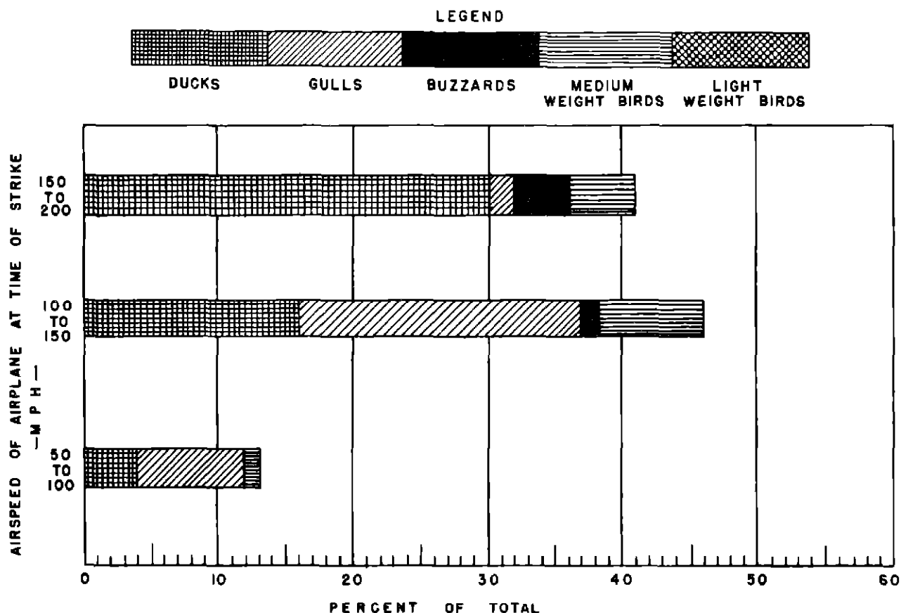
Fig 5 Identified Bird Types Struck at Various Aircraft Velocities
