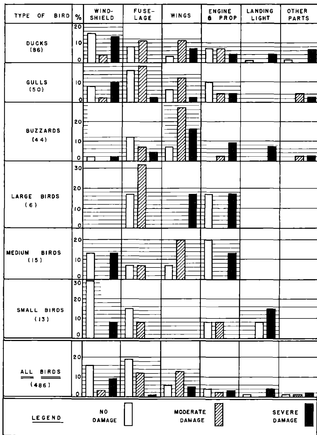
Fig. 8 Severity of Damage to Different Portions of the Aircraft Structure Caused by Various Types of Birds
