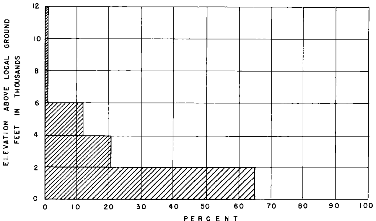
Fig. 2 Frequency of Bird Strikes as Effected by Elevation Above Local Ground
