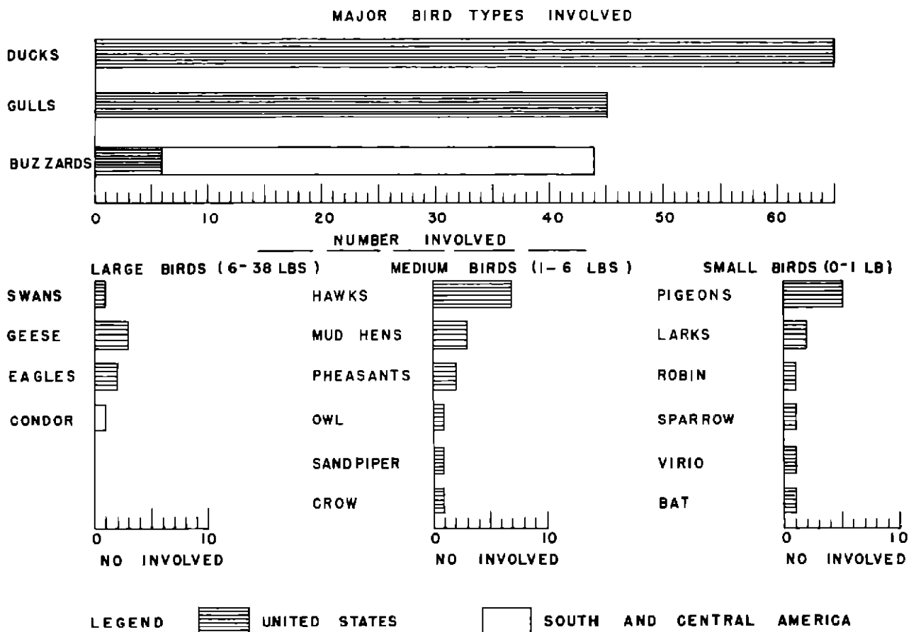
Fig 3 Relative Frequencies of Bird Strikes Involving Various Types of Identified Birds
