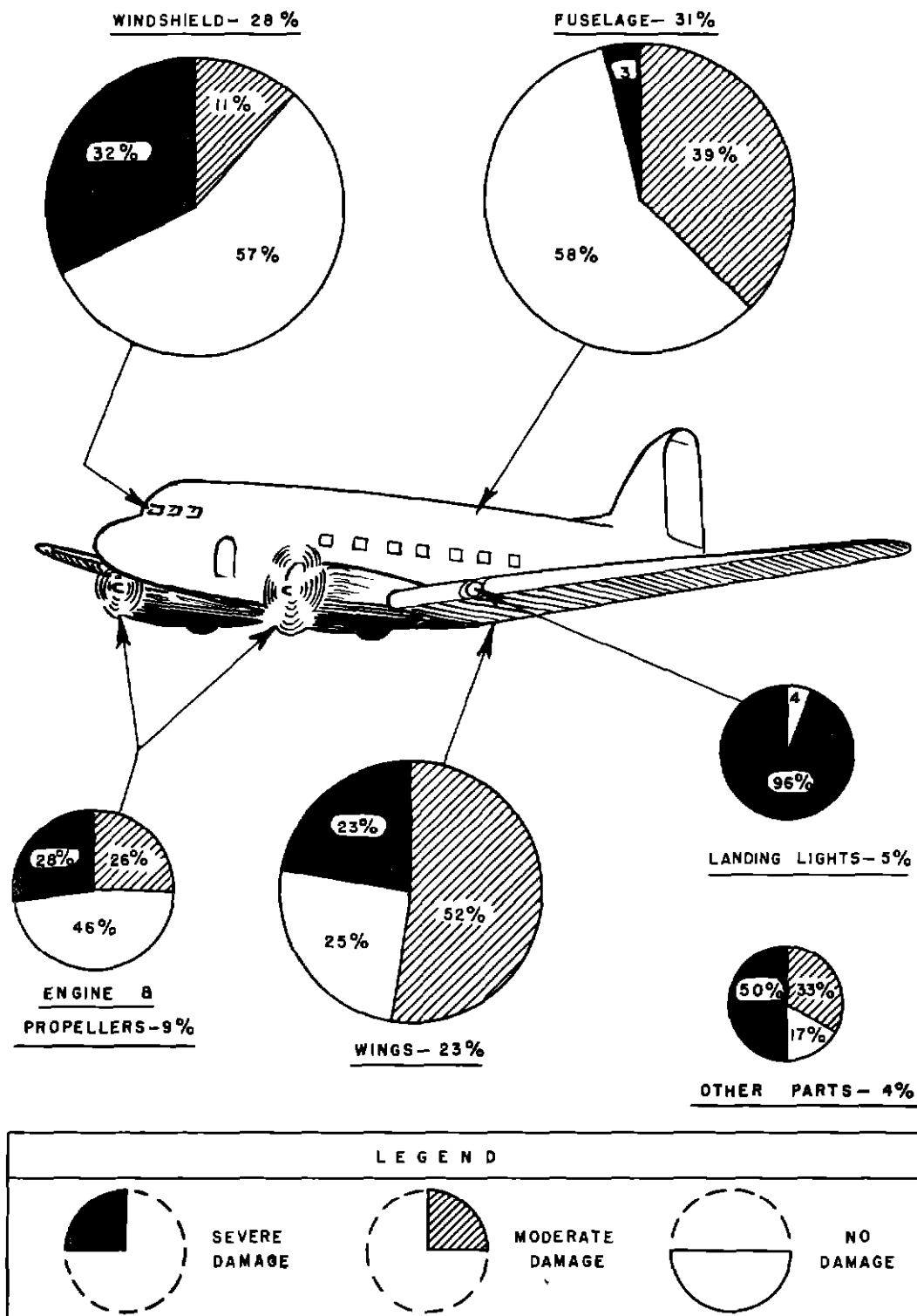
Fig 7 Location, Severity, and Relative Frequency of Bird Strikes on Airplanes
