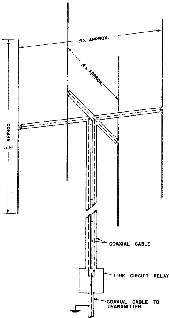
Figure 1.—Schematic diagram of the UHF radio range antenna system.
