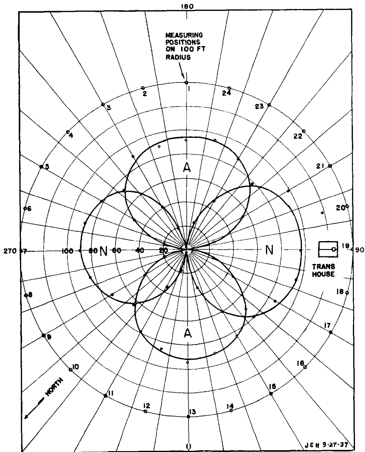
Figure 5 — Field pattern taken on the ground at 100-foot radius
