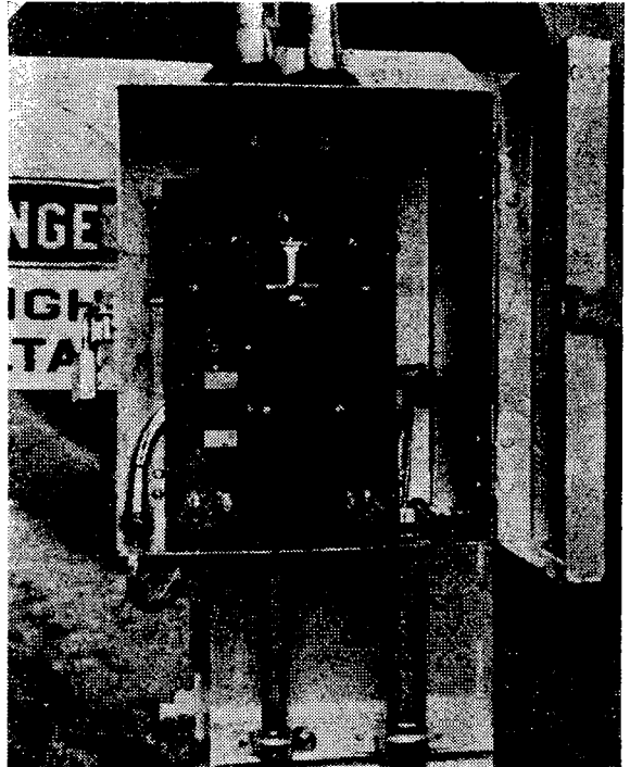
Figure 4.—The modified link circuit relay mounted on pole.
