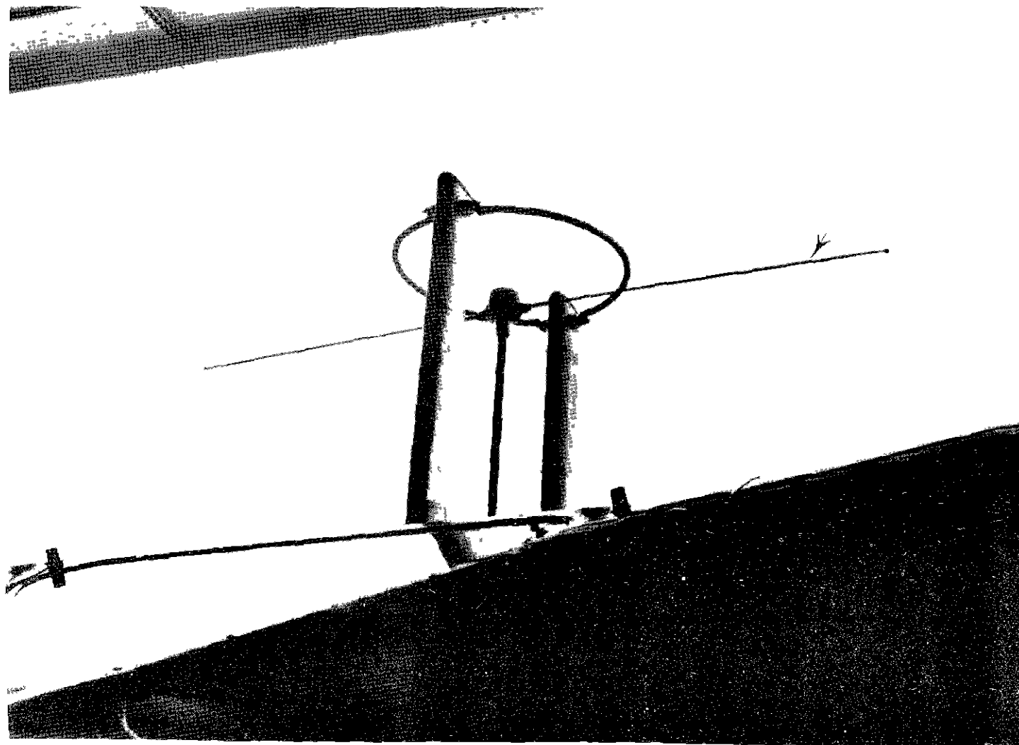
FIG.15 SPECIAL HORIZONTAL DOUBLET RECEIVING ANTENNA FOR 125 MEGACYCLES
