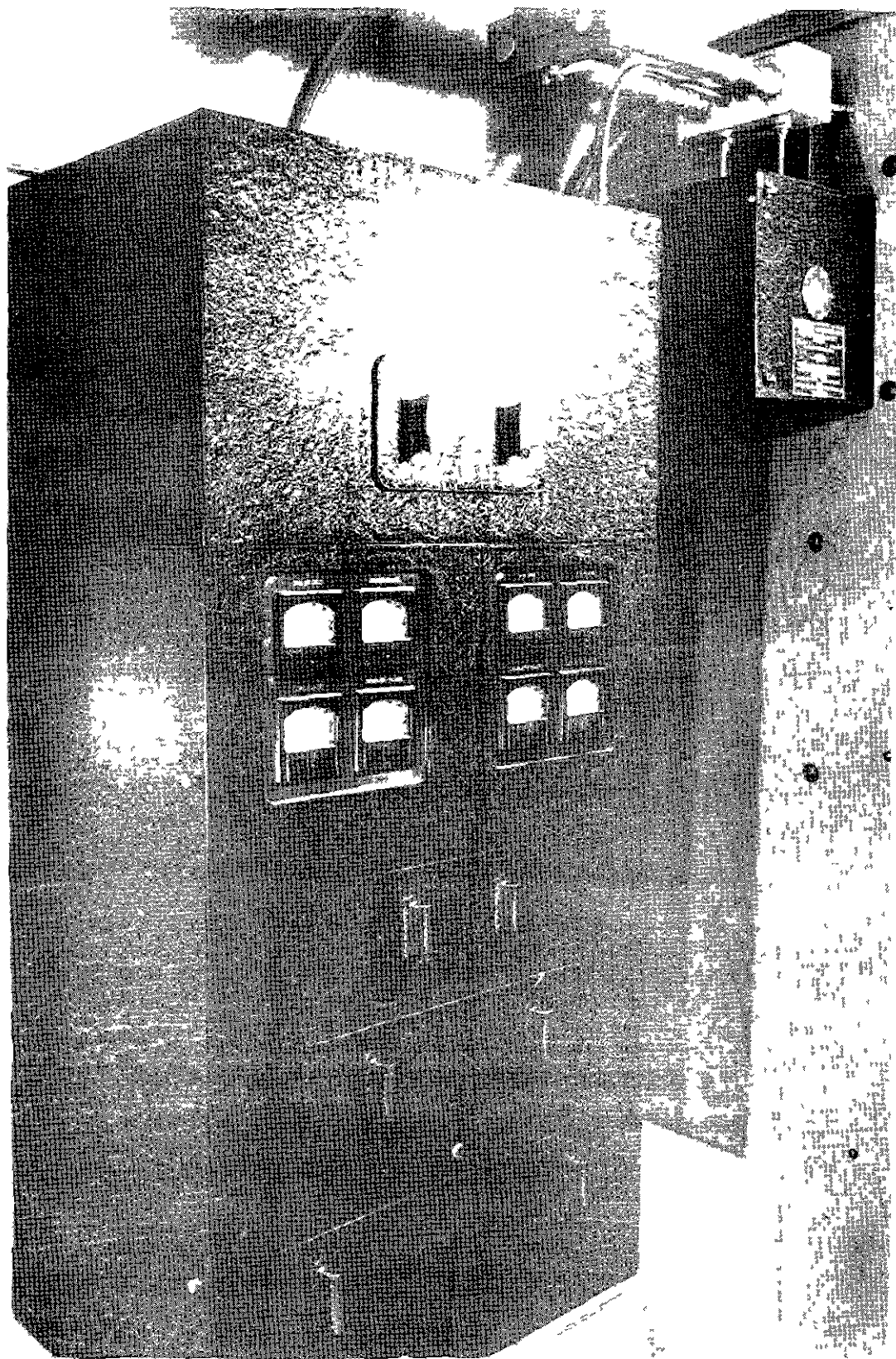
FIG 3 TRANSMITTER AND BEACON CONVERTER
