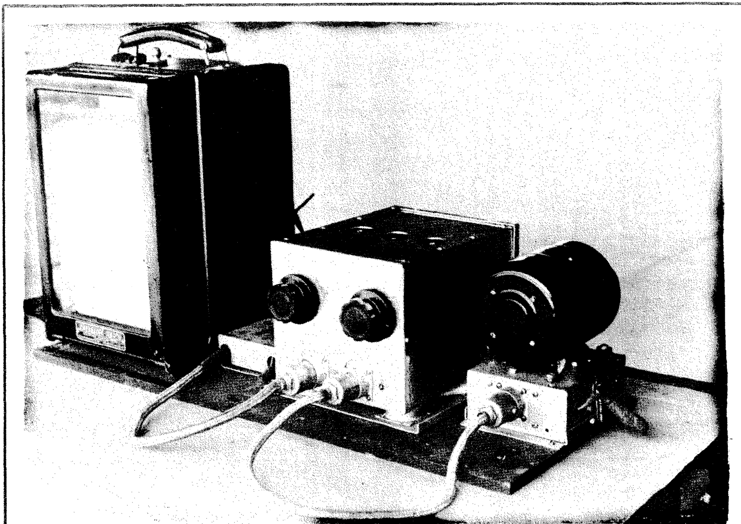
FIG. 12 RECORDER, AMPLIFIER-RECTIFIER AND DYNAMOTOR
