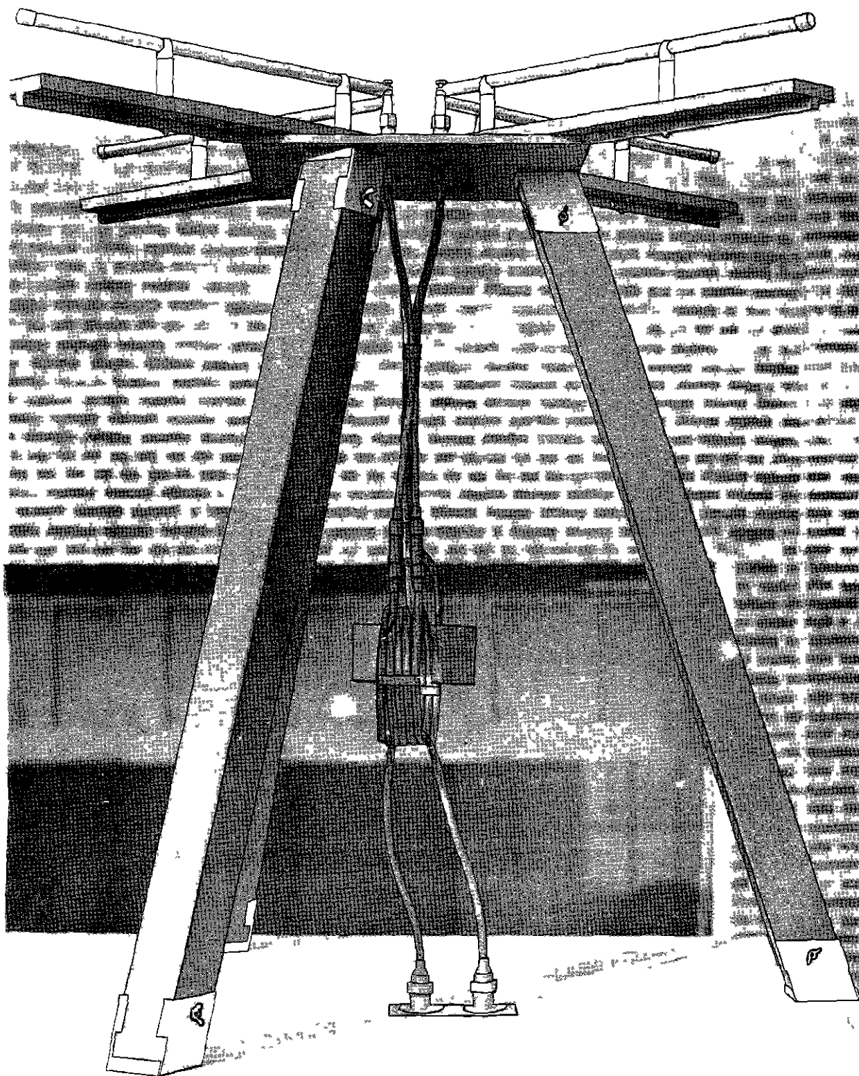
FIG 9 HORIZONTAL FOUR-COURSE ANTENNA
