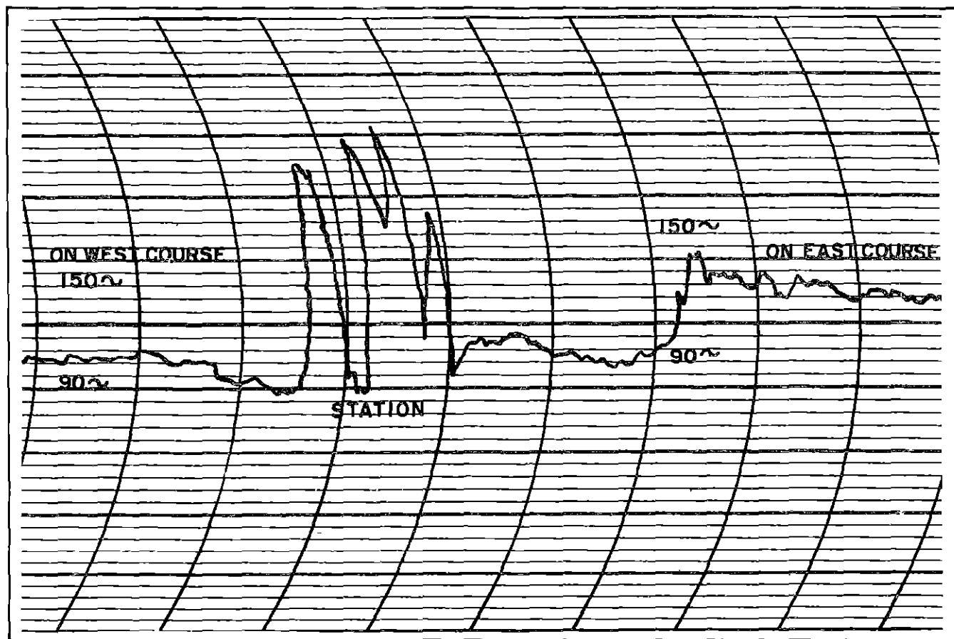
FIG. 27 125 MC FOUR COURSE RADIO RANGE ON-COURSE FLIGHT OVER STATION, HORIZONTAL POLARIZATION
