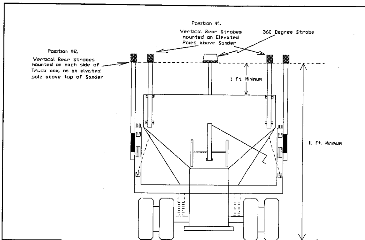
Figure 16 Two possible rear vertical strobe mounting locations
