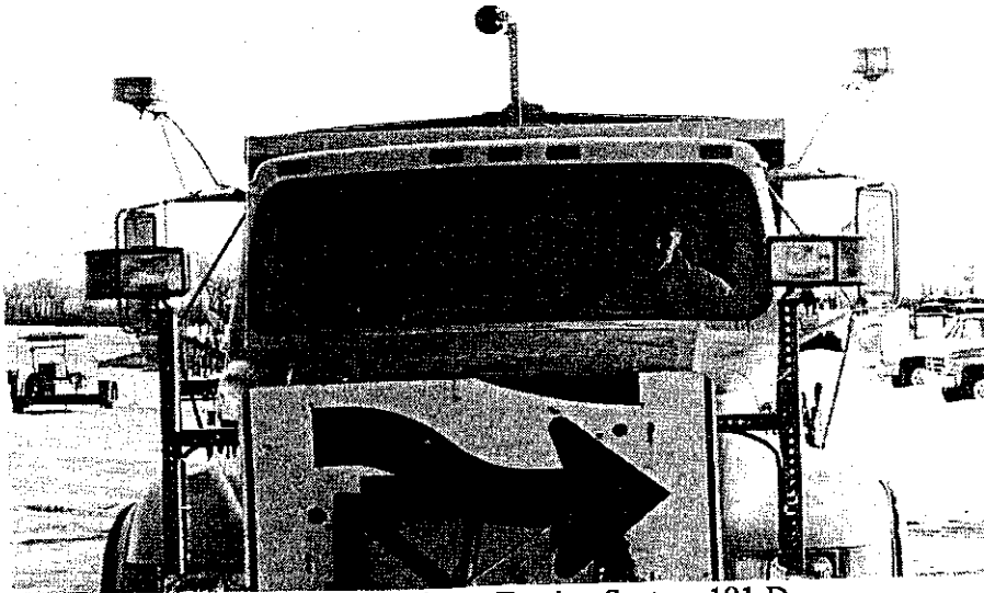
Figure 8 Aberdeen Truck - System 101-D
