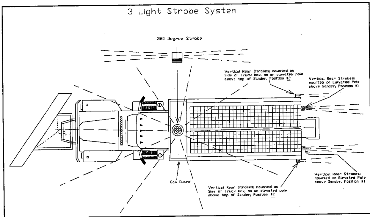
Figure 15 Minimum Lighting System
