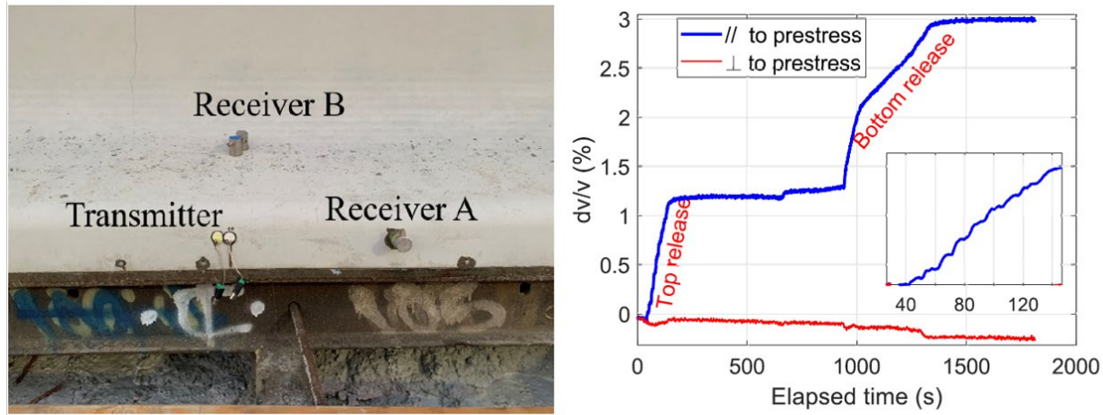
Figure 69. Ultrasound transmitter and receiver layout and coda-wave interferometry results for full-scale prestressed AASHTO girder at stress transfer (Zhang et al. 55 )
