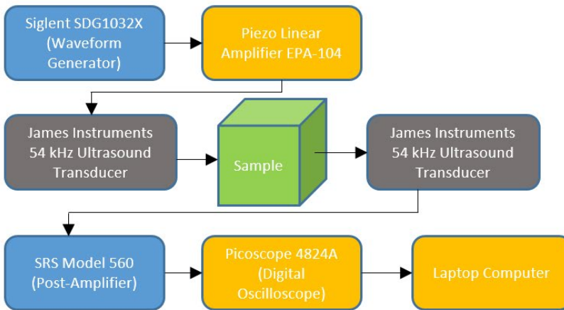
Figure 133. Instrumentation for ultrasound generation and data acquisition
