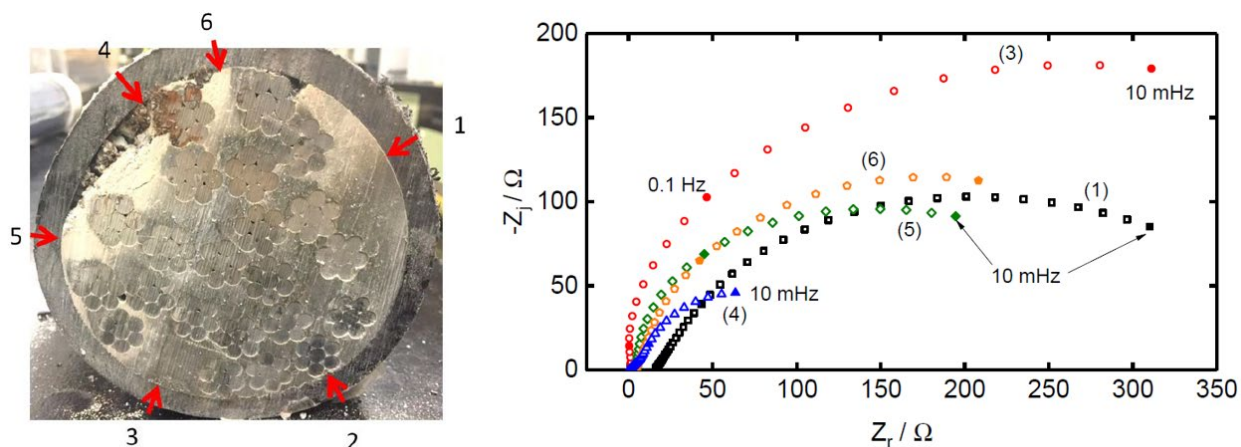
Figure 26. Electrochemical impedance spectroscopy results from corroded tendon. 26 Numbers in parentheses on chart correspond to circumferential locations on the tendon.
