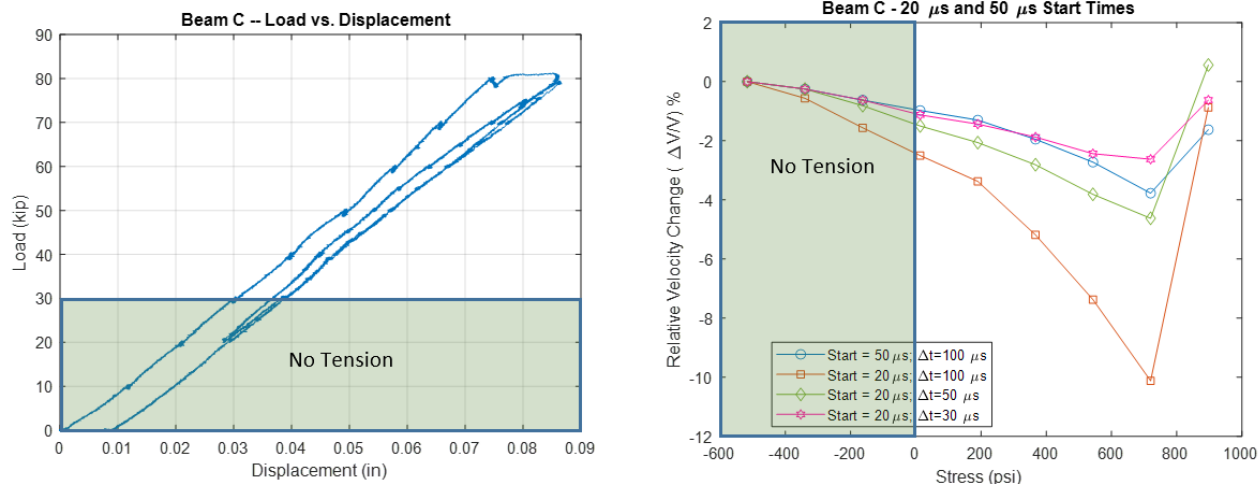
Figure 158. Load vs. deflection and CWI results for Beam C (Step 1: 0 to barely-visible cracking load)
