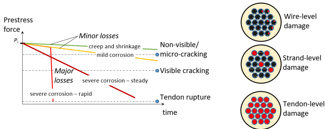
Figure 10. Prestress losses over the service-life of a tendon
