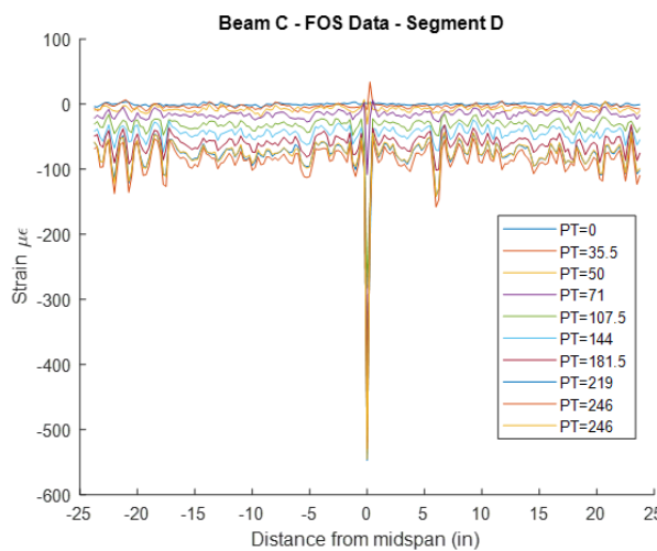
Figure 145. Beam C: FOS data for Segment D
