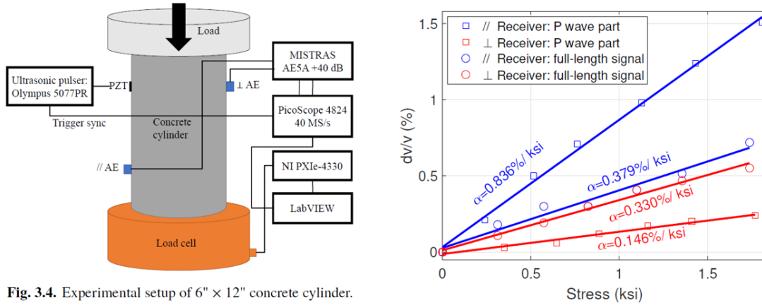
Figure 67. Experimental setup and results for coda-wave interferometry applied to compression test for concrete cylinder (Zhang et al. 55 )
