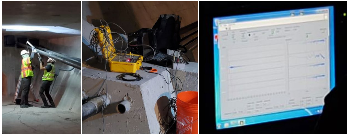
Figure 5. Ultrasonic pulse velocity testing on external tendon. Broadway Bridge, Daytona Beach
