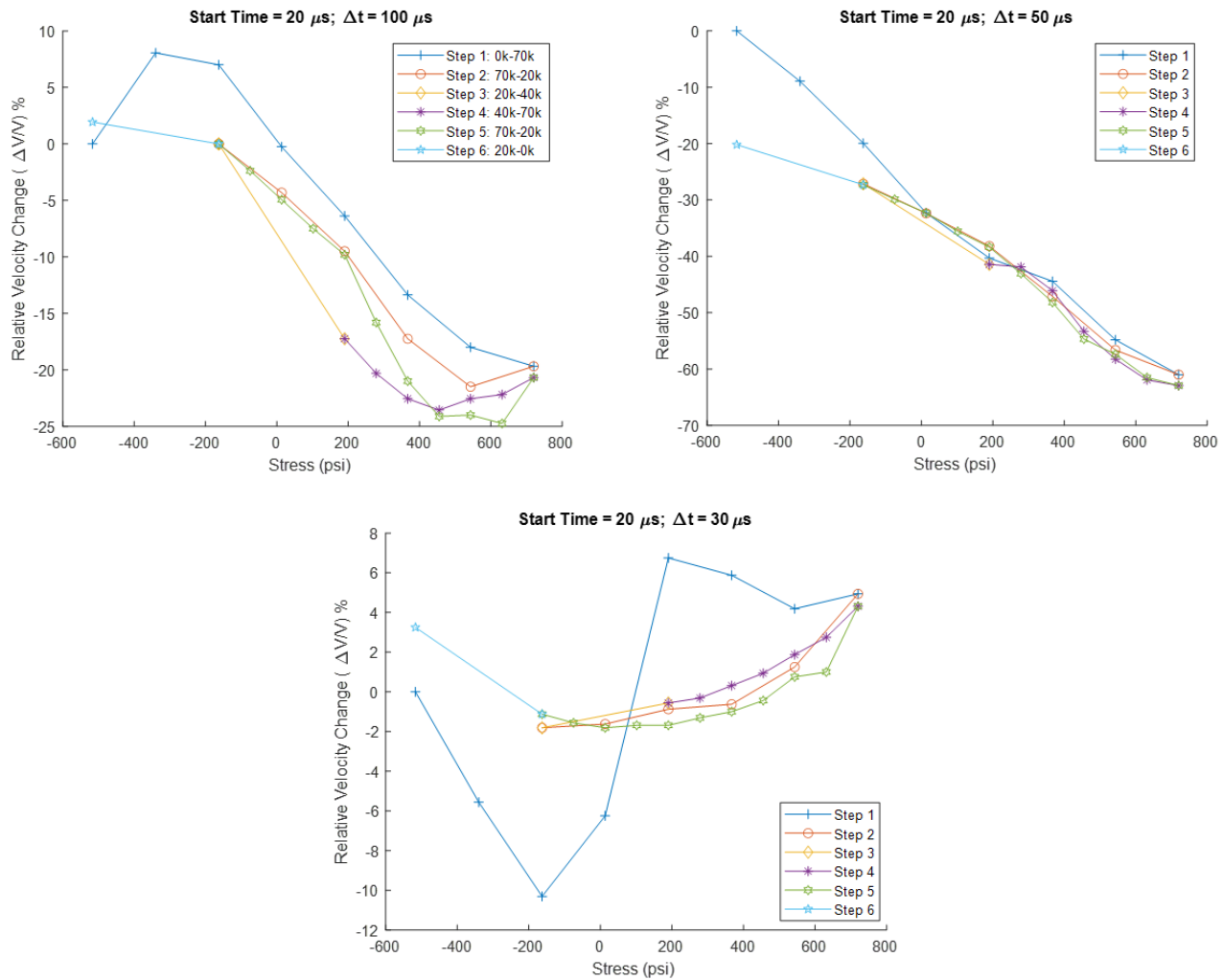
Figure 157. Coda-wave interferometry results for Beam B (all six load steps – t_o=20 , \Delta t = 30, 50, 100 )
