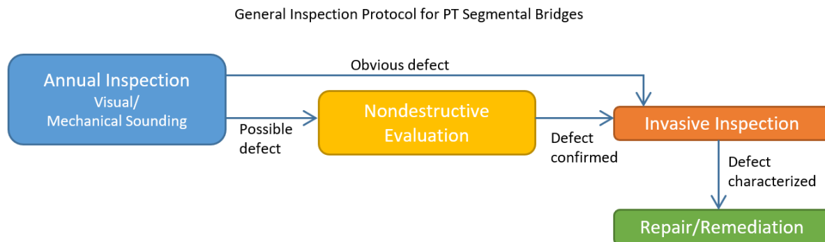
Figure 9. General inspection protocol for PT segmental bridges
