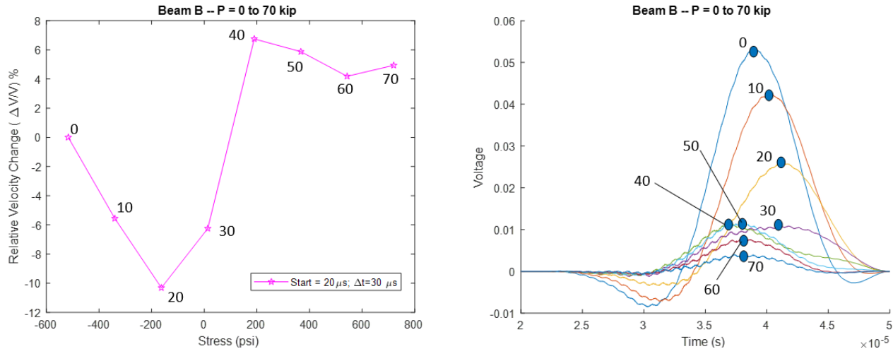
Figure 156. Interferometry results and ultrasound waveforms for Beam B ( P=0\text{ kip} to P=70\text{ kip} ; t_o = 20 and \Delta t = 30 )
