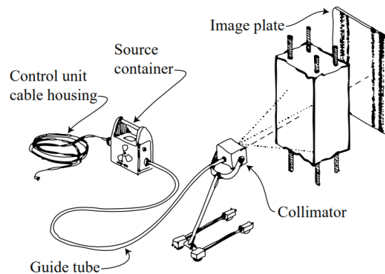
Figure 51. Schematic representation of a conventional ^{192}\text{Ir} source assembly (Mariscotti et al. 40 )
