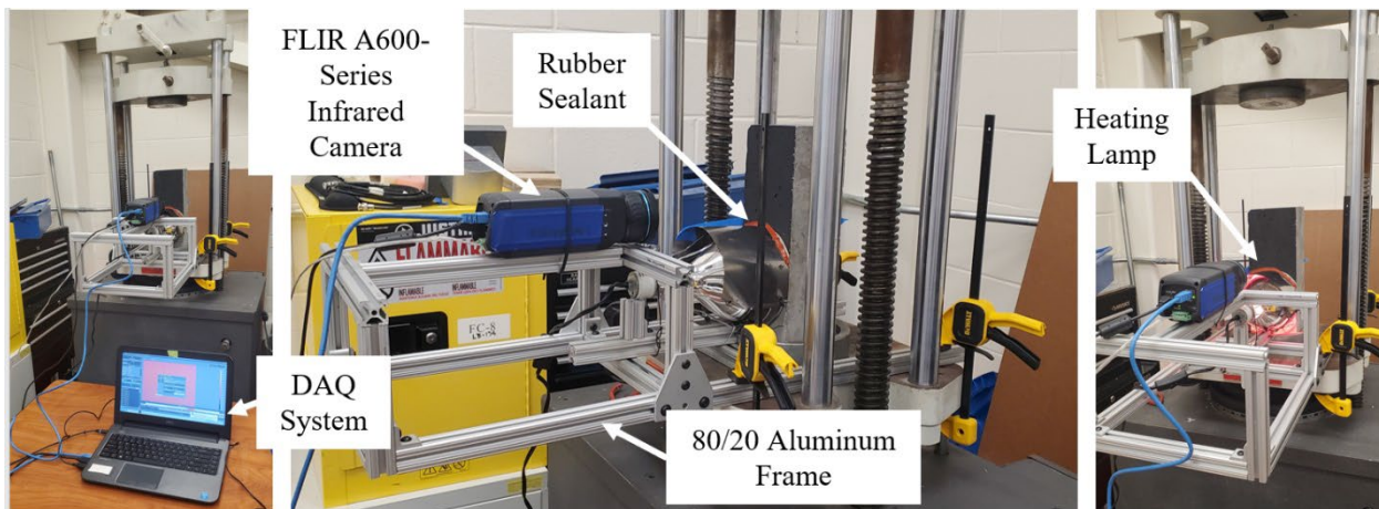
Figure 102. Testing setup
