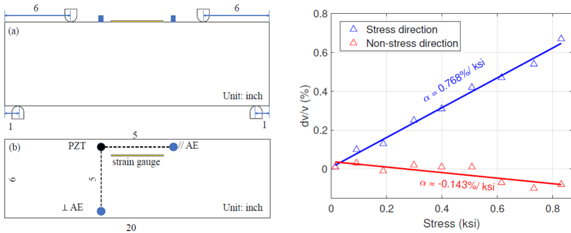
Figure 68. Experimental setup and results for coda-wave interferometry applied to flexural test for concrete beam (Zhang et al. 55 )
