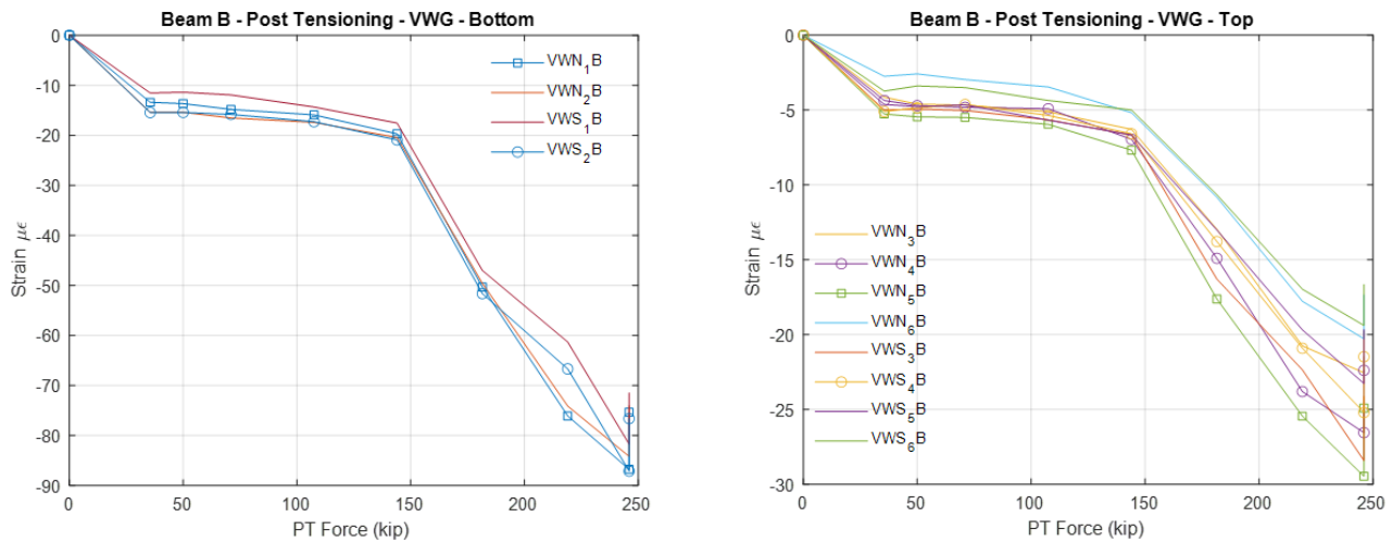
Figure 143. Beam B: VWG Results
