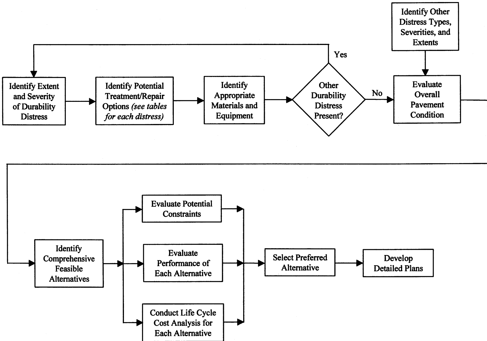
Figure III-1. Flowchart for selecting preferred treatment and rehabilitation options.
