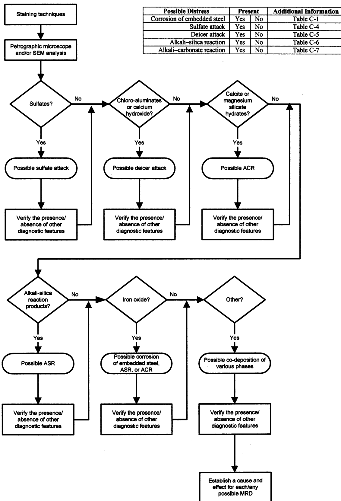
Figure C-3. Flowchart for identifying infilling materials in cracks and voids.
