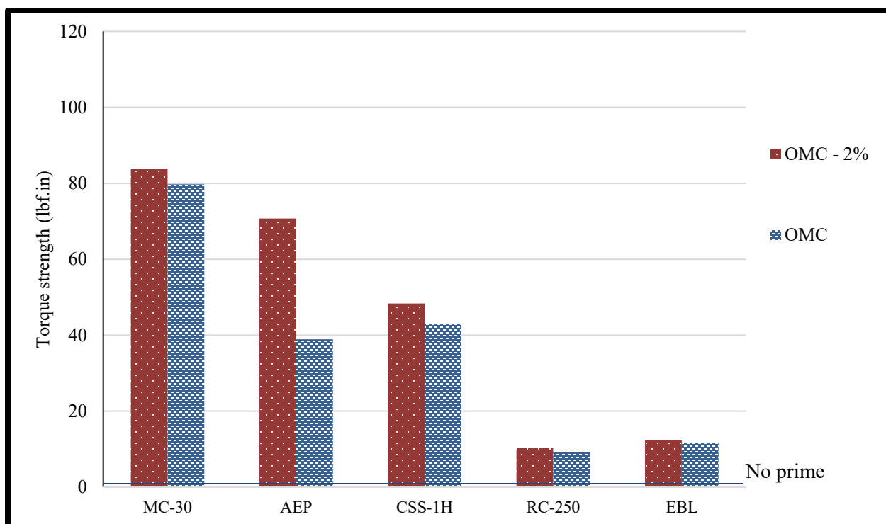
Figure 23. Torque Strength at Different Moisture Contents for Flexible Base.
