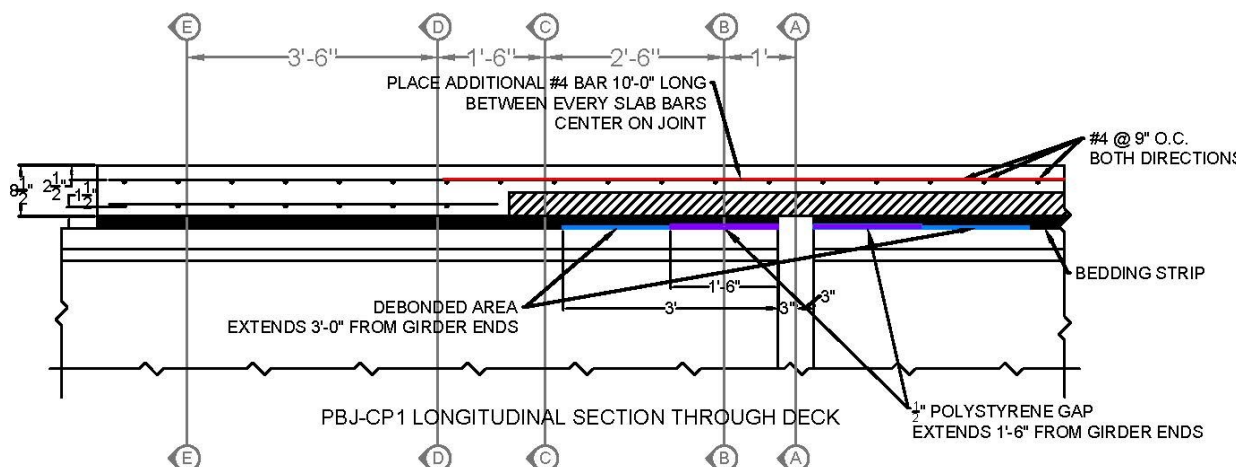
Figure 9.13. PBJ-CP1 details—elevation view.
