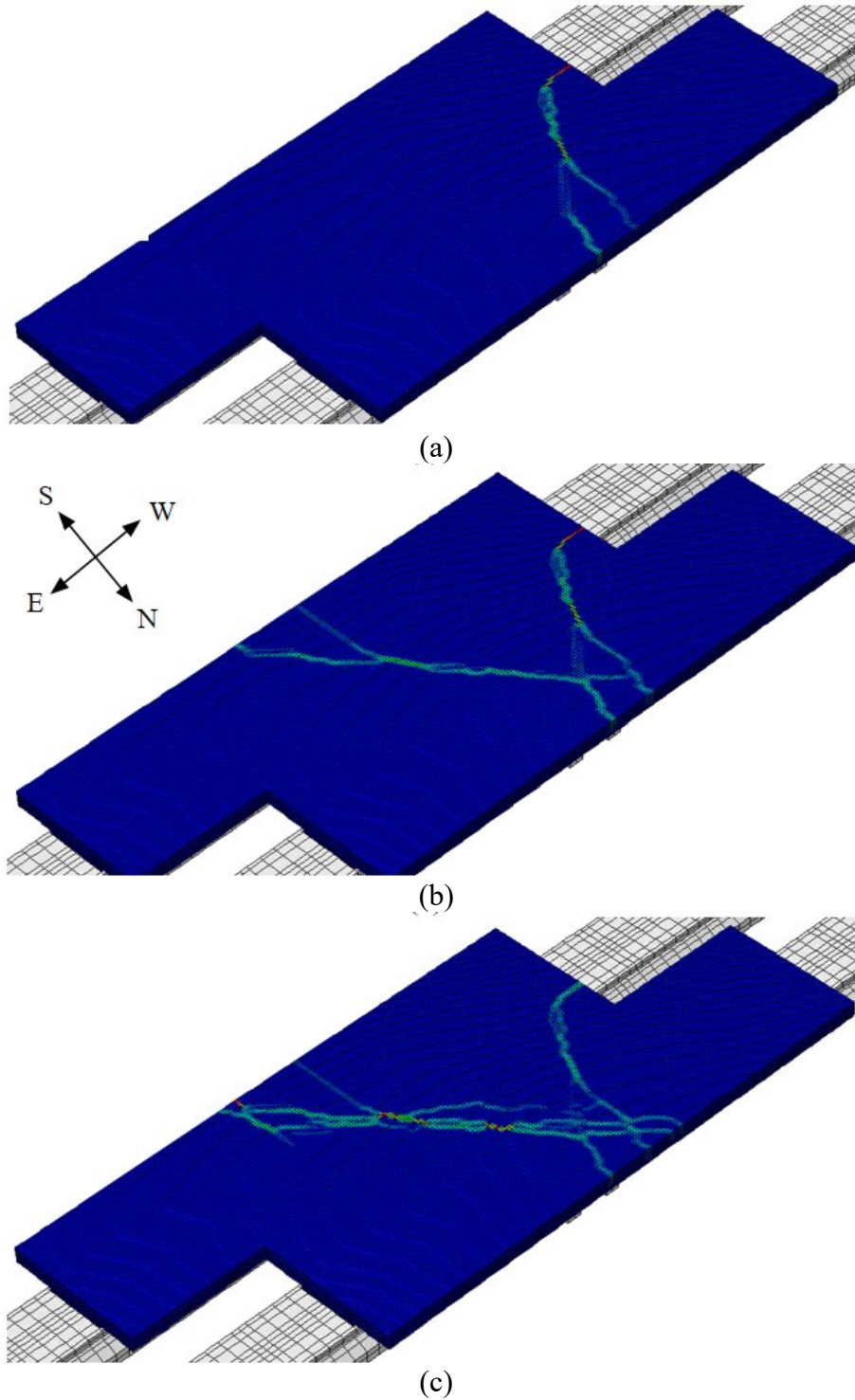
Figure 8.81. Crack propagation in the debonded dual-girder skewed model with offset panels for loading progressing from the (a) northwest girder, (b) southwest girder, and (c) southeast and northeast girders.
