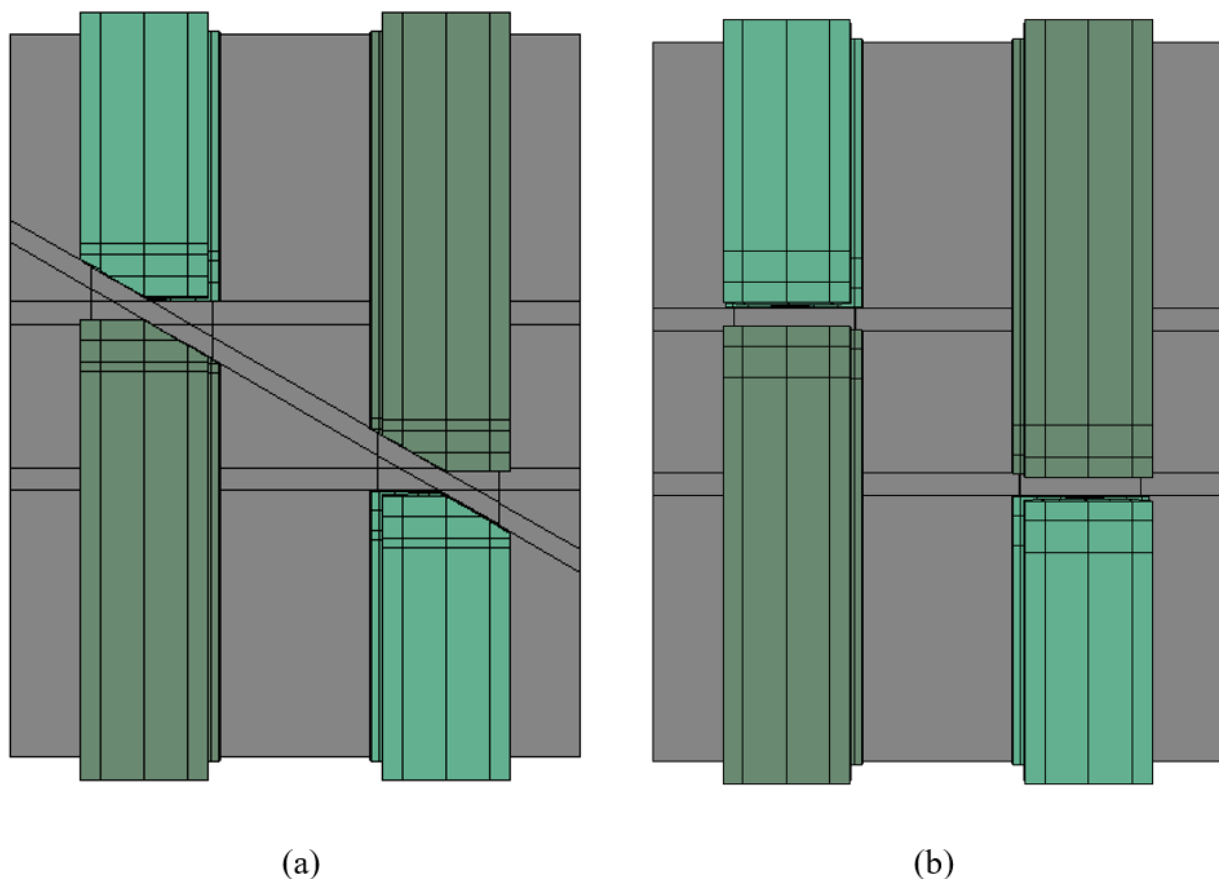
Figure 8.67. Underside of skewed stub models, showing (a) a skewed girder end condition and (b) a flat girder end condition.
