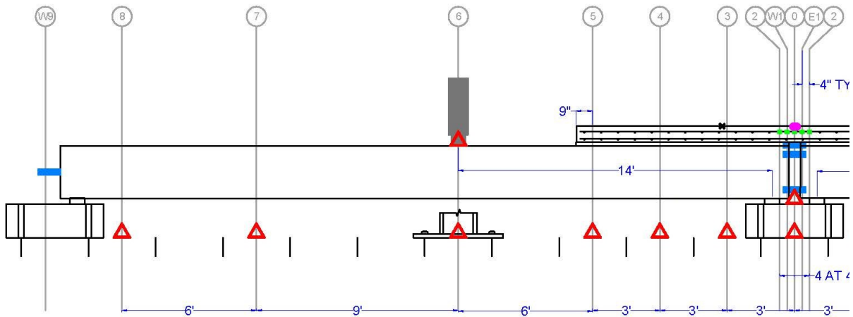
Figure 9.36. Generic elevation for string pots and LVDTs (single full span shown with portion of other span; blue rectangles represent LVDTs, and red triangles represent string pots).
