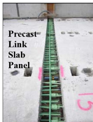
(a) Reinforced continuity provided by mechanical couplers
