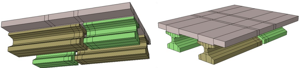
Figure 8.3. Dual-girder model for skewed girder configuration without clipped girders.
