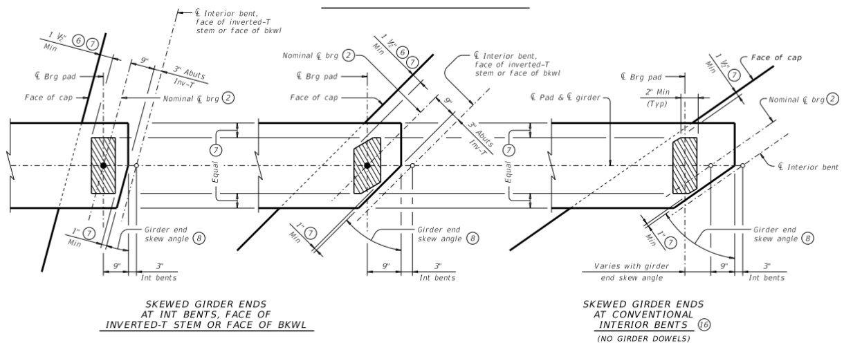
Figure 6.8. Current standard details for skewed ends from elastomeric bearings and girder end details sheet.
