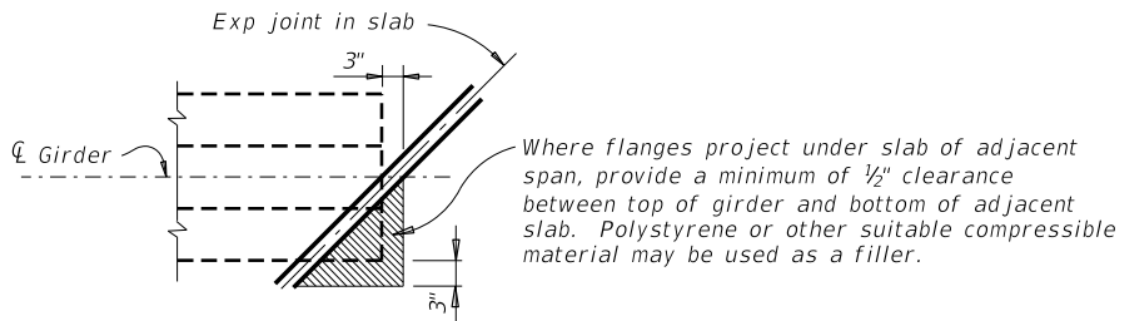
Figure 6.8. Current standard details for skewed ends from elastomeric bearings and girder end details sheet.
