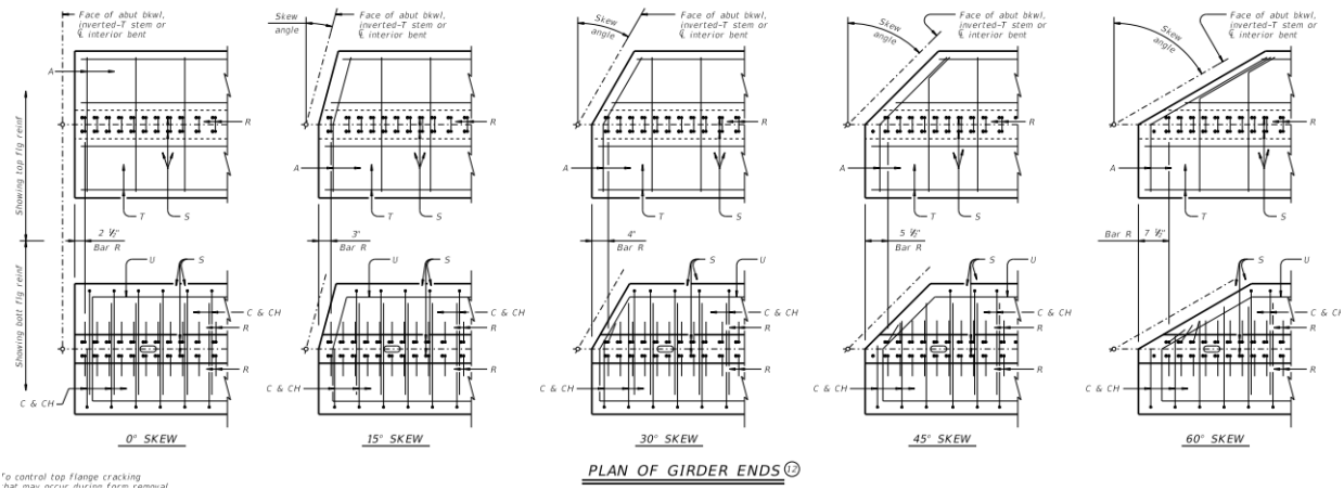
Figure 6.7. Current standard details for skewed ends from prestressed concrete I-girder details sheet.
