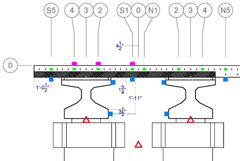
Figure 9.37. Instrumentation on general cross-section (FP1 shown; blue rectangles represent LVDTs, pink ovals represent concrete surface gages, green rectangles represent steel strain gages, and red triangles represent string pots).
