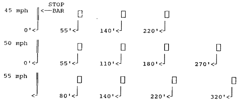
Figure 6.1 Recommended Loop Layouts
