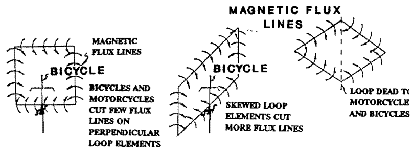
Figure 1.3 Loop Shape Effects on Small Vehicle Detection
