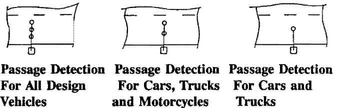
Figure 8.1 Suggested Microloop Installation Patterns
