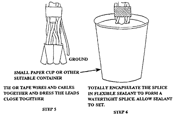
Figure 5.7 Paper Water Cup Watertight Seal Installation Procedure
