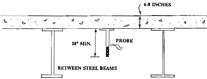
Figure 8.2 Application of the Microloop Under a Bridge Deck
