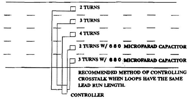
Figure 4.3 Crosstalk Control On Multilane Freeway Detectors
