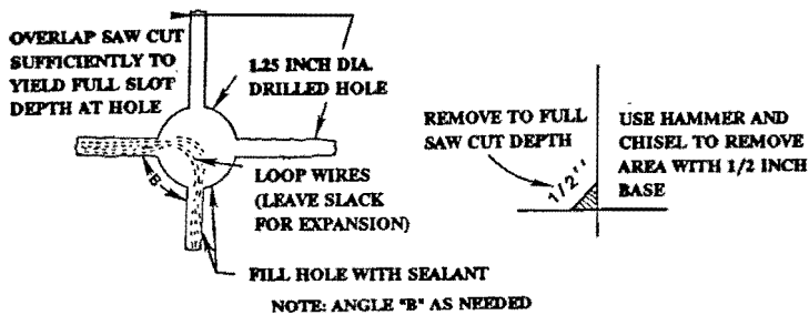
Drilled Hole Chiseled Corner Figure 5.1 Alternative Corner Treatments
