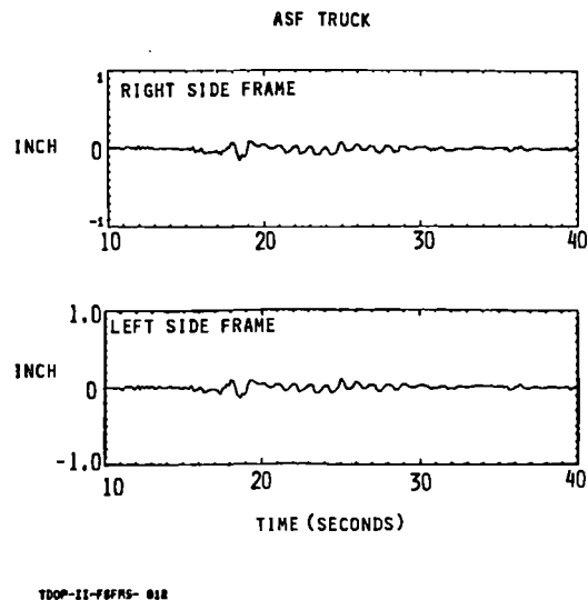
Figure 5-19. Relative Lateral Displacement (ASF Truck Side Frames)
