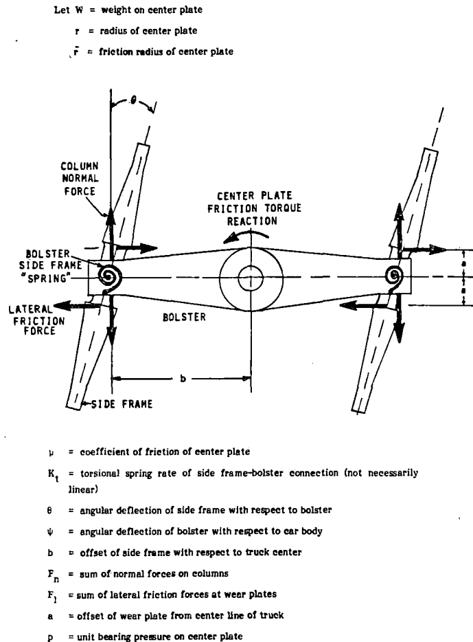
Figure 5-8. Definition Sketch of Forces Acting against Center Plate Friction Torque
