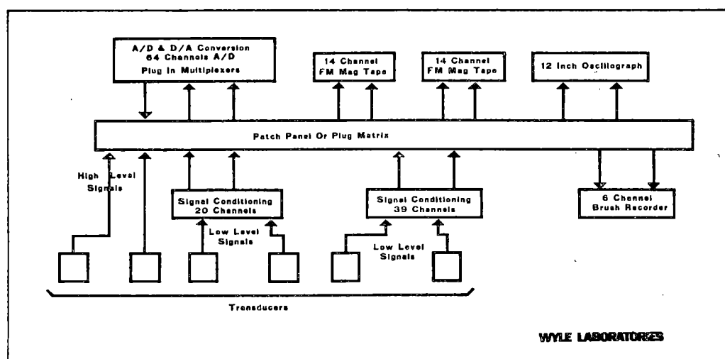
Figure 2-5. Analog Subsystem
