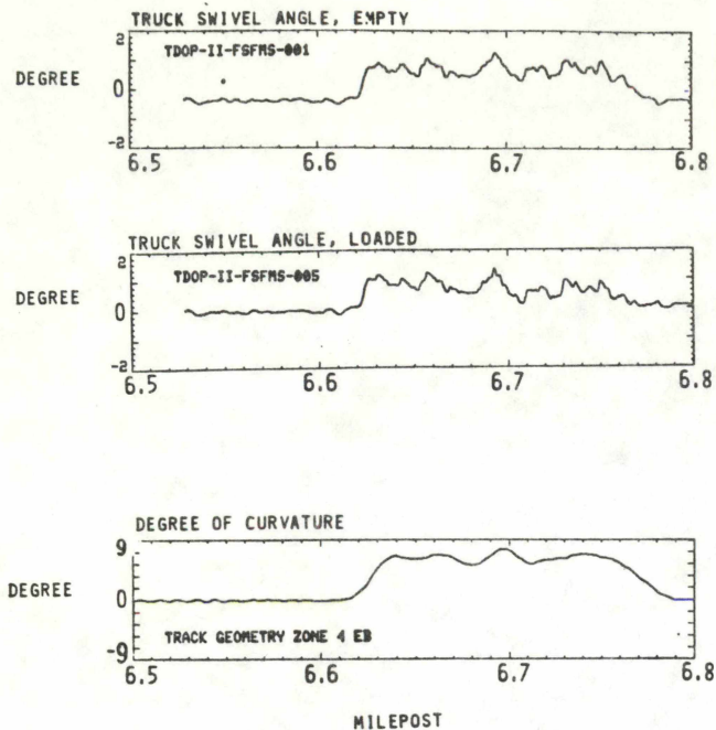
Figure 5-32. Truck Swivel Angle vs Track Curvature, Barber Truck
