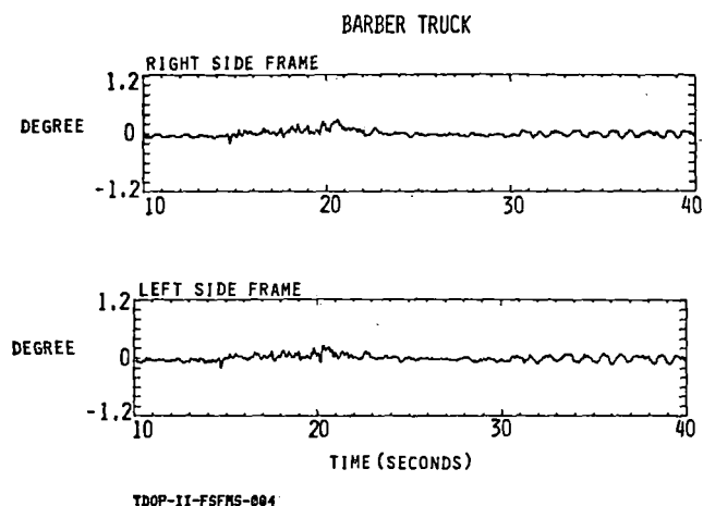
Figure 5-22. Side Frame Yaw Rotation, Barber Truck
