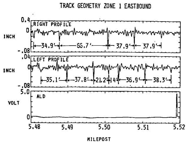
Figure 5-17. Track Geometry Rail Profile
