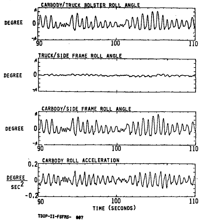
Figure 5-26. Empty ASF Truck Test, Carbody Roll
