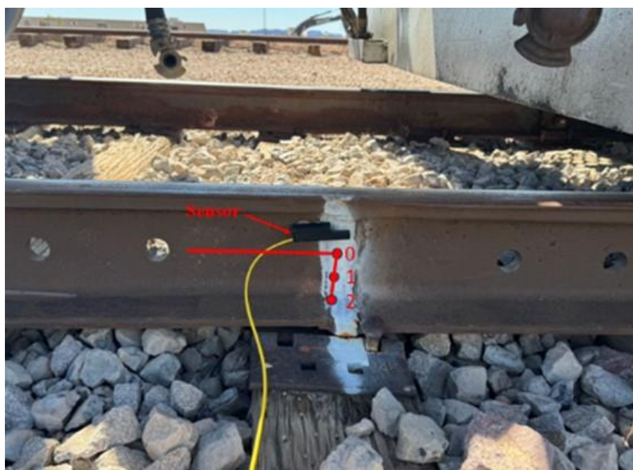
Figure 41 Internal defect location and size
