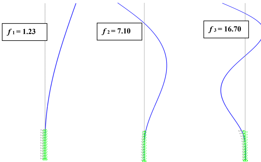
Figure 6.28 Mode shapes and natural frequencies obtained from FEA for Case 4
