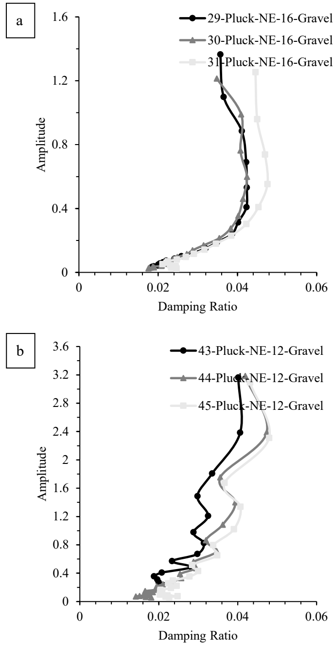
Figure 6.24 The change in damping ratio with amplitude for (a) 16-Gravel pole, and (b) 12-Gravel pole
