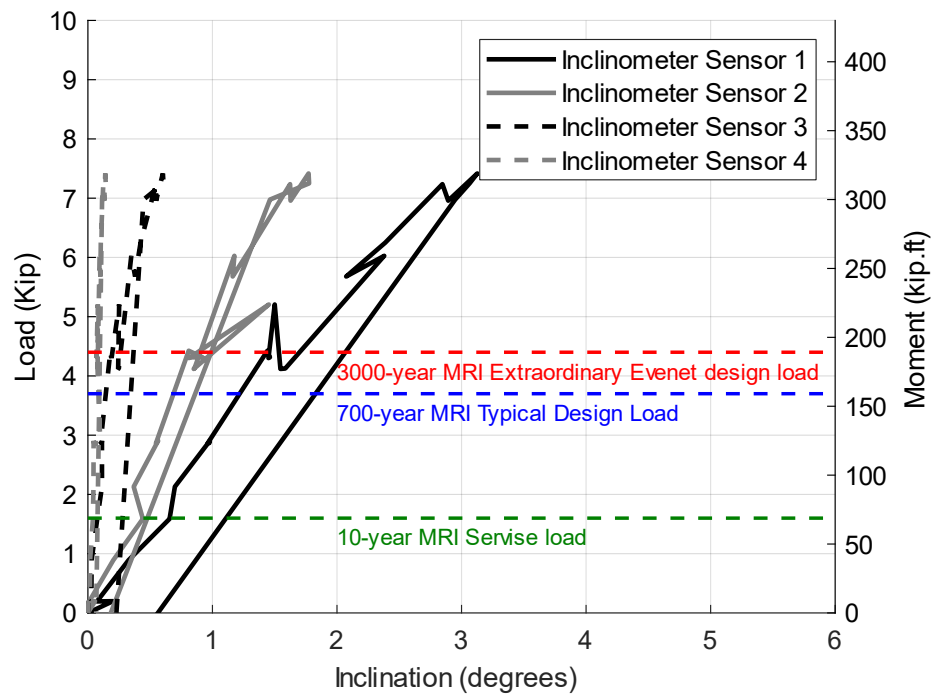
Figure C.13 The results of the first static test performed in the SW direction on Pole 12-Concrete showing the inclination vs load and moment
