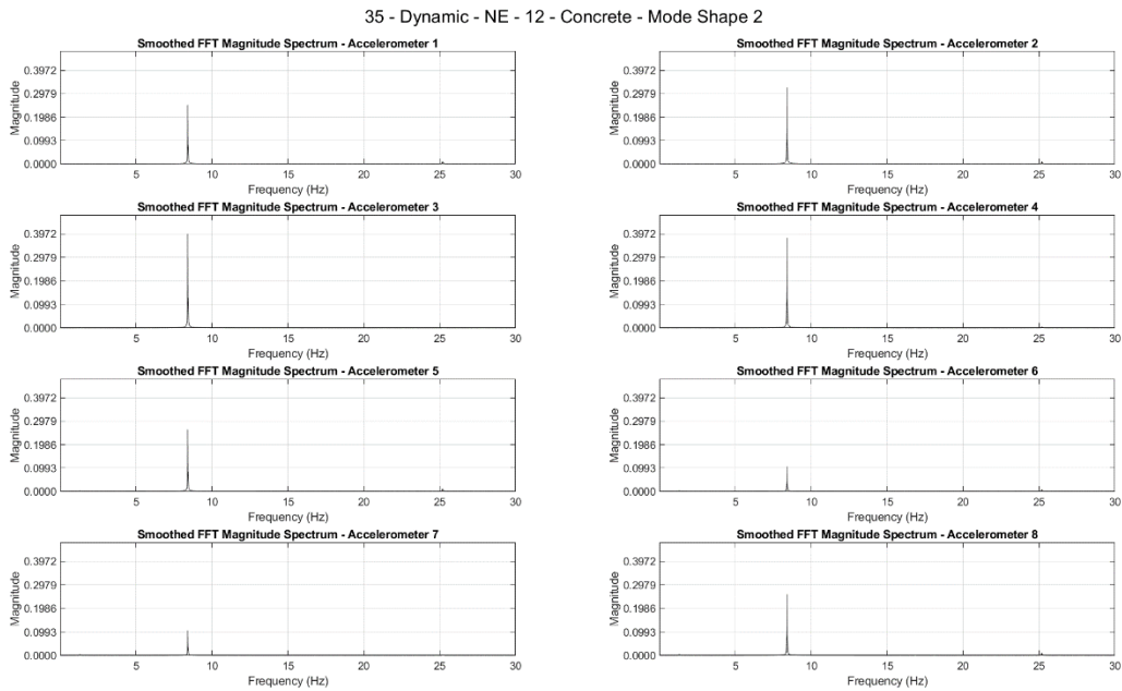
Figure B.14 The results of FFT of the forced vibration test performed on the NE direction on Pole 12-Concrete showing the natural frequency of second mode shape
