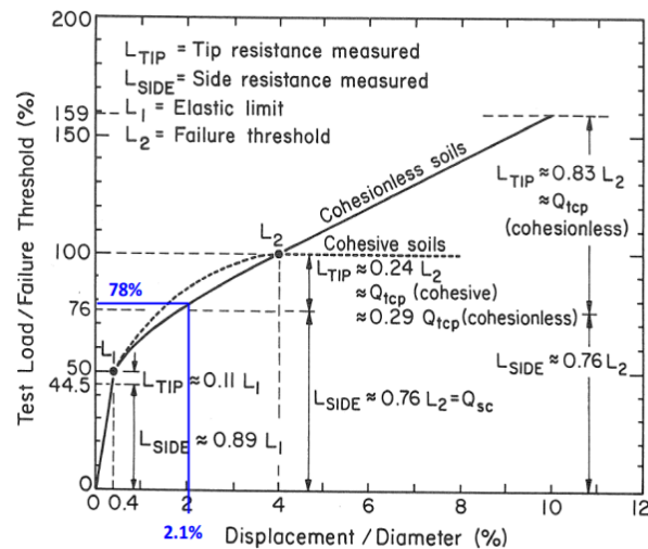
Figure A.2 Normalized load-translation curve
