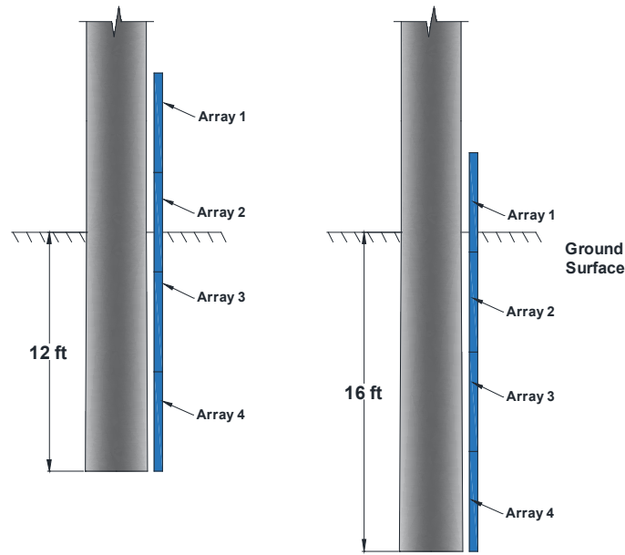
Figure 4.2 Layout of the casing and inclinometer for each embedment length
