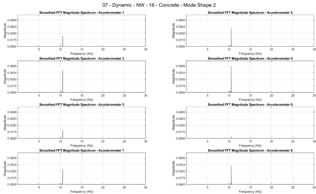
Figure B.2 The results of FFT of the forced vibration test performed in the NW direction on Pole 16-Concrete showing the natural frequency of the second mode shape
