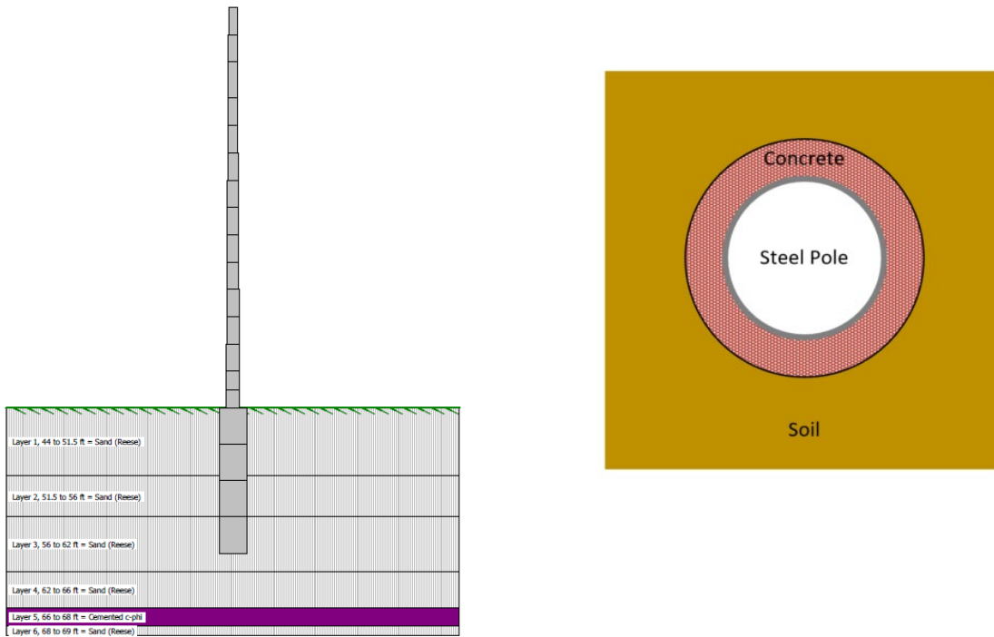
Figure 5.2 Case 1 – modeled in LPILE with a Round Shaft with casing and core/insert, and 16-ft embedment depth
