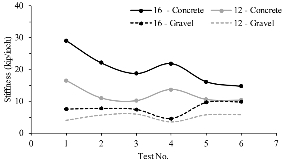
Figure 6.5 Reduction in stiffness for all poles as more static tests performed (tests 1-3 are pulled in one direction, and 4-6 are pulled in the opposite direction)
