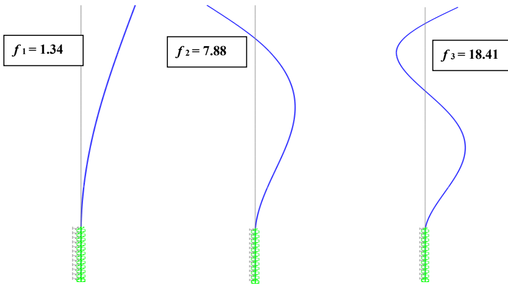
Figure 6.30 Mode shapes and natural frequencies obtained from FEA for Case 6
