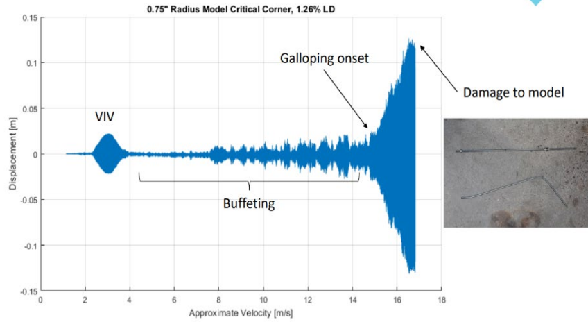
Figure 7.9 Wind-tunnel testing of a multisided pole section (courtesy of WYDOT)
