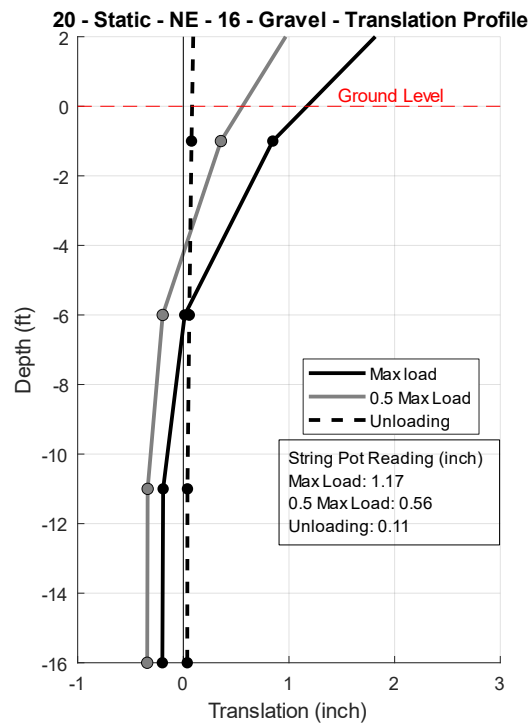
Figure 6.7 Translation vs depth of static tests on NE direction performed on pole 16 – Gravel, the 700-yr design load is approximately 0.5 of the maximum load
