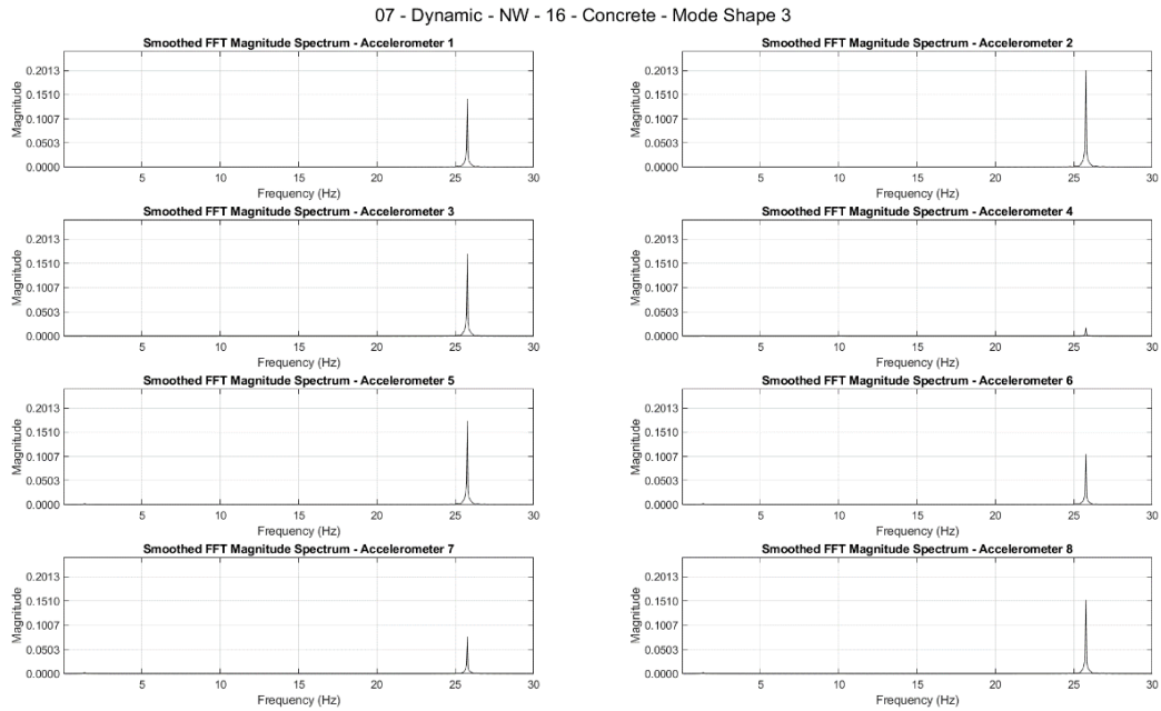
Figure B.3 The results of FFT of the forced vibration test performed in the NW direction on Pole 16-Concrete showing the natural frequency of the third mode shape
