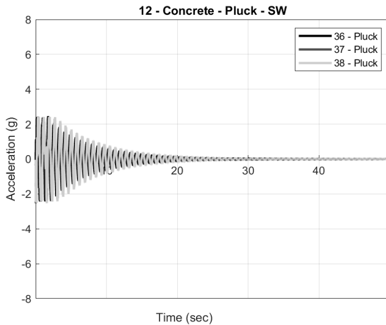
Figure 6.18 Time vs acceleration response of the pluck tests performed in the SW direction for pole 12–Concrete
