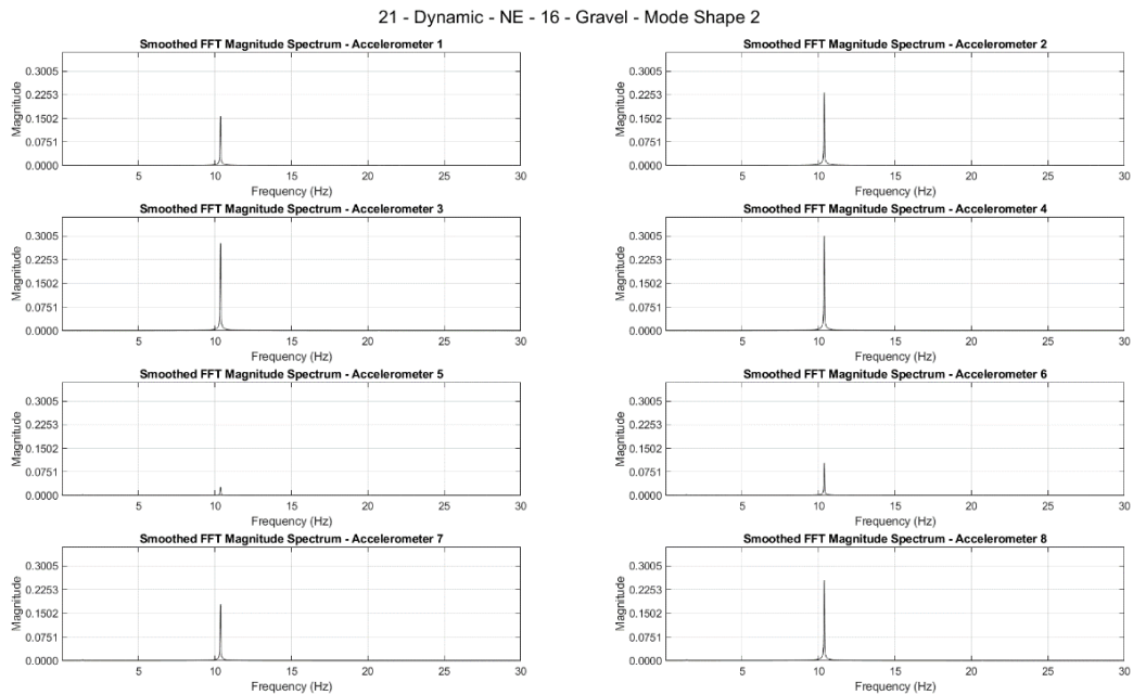
Figure B.8 The results of FFT of the forced vibration test performed in the NE direction on Pole 16-Gravel showing the natural frequency of the second mode shape
