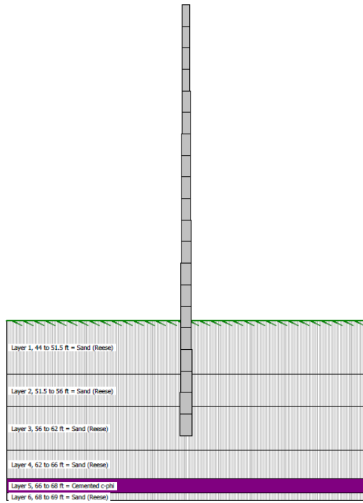
Figure 5.4 Case 3 – modeled in LPILE with steel pipe section and 16-ft embedment depth
