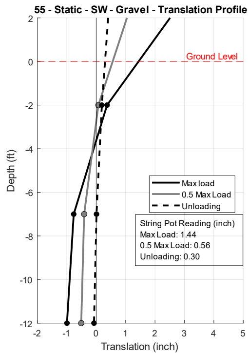
Figure 6.12 Translation vs depth of static tests on SW direction performed on pole 12–Gravel, the 700-yr design load is approximately 0.5 of the maximum load
