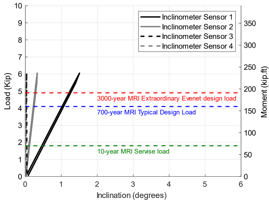
Figure C.2 The results of the second static test performed in the SE direction on Pole 16-Concrete showing the inclination vs load and moment
