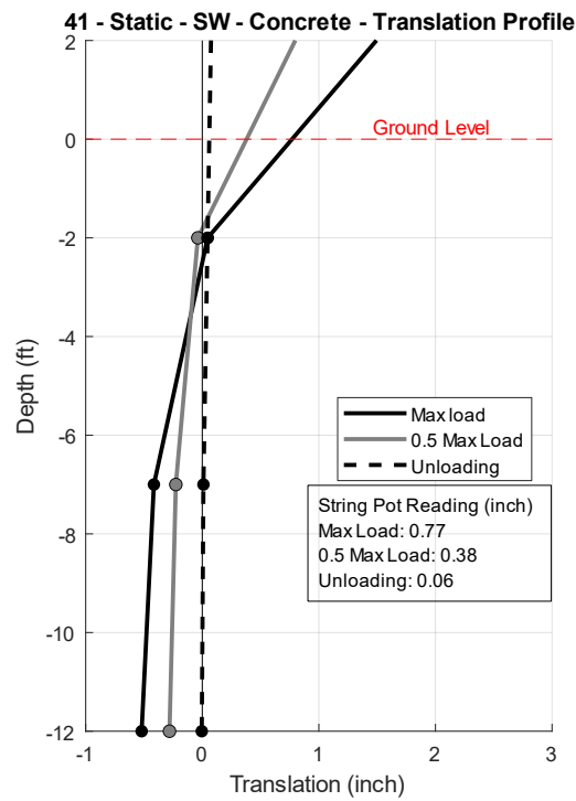
Figure 6.10 Translation vs depth of static tests on SW direction performed on pole 12–Concrete, the 700-yr design load is approximately 0.5 of the maximum load
