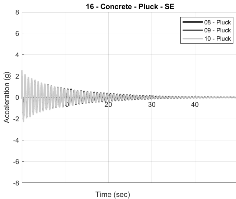
Figure 6.14 Time vs acceleration response of the pluck tests performed in the SE direction for pole 16-Concrete
