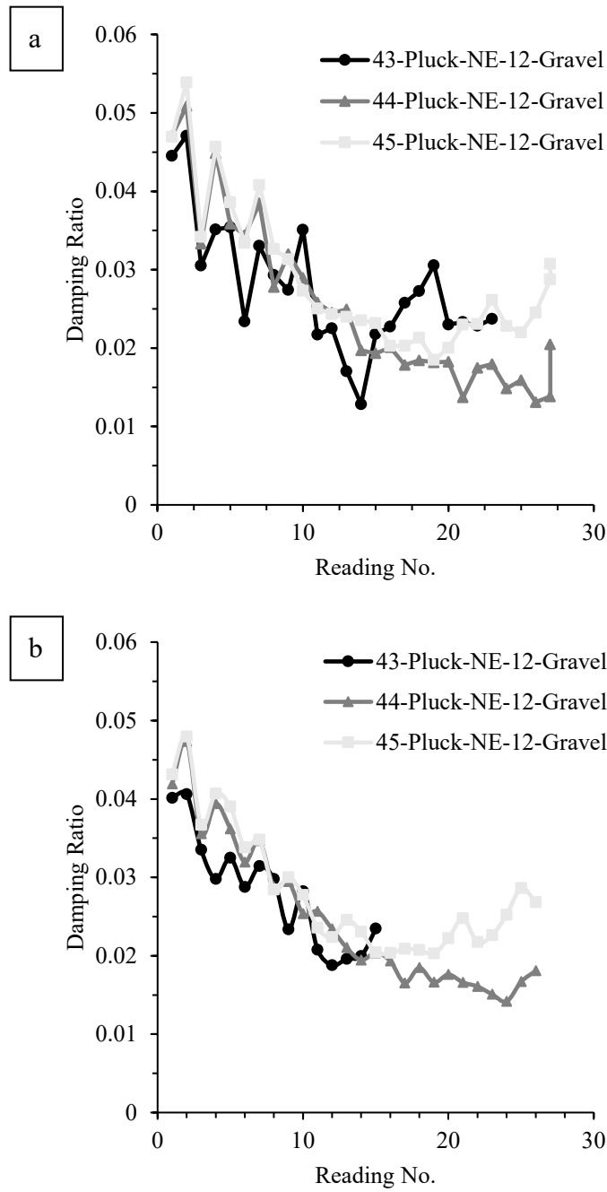
Figure 6.23 The reduction in damping ratio with time for 12-Gravel pole (a) 5-cycle running, and (b) 7-cycle running
