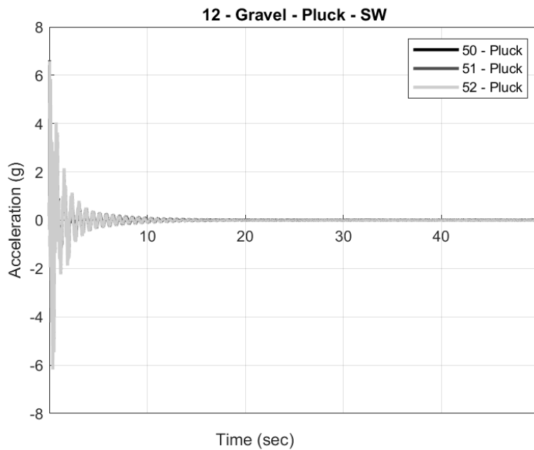
Figure 6.20 Time vs acceleration response of the pluck tests performed in the SW direction for pole 12-Gravel
