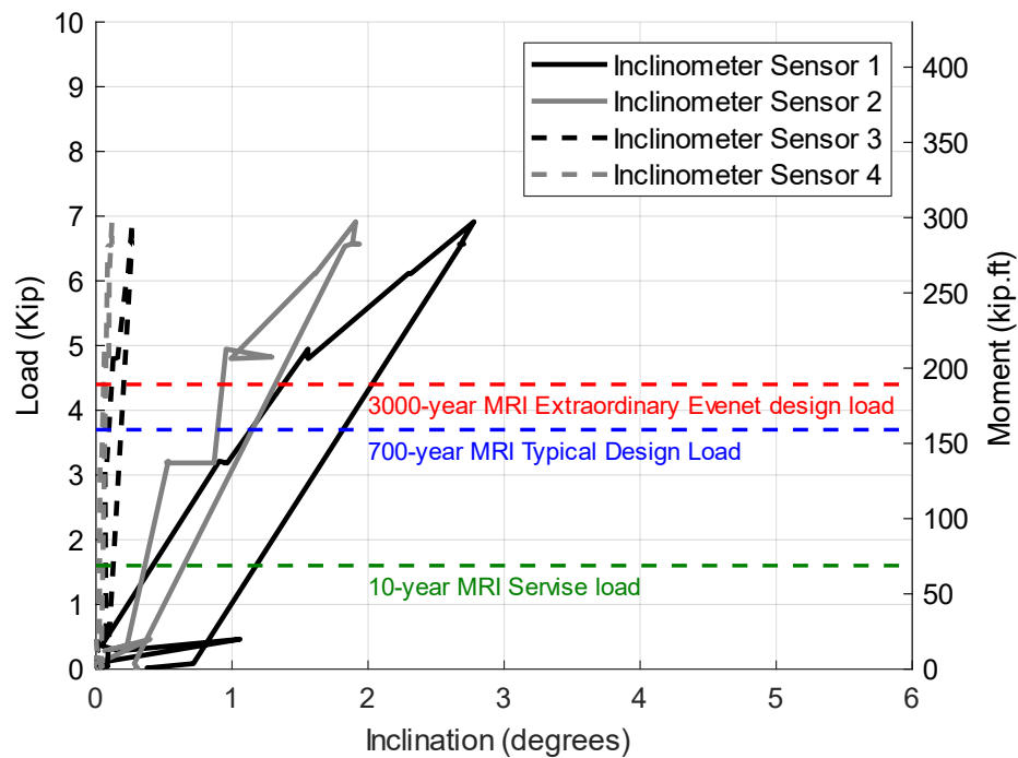
Figure C.10 The results of the first static test performed in the NE direction on Pole 12-Concrete showing the inclination vs load and moment
