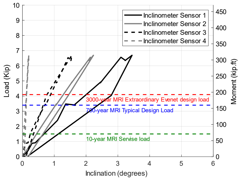
Figure C.18 The results of the second static test performed in the NE direction on Pole 12-Gravel showing the inclination vs load and moment
