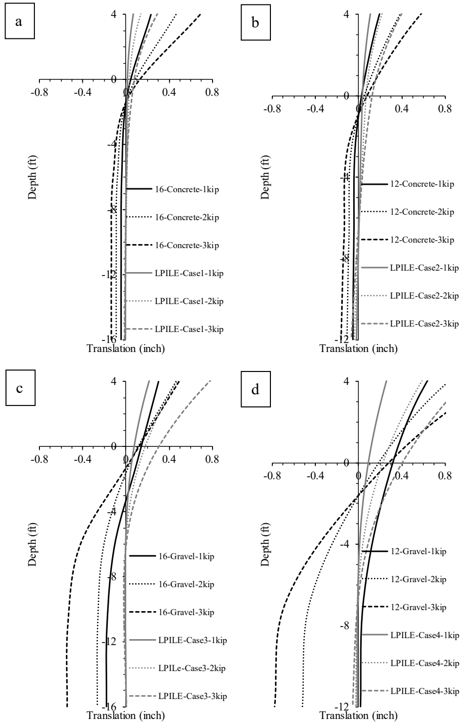
Figure 7.3 Comparison between the translation profile obtained from experimental results and LPILE for poles with different backfill and embedment depths at various loads (a) pole with concrete backfill and 16-ft embedment depths, (b) pole with concrete backfill and 12-ft embedment depths, (c) pole with gravel backfill and 16-ft embedment depths, and (d) pole with gravel backfill and 12-ft embedment depths
