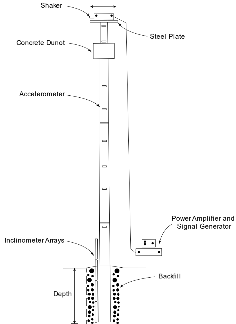
Figure 4.19 Forced-vibration test setup
