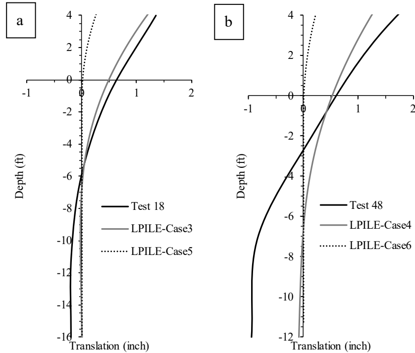
Figure 6.31 Comparison between LPILE cases for gravel backfill (a) 16-foot gravel backfilled pole, and (b) 12-foot backfilled pole
