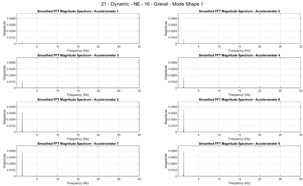
Figure B.7 The results of FFT of the forced vibration test performed on the NE direction on Pole 16-Gravel showing the natural frequency of first mode shape
