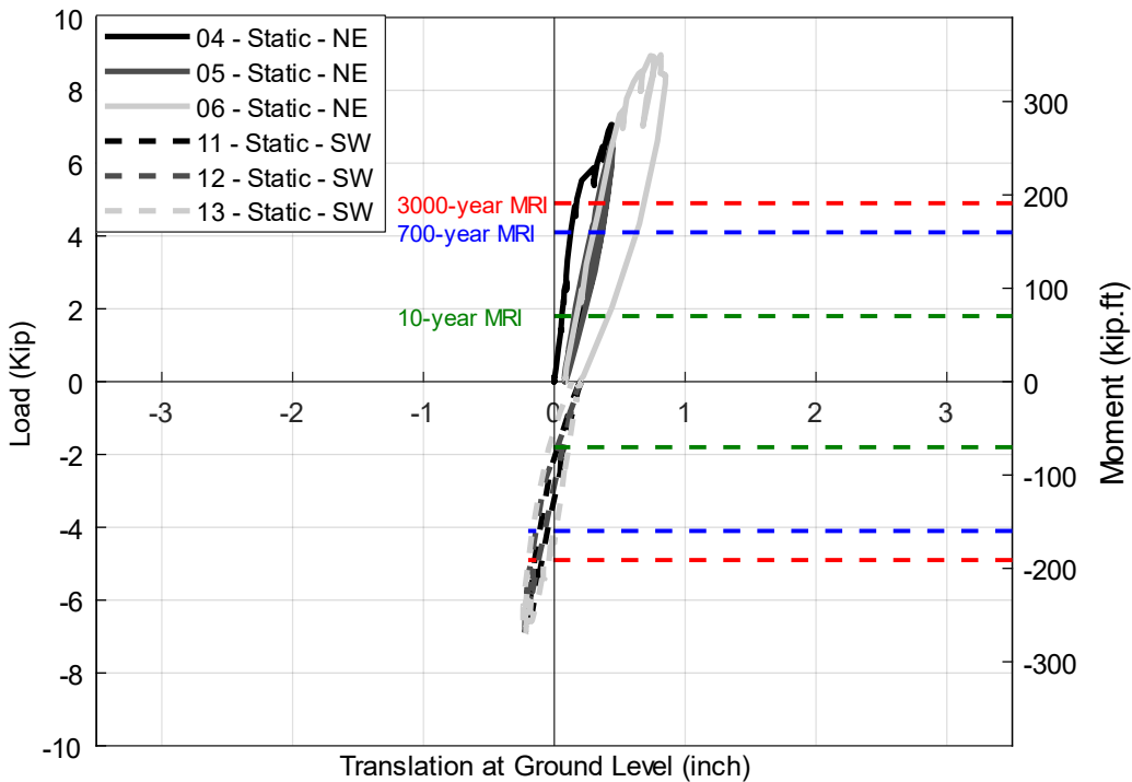
Figure 6.1 The load and moment vs translation at ground level of static tests performed on pole 16-Concrete
