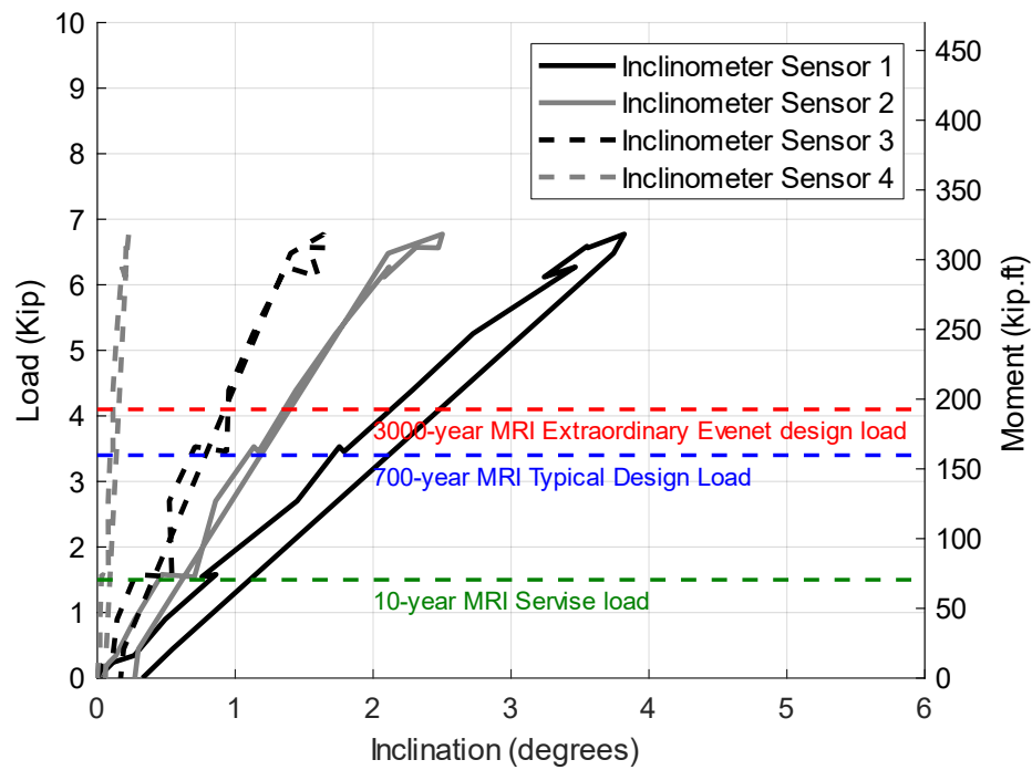
Figure C.17 The results of the second static test performed in the NE direction on Pole 12-Gravel showing the inclination vs load and moment
