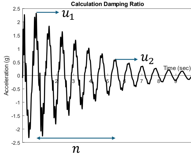
Figure 5.11 Illustration of a log-decrement method to calculate the damping ratio
