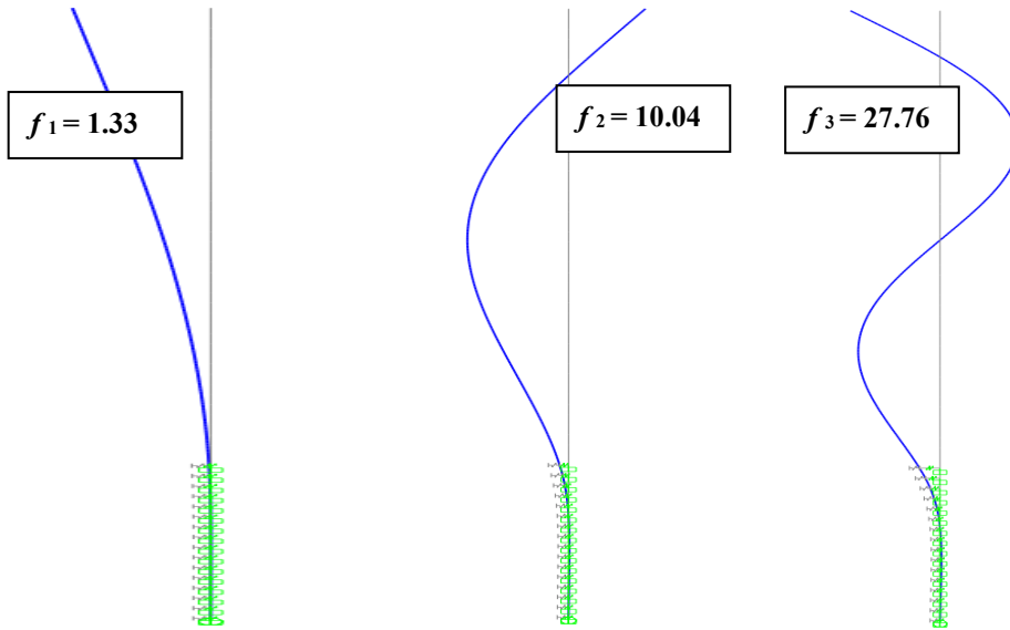
Figure 6.27 Mode shapes and natural frequencies obtained from FEA for Case 3
