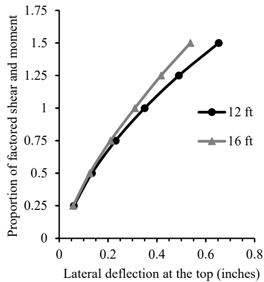
Figure A. 5 Lateral translation at the top with loads increments for steel pipe case
