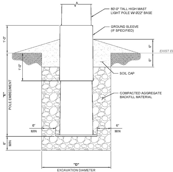
Figure 3.6 Section in directly embedded foundations of poles with gravel backfill
