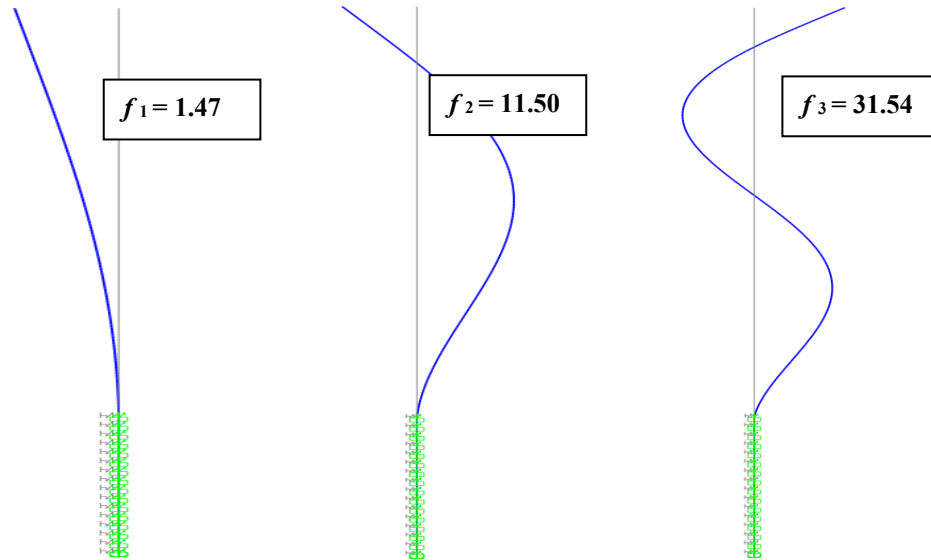
Figure 6.29 Mode shapes and natural frequencies obtained from FEA for Case 5
