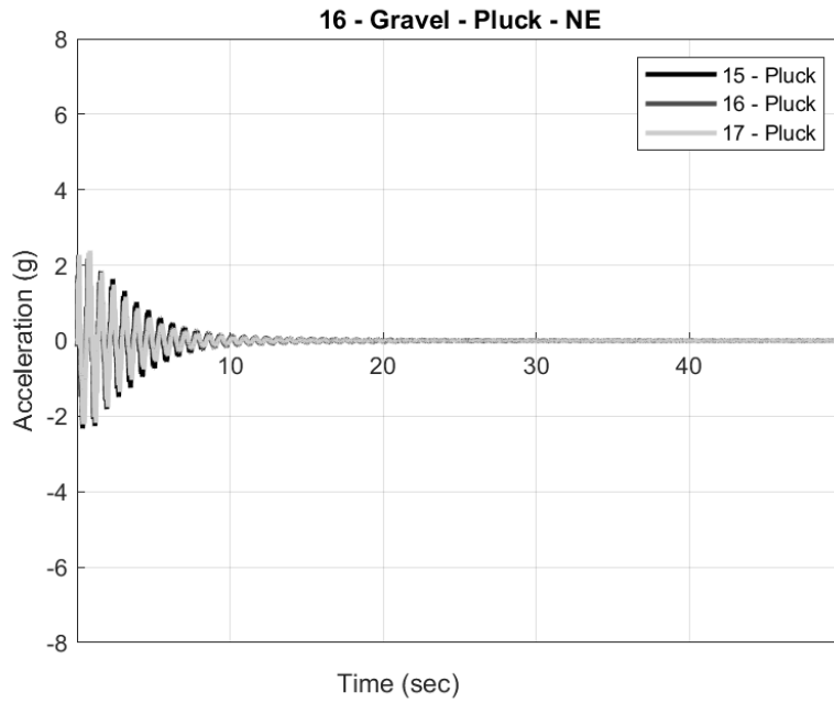
Figure 6.15 Time vs acceleration response of the pluck tests performed in the NE direction for pole 16–Gravel
