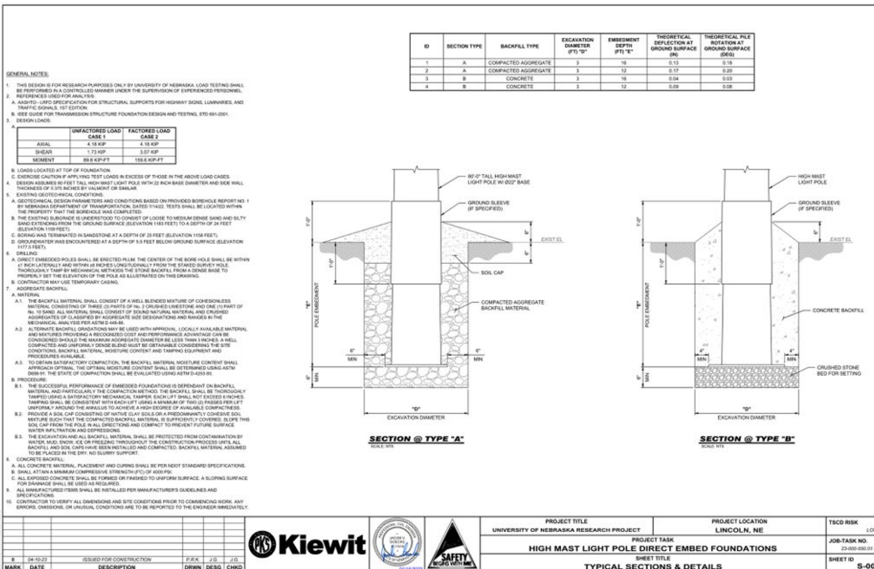
Figure F.4 High mast light pole direct embed foundations. (a) gravel backfill , and (b) concrete backfill
