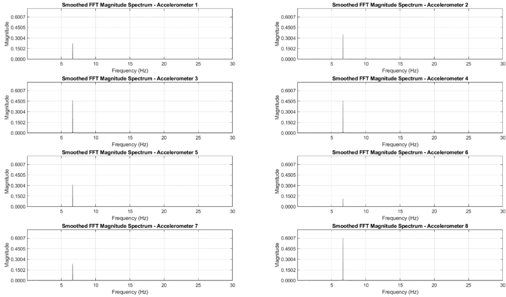
49 - Dynamic - NE - 12 - Gravel - Mode Shape 2
