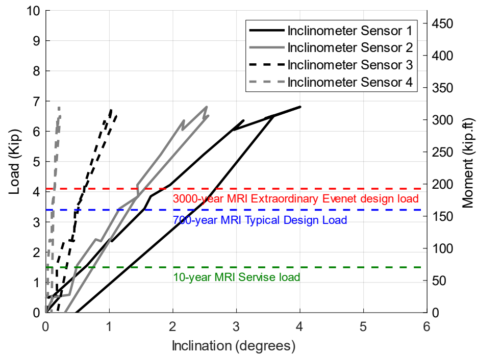
Figure C.21 The results of the third static test performed in the SW direction on Pole 12-Gravel showing the inclination vs load and moment
