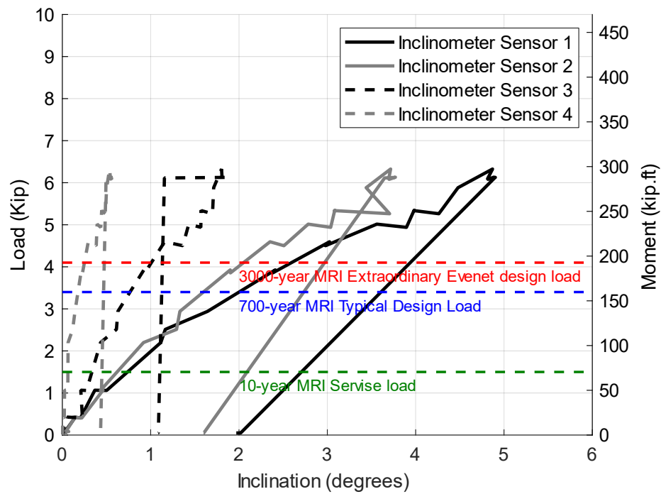
Figure C.19 The results of the first static test performed in the SW direction on Pole 12-Gravel showing the inclination vs load and moment
