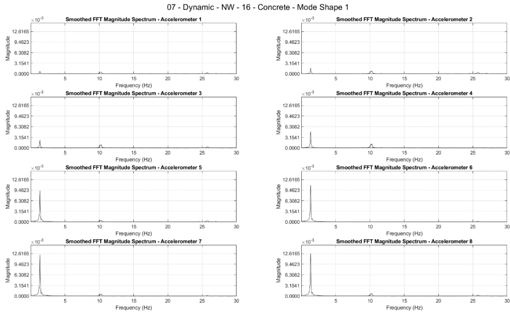
Figure B.1 The results of FFT of the forced vibration test performed on the NW direction on Pole 16-Concrete showing the natural frequency of first mode shape
