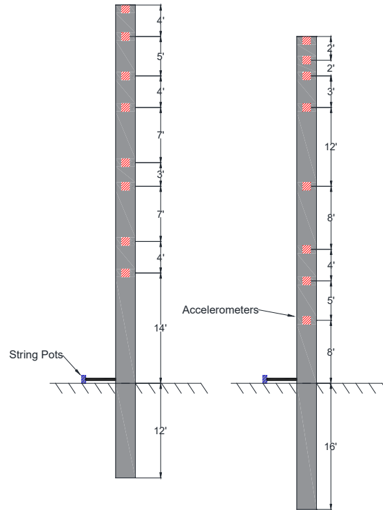
Figure 4.12 Locations of accelerometers installed for the dynamic tests for 12- and 16-ft direct embedments
