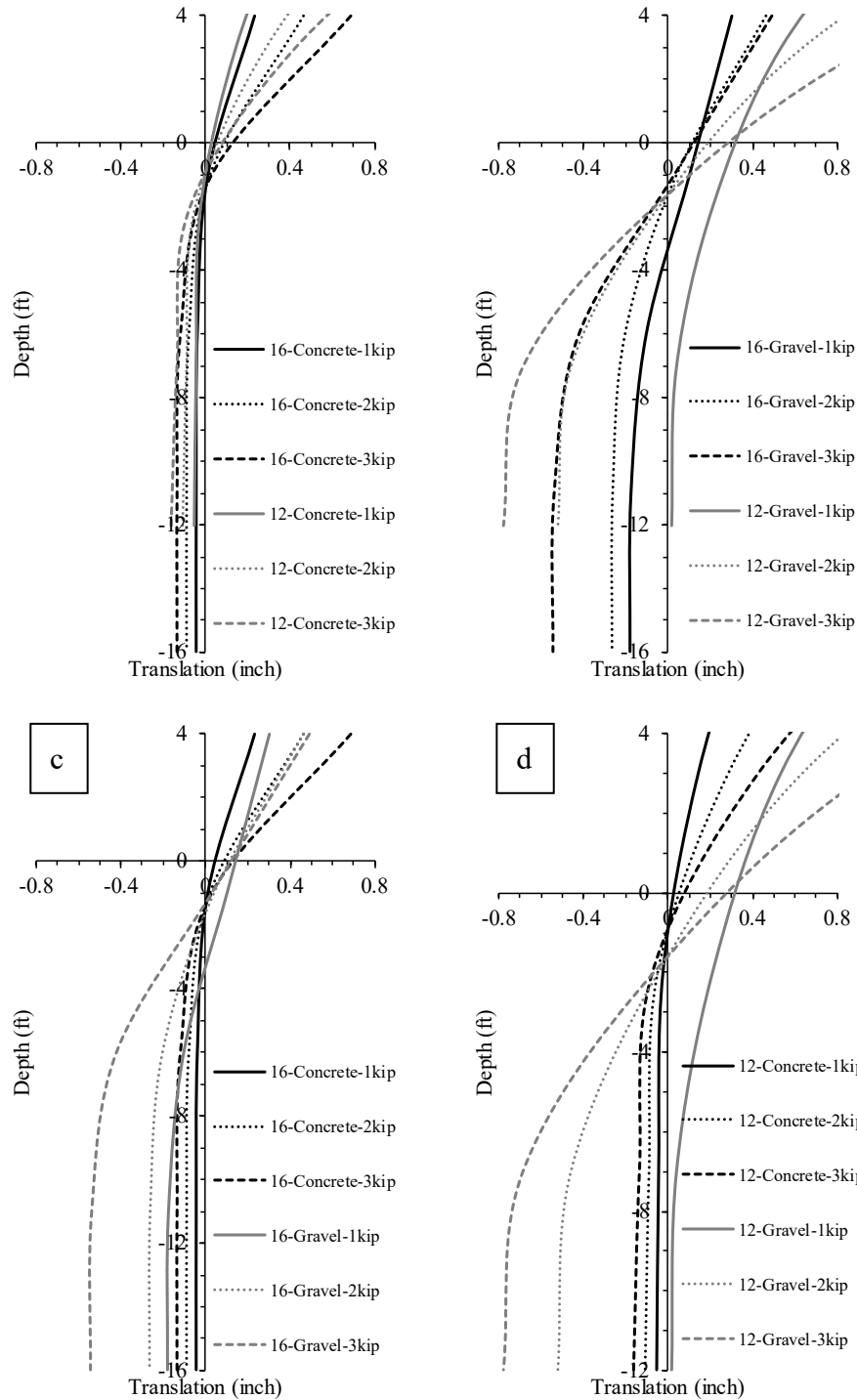
Figure 7.1 Comparison between translation profiles obtained from experimental results for poles with different backfill and embedment depths at various loads (a) pole with concrete backfill and different 16-ft embedment, (b) pole with gravel backfill and different embedment depths, (c) pole with 16-ft embedment depth and concrete backfill, and (d) poles with 12-ft embedment depth and gravel backfill
