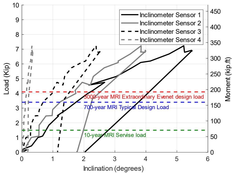
Figure C.16 The results of the first static test performed in the NE direction on Pole 12-Gravel showing the inclination vs load and moment
