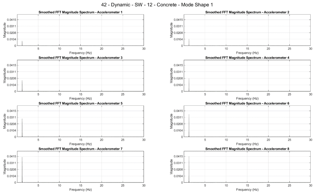
Figure B.16 The results of FFT of the forced vibration test performed in the SW direction on Pole 12-Concrete showing the natural frequency of the first mode shape
