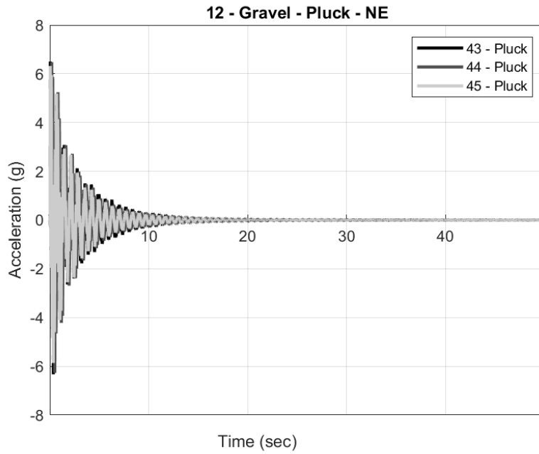
Figure 6.19 Time vs acceleration response of the pluck tests performed in the NE direction for pole 12-Gravel
