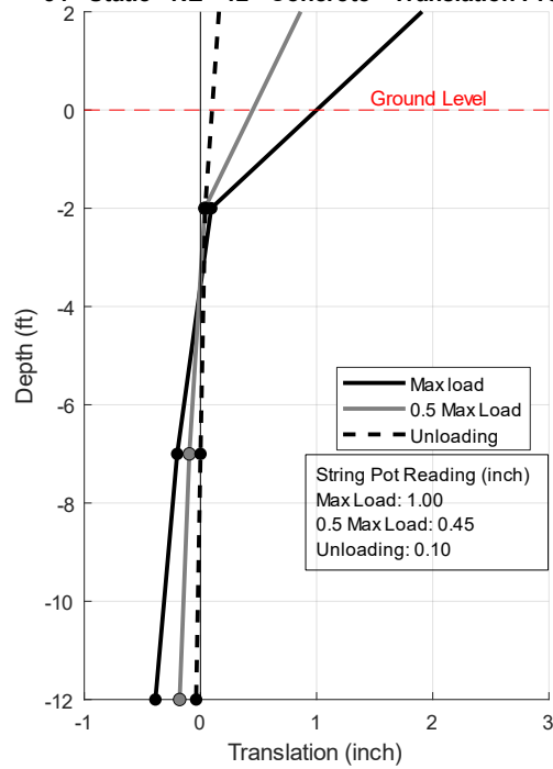
Figure 6.9 Translation vs depth of static tests on NE direction performed on pole 12–Concrete, the 700-yr design load is approximately 0.5 of the maximum load
