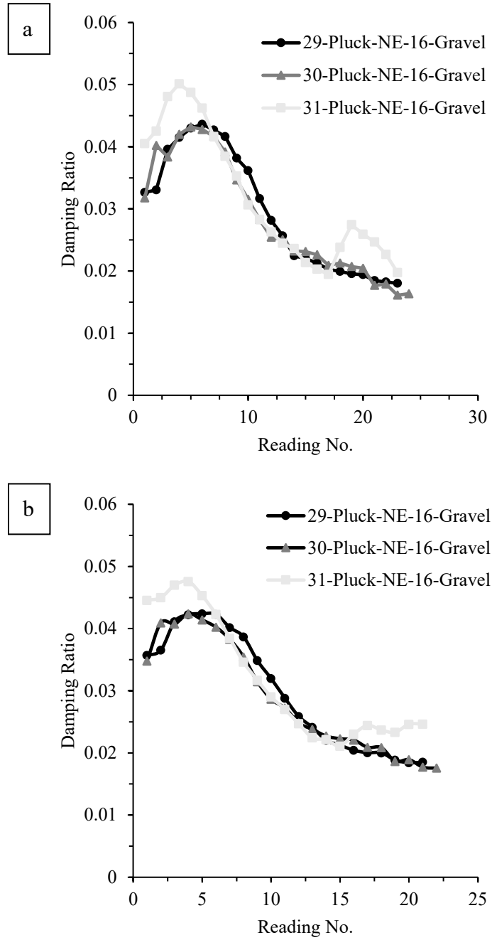
Figure 6.22 The reduction in damping ratio with time for 16-Gravel pole (a) 5-cycle running, and (b) 7-cycle running
