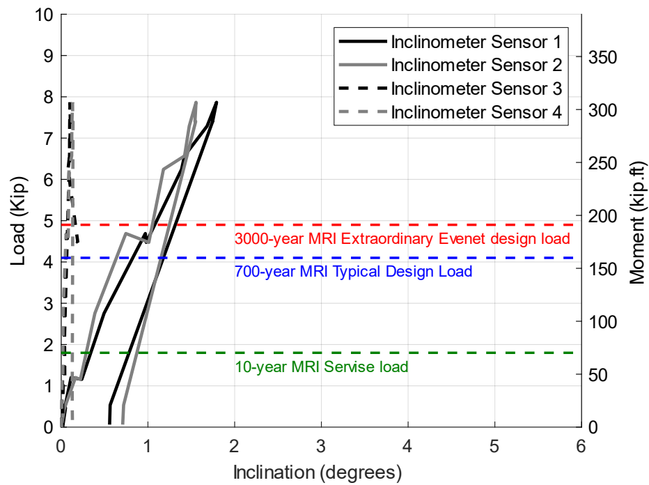
Figure C.7 The results of the first static test performed in the SW direction on Pole 16-Gravel showing the inclination vs load and moment
