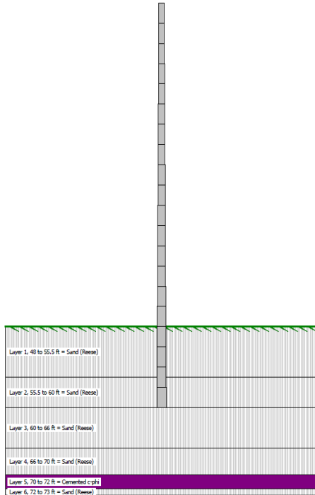
Figure 5.5 Case 4 – modeled in LPILE with steel pipe section and 12-ft embedment depth
