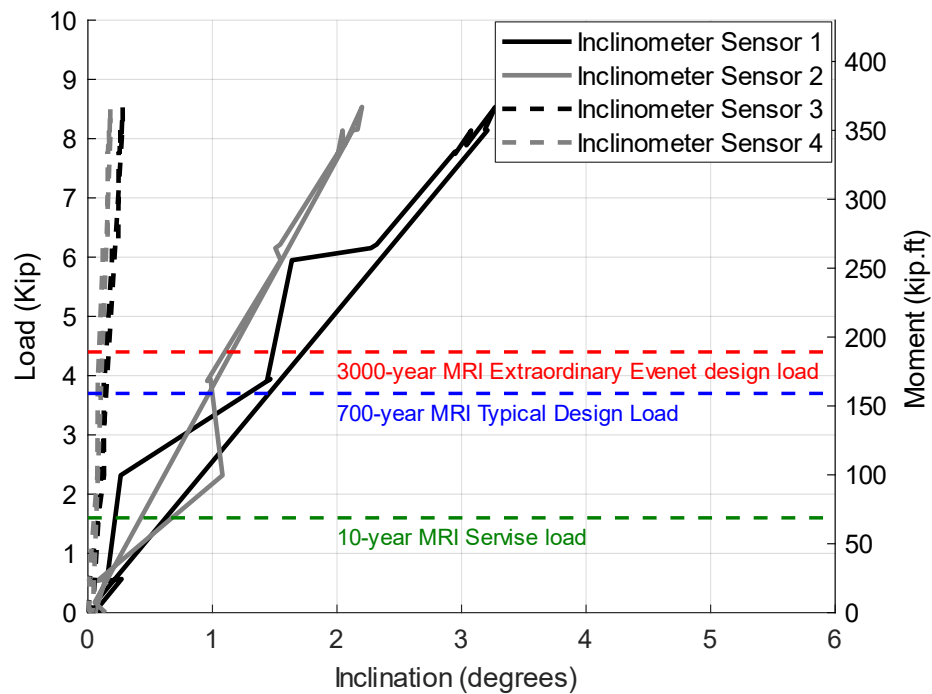
Figure C.12 The results of the third static test performed in the NE direction on Pole 12-Concrete showing the inclination vs load and moment
