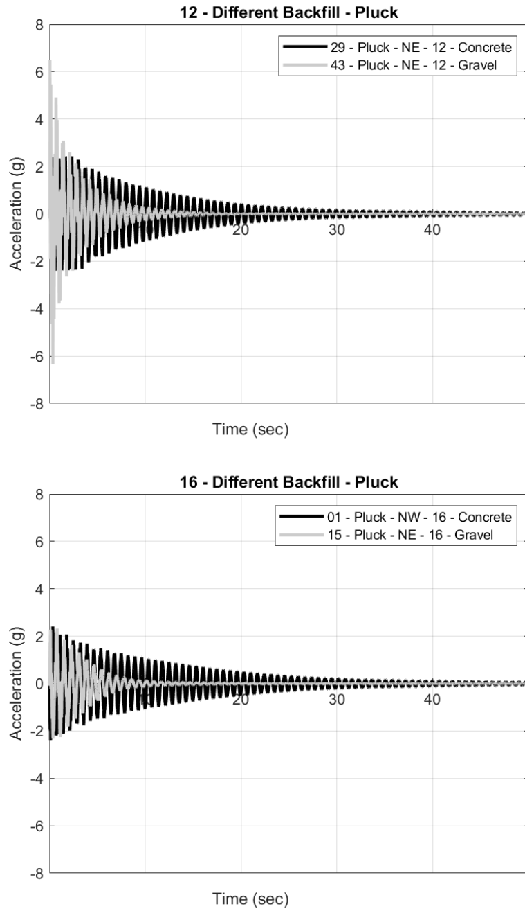
Figure 6.21 Comparison between the damping performance for poles with different backfill material
