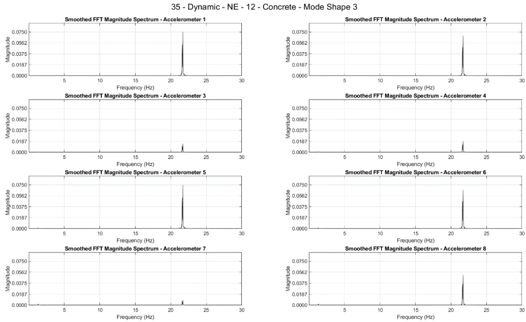
Figure B.15 The results of FFT of the forced vibration test performed in the NE direction on Pole 12-Concrete showing the natural frequency of the third mode shape
