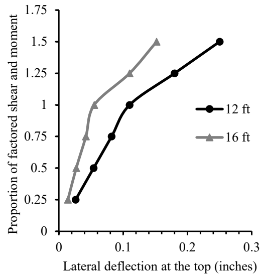
Figure A.4 Lateral translation at the top with loads increments for round shaft case
