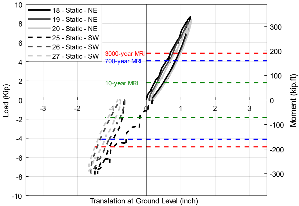
Figure 6.2 The load and moment vs translation at ground level of static tests performed on pole 16-Gravel
