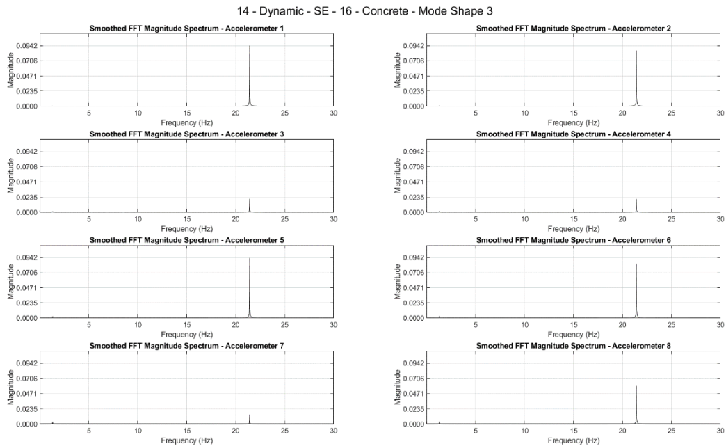
Figure B.6 The results of FFT of the forced vibration test performed on the SE direction in Pole 16-Concrete showing the natural frequency of the third mode shape
