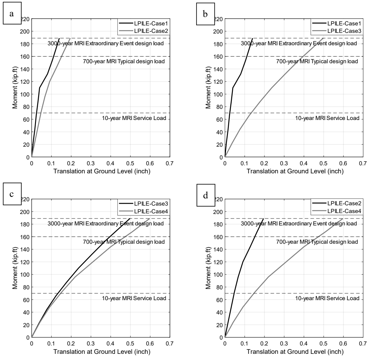
Figure 7.6 A comparison between translation at ground level obtained from LPILE for poles with different backfill and embedment depths (a) cases with concrete backfill and different embedment depths, (b) cases with different backfill and 16 ft embedment depths, (c) cases with gravel backfill and different embedment depths, and (d) cases with different backfill and 12-ft embedment depths
