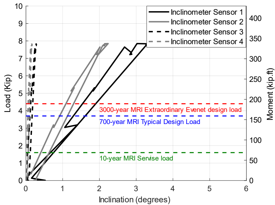
Figure C.11 The results of the second static test performed in the NE direction on Pole 12-Concrete showing the inclination vs load and moment
