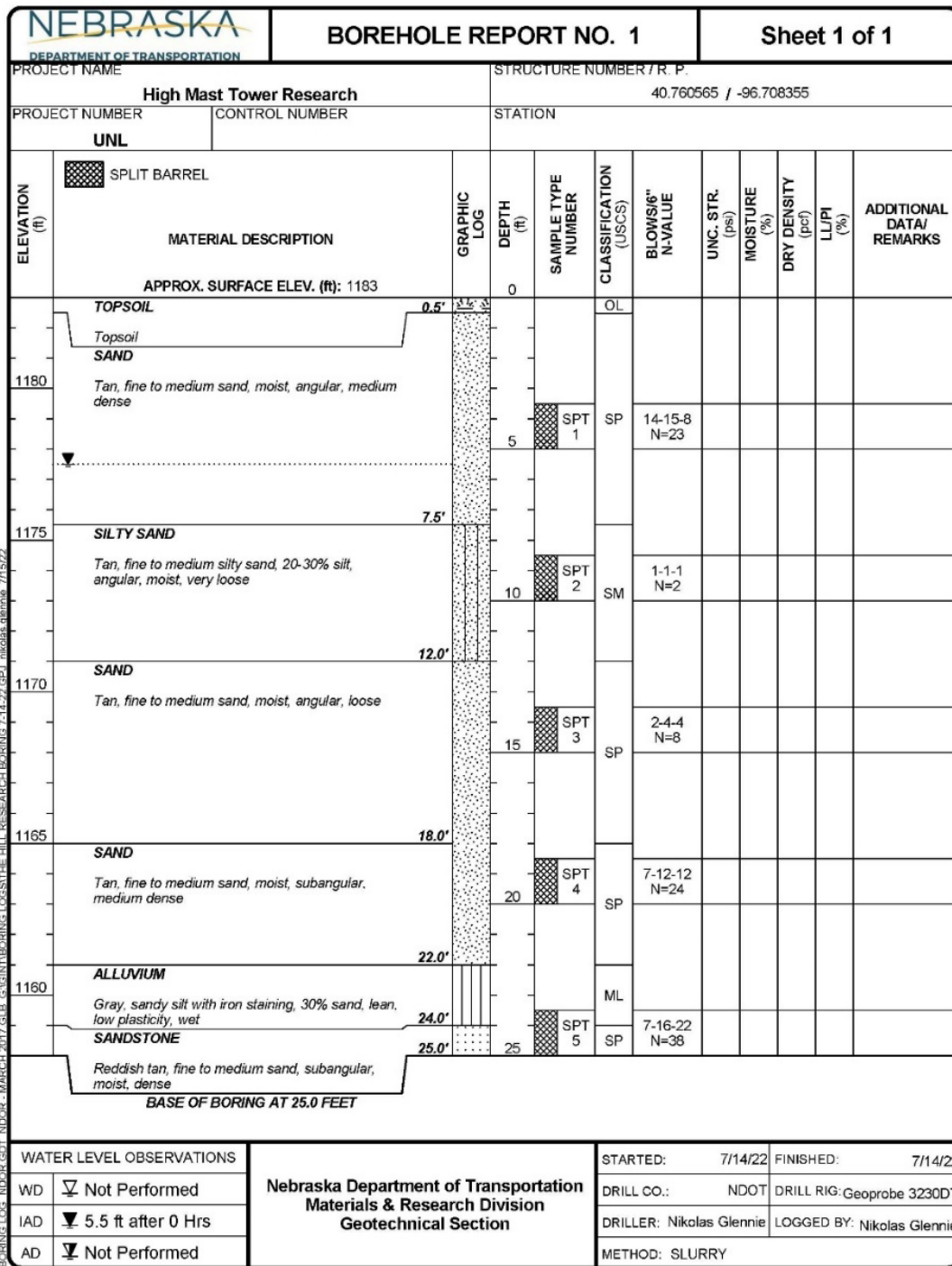
Figure A.1 Borehole report
