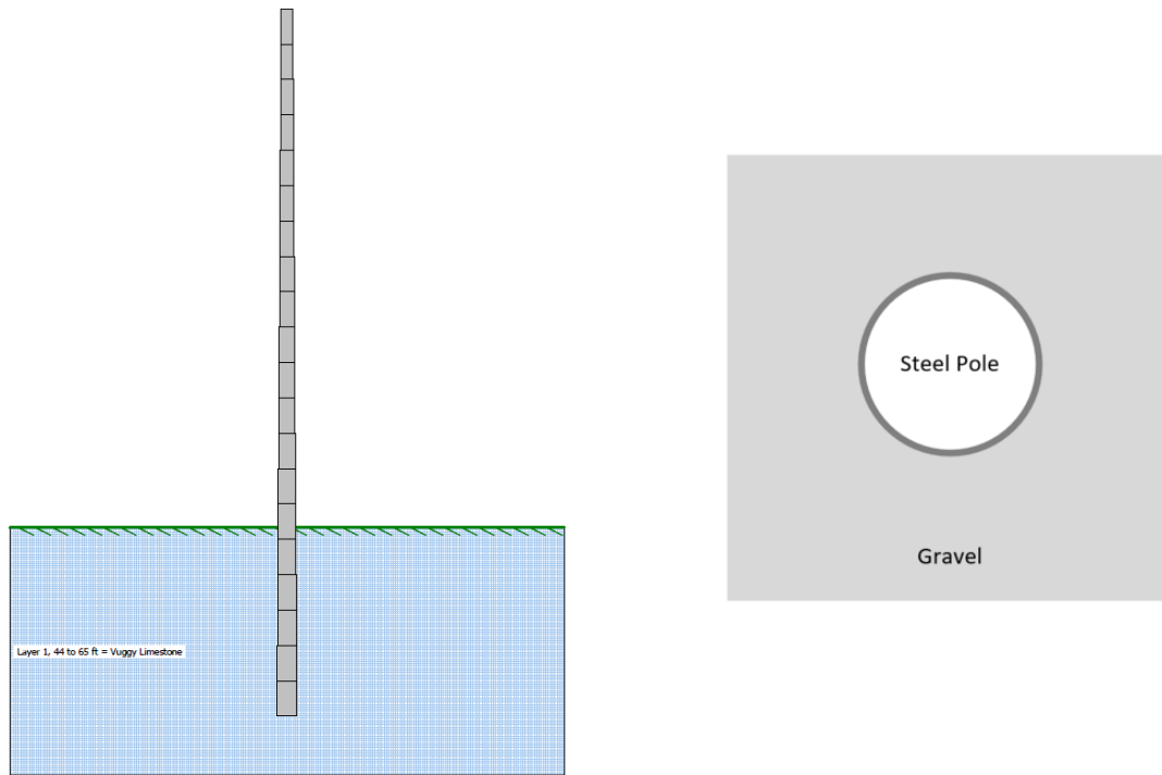
Figure 5.6 Case 5 – modeled in LPILE with steel pipe section, and 16-ft embedment depth surrounding with gravel medium
