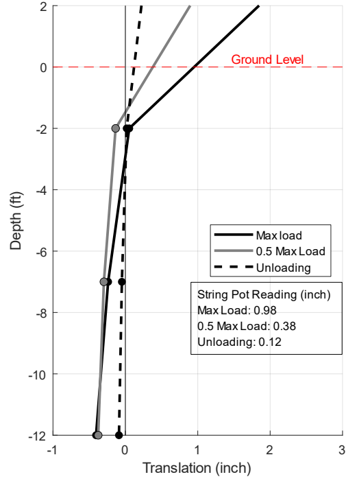
33 - Static - NE - 12 - Concrete - Translation Profile
