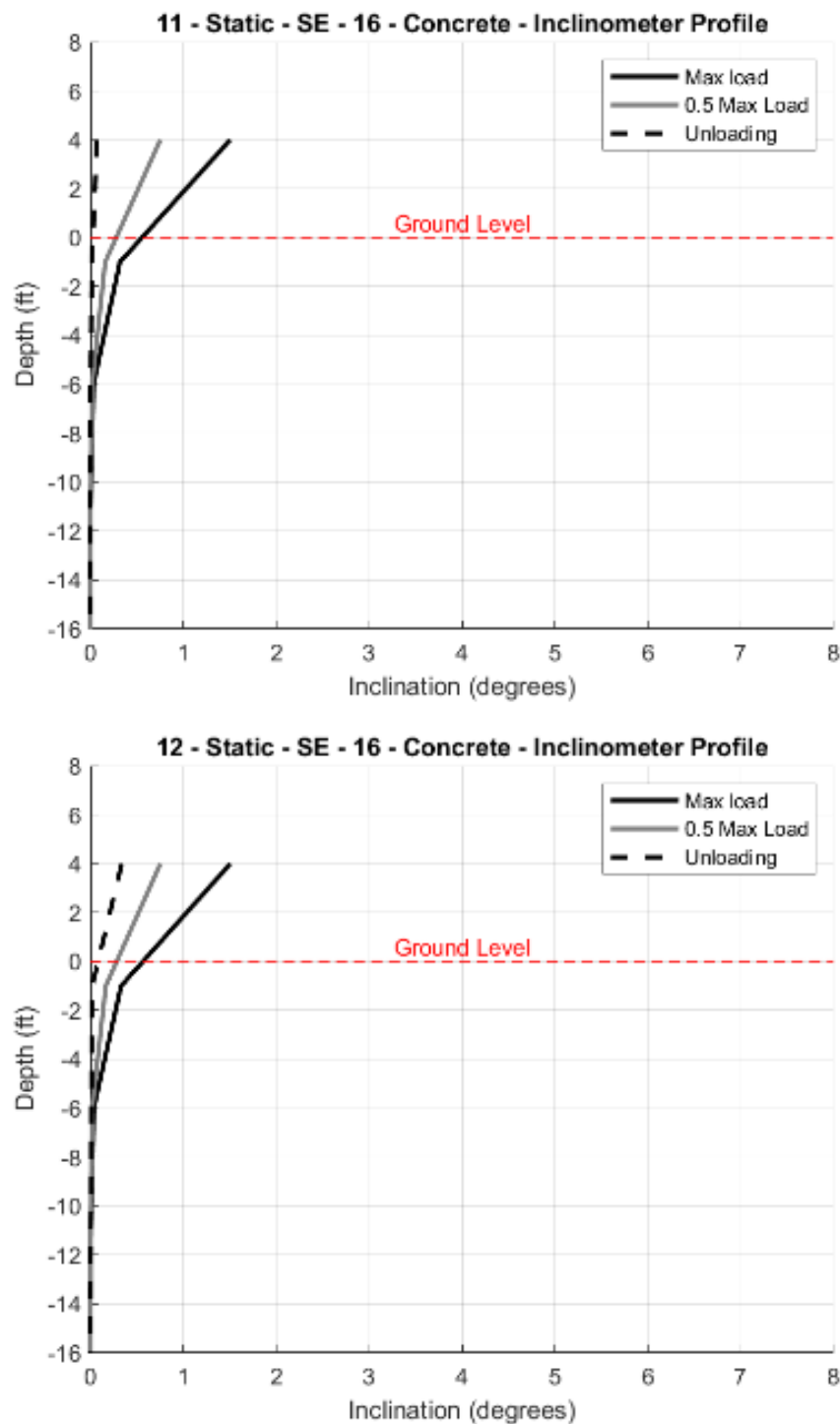
Figure D.1 The rotation vs inclination at ground level of static test 11 and 12 in SE direction performed on pole 16 – Concrete, the 700-yr design load is approximately 0.5 of the maximum load
