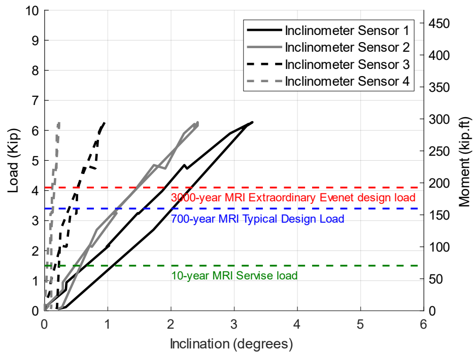
Figure C.20 The results of the second static test performed in the SW direction on Pole 12-Gravel showing the inclination vs load and moment
