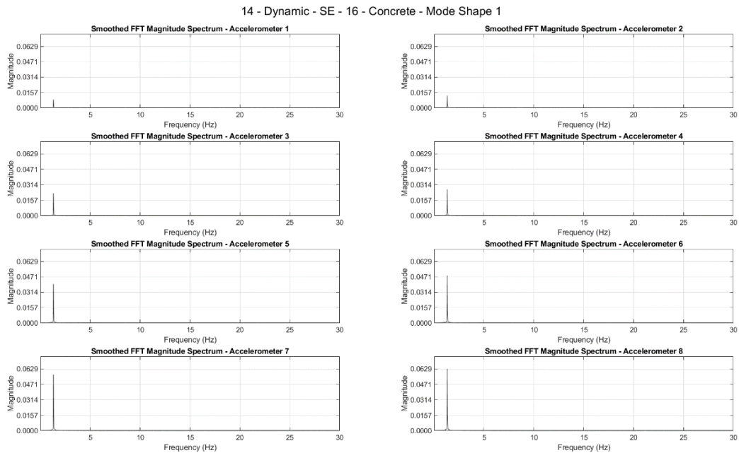
Figure B.4 The results of FFT of the forced vibration test performed in the SE direction on Pole 16-Concrete showing the natural frequency of the first mode shape
