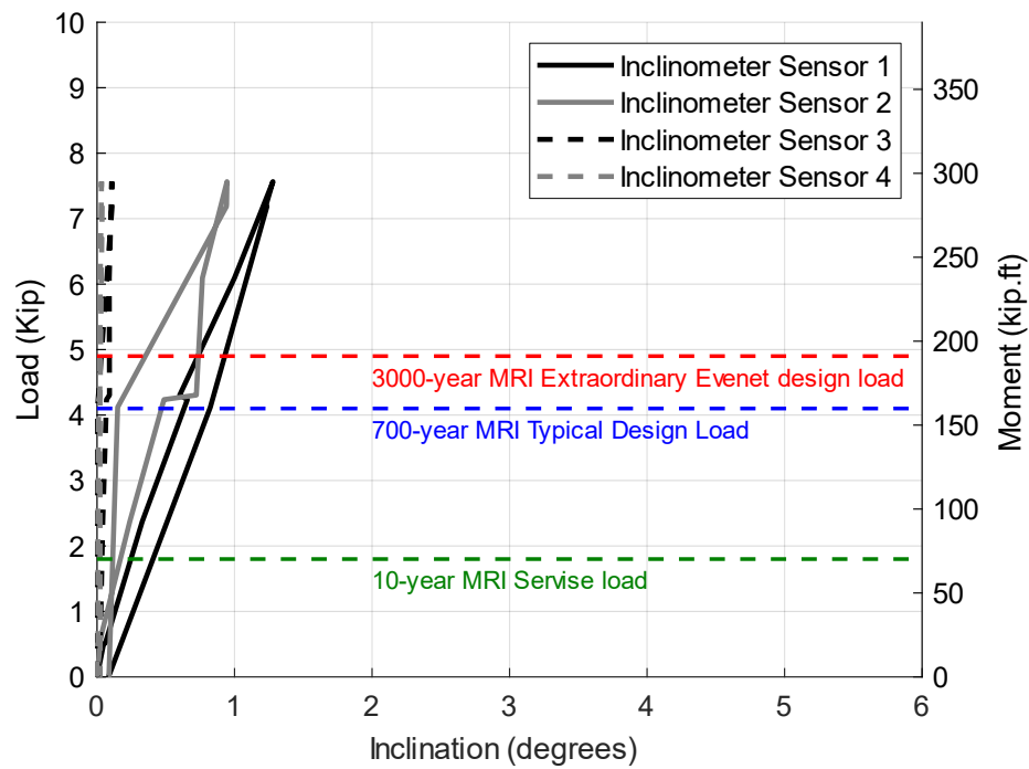
Figure C.8 The results of the second static test performed in the SW direction on Pole 16-Gravel showing the inclination vs load and moment
