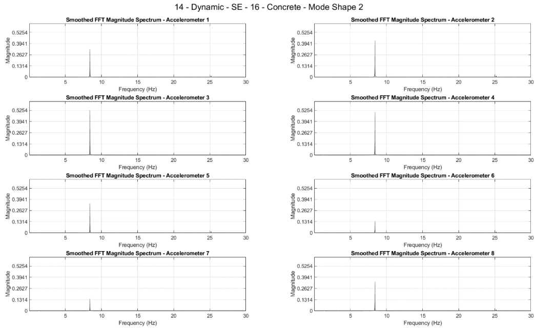
Figure B.5 The results of FFT of the forced vibration test performed on the SE direction in Pole 16-Concrete showing the natural frequency of the second mode shape
