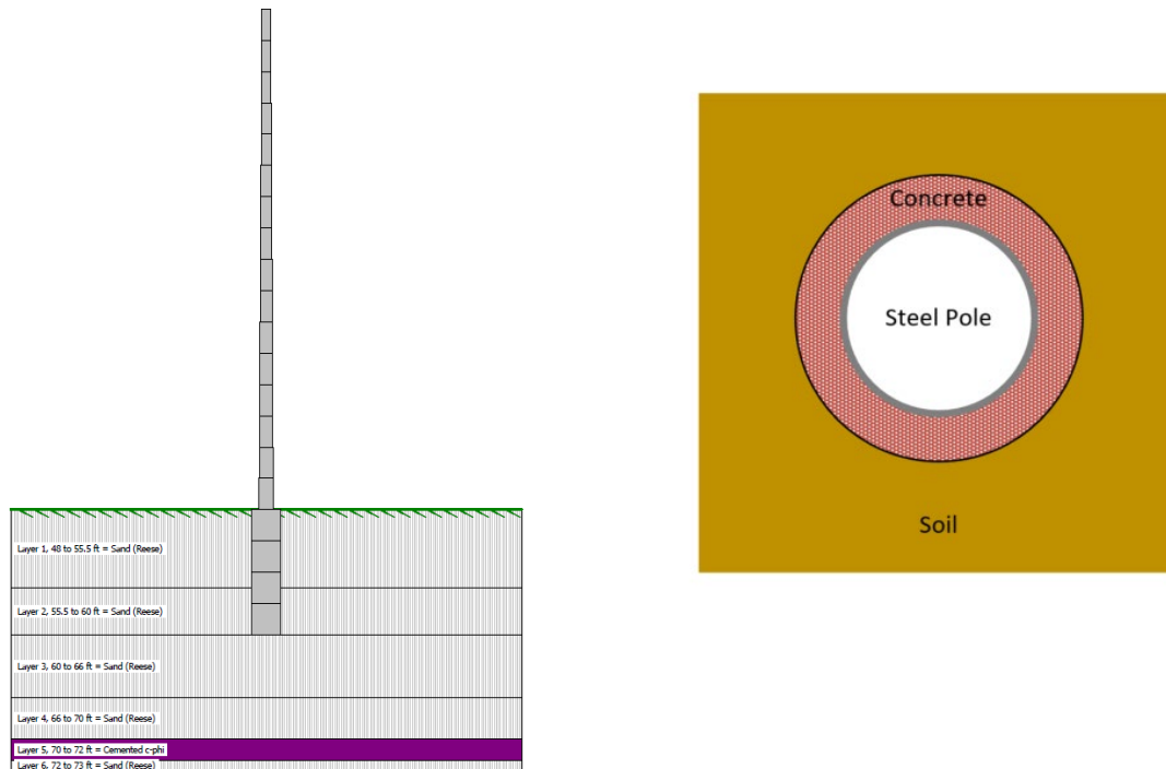
Figure 5.3 Case 2 – modeled in LPILE with Round Shaft with casing and core/insert, and 16-ft embedment depth
