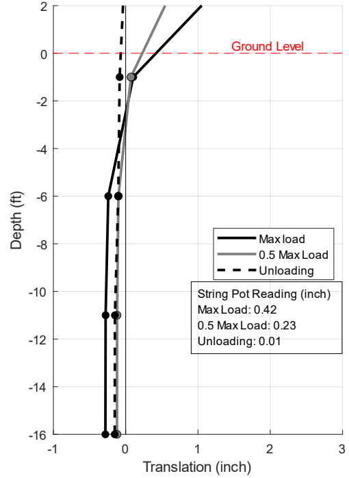
12 - Static - SE - 16 - Concrete - Translation Profile
