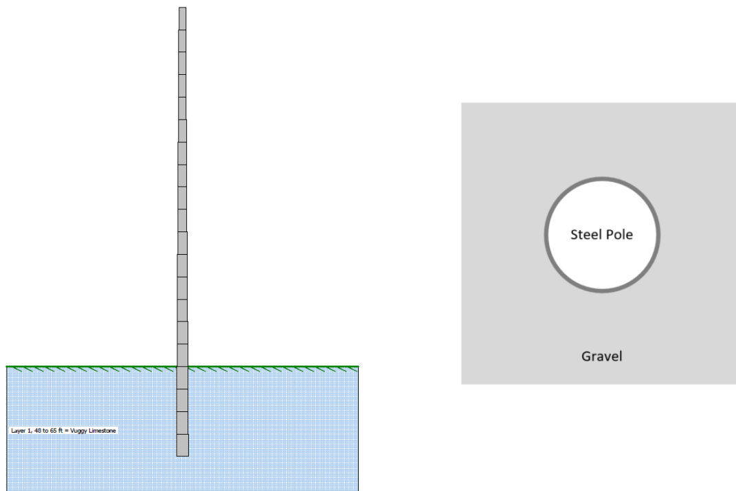
Figure 5.7 Case 6 – modeled in LPILE with steel pipe section, and 12-ft embedment depth surrounding with gravel medium
