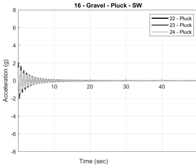
Figure 6.16 The time vs acceleration response of the pluck tests performed in the SW direction for pole 16-Gravel
