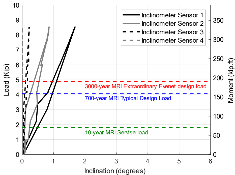
Figure C.4 The results of the first static test performed in the NE direction on Pole 16-Gravel showing the inclination vs load and moment
