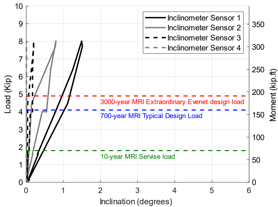
Figure C.5 The results of the second static test performed in the NE direction on Pole 16-Gravel showing the inclination vs load and moment
