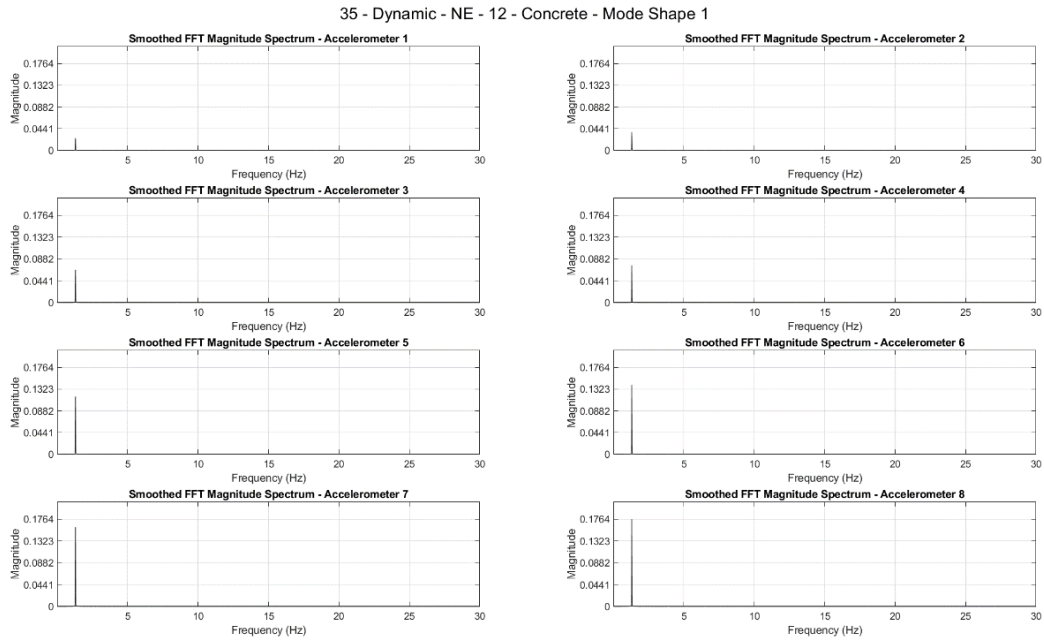
Figure B.13 The results of FFT of the forced vibration test performed in the NE direction on Pole 12-Concrete showing the natural frequency of the first mode shape
