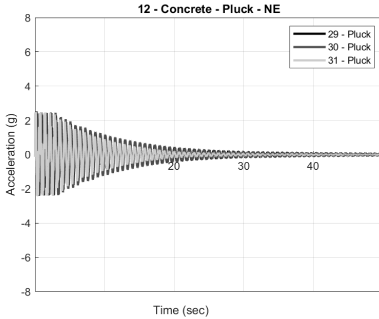
Figure 6.17 Time vs acceleration response of the pluck tests performed in the NE direction for pole 12–Concrete
