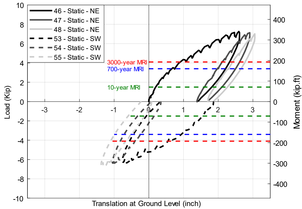
Figure 6.4 The load and moment vs translation at ground level of static tests performed on pole 12-Gravel
