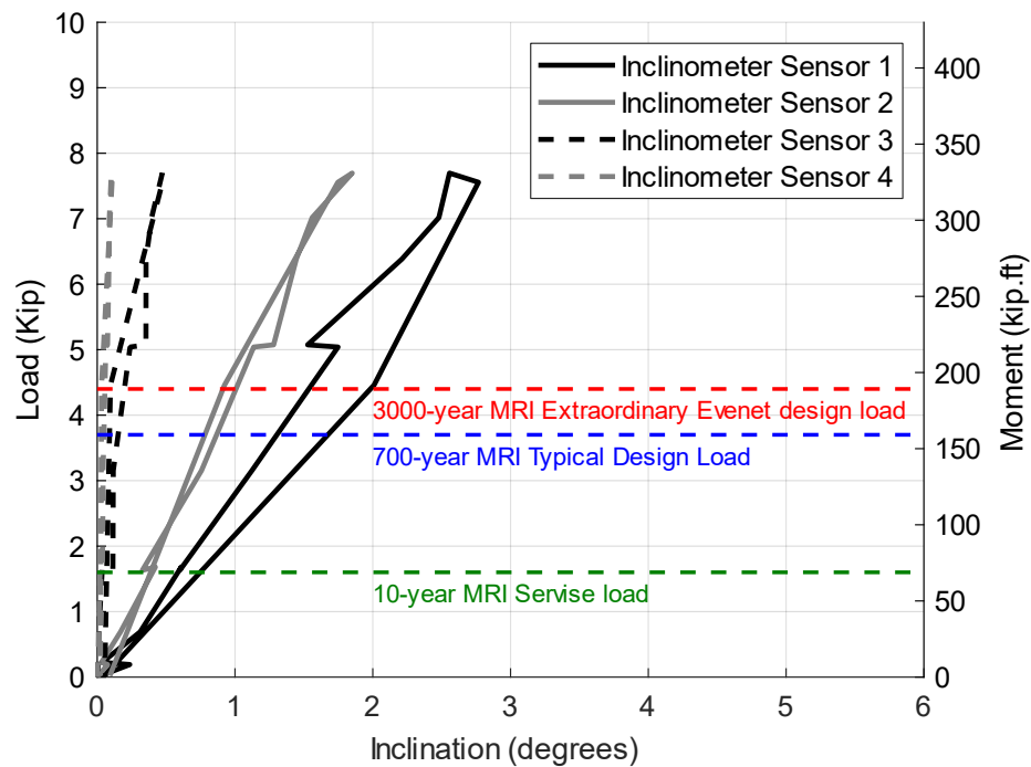
Figure C.14 The results of the second static test performed in the SW direction on Pole 12-Concrete showing the inclination vs load and moment
