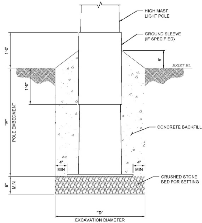
Figure 3.5 Section for directly embedded foundations of poles with concrete backfill
