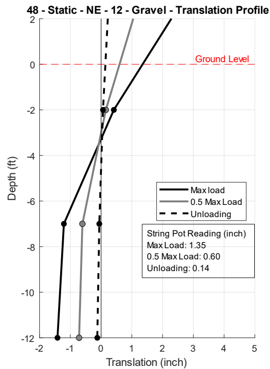
Figure 6.11 Translation vs depth of static tests on NE direction performed on pole 12–Gravel, the 700-yr design load is approximately 0.5 of the maximum load
