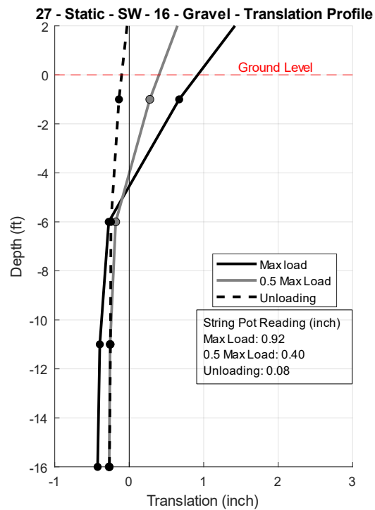
Figure 6.8 Translation vs depth of static tests on SW direction performed on pole 16–Gravel, the 700-yr design load is approximately 0.5 of the maximum load
