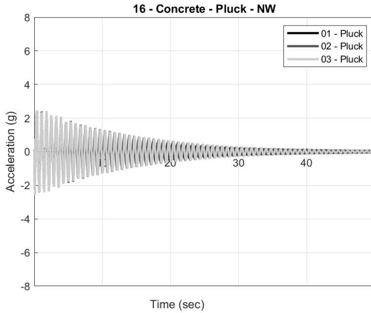
Figure 6.13 Time vs acceleration response of the pluck tests performed in the NW direction for pole 16-Concrete
