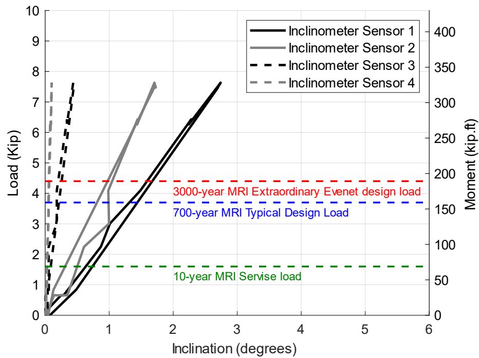
Figure C.15 The results of the third static test performed in the SW direction on Pole 12-Concrete showing the inclination vs load and moment
