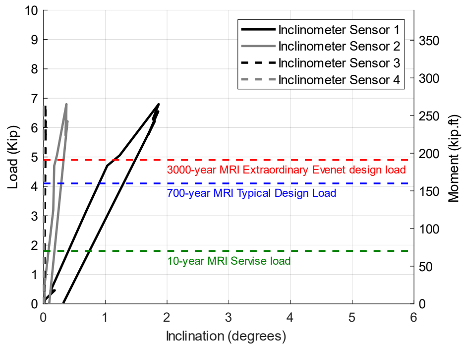
Figure C.3 The results of the third static test performed in the SE direction on Pole 16-Concrete showing the inclination vs load and moment
