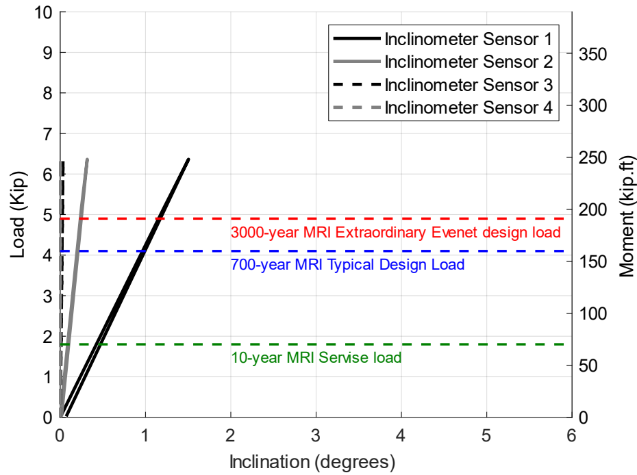
Figure C.1 The results of the first static test performed in the SE direction on Pole 16-concrete showing the inclination vs load and moment
