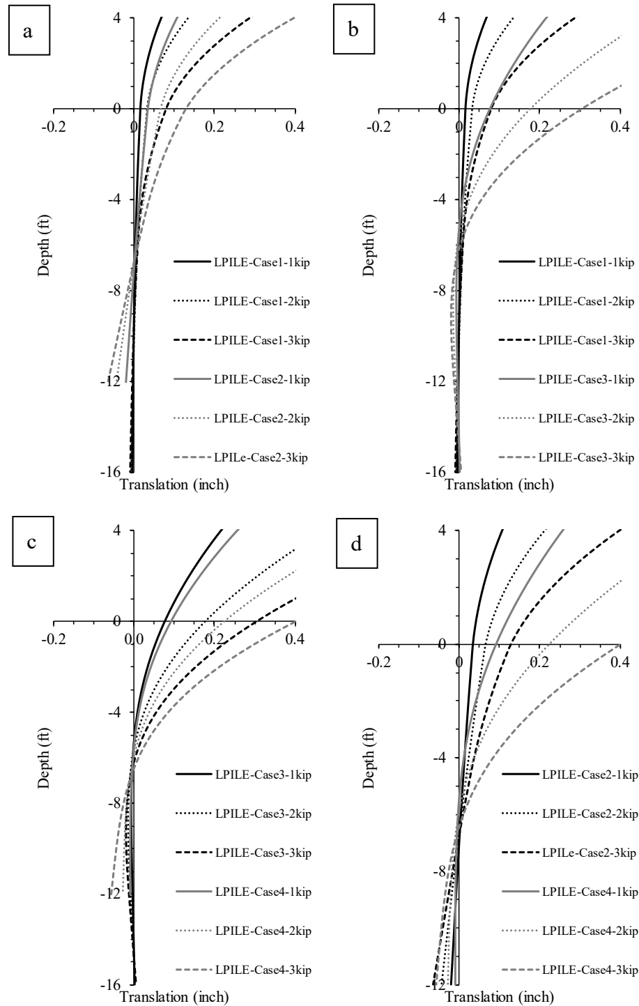
Figure 7.5 Comparison between translation profiles obtained from LPILE for cases with different backfill and embedment depths at various loads (a) cases with concrete backfill and different embedment depths, (b) cases with different backfill and 16-ft embedment depths, (c) cases with gravel backfill and different embedment depths, and (d) cases with different backfill and 12-ft embedment depths
