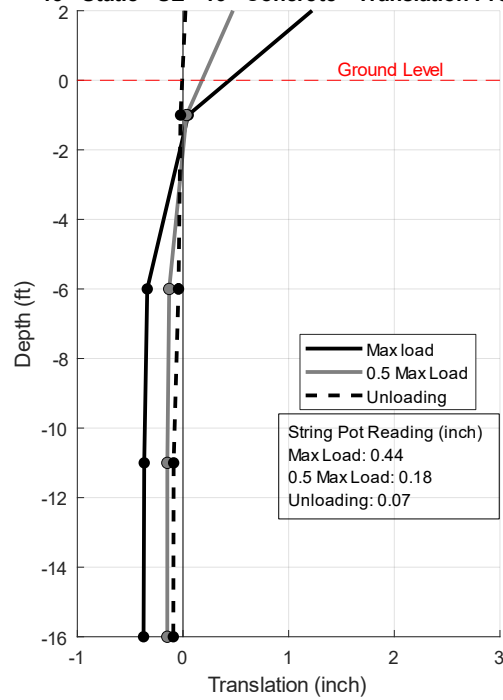
Figure 6.6 Translation vs depth of static tests on SE direction performed on pole 16 – Concrete, the 700-yr design load is approximately 0.5 of the maximum load
