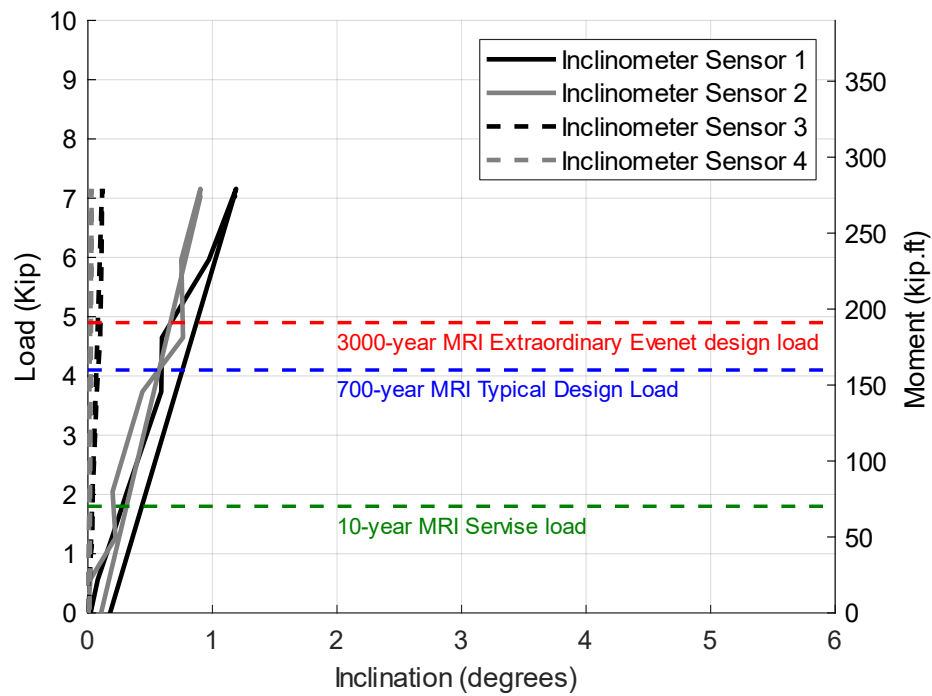
Figure C.9 The results of the third static test performed in the SW direction on Pole 16-Gravel showing the inclination vs load and moment
