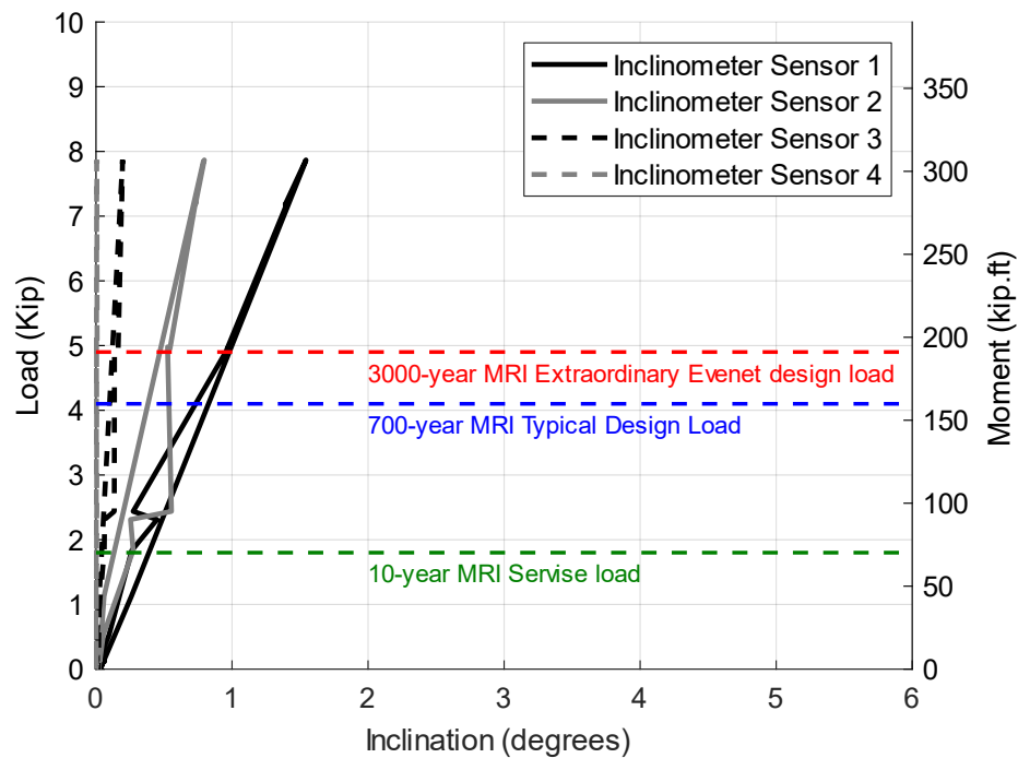
Figure C.6 The results of the third static test performed in the NE direction on Pole 16-Gravel showing the inclination vs load and moment
