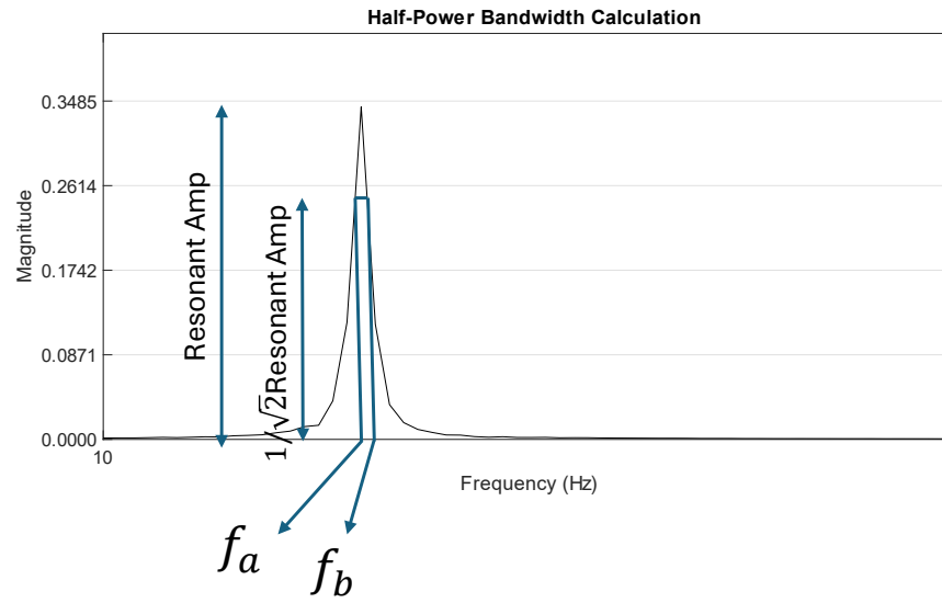
Figure 5.12 Illustration of half-power bandwidth method to calculate the damping ratio
