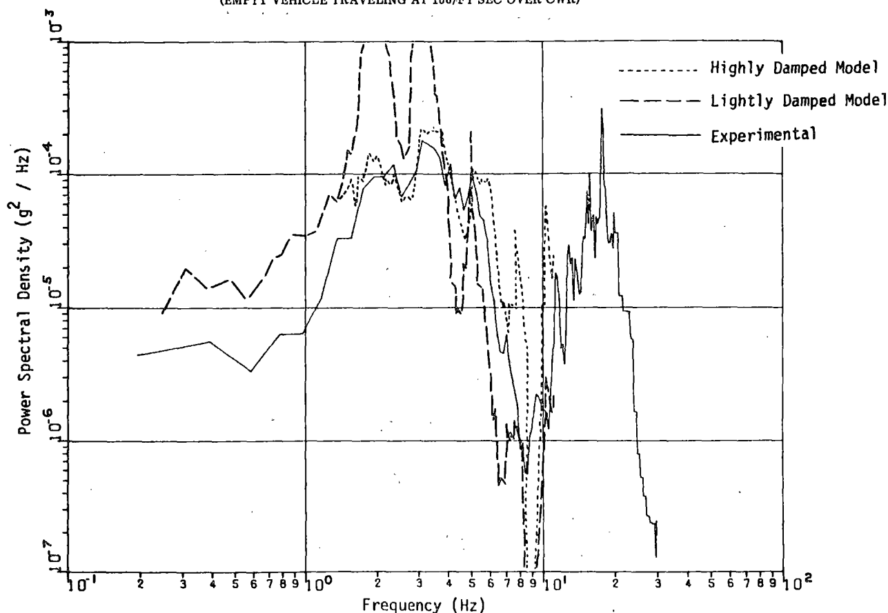
FIGURE 3-24. POWER SPECTRAL DENSITIES OF CARBODY FRONT END VERTICAL ACCELERATION (LOADED VEHICLE TRAVELING AT 100 FT/SEC OVER CWR)
