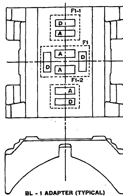
FIGURE 2-3. FORCE TRANSDUCER-BEARING ADAPTER
