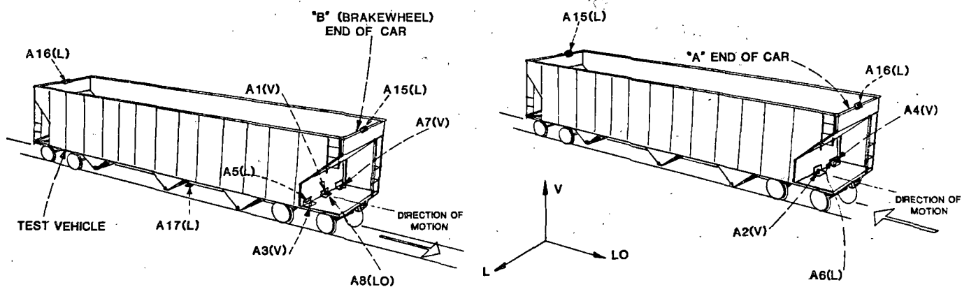
FIGURE 2-9. CARBODY INSTRUMENTATION
