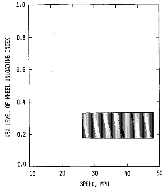
FIGURE 4-11. WU_{95} LEVELS FOR TYPE II TRUCKS WITH LOADED OPEN HOPPER CARS - 2.5 DEGREES CURVED ENTRY/EXIT
