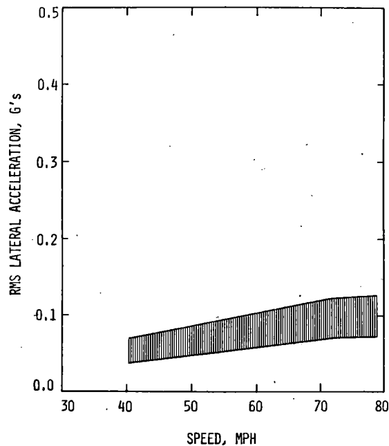
FIGURE 4-41. RMS LATERAL ACCELERATION LEVELS (0-20 HZ) FOR TYPE II FREIGHT CAR TRUCKS WITH LOADED OPEN HOPPER CARS
