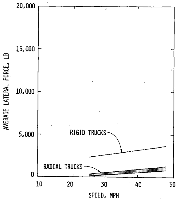
FIGURE 4-20. LATERAL FORCE ON LEADING OUTER WHEEL FOR TYPE II FREIGHT CAR TRUCKS WITH EMPTY OPEN HOPPER CARS - 3.7 DEGREE CURVES
