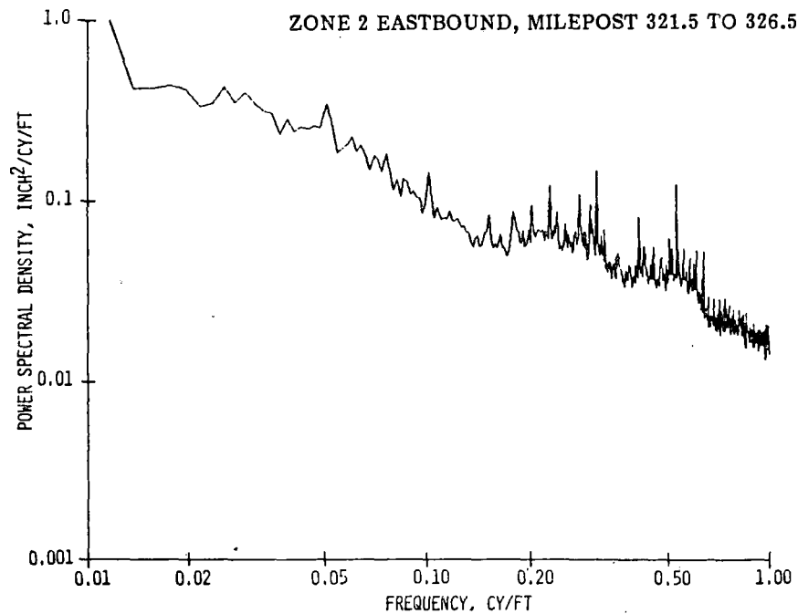
FIGURE 2-20. POWER SPECTRAL DENSITY - ZONE 2, GAUGE
