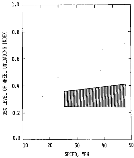
FIGURE 4-10. WU_{95} LEVELS FOR TYPE II TRUCKS WITH EMPTY OPEN HOPPER CARS - 2.5 DEGREES CURVED ENTRY/EXIT
