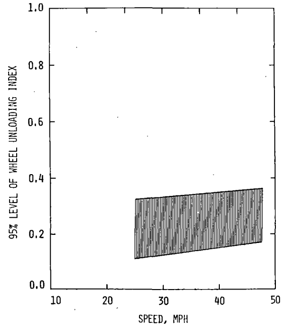
FIGURE 4-13. WU_{95} LEVELS FOR TYPE II TRUCKS WITH LOADED OPEN HOPPER CARS - 3.7 DEGREES CURVES ENTRY/EXIT
