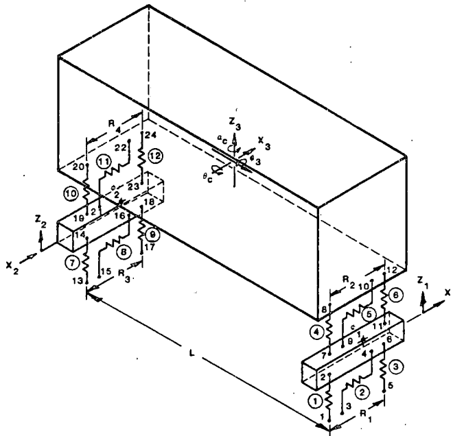
FIGURE 3-13. FRATE 11 MODEL
