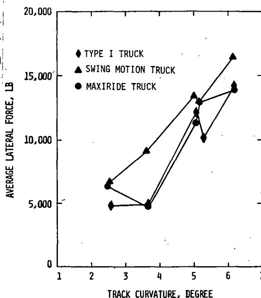
FIGURE 5-18. AVERAGE LATERAL FORCE VS CURVATURE FOR LEFT HAND CURVES FOR LOADED NON-STEERING TRUCKS
