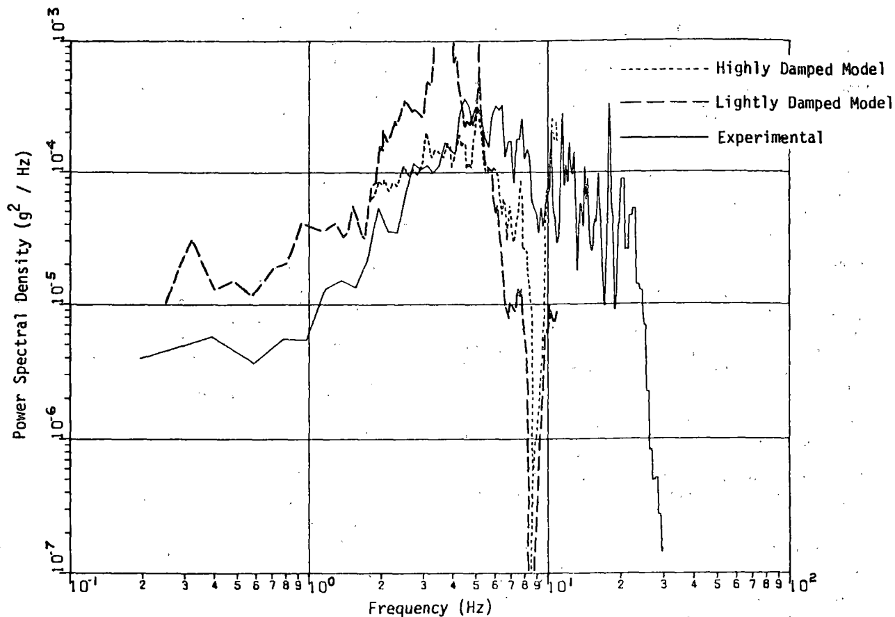
FIGURE 3-23. POWER SPECTRAL DENSITIES OF CARBODY FRONT END VERTICAL ACCELERATION (EMPTY VEHICLE TRAVELING AT 100/FT SEC OVER CWR)
