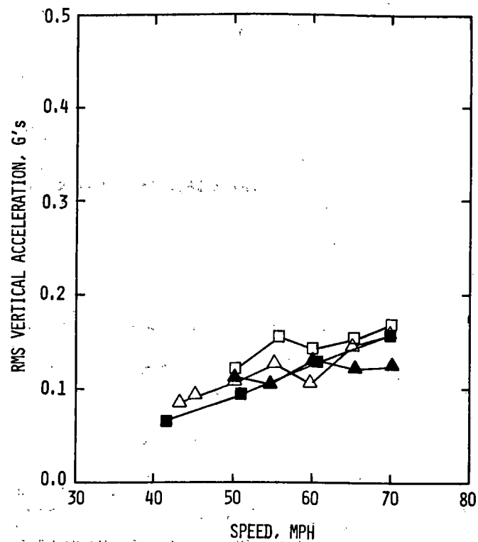
FIGURE 5-20. RMS VERTICAL ACCELERATION VS SPEED - 0-20 HZ FREQUENCY BAND/LOADED CARS/SECONDARY SUSPENSION TRUCKS
