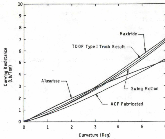
FIGURE 5-7. NON-STEERING TRUCK CURVING RESISTANCE VS CURVATURE
