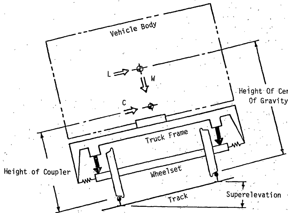
FIGURE 3-16. VEHICLE BODY/TRUCK/TRACK INTERFACES
