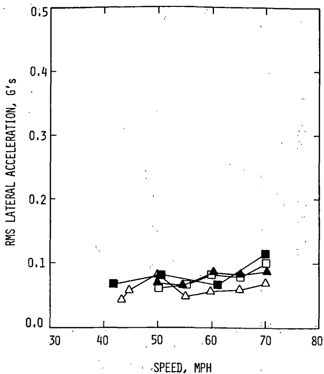
FIGURE 5-23. RMS LATERAL ACCELERATION VS SPEED - 0-20 HZ FREQUENCY BAND/LOADED CARS/ SECONDARY SUSPENSION TRUCKS
