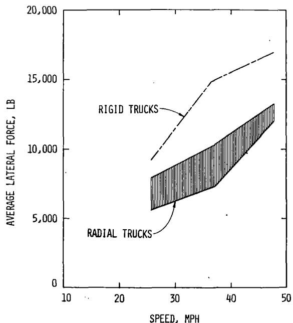
FIGURE 4-25. LATERAL FORCE ON LEADING OUTER WHEEL FOR TYPE II FREIGHT CAR TRUCKS WITH LOADED OPEN HOPPER CARS - 6.2 DEGREE CURVES
