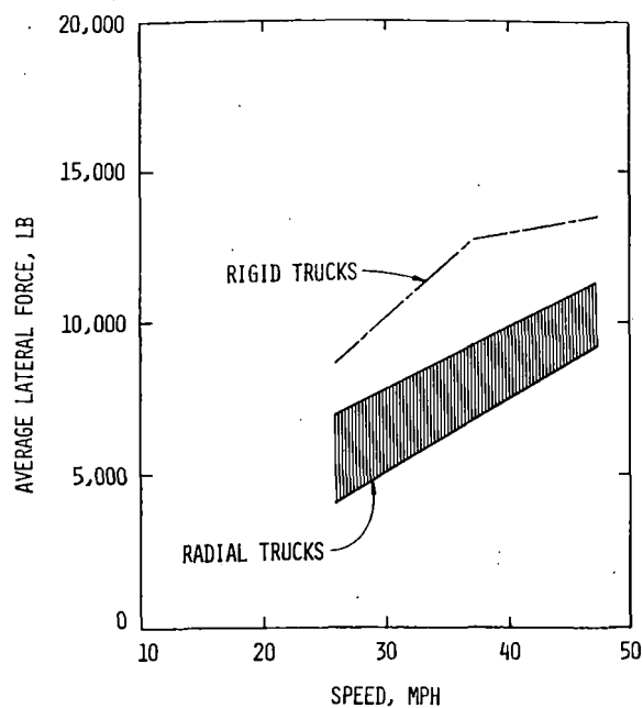
FIGURE 4-23. LATERAL FORCE ON LEADING OUTER WHEEL FOR TYPE II FREIGHT CAR TRUCKS WITH LOADED OPEN HOPPER CARS - 5.2 DEGREE CURVES
