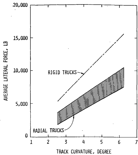
FIGURE 4-27. LATERAL FORCE ON LEADING OUTER WHEEL FOR TYPE II FREIGHT CAR TRUCK WITH LOADED OPEN HOPPER CARS AT BALANCE SPEED ( \pm 2.5 MPH)
