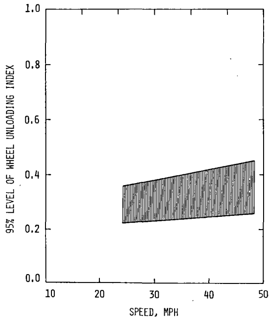
FIGURE 4-12. WU_{95} LEVELS FOR TYPE II TRUCKS WITH EMPTY OPEN HOPPER CARS - 3.7 DEGREES CURVES ENTRY/EXIT
