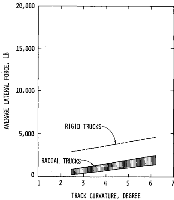
FIGURE 4-26. LATERAL FORCE ON LEADING OUTER WHEEL FOR TYPE II FREIGHT CAR TRUCK WITH EMPTY OPEN HOPPER CARS AT BALANCE SPEED ( \pm 2.5 MPH)
