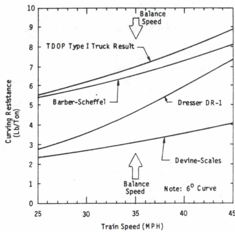
FIGURE 5-8. STEERING TRUCK CURVING RESISTANCE VS TRAIN SPEED
