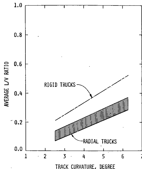
FIGURE 4-37. L/V RATIO ON LEADING OUTER WHEEL FOR TYPE II FREIGHT CAR TRUCKS WITH LOADED OPEN HOPPER CARS AT BALANCE SPEED (+ 2.5 MPH)
