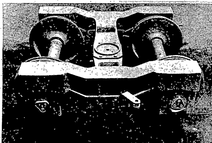
FIGURE 2-35. DEVINE-SCALES TRUCK
