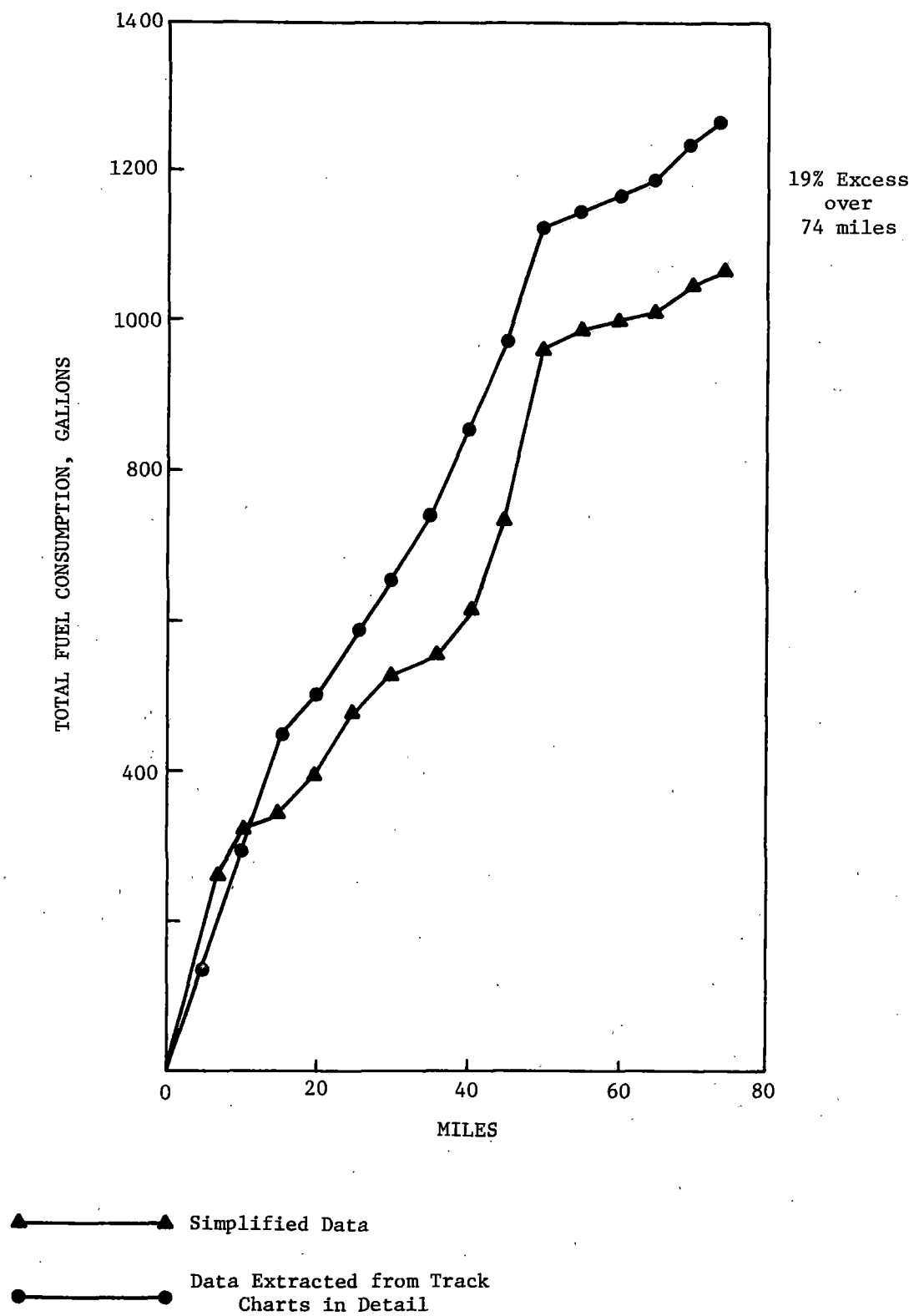
FIGURE 2 TOTAL FUEL CONSUMPTION FOR SAME TRACK, USING DIFFERENT COMPLEXITY OF DATA
