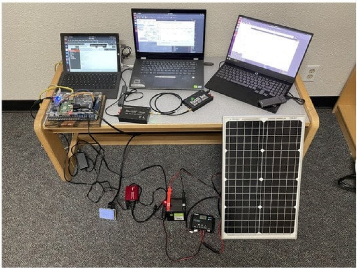
Figure 3. System Layout
