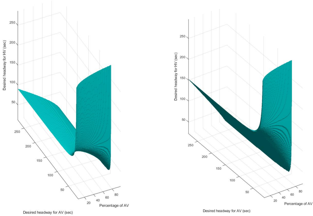
Figure 4 The stability region of maximal acceleration under different penetration rate of AV. reaction time 0.5 sec (left) and 1.0 sec (right) (fixing comfortable deceleration for vehicles as 2 m/s^2 ; maximal acceleration for vehicles as 1.4 m/s^2 )
