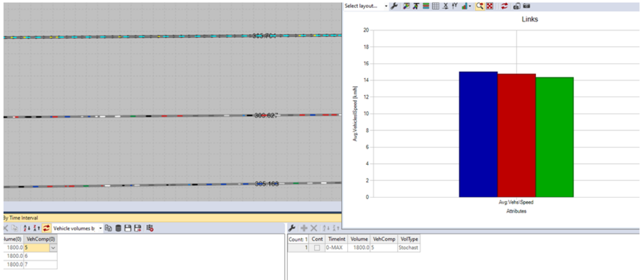
Figure 5 VISSIM simulation and average speed using proposed method compared to fixed AV headway and IDM car following model.
