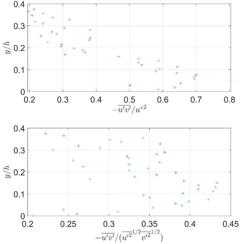
Figure 4.30 Measured Reynolds stress profile at location 1; u^* = 0.0396 m/s (from log law), h = 20.9 mm
