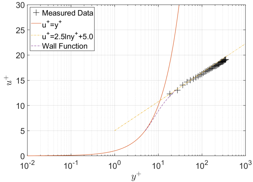
Figure 4.17 Mean velocity profile at location 5 in semi log plot; u^* = 0.0365 m/s, \tau_b = 1.33 N/m 2
