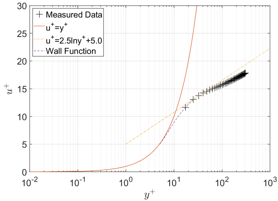
Figure 4.6 Mean velocity profile at location 4 in semi log plot; u^* = 0.0331 m/s, \tau_b = 1.092 N/m 2
