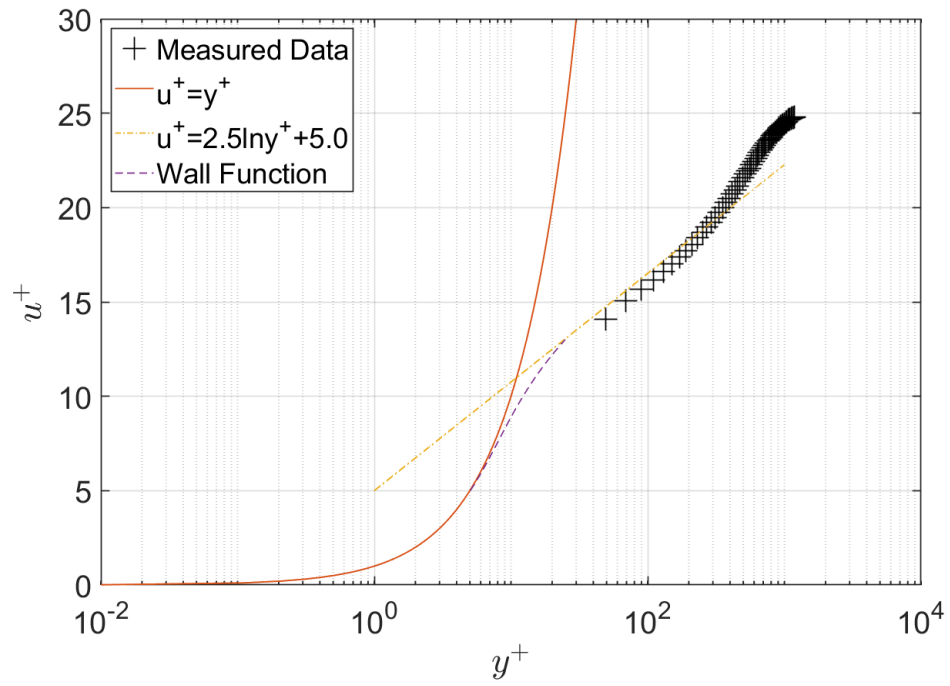
Figure 4.38 Mean velocity profile at location 2 in semi log plot; u^* = 0.0369 m/s, \tau_b = 1.36 N/m 2
