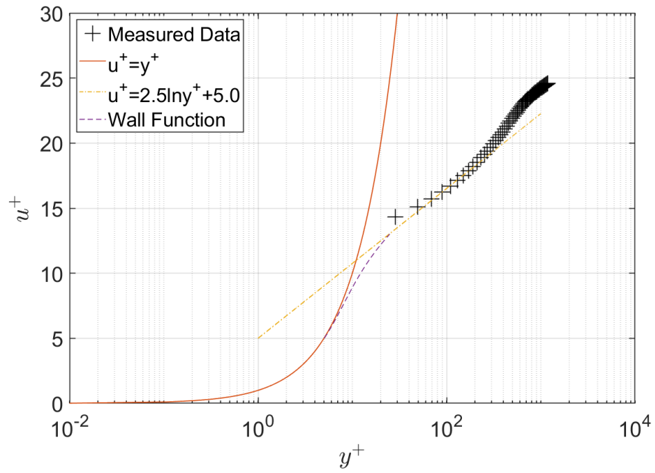
Figure 4.37 Mean velocity profile at location 1 in semi log plot; u^* = 0.0369 m/s, \tau_b = 1.36 N/m 2
