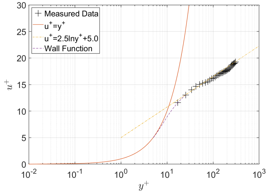
Figure 4.16 Mean velocity profile at location 4 in semi log plot; u^* = 0.0343 m/s, \tau_b = 1.17 N/m 2
