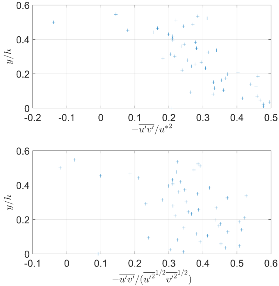
Figure 4.34 Measured Reynolds stress profile at location 5; u^* = 0.0414 m/s (from log law), h = 16.8 mm
