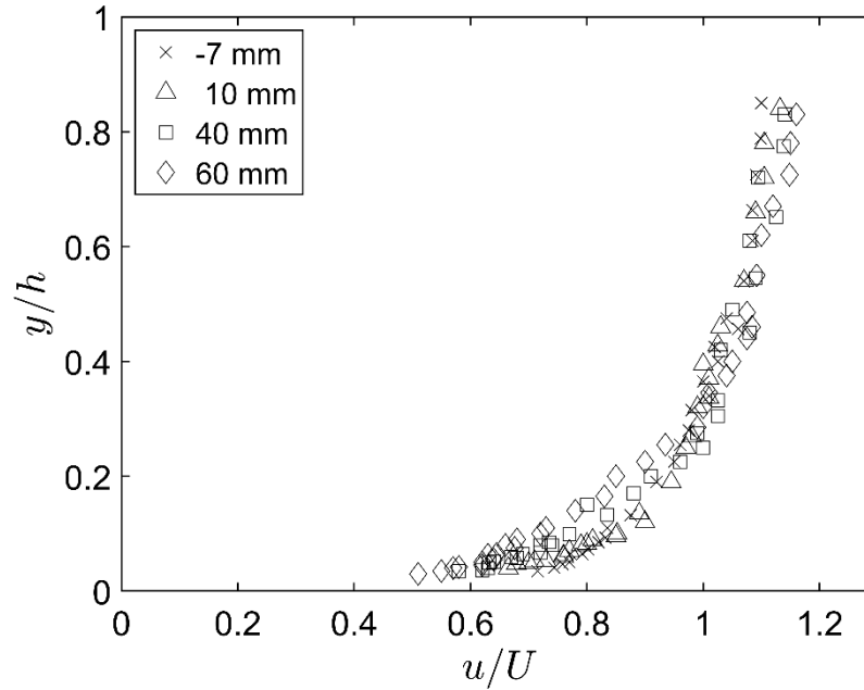
Figure A1 Horizontal mean velocity profiles at different locations in case C of Chen and Chiew (2003)
