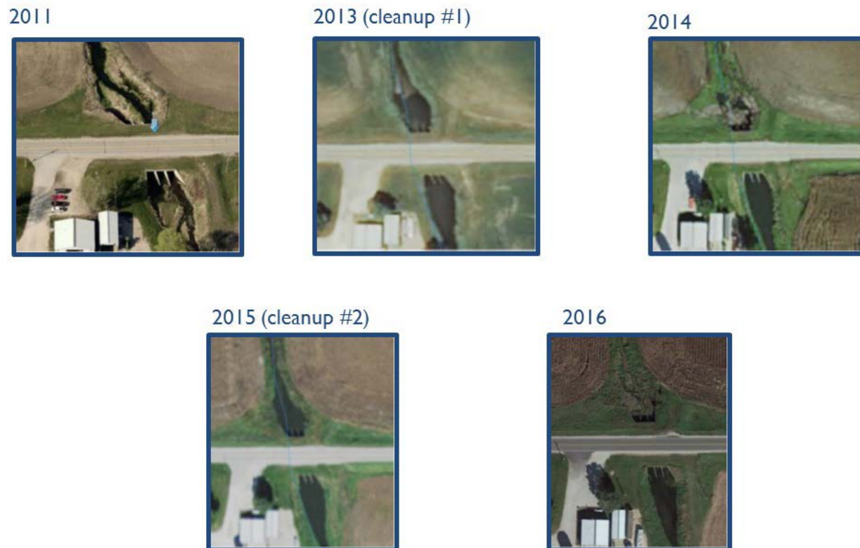
Figure 5. Sedimentation is fast and can quickly reduce a culvert's conveyance capacity.
