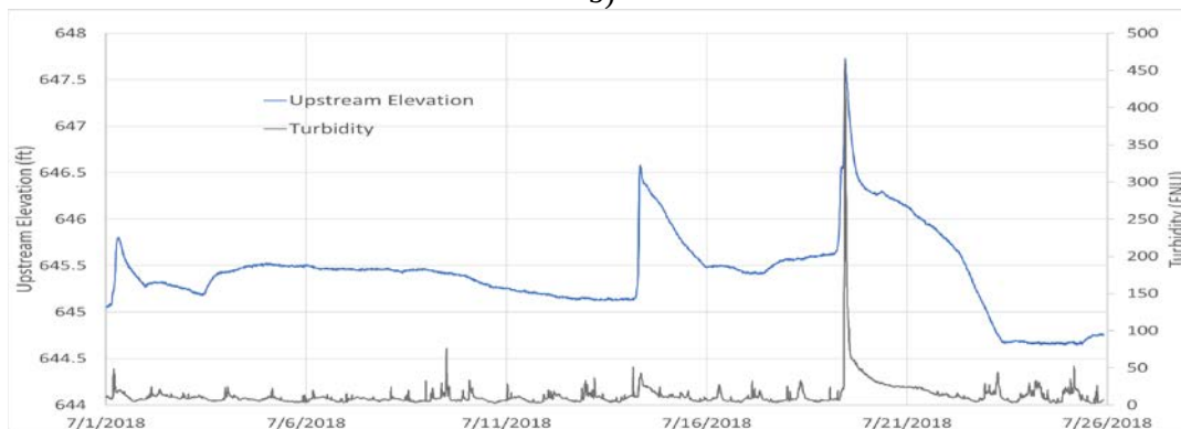
Figure 21. Recordings of water stages and turbidity at the retrofitted culvert for FHWA #364790 site: a) upstream stage and free-surface slope, b) stage and turbidity recording at the inlet of the culvert
