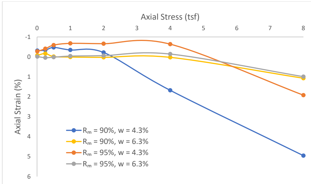
Figure B.45: One-dimensional Double Consolidometer Test Results for A-1-a (SC-SM) Soil
