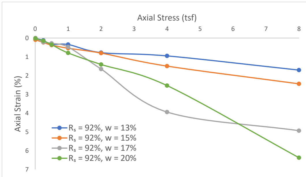
Figure 4.13 Comparison of Loading-induced Stress-strain Characteristics for A-2 (SC) PI >> 11 Soil at a Constant Relative Compaction R_s = 92\%
