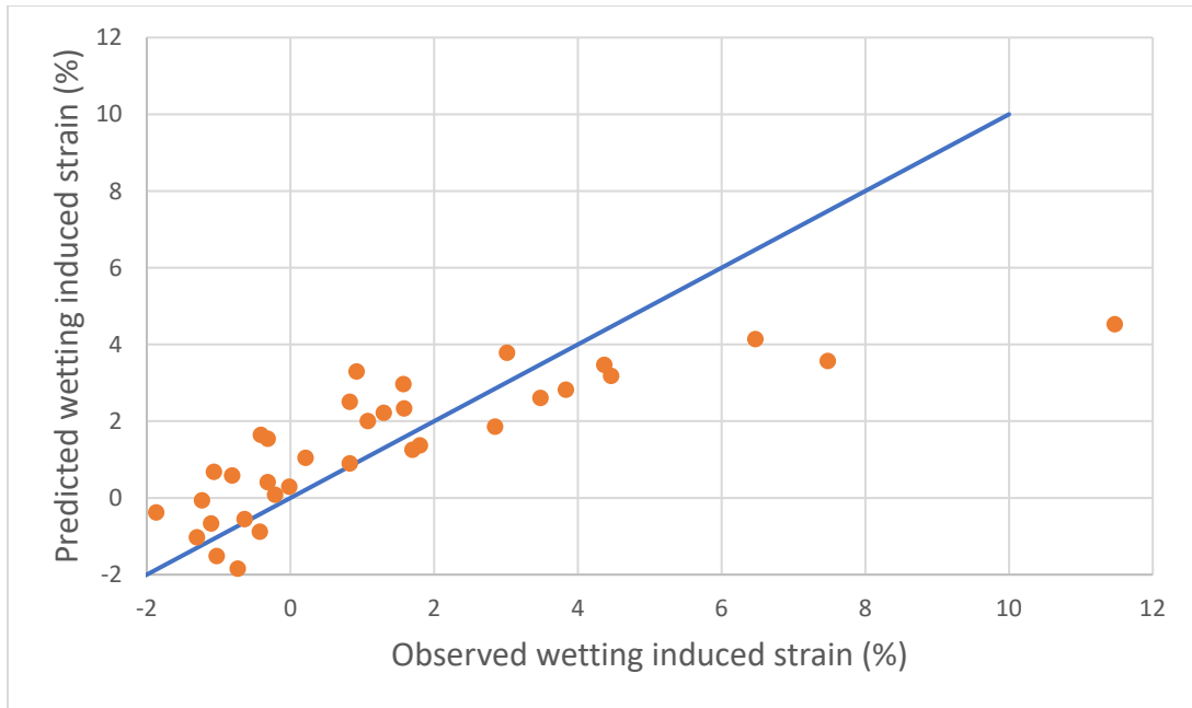
Figure C.15: Predicted vs. Observed Wetting-induced Strain for A-2 (SC) With PI > 11 Soil Using Equation 4.2
