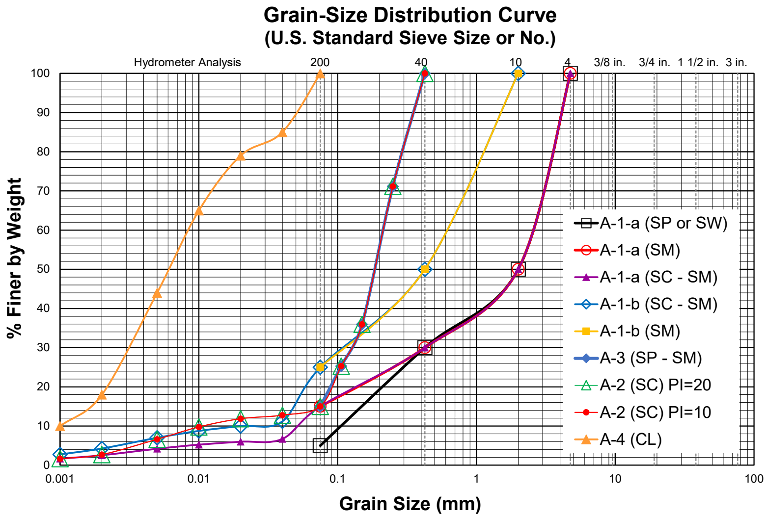
Figure 3.3 Grain Size Distribution of the Test Materials for the Standard Consolidometer Tests
