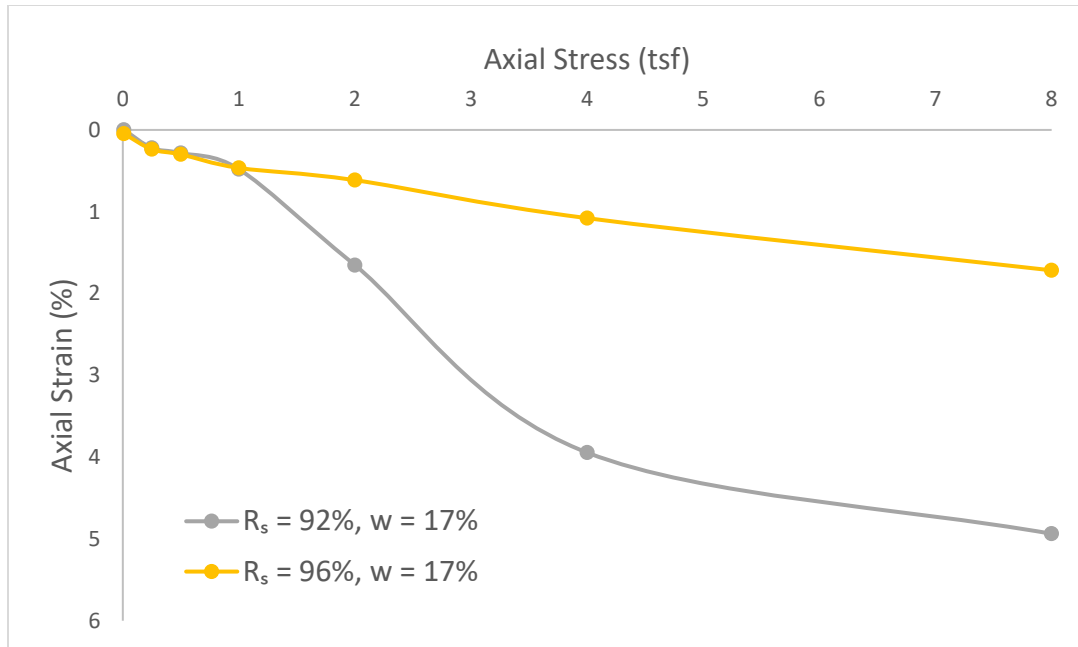
Figure 4.17 Comparison of Loading-induced Stress-Strain Characteristics for A-2 (SC) PI>>11 Soil at a Constant As-compacted Moisture Content w = 17\%
