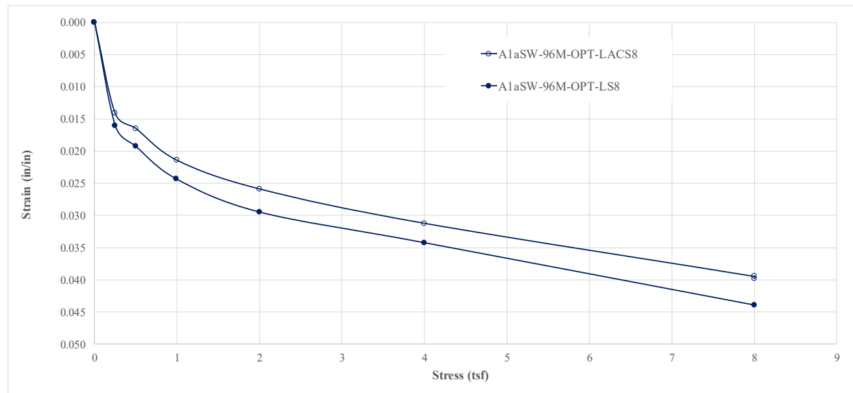
Figure 5.24 Effect of Moisture Condition during Loading on Strain vs. Stress Results for Specimens of A1aSW Compacted to 96% Relative Compaction at Optimum Water Content
