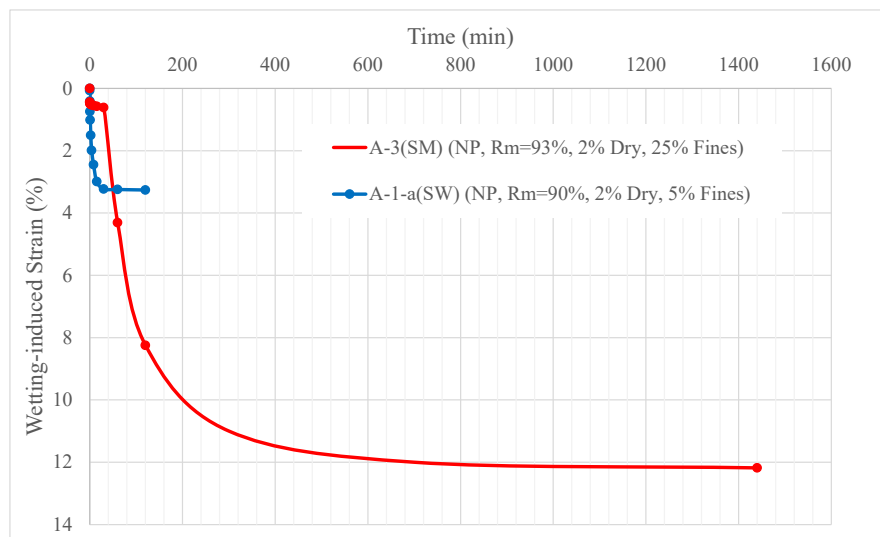
Figure 6.10 Comparison of Wetting-induced Strain vs. Time for an A-1-a(SW) Specimen Compacted to 90% Relative Compaction and an A-3(SM) Specimen Compacted to 93% Relative Compaction. Both Specimens were Compacted 2% Dry of Optimum and Wetted at a Stress of 8 tsf.
