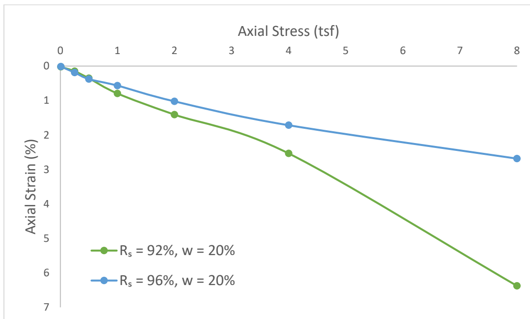
Figure 4.18 Comparison of Loading-induced Stress-strain Characteristics for A-2 (SC) PI>>11 Soil at a Constant As-compacted Moisture Content w = 20\%
