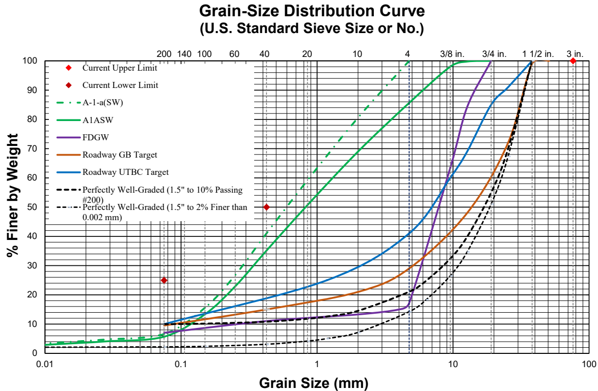
Figure 6.13 Comparison of Grain-size Distribution Curves for Five Nonplastic Granular Soils, Current Specifications for Bridge Approach Embankment, and Two Perfectly Well-graded Soils
