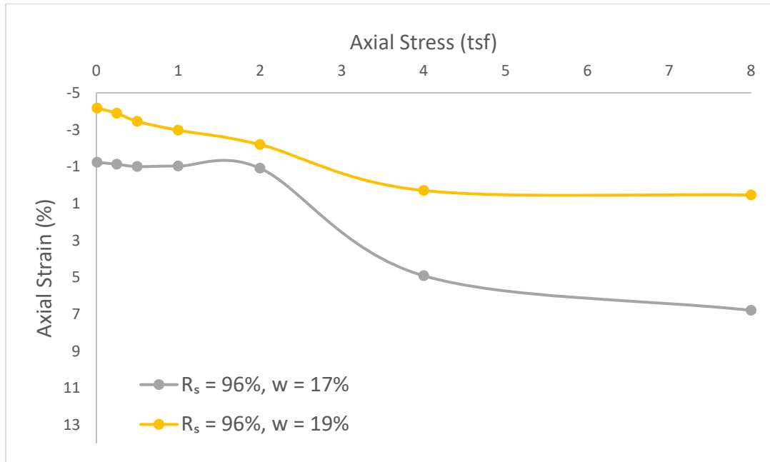
Figure B.49: One-dimensional Double Consolidometer Test Results for A-2 (SC) PI \gg 11 Soil
