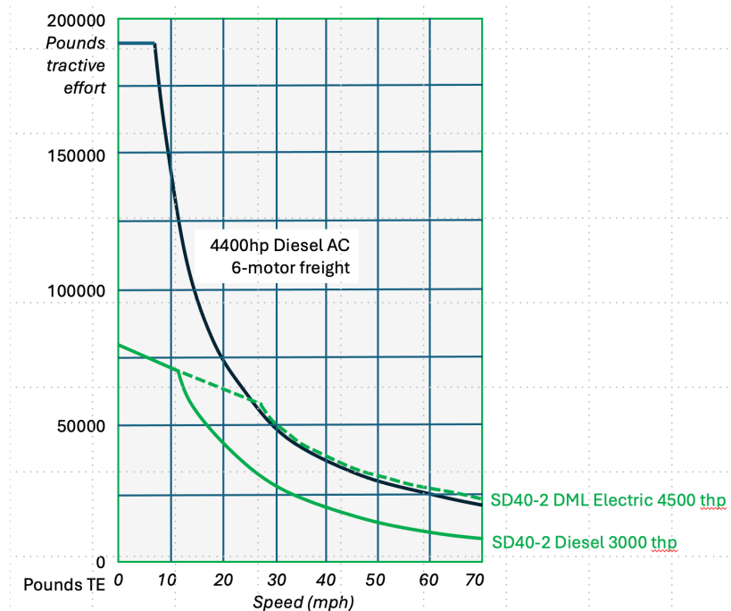
Figure 27. Comparison of the Estimated Performance of the SD40-2 DML with a Modern 4,400 hp Diesel-electric Locomotive with AC Traction Motors
