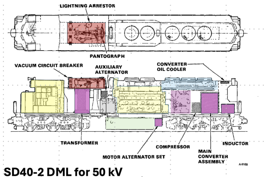
Figure 25. Equipment Layout for the 50 kV SD40-2 DML
