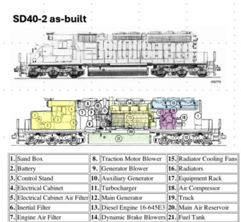
Figure 26. Components of the SD40-2 As-built
