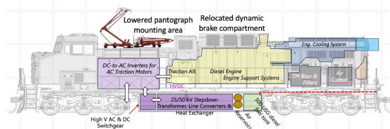
Figure 38. Alternate Configuration for a DML with DFT Repositioning the Dynamic Brake Compartment to Allow Room for Pantographs without Increasing Locomotive Height
