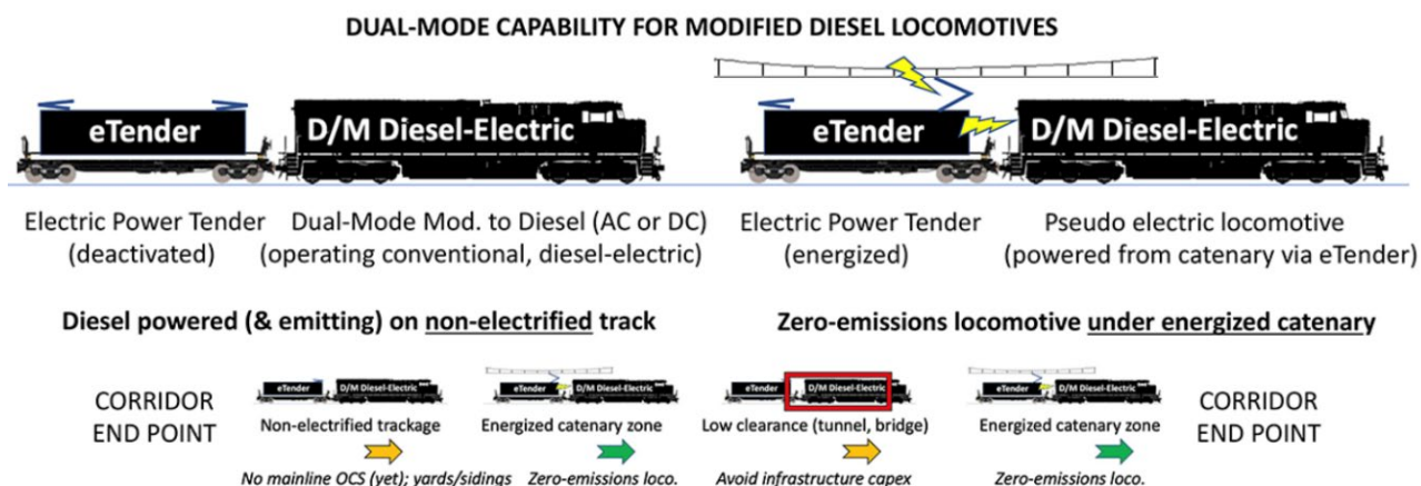
Figure 40. Relationship of the DML with EPT (i.e., eTender) to Electrification Schemes with Partial OCS
