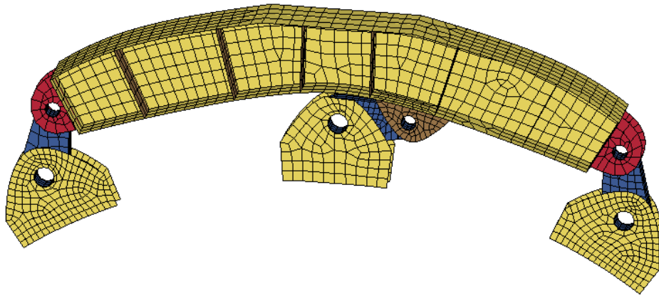
Figure 63. Forward Mount
