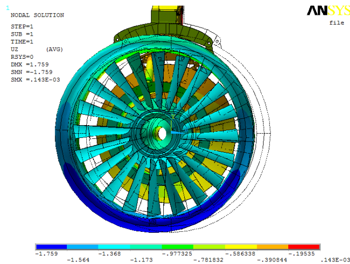
Figure 35. Lateral Displacement of the FBO Full-Fan Rig Model Under Lateral 1000-lb Loading on A-Flange
