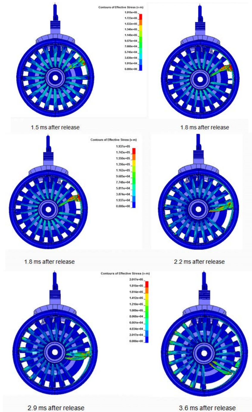
Figure 101. Phases of the Fan Blade–Case Interaction
