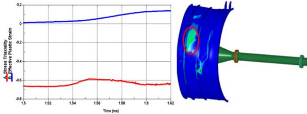
Figure 78. Stress Triaxiality of the Most Stressed Element on the Footprint of Initial Impact (outer surface of the containment case)
