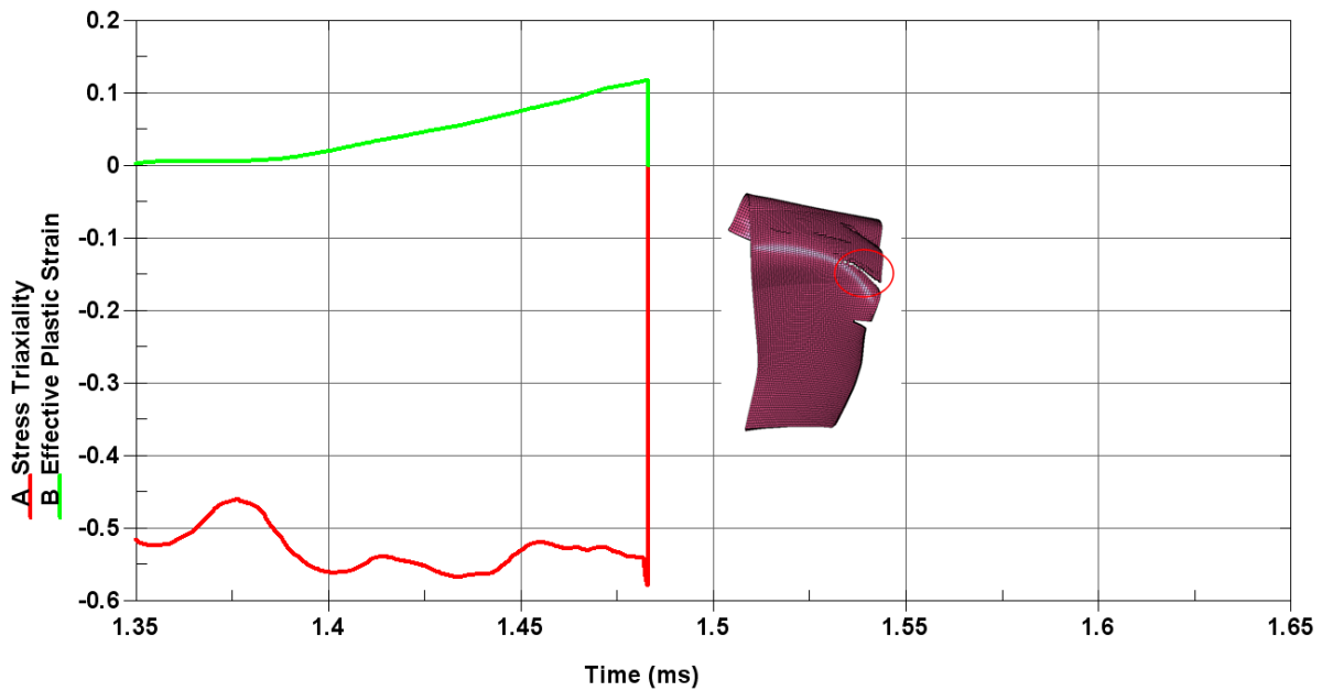
Figure 92. Stress Triaxiality at the Blade Breakup Zone
