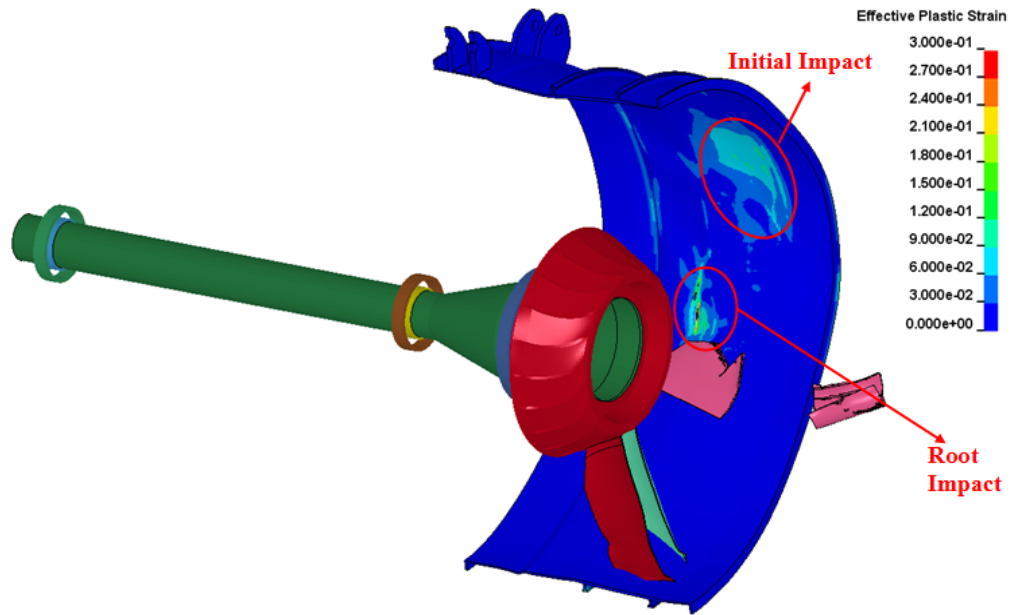
Figure 76. Main Damage Zones of the Containment Case
