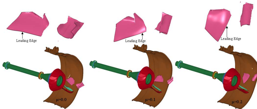
Figure 96. Effect of Friction Coefficient on the Blade Breakup and Case Damage
