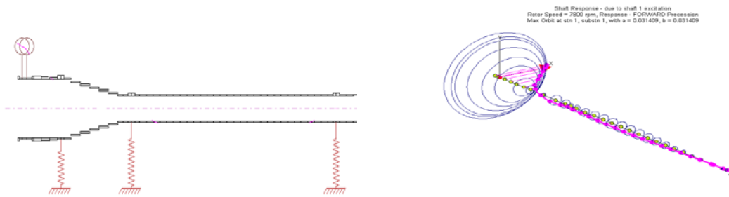
Figure 12. Imbalance Orbit of the DYROBES Beam Model
