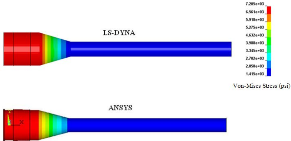
Figure 9. Rotor Shaft Prestress Field With LS-DYNA and ANSYS Implicit Solvers
