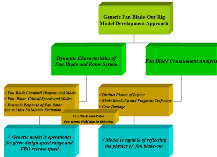
Figure 1. Model Development Approach
