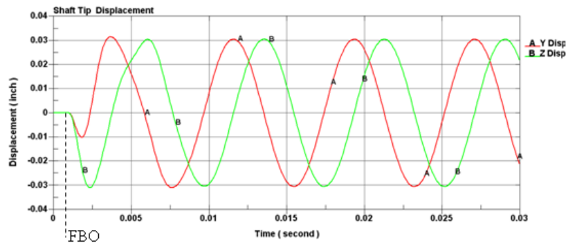
Figure 15. Shaft Centerline Displacement Due to Imbalanced Load
