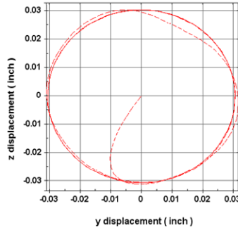
Figure 17. Disk Center Orbit Due to Imbalanced Load
