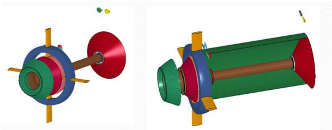
Figure 23. Fan Frame Struts, Core Case, Bearing Supports, and Fan Shaft Isometric View
