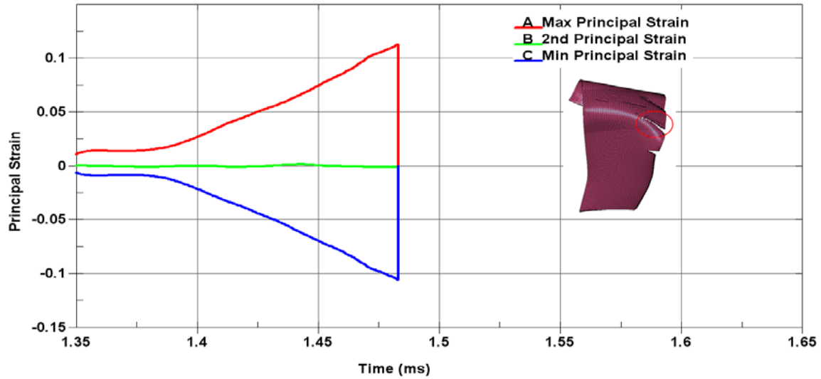
Figure 91. Principal Strains at the Blade Breakup Zone
