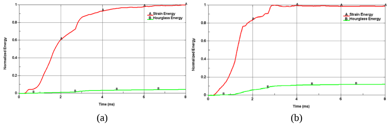
Figure 70. Normalized Hourglass Energies for the (a) Containment Case and the (b) Released Blade (normalized with respect to maximum strain energy)
