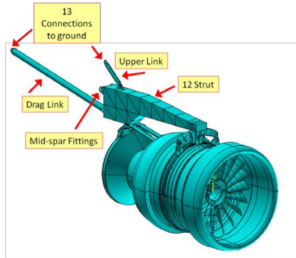
Figure 19. Ground Connections and Links of Rig Model
