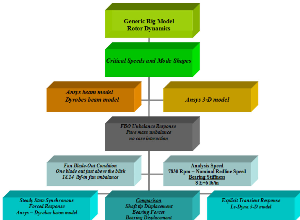
Figure 5. Model Checkout Stages Based on Generic Rig Model Rotor Dynamics
