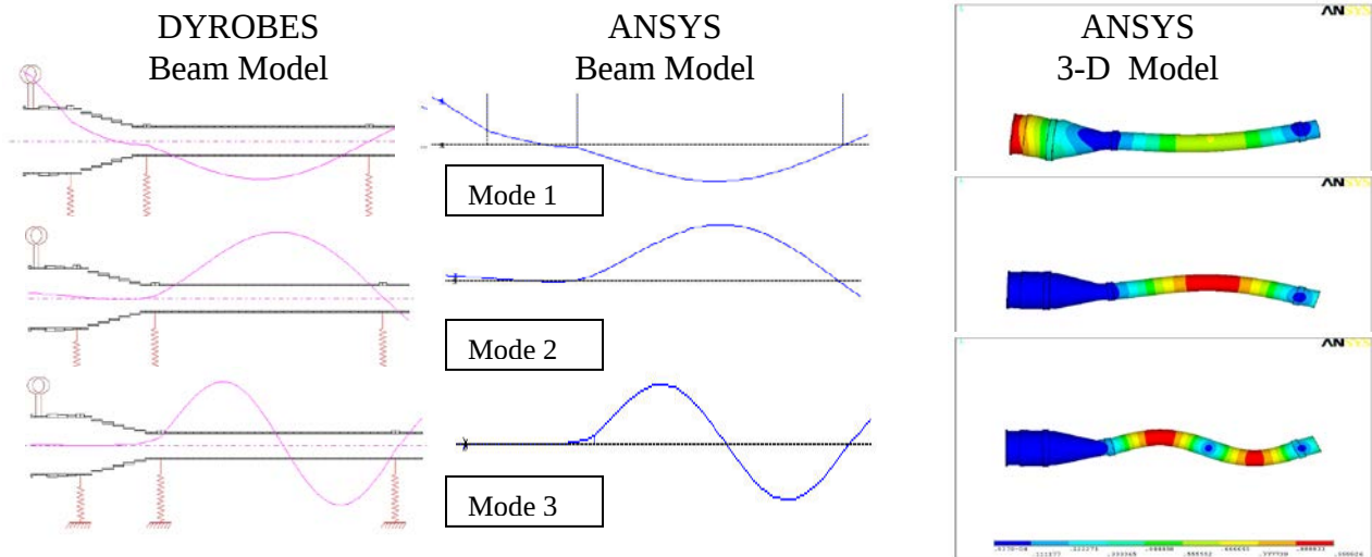
Figure 11. Critical Speed Mode Shapes of the Fan Shaft System
