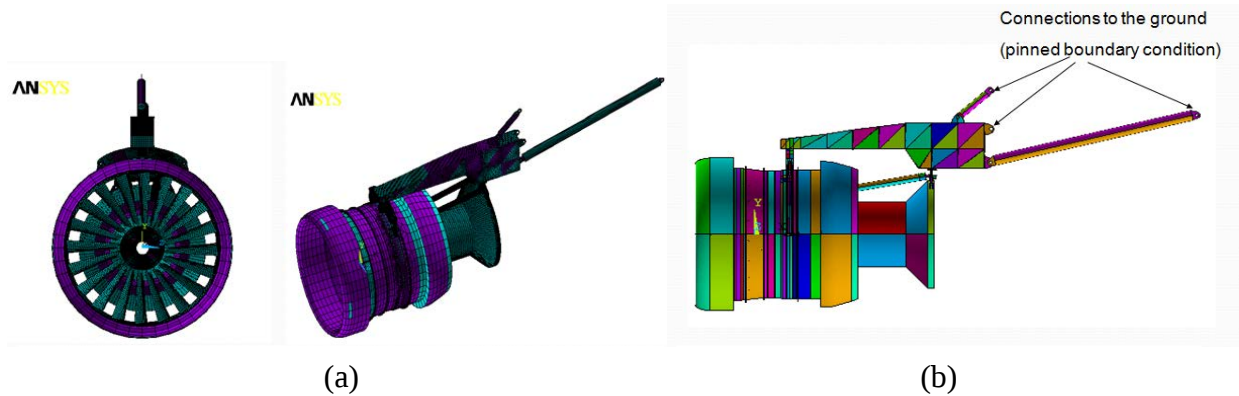
Figure 29. The (a) Mesh and (b) Boundary Conditions for the FBO Full-Fan Rig Model in ANSYS
