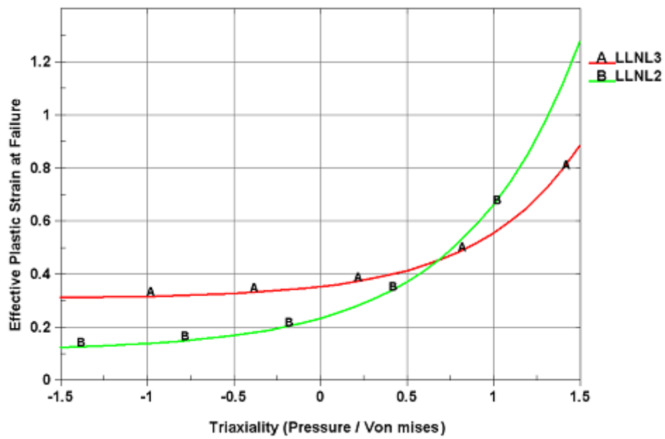
Figure 68. Difference in Fracture Locus of Al 2024-T3/T351 Nominal Strain Rate of 1/s
