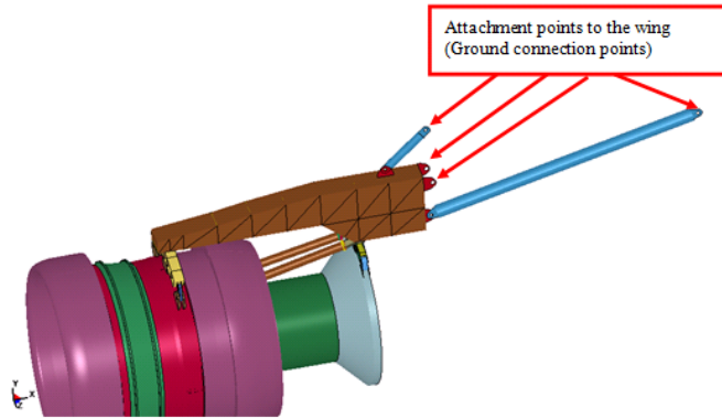
Figure 52. Ground Connection Points of the Rig Model (phase 2)
