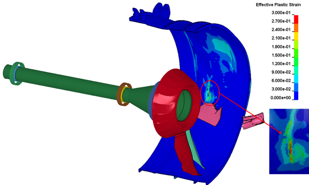
Figure 79. Damage of the Containment Case Inner Surface at the Footprint of the Root Impact
