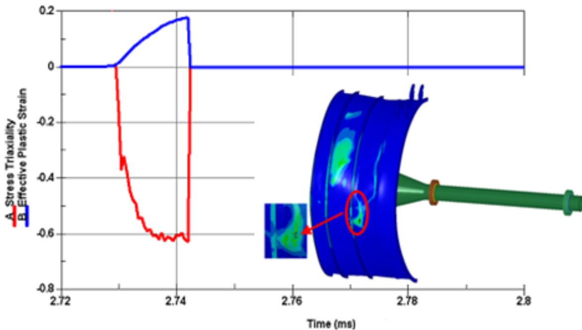
Figure 82. Stress Triaxiality of the Failed Element on the Outer Case Footprint of Initial Impact
