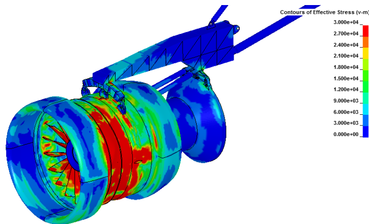
Figure 106. Stresses Scaled to Highlight Strut and Containment Case Damage at 3.5 ms
