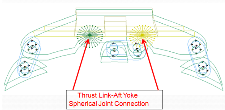
Figure 57. Connection Points of Aft Mount
