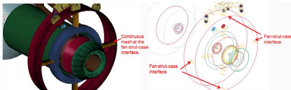
Figure 51. Fan Strut-Fan Case Interface (phase 2)
