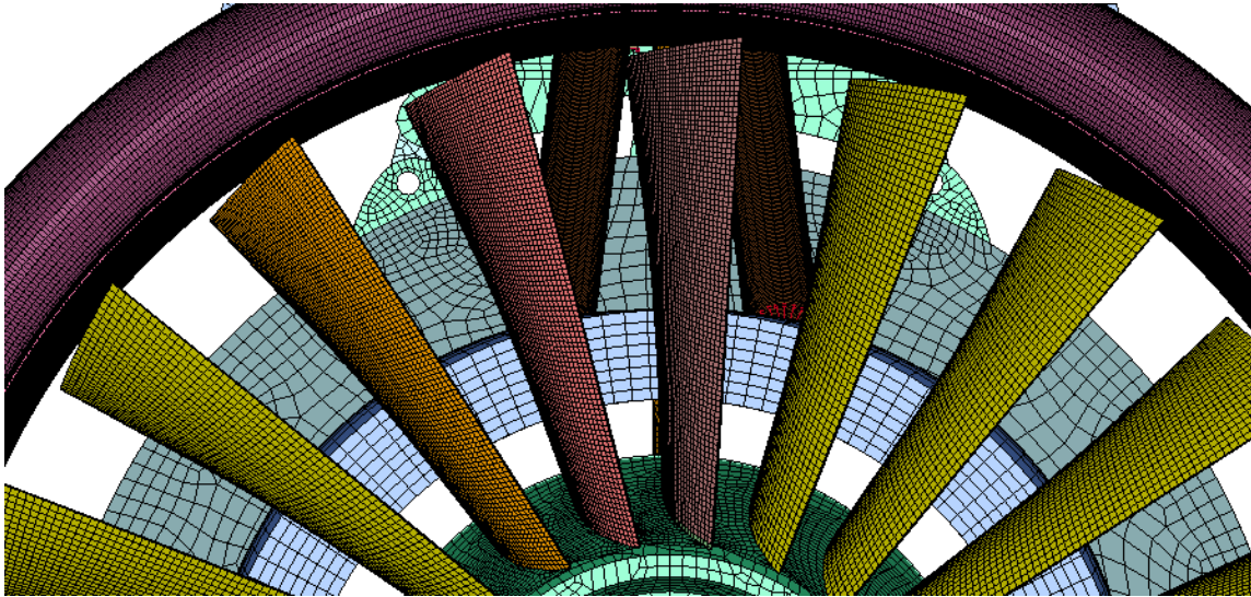
Figure 53. Mesh Details for the Fan Blades (brick elements)
