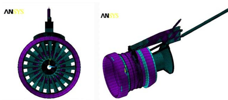
Figure 41. Mesh of the FBO Full-Fan Rig Model in ANSYS
