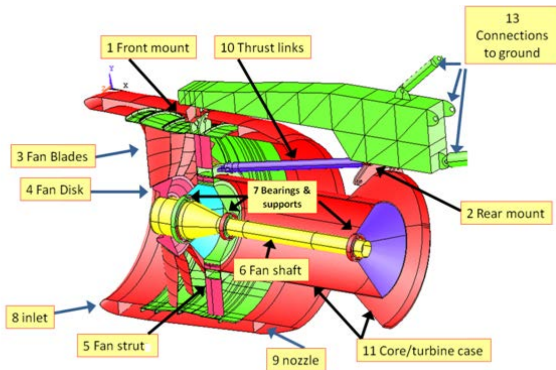
Figure 18. Components of Full-Fan Rig Model
