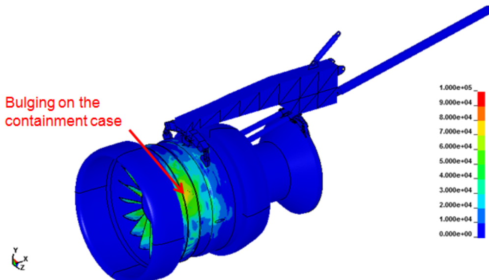
Figure 104. Containment Case Damage at 2.0 ms
