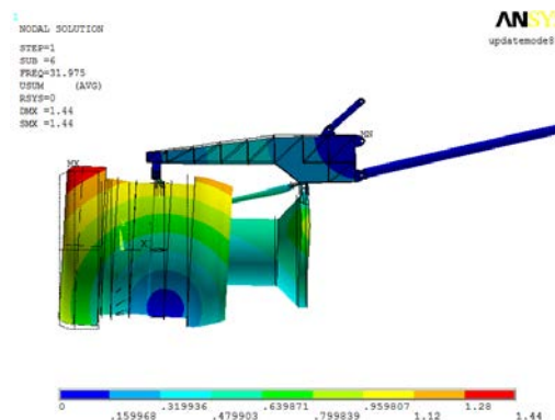
Figure 47. Mode 5—Fan Case Rocking With Core Case and Front Mount Flexure—32 Hz
