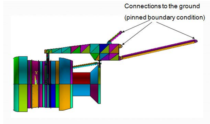
Figure 42. Modal Analysis Boundary Conditions
