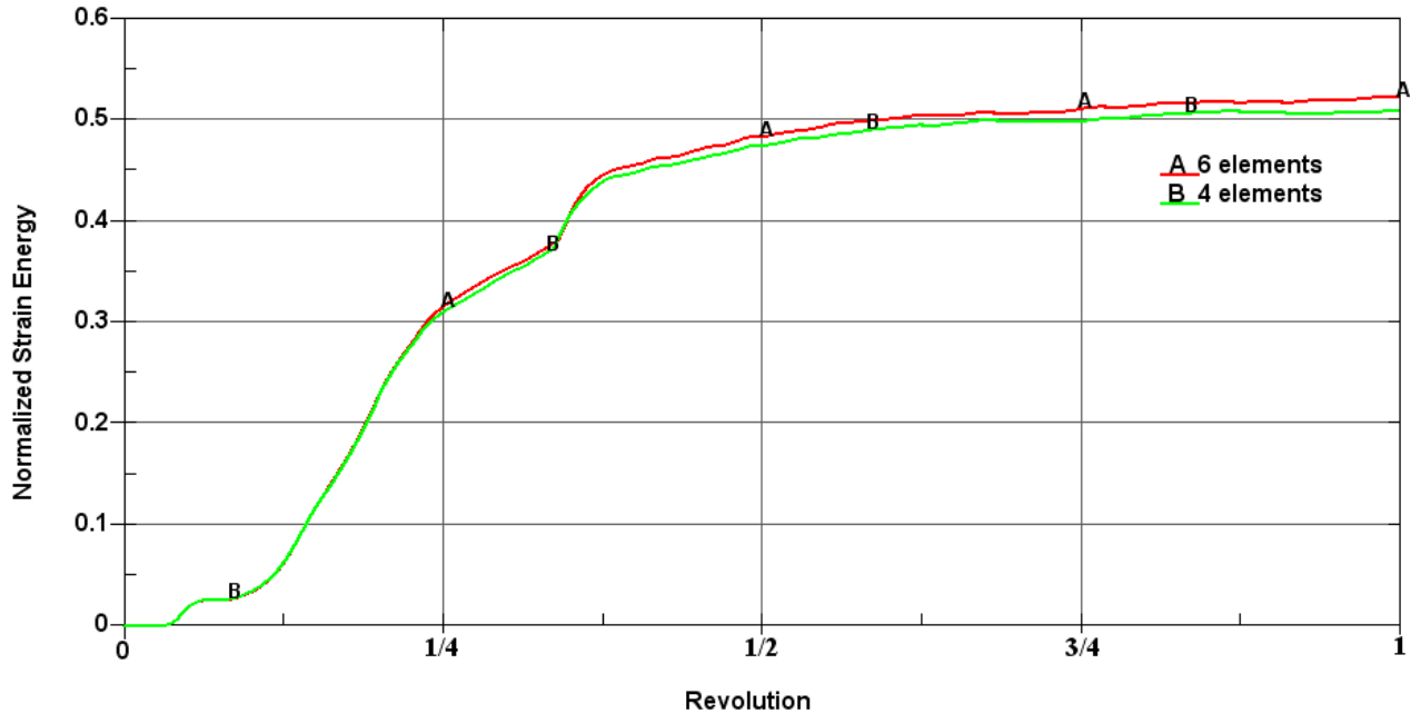
Figure 84. Effect of Through-the-Thickness Element Number on the Containment Case Normalized Strain Energy
