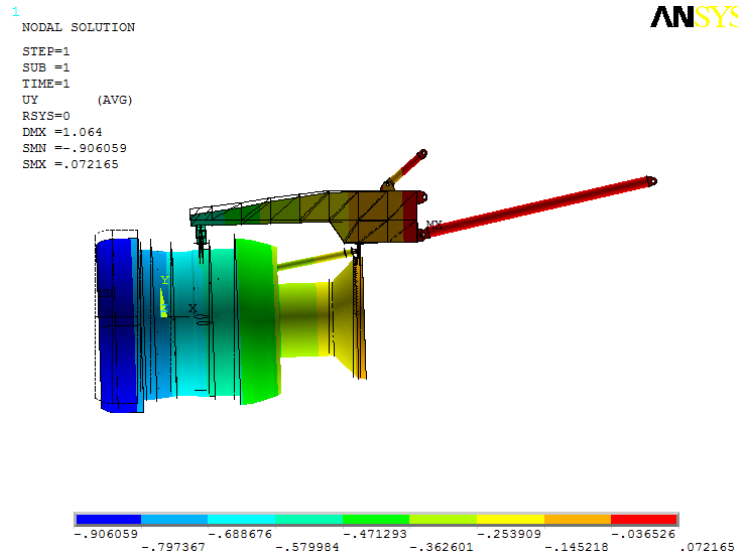
Figure 34. Vertical Displacement of the FBO Full-Fan Rig Model Under Vertical 1000-lb Loading on A-Flange
