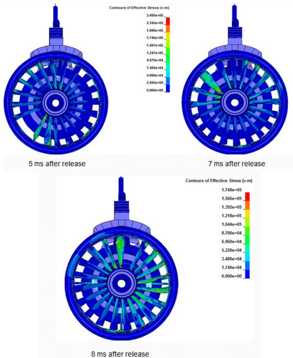
Figure 102. Phases of the Fan Blade-Case Interaction
