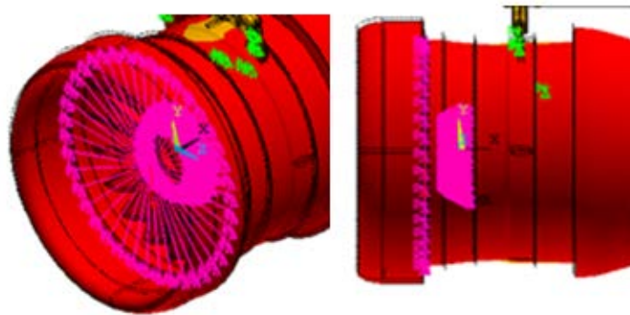
Figure 33. Details of Static Fan Disk Centerline Loading
