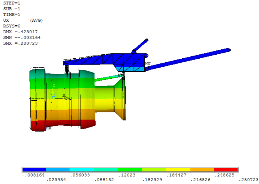
Figure 31. Longitudinal Displacement (inch) of the FBO Full-Fan Rig Model Under 1g Axial Loading
