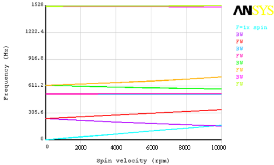
Figure 10. Fan Shaft System Campbell Diagram
