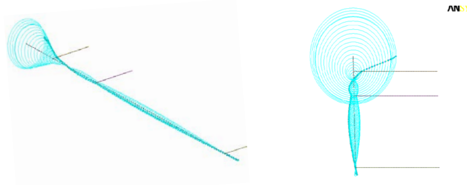
Figure 13. Imbalance Orbit of the ANSYS Rotordynamics Beam Model (isometric and plan view)
