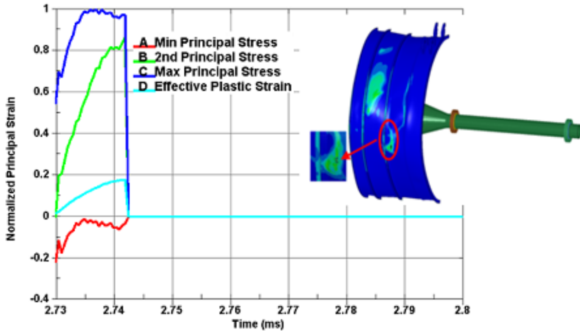
Figure 81. Normalized Principal Stresses of the Failed Element on the Footprint of Initial Impact (outer surface of the containment case)
