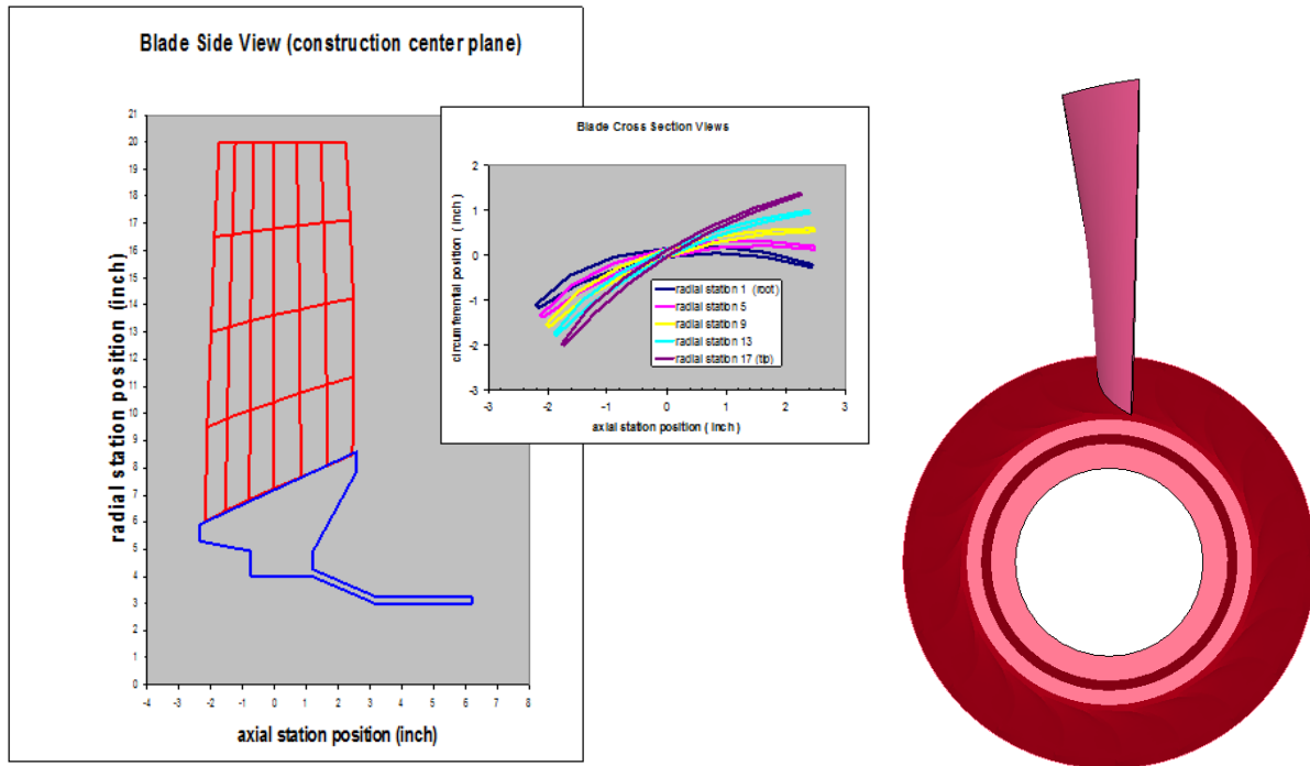
Figure 2. Generic Fan Blade Geometric Details
