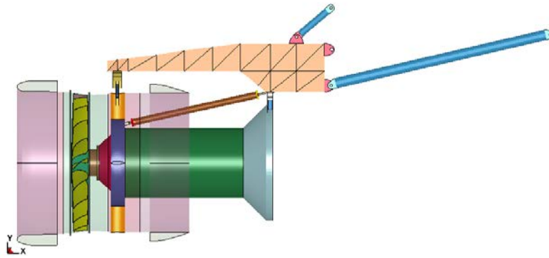
Figure 21. Side View, Full-Fan Rig Model With Inlet and Nozzle
