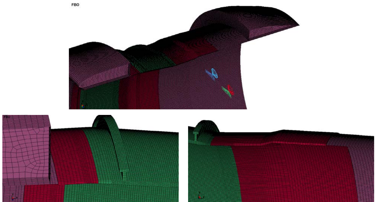
Figure 54. Mesh Details for the Fan Containment Case (brick elements)
