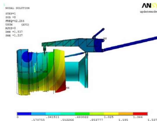
Figure 48. Mode 6—Fan Case Rocking With Strut—42 Hz
