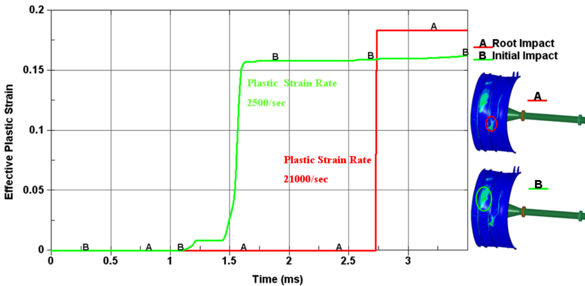
Figure 83. Comparison of the Effective Plastic Strains in the Fan Casing Impact Zones
