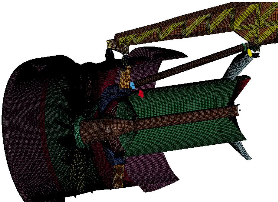
Figure 55. Half-Section Cut View of the Rig Model Mesh
