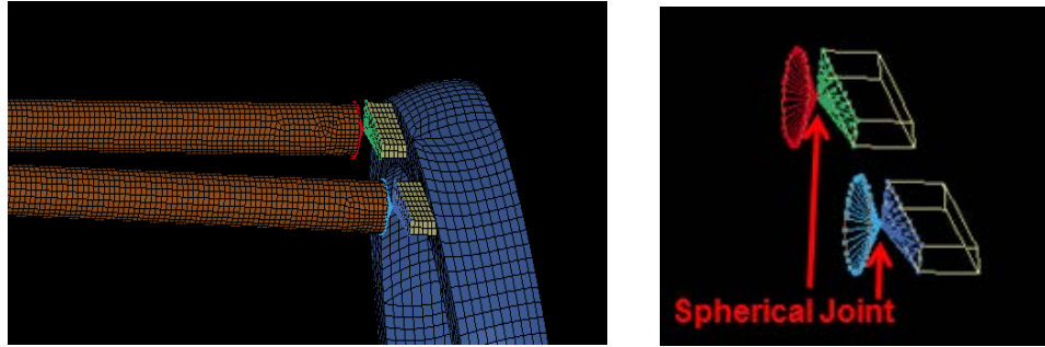
Figure 60. Thrust Link to Thrust Yoke Spherical Joint Details
