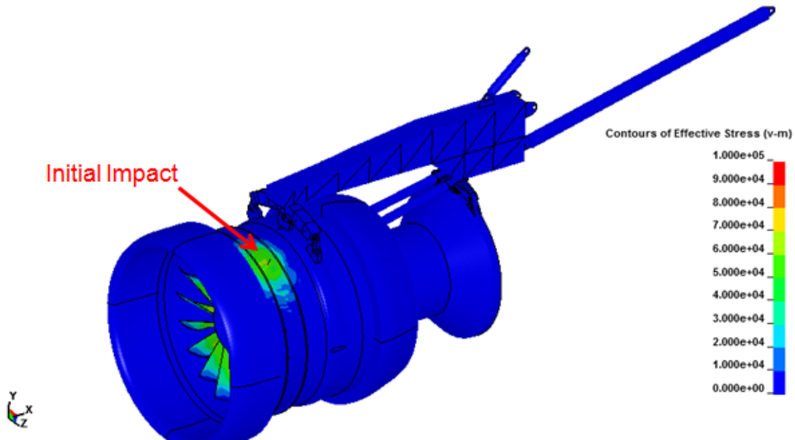
Figure 103. Containment Case Damage at 1.2 ms
