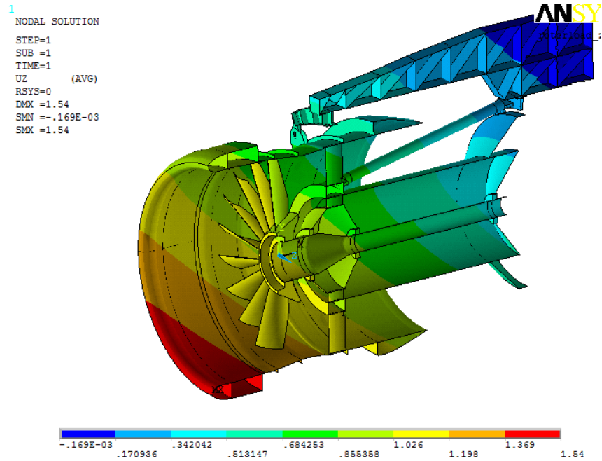
Figure 38. Lateral Displacement of the FBO Full-Fan Rig Model Under Lateral 1000-lb Loading on Fan Disk Centerline
