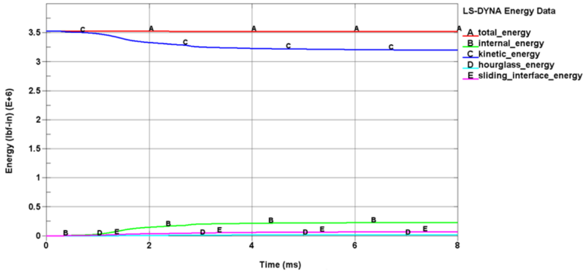
Figure 69. LS-DYNA Energy Data
