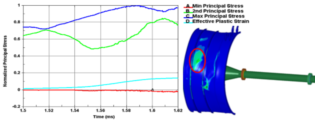
Figure 77. Normalized Principal Stresses of the Most Stressed Element on the Footprint of Initial Impact (outer surface of the containment case)
