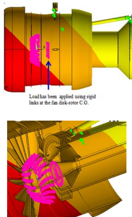
Figure 36. Details of Static Fan Disk Centerline Loading
