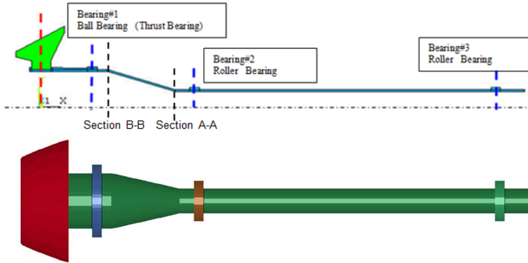
Figure 3. Generic Rotor and Bearing Configuration
