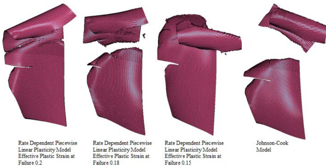
Figure 90. Effect of Material Model on the Blade Breakup
