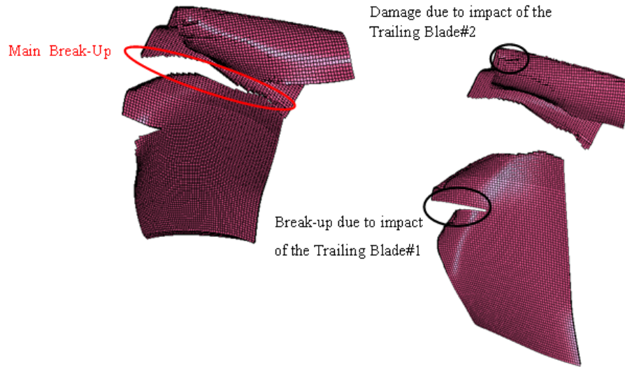
Figure 89. Details of the Released Blade Breakup Zones
