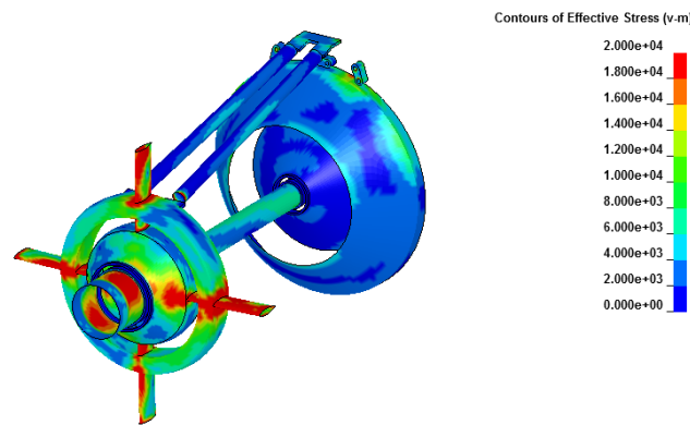
Figure 108. Fan Struts, Bearing Supports, and Fan Shaft Damage at 3.5 ms
