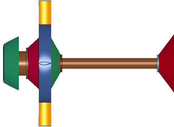
Figure 22. Fan Struts, Fan Strut Core Base, Bearing Supports, and Fan Shaft Side View
