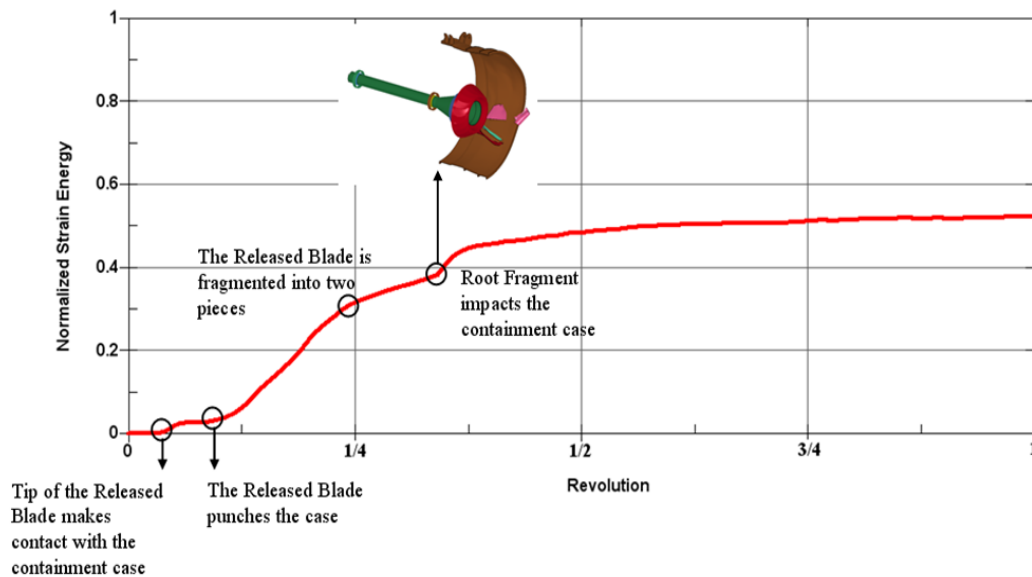
Figure 74. Normalized Strain Energy of the Containment Case (normalized with respect to initial kinetic energy of the released blade)
