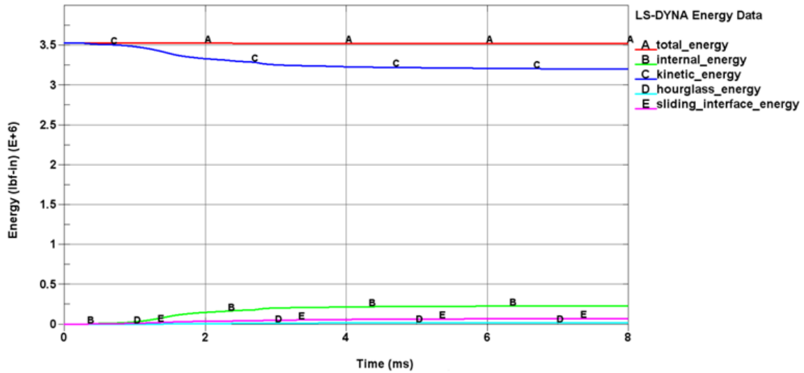
Figure 99. The LS-DYNA Energy Data
