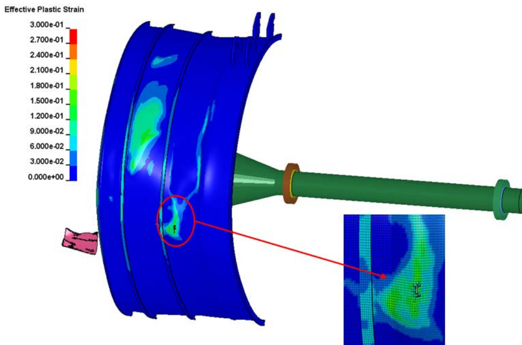
Figure 80. Damage of the Containment Case Outer Surface at the Footprint of the Root Impact
