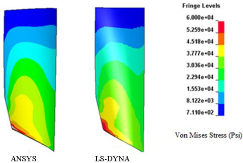
Figure 8. Fan Blade Prestress Field With ANSYS and LS-DYNA Implicit Solver
