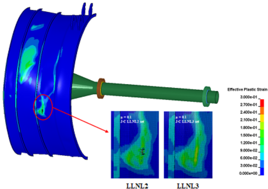
Figure 86. Effect of Johnson-Cook Damage Parameters on the Root Impact Footprint of the Fan Casing Outer Surface
