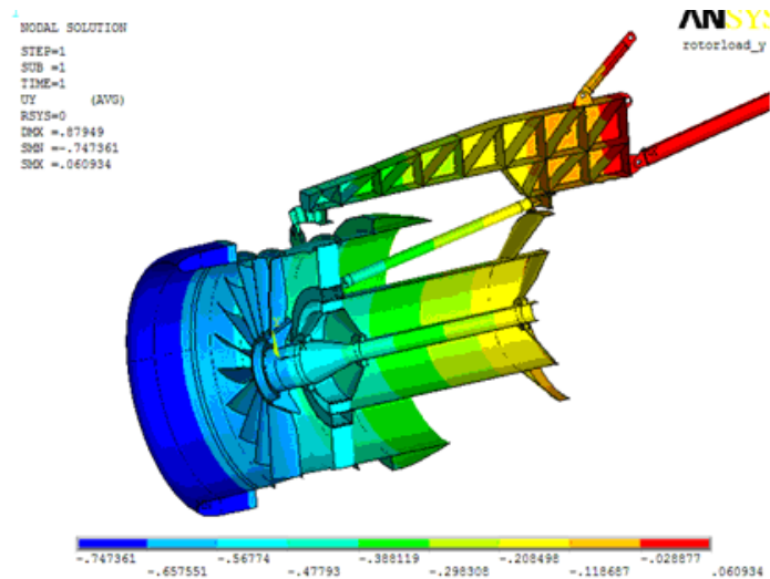
Figure 40. Vertical Displacement of the FBO Full-Fan Rig Model Under Vertical 1000-lb Loading on Fan Disk Centerline
