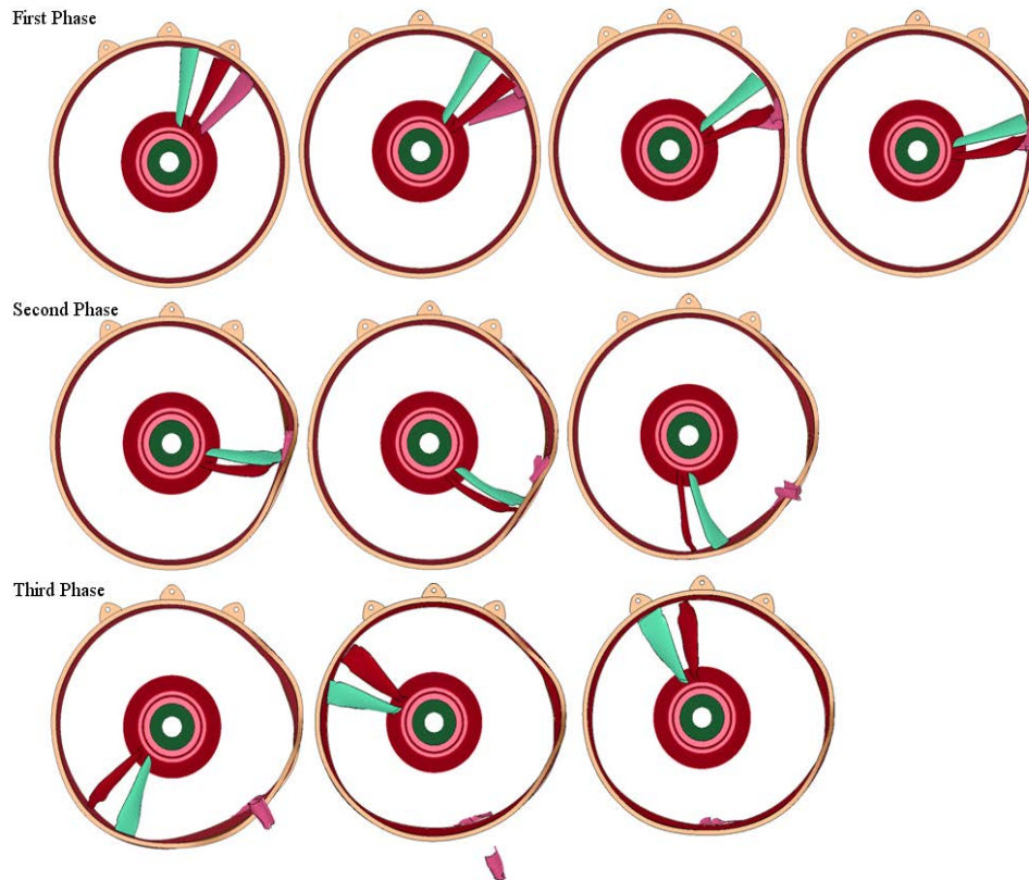
Figure 71. Distinct Phases of the Blade-Case Interaction (view is forward looking aft; fan rotation is clockwise)
