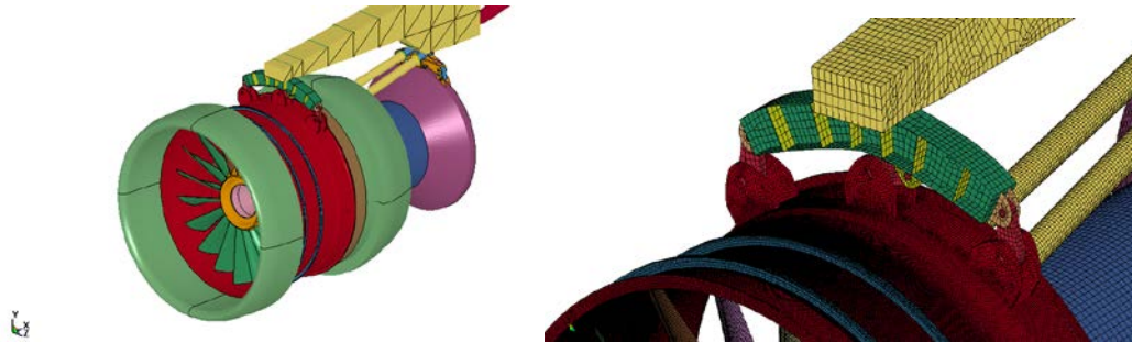
Figure 50. Fan Case Mounting Lugs—Front Mount Connection (phase 2)
