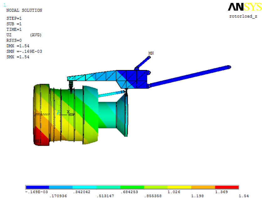
Figure 37. Lateral Displacement of the FBO Full-Fan Rig Model Under Lateral 1000-lb Loading on Fan Disk Centerline
