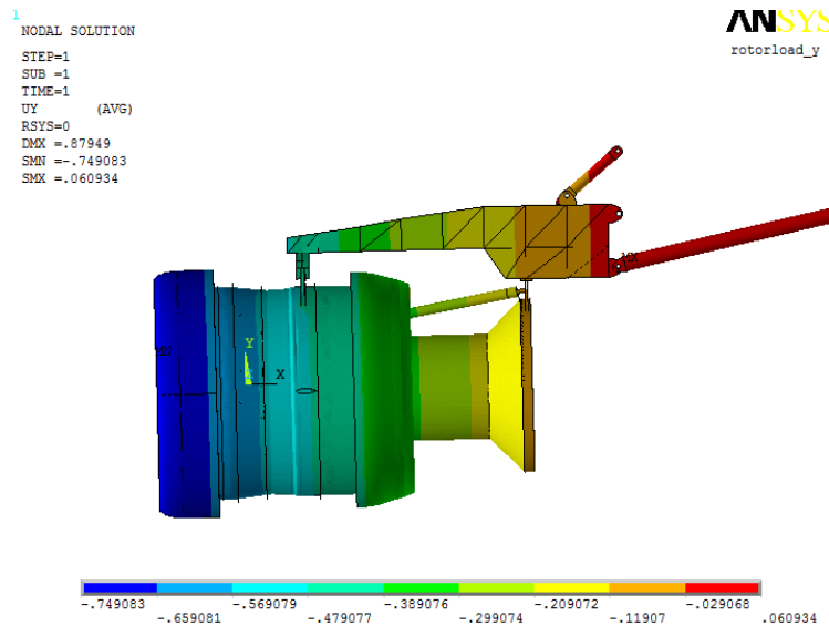
Figure 39. Vertical Displacement of the FBO Full-Fan Rig Model Under Vertical 1000-lb Loading on Fan Disk Centerline
