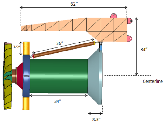
Figure 20. Major Dimensions for the Full-Fan Rig Core and Strut Models
