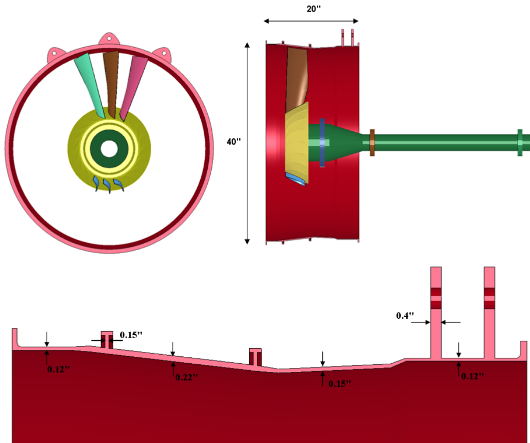
Figure 4. Geometry of the Containment Case
