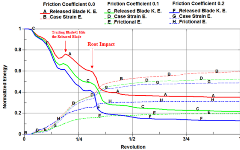
Figure 93. Effect of Friction Coefficient on the Containment Case Strain Energy and Released Blade Kinetic Energy (normalized with respect to initial kinetic energy of the released blade)
