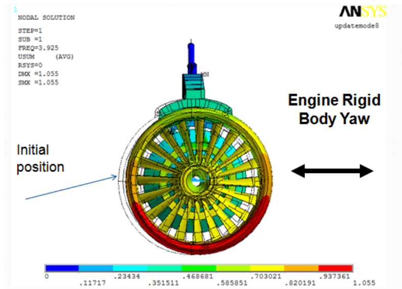
Figure 43. Mode 1—Engine Rigid Body Yaw Mode—3.9 Hz
