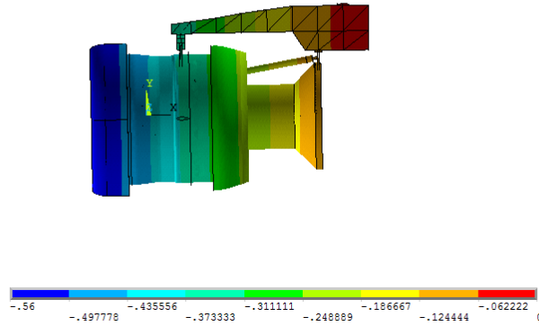
Figure 30. Vertical Displacement (inches) of the FBO Full-Fan Rig Model Under 1g Vertical Loading
