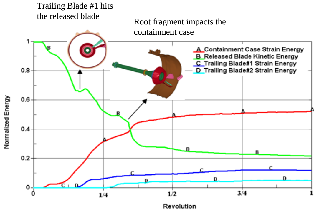
Figure 73. Normalized Kinetic Energy of the Released Blade and Normalized Strain Energy of the Containment Case, Trailing Blade #1, and Trailing Blade #2 (normalized with respect to initial kinetic energy of the released blade)
