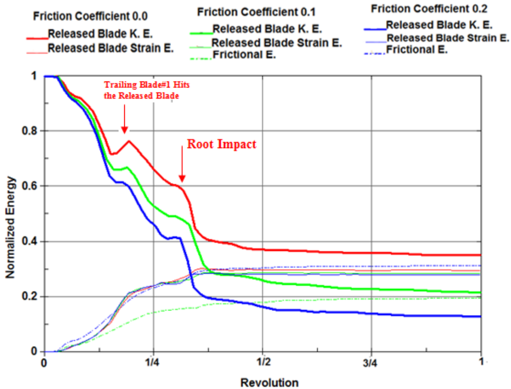
Figure 94. Effect of Friction Coefficient on the Released Blade Strain Energy and Kinetic Energy (normalized with respect to initial kinetic energy of the released blade)
