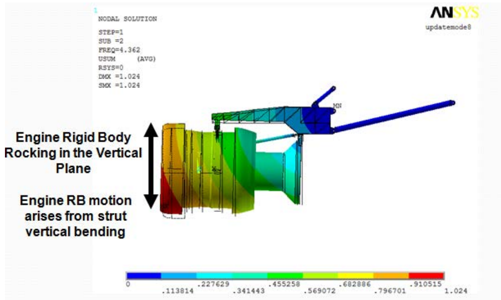
Figure 44. Mode 2—Engine Rigid Body Rocking in the Vertical Plane 4.3 Hz
