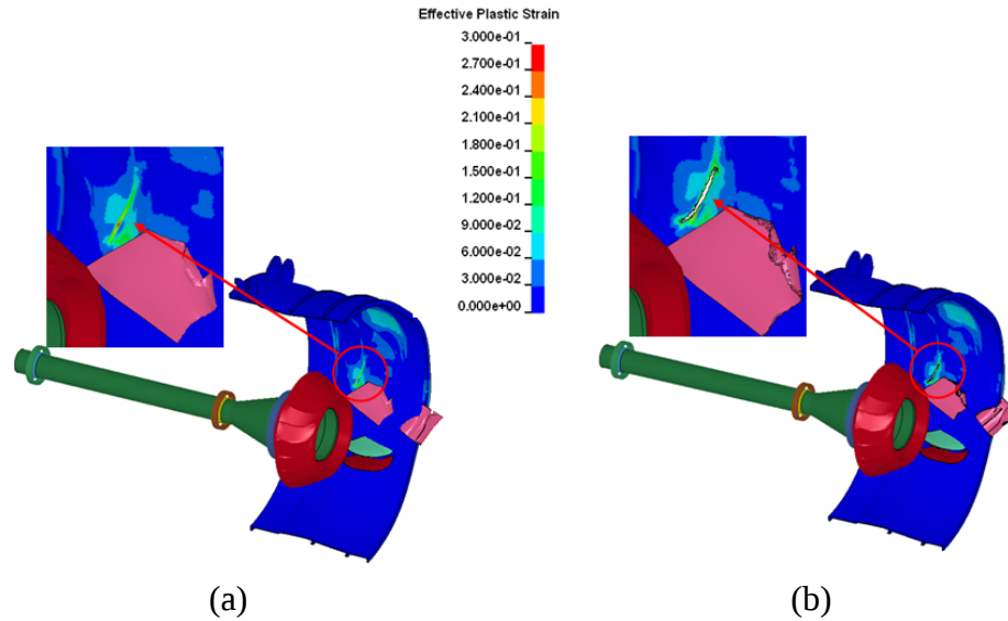
Figure 97. Effect of Johnson-Cook Damage Parameters (a) LLNL-3 and (b) LLNL-2 on the Containment Case Damage for Case 1 ( \mu = 0.0 )
