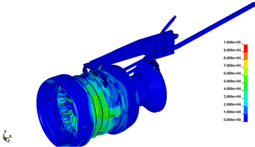
Figure 105. Stresses Scaled to Highlight Containment Case Damage at 3.5 ms
