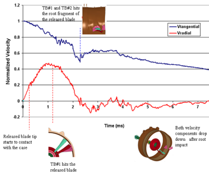
Figure 75. Velocity of the Released Blade Initial CG During Interaction With the Case (normalized with respect to initial velocity of the released blade)
