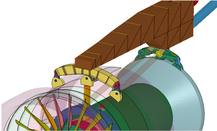
Figure 25. Front and Aft Mount Isometric View
