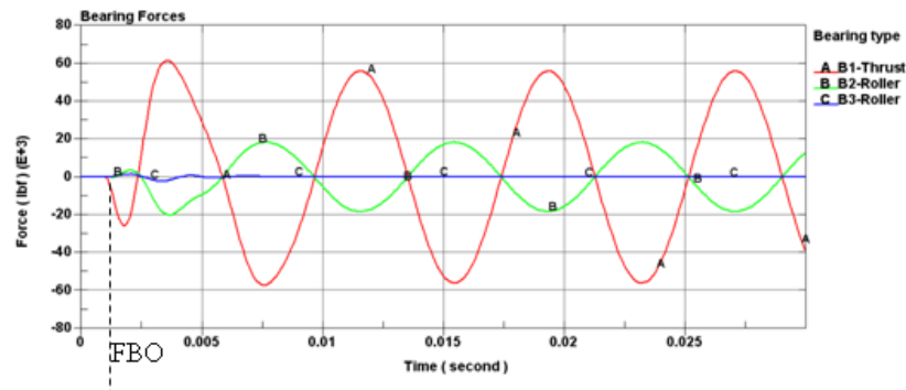
Figure 16. Bearing Forces Due to Imbalanced Load
