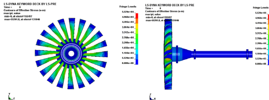
Figure 14. Imbalance Analysis of the Fan Rotorblade System in LS-DYNA
