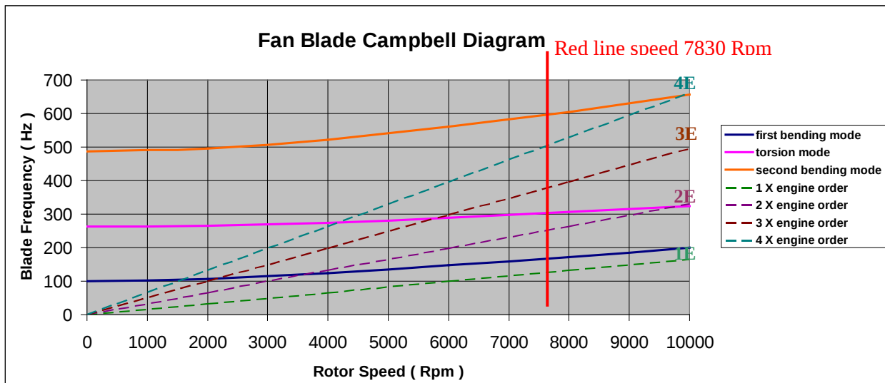
Figure 7. Fan Blade Campbell Diagram
