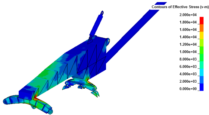
Figure 107. Strut, Forward, and Aft Mount Damage at 3.5 ms
