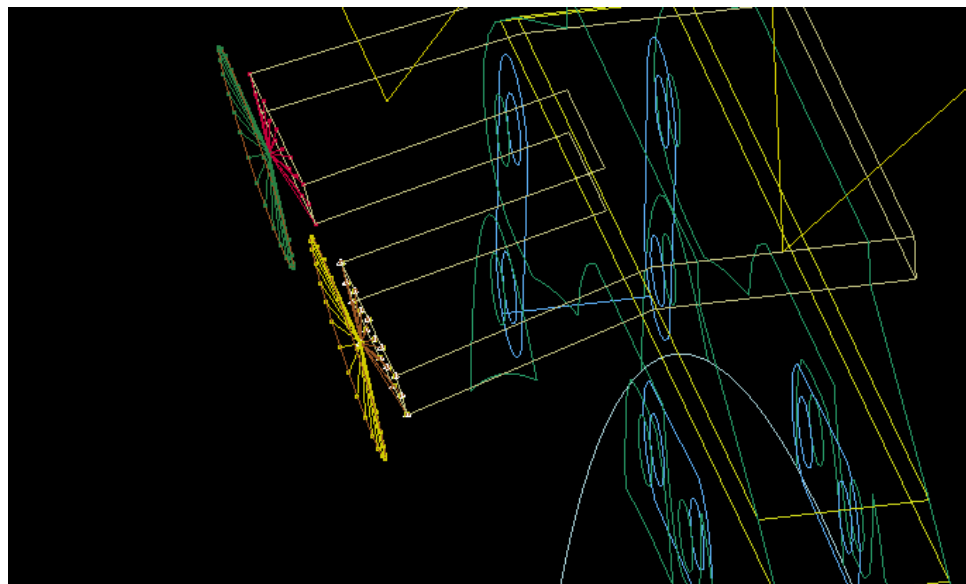
Figure 59. Thrust Link to Aft Mount Yoke Spherical Joint Details
