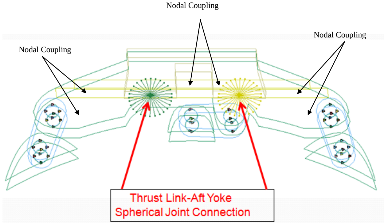
Figure 66. Connection Points of the Aft Mount to Spherical Joint and Nodal Coupling
