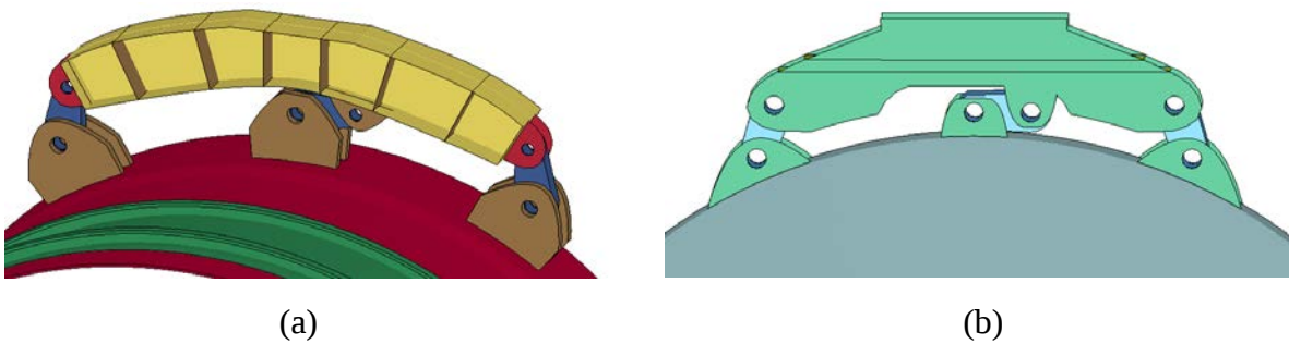
Figure 26. Closeup View of the (a) Front Mount and (b) Aft Mount
