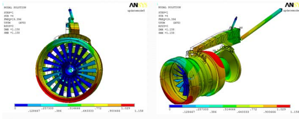
Figure 46. Mode 4—Strut Second Lateral Bending Mode—19.3 Hz
