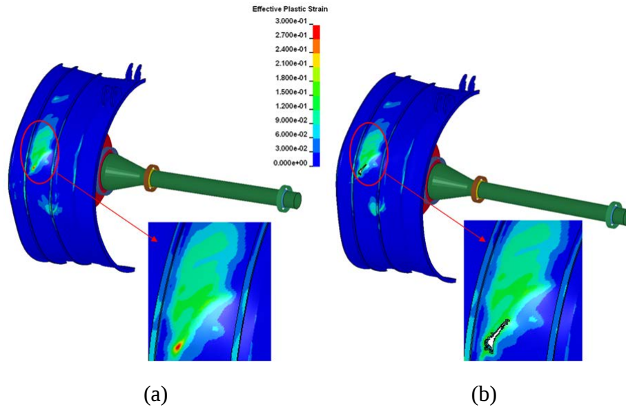
Figure 98. Effect of Johnson-Cook Damage Parameters (a) LLNL-3 and (b) LLNL-2 on the Containment Case Damage for Case 3 ( \mu = 0.2 )
