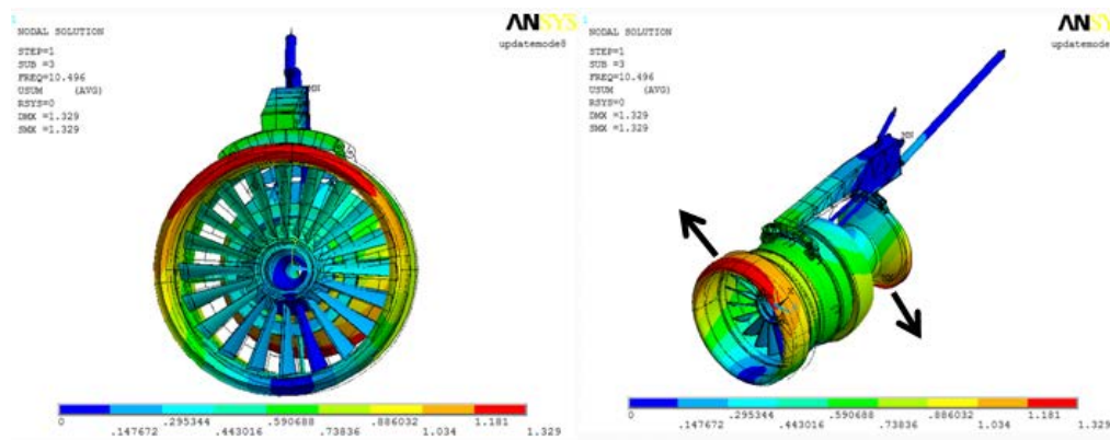
Figure 45. Mode 3—Engine Rigid Body Roll Mode 10.4 Hz
