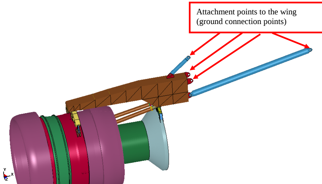
Figure 27. Wing Strut Attachment Points
