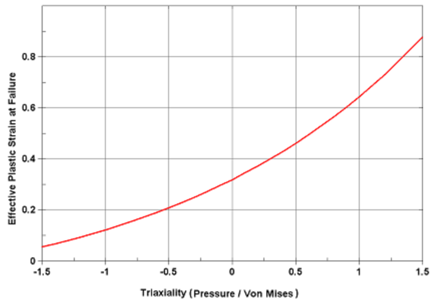
Figure 67. Fracture Locus of Ti 6Al-4V at Nominal Strain Rate of 1/s
