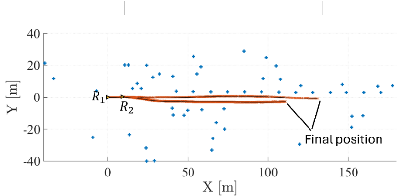
Fig. A2. 3\sigma envelope of robots' state of interest, with the robots' heading direction selected.
