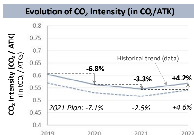
Figure 4. Historical trends in combustion CO 2 intensity (in CO 2 /ATK) for the U.S. aviation sector from 2019 to 2022 in context of the projections from the 2021 U.S. Aviation Climate Action Plan.
