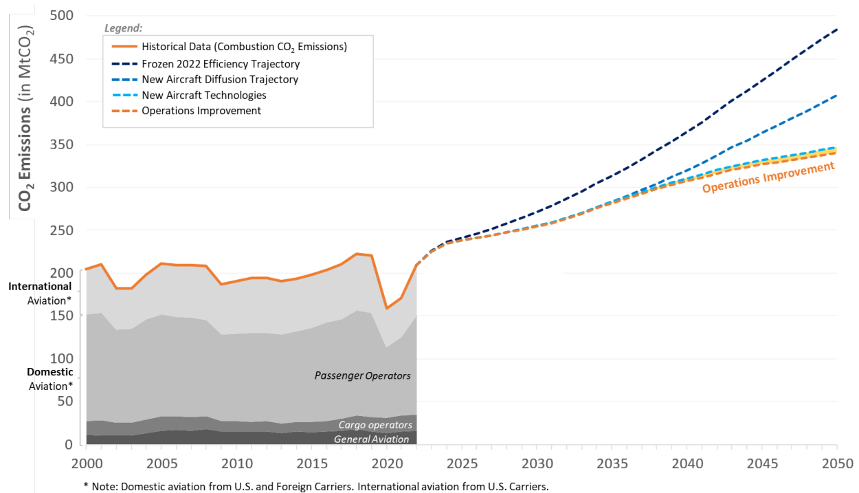
Figure 9. Analysis of Future Domestic and International Aviation CO 2 Emissions: Operations Improvement Scenario
