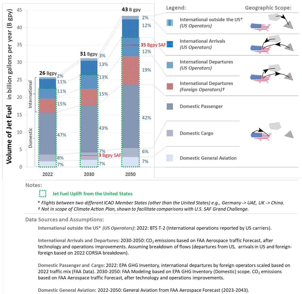
Figure 11. Potential demand for jet fuel in gallons per year (GPY) across domestic operations (by U.S. and Foreign Carriers), international departures from foreign carriers and international operations by U.S. carriers. Red text indicates SAF Grand Challenge volumetric production goals.
