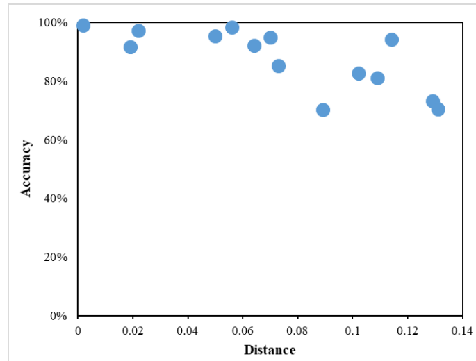
Figure 7.6 Vehicle measurement accuracy vs distance between the embedded sensor and wheel loading position.
