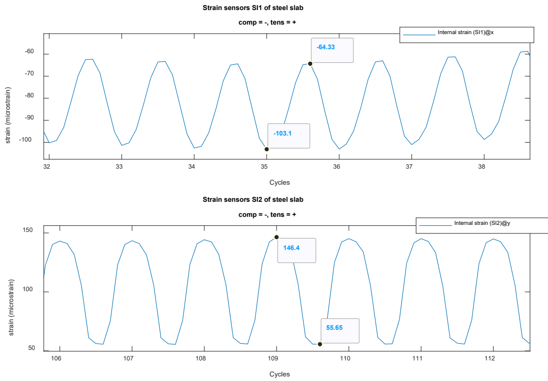
Figure B-8 Internal strain gauges reading (SI1 and SI2), closed-up view, for Panel 2
