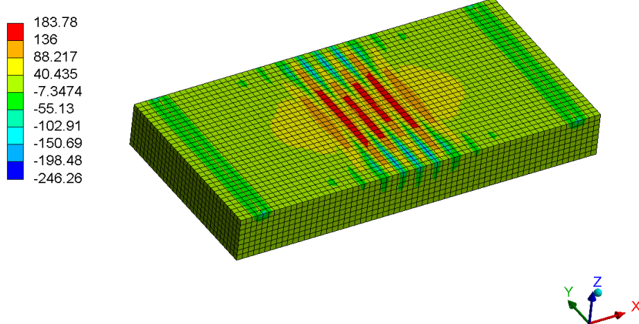
Figure 5.43 Stress component (SY) concrete of Panel 1 at ultimate limit load: (a) bottom face view, and (b) top face view
