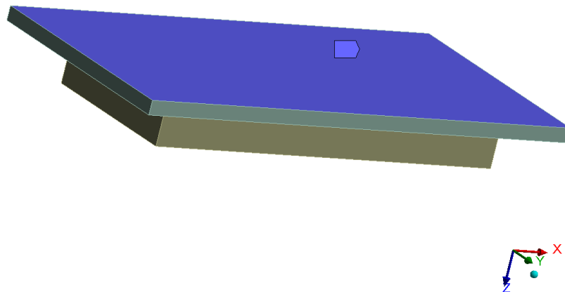
Figure 4.12 Fixed support applied at the bottom face of the gravel support
