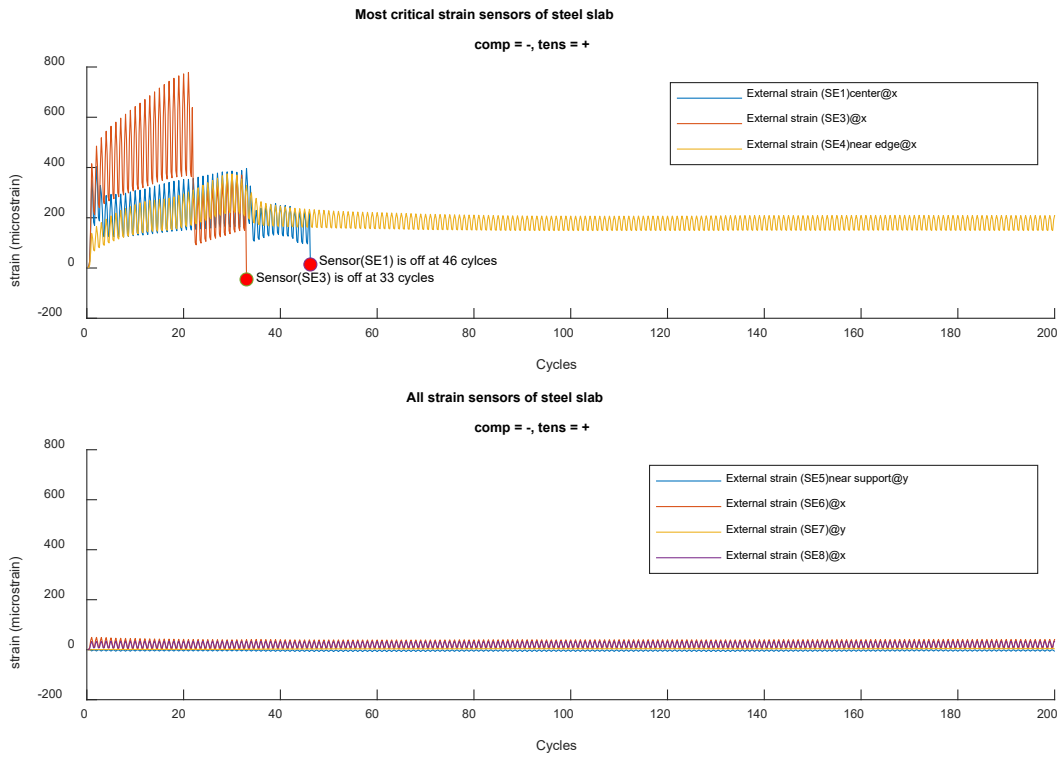
Figure B-7 External strain gauges reading (SE1, SE3, SE4, SE5, SE6, SE7, and SE8) for Panel 2
