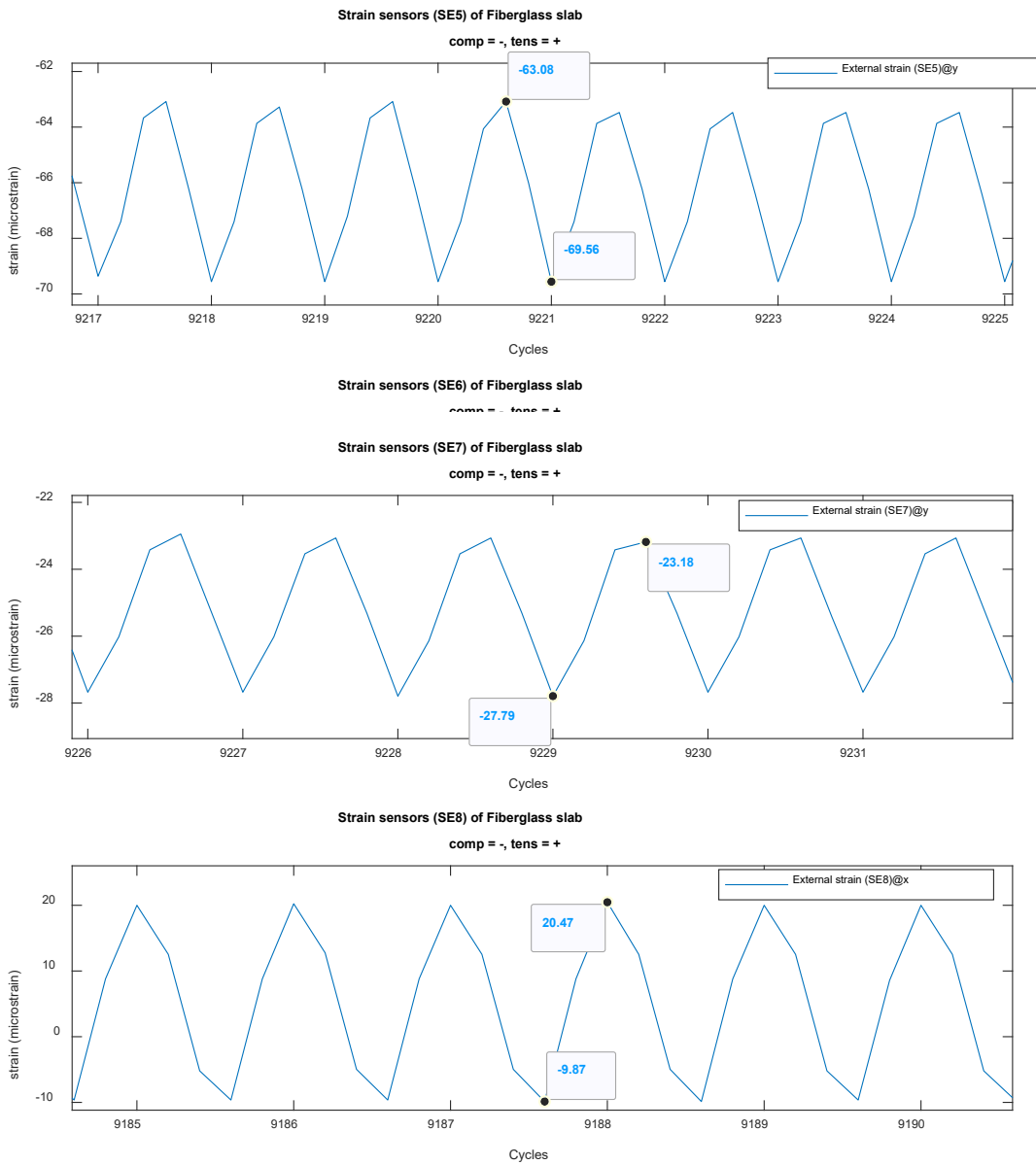
Figure B-5 All external strain gauges reading (SE1 to SE8), closed-up view, for Panel 1
