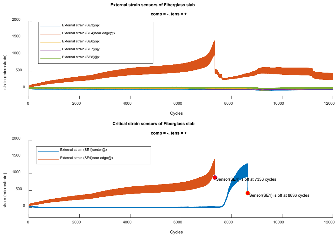
Figure B-3 External strain gauges reading (SE1, SE3, SE4, SE5, SE6, SE7, and SE8) for Panel 1
