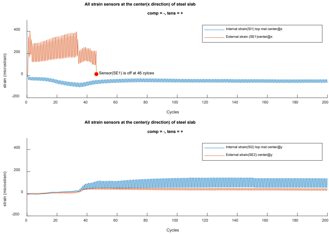
Figure B-6 Comparison of internal and external strain gauges reading (SI1 and SE1) and (SI2 and SE2) for Panel 2
