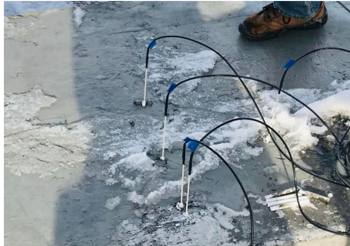
Figure 3.14 Temperature sensors inserted into the tubes
