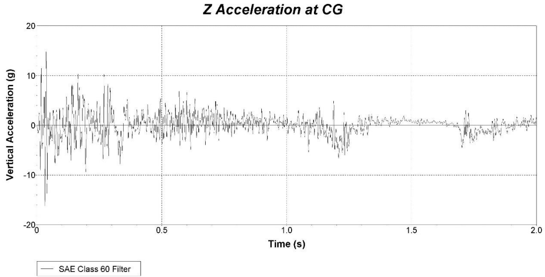
Figure C.10. Vehicle Vertical Accelerometer Trace for Test 440863-03-1 (Accelerometer Located at Center of Gravity).
