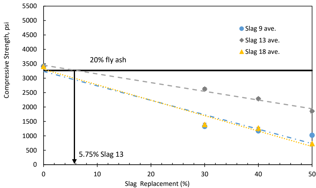
Figure 34: Compressive strength of concrete containing fly ash, slag 9, slag 13 and slag 18 at 18 hr under lab temperature curing (73°F)
