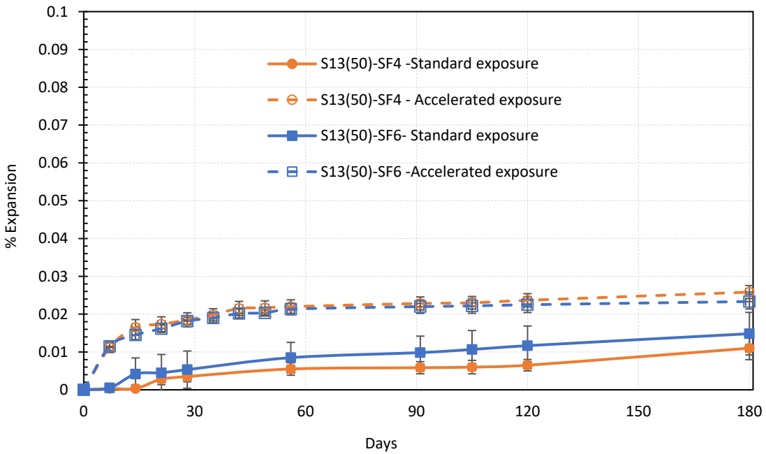
Figure 31: Comparison of the expansion behavior of ternary blended mixture of 50% cement replacement with slag 13 and 4% and 6% silica fume under standard and accelerated exposure
