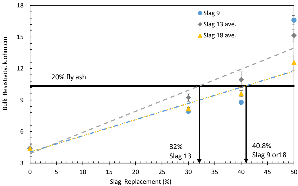
Figure 45: Bulk electrical resistivity of concrete containing fly ash, slag 9, slag 13, and slag 18 mixtures at 28 days under accelerated curing (100°F)
