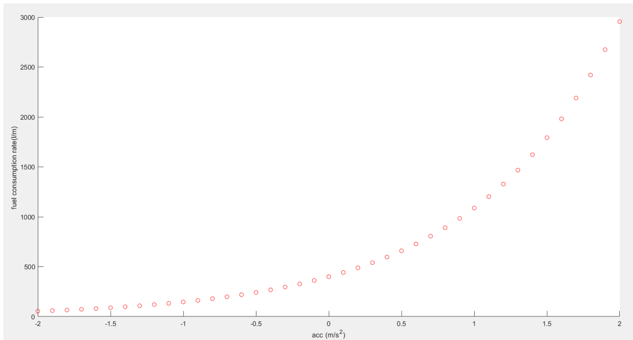
Figure 18 a sample proposed model (a log-transferred) with v=20 \text{ m/s} a from -2 \text{ m/s}^2 to 2 \text{ m/s}^2
