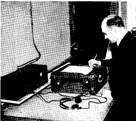
Figure 7.—Recorded in operation. Operator is drawing lines connecting signal impulse marks for each element, for later measurement and evaluation. Radio receiver (left) with earphones for tuning.
