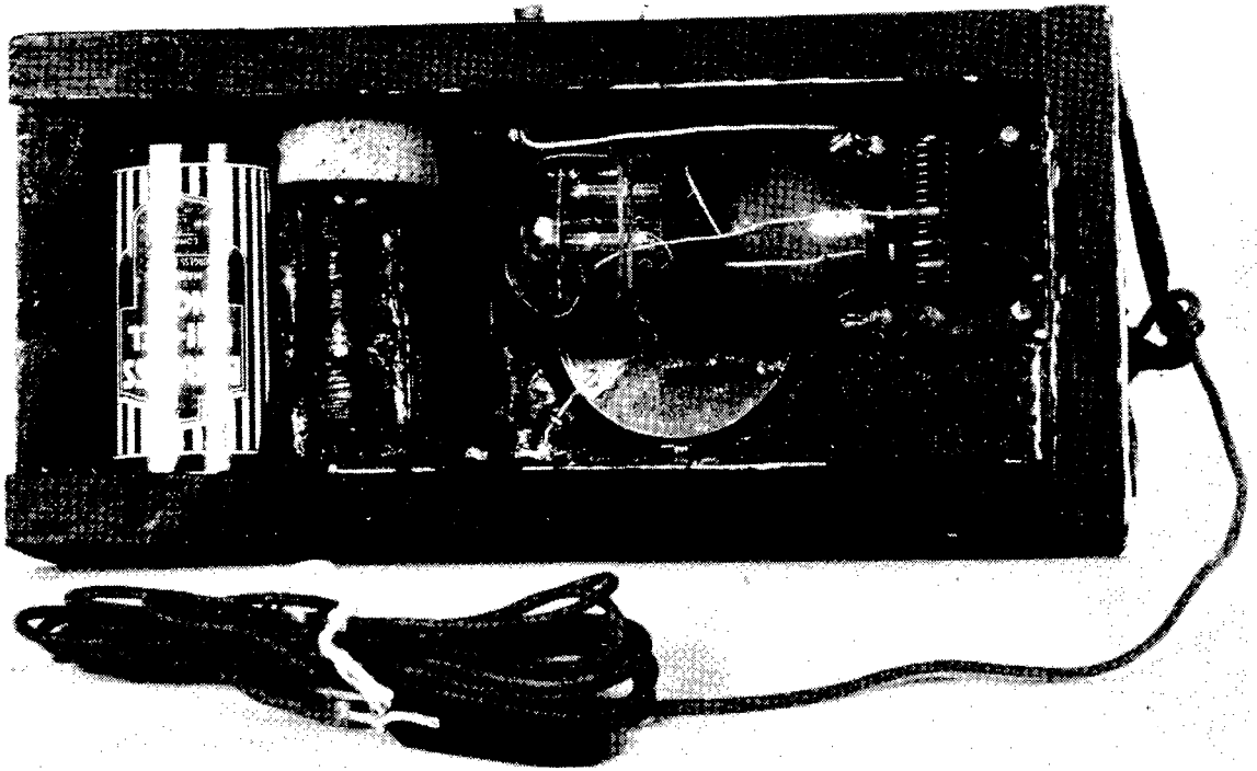
Figure 4.—Complete transmitter used in the Harvard instrument. The clock is located behind the tube.
