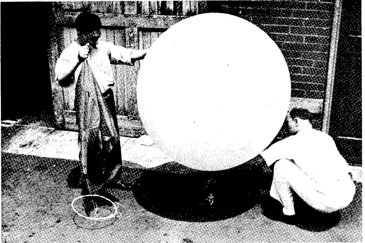
Figure 5.—Inflating the balloon. Note the weights under balloon. It is inflated until capable of lifting more than 2 lbs. Operator at left is holding parachute ready to be attached in the final assembly.
