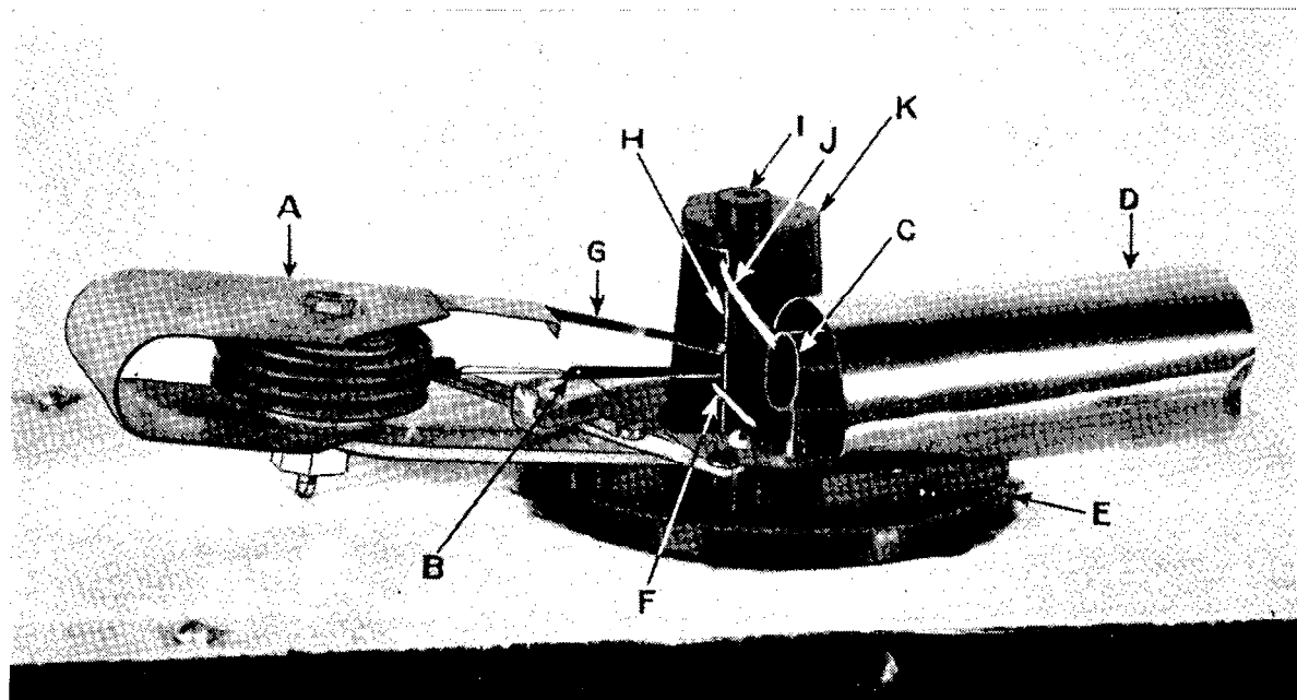
Figure 2.—A. Aneroid barometer with 4 cells. B. Hygrometer showing hairs and pen. C. Temperature element. D. Shield for temperature element. E. Bakelite base. F. Reference pen. G. Pressure pen. H. Helix. I. Upper bearing for helix J. Temperature pen. K. Rain shield around helix.
