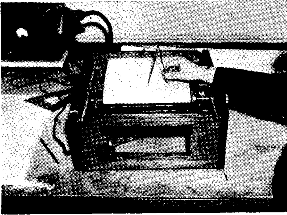
Figure 9.—The recorder. Operator is measuring distances from the reference line to the other lines with a divider. He then sets off the same distance on the calibration curve, reads the value from the scale, then plots the data on the adiabatic chart.
