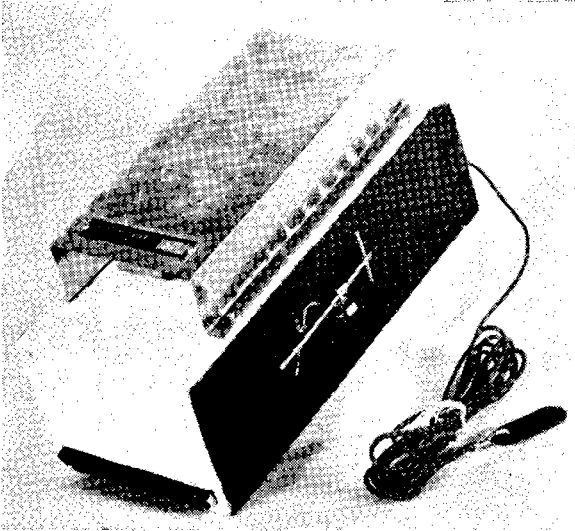
Figure 1.—The Harvard Radiotelemeter with antenna attached. Box painted black and white houses the transmitter and clock. The key is for winding the clock. The aluminum shield covers the aerological instruments. Sliding door (on bottom) is for access to transmitter. Total weight 1.8 pounds.
