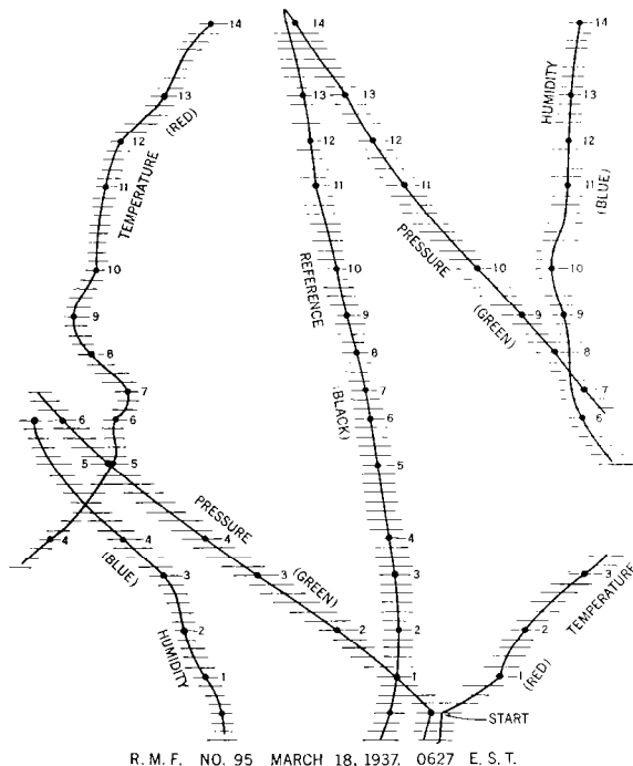
Figure 8.—A typical recording. Note comparatively straight reference line, also temperature inversions, fluctuating humidity and steady fall of pressure, the latter denoting increasing altitude. The temperature recording was picked up (lower left) where it ran off paper (lower right). Likewise the pressure recording was picked up (center right) where it ran off paper (center left). Numbers denote corresponding positions. They are written in as the recording progresses to obtain correct measurements. For example, measurement from the reference line at station "10" would be to station "10" of the other recordings.
