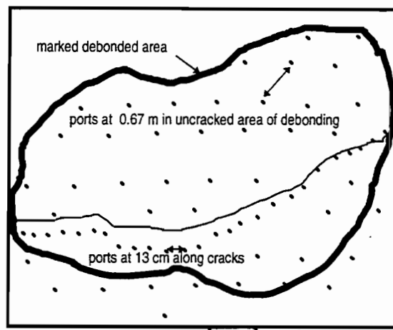
Figure 3.4 Typical port spacing for epoxy injection of debonded overlay areas
