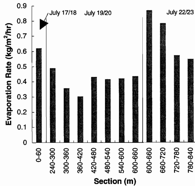
Figure 2.5 Average evaporation rates during westbound lane construction
