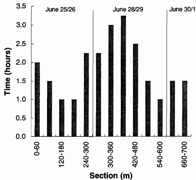
Figure 2.6 Time between concrete placement and application of the curing compound on the eastbound lane
