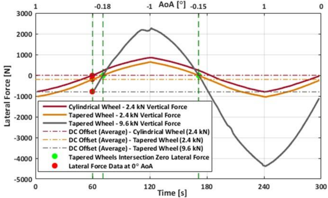
Figure 5.25 Lateral Forces Measured During the Experiments
