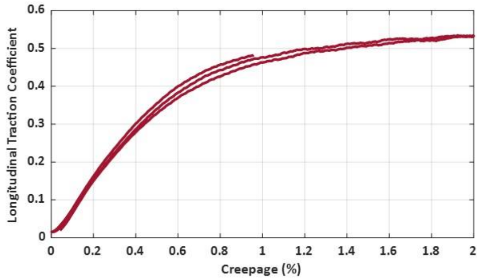
Figure 5.9 Longitudinal Traction Coefficient vs. Creepage Curve
