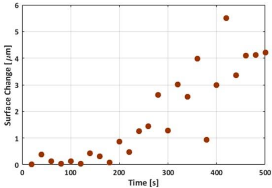
Figure 6.15 Average of the Wheel Wear on the Wheel Surface in the Running Band
