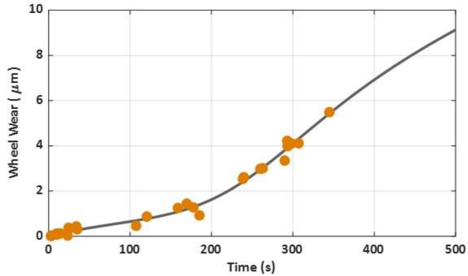
Figure 6.17 Time-Adjusted Wheel surface Change Due to the Wheel Wear
