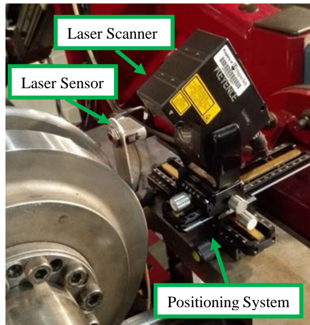
Figure 6.2 Laser Scanner System Mounted on the Rig
