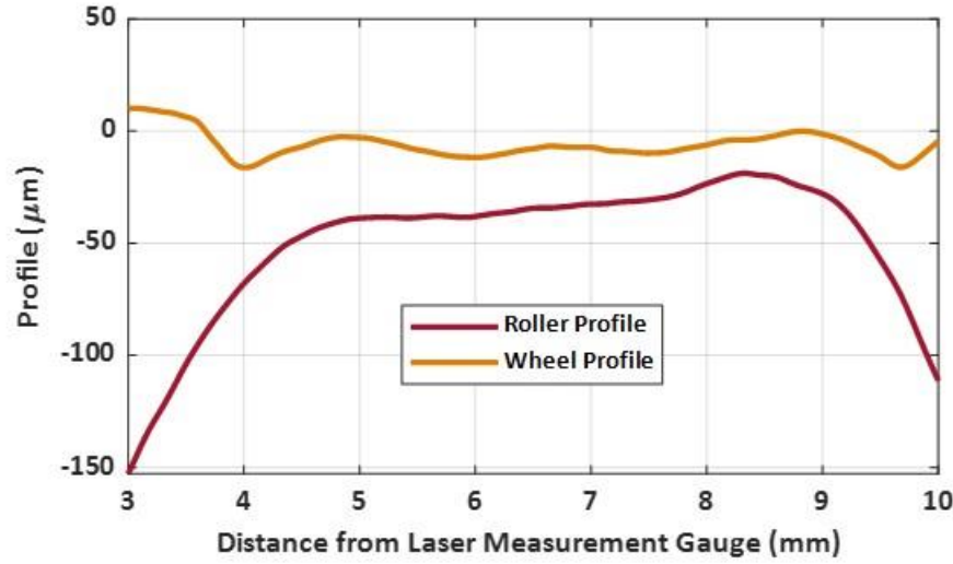
Figure 7.20 Wheel and Roller Surface Profiles Used for Contact Patch Simulation
