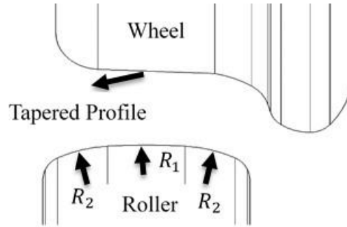
Figure 7.1 The Wheel and the Roller Profiles at Contact
