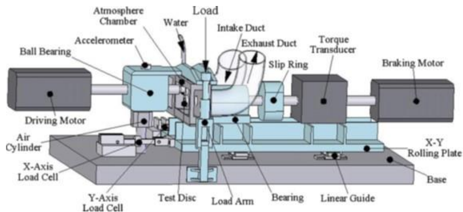
Figure 2.1 Twin-Disc Rolling-Sliding Frictional Machine [1]
