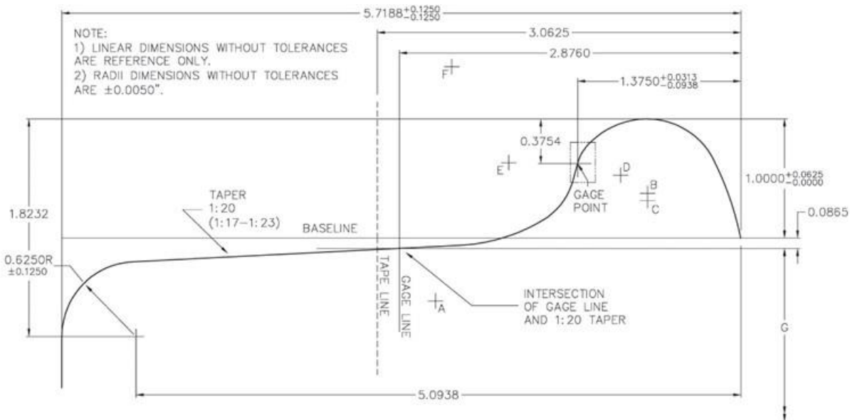
Figure 3.1 AAR-1B Wheel Profile [43]
