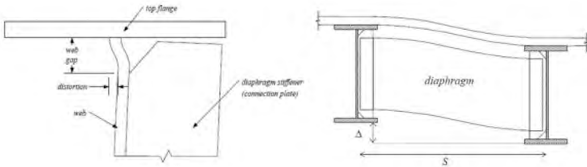
Figure 2.14: Distortion induced fatigue (Li and Schultz 2005)
