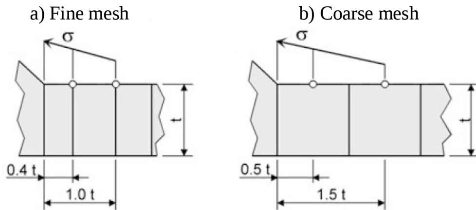
Figure 3.37: Hot-spot method reference point locations (Hobbacher 2016)
