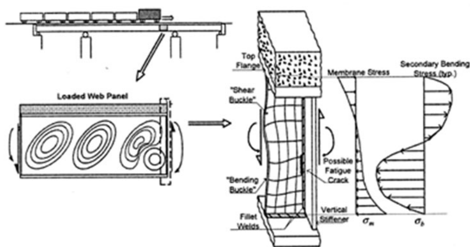
Figure 2.17: Web breathing effect for a slender composite bridge girder (Crocetti 2001)
