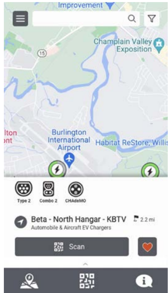
Figure 4.1 – BETA App
