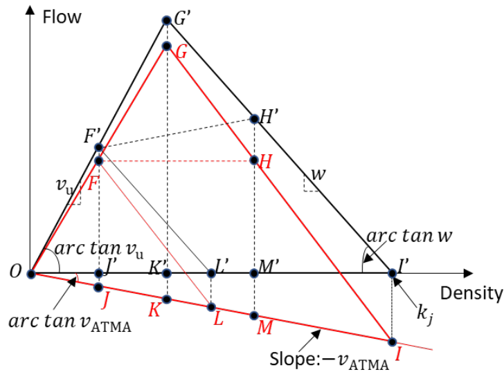
Figure 2.2 Flow-density relationship from both a moving observer's view and a stationary observer's view.
