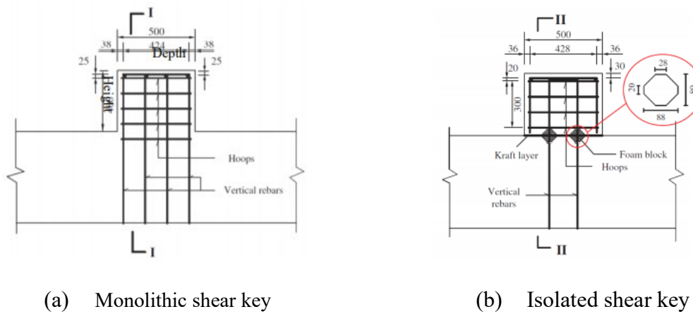
Figure 1.4 Interior shear keys: (a) monolithic and (b) isolated (Han et al., 2018)
