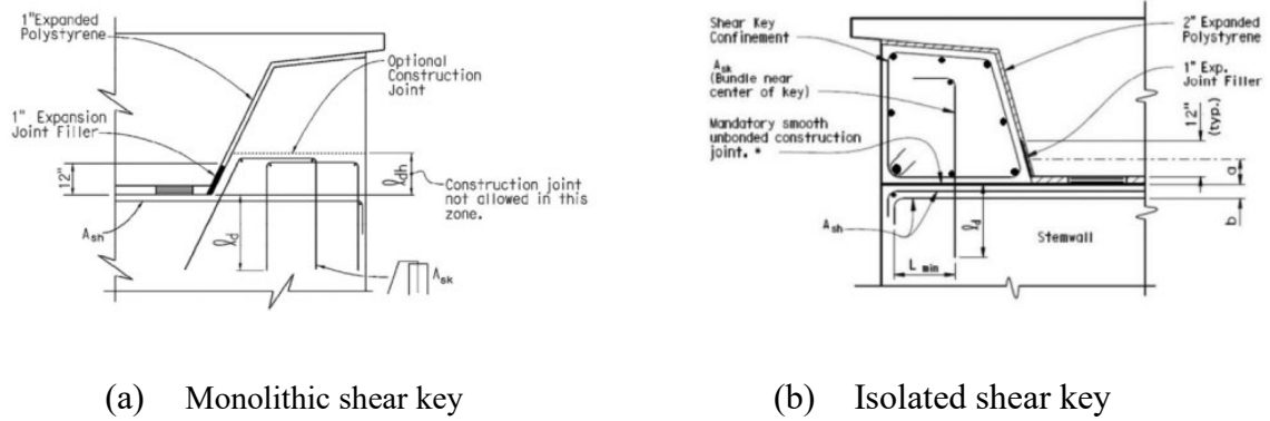
Figure 1.3 Exterior shear keys: (a) monolithic and (b) isolated (Kottari et al., 2020)
