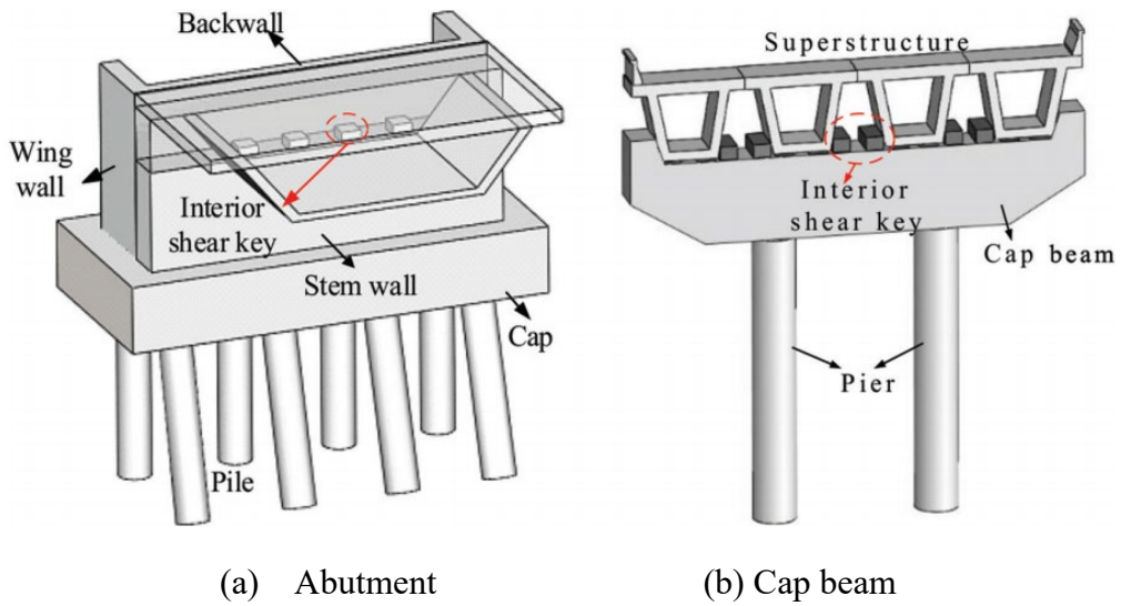
Figure 1.2 Interior shear keys at (a) abutment and (b) cap beam (Han et al., 2018)
