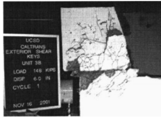
(b) Exterior (Megally et al. , 2001)
