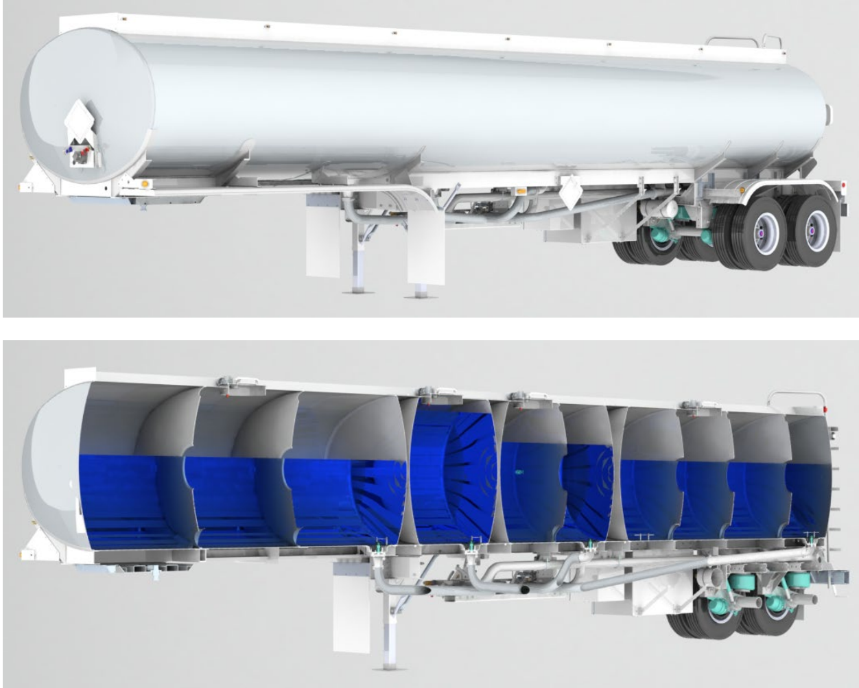
Figure 5.13 Ballast Fill Heights, Test No. MTL6-1
