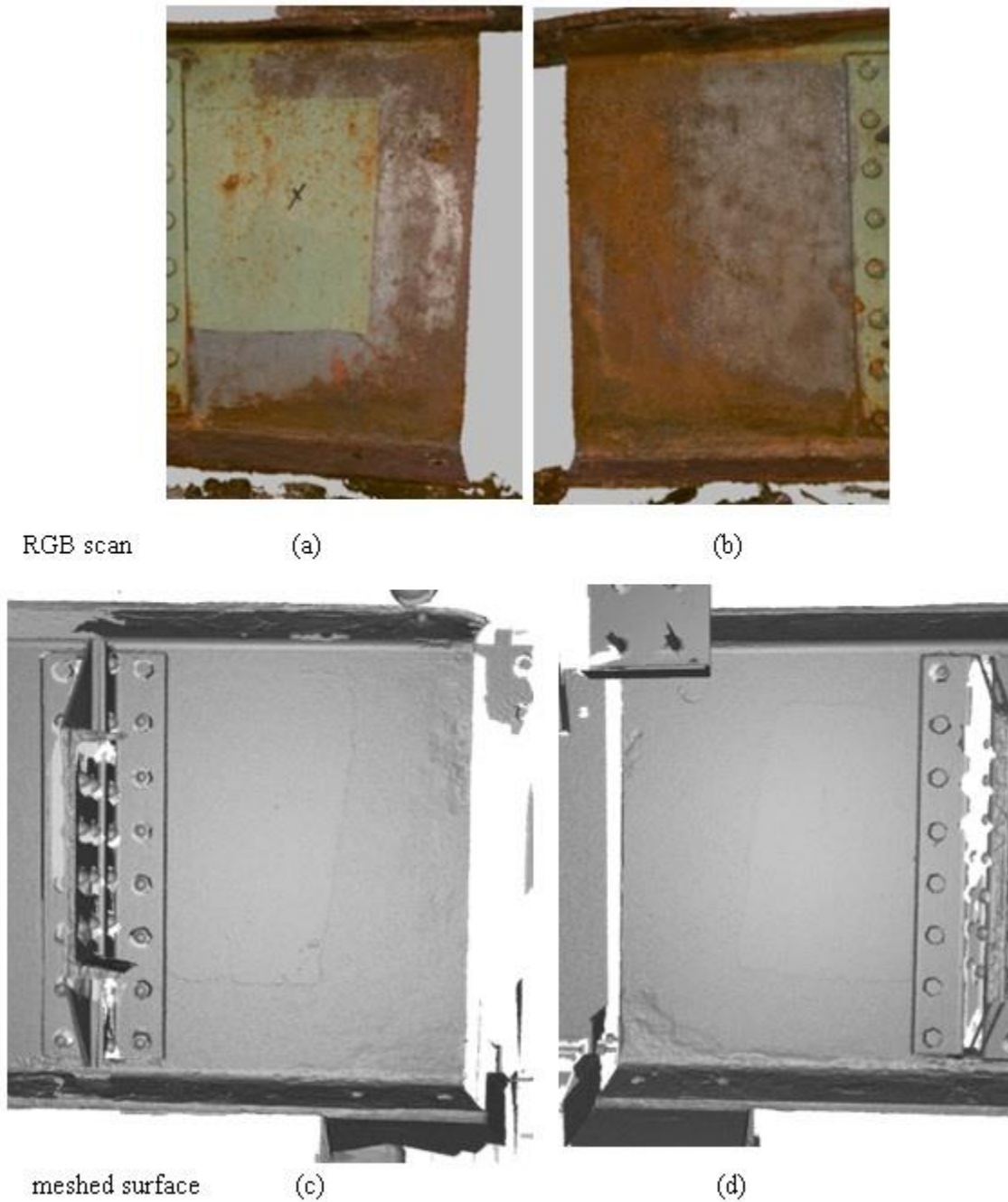
Figure 4.7: Laboratory beam 4
