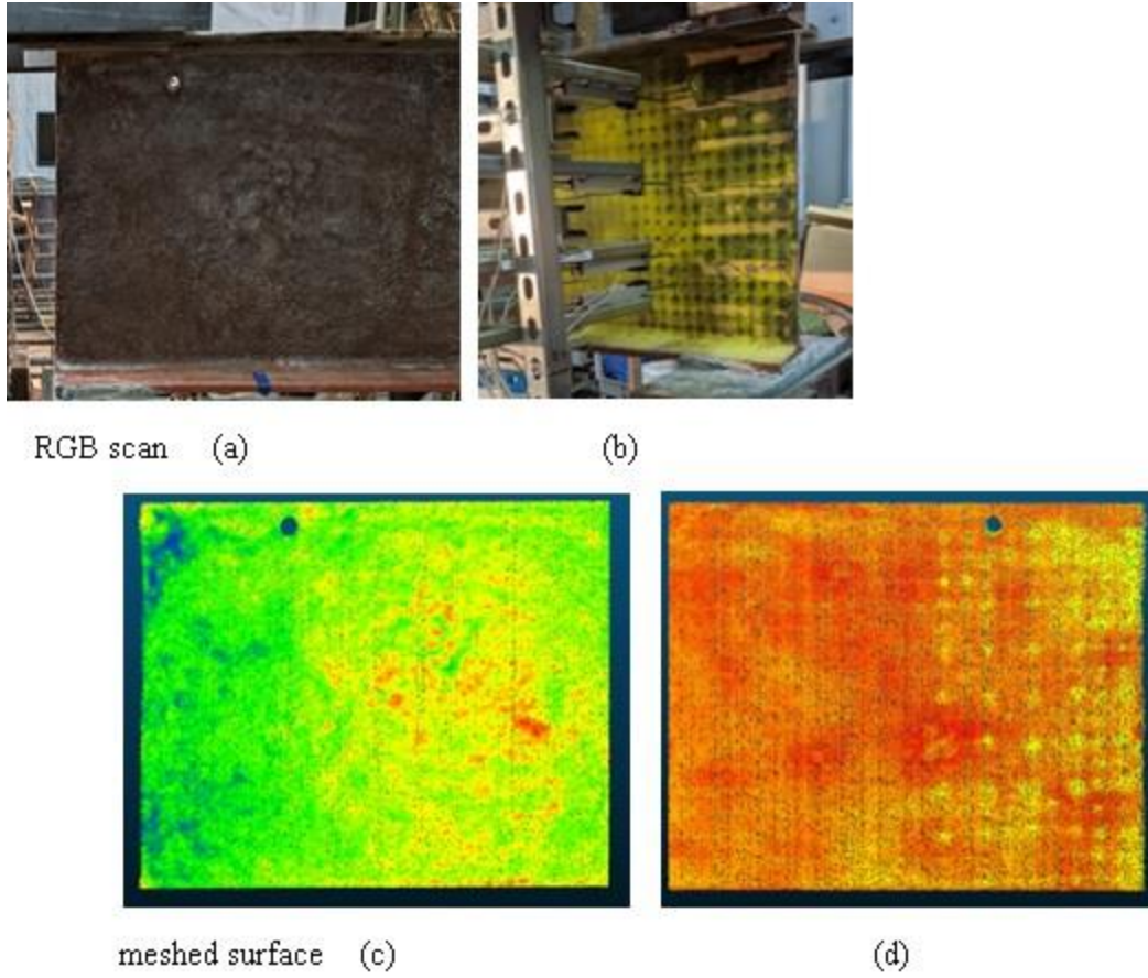
Figure 4.1: Laboratory beam 1
