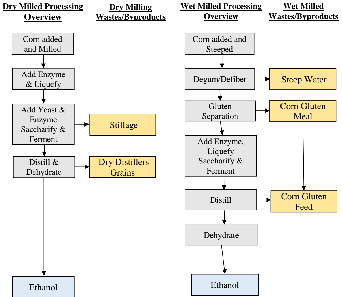
Figure 5.4 Overview of the corn-milling process for ethanol production
