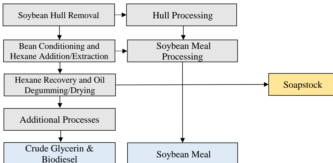
Figure 5.3 Overview of a typical soybean processing plant operation waste product generation
