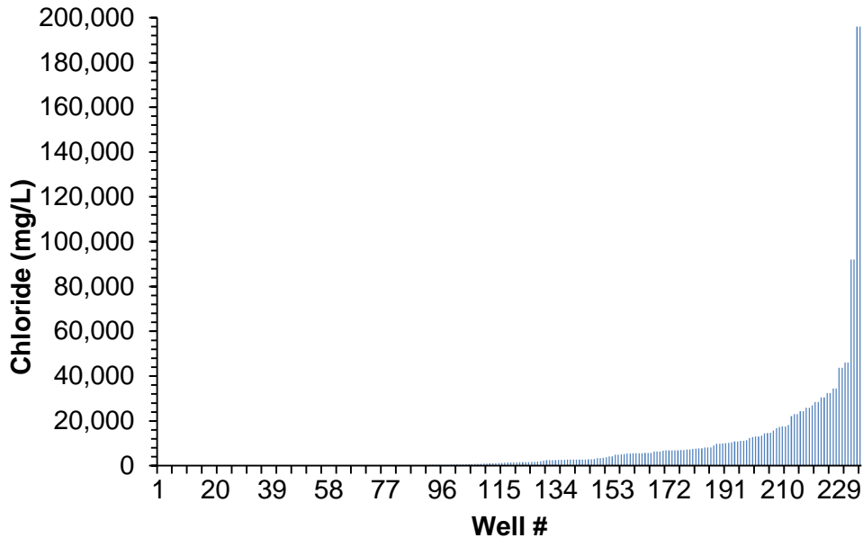
Figure 5.1 Chloride Concentrations in Selected Oil Wells in South Dakota (USGS)
