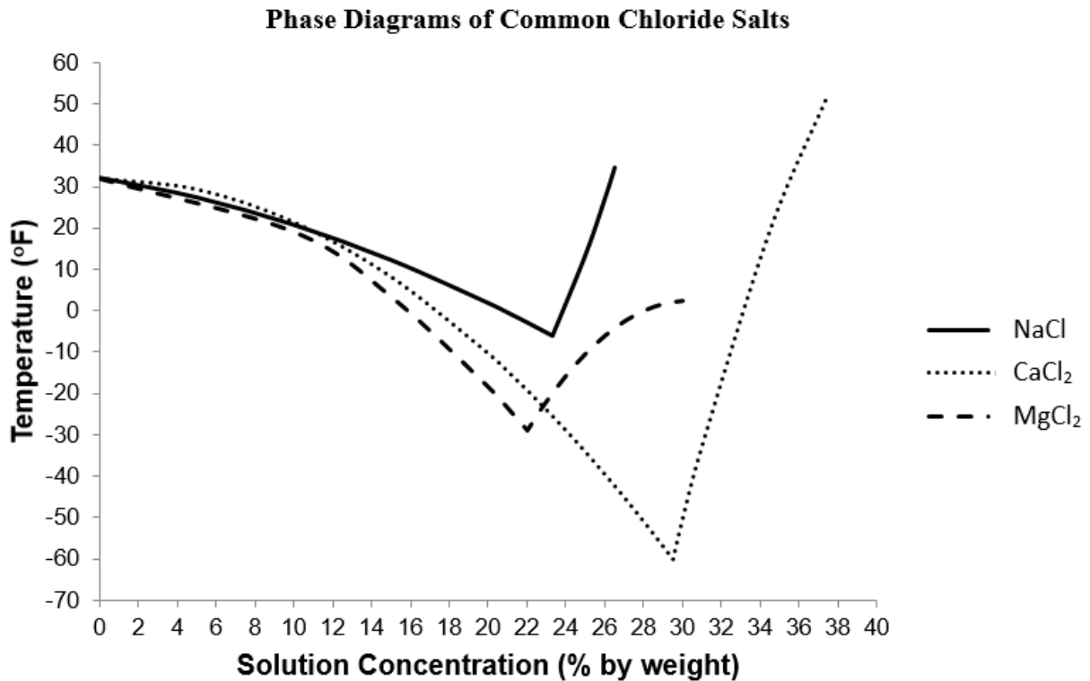
Figure 6.1 Phase diagrams for major chloride salts in brine solutions (Shi, 2009)
