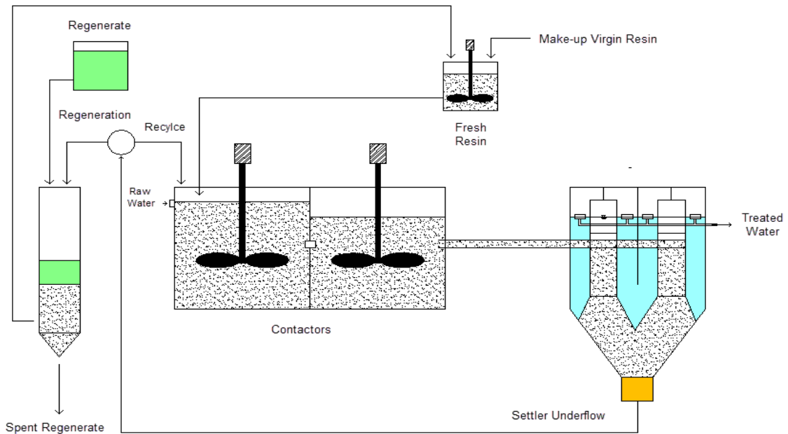
Figure 9.1 An overview of the MIEX ® process (Reproduced from Orica Watercare, Inc)
