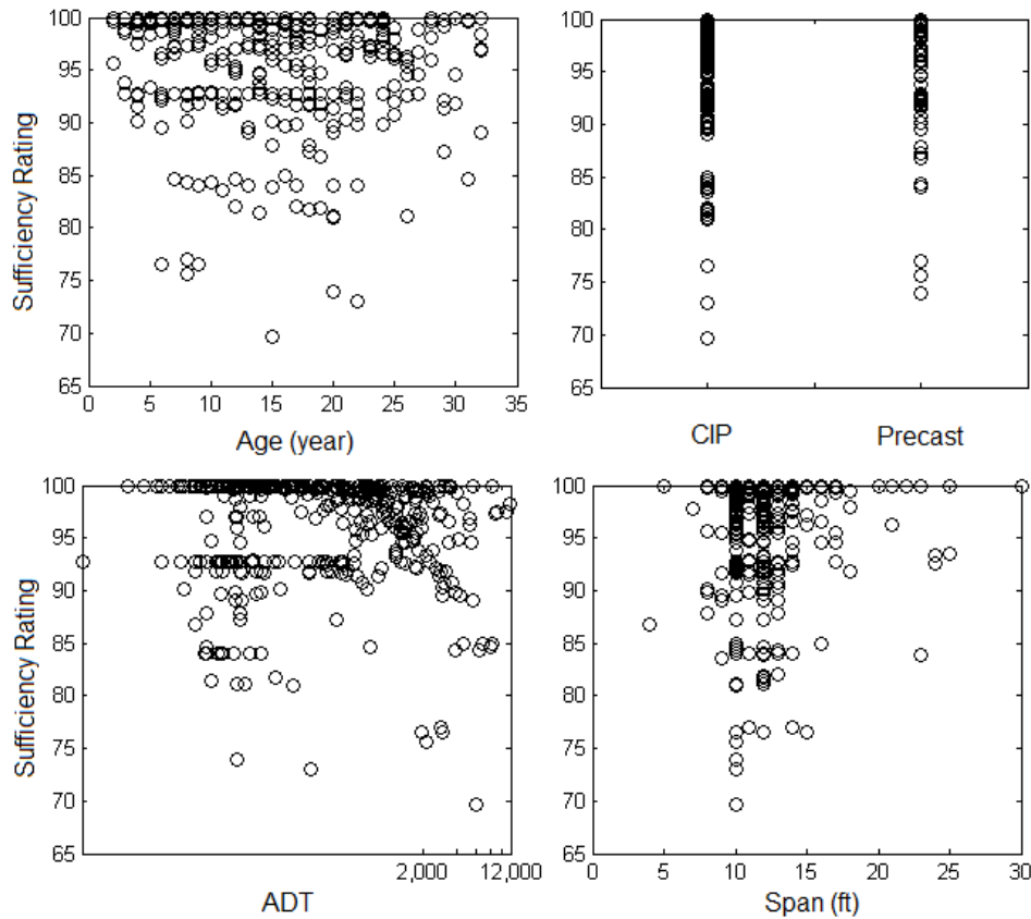
Figure 6-10: Correlation between control variables and current sufficiency rating for concrete culverts
