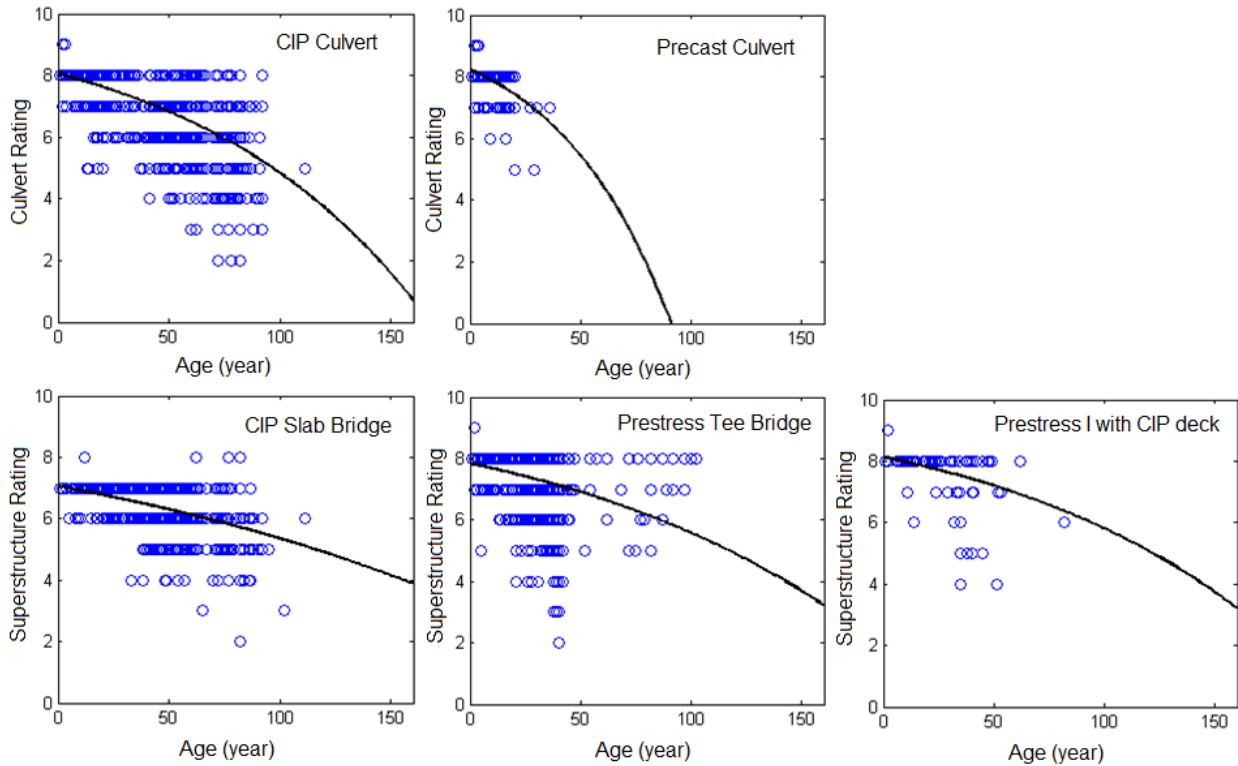
Figure 7-11: Regression analysis on structure rating for service life prediction
