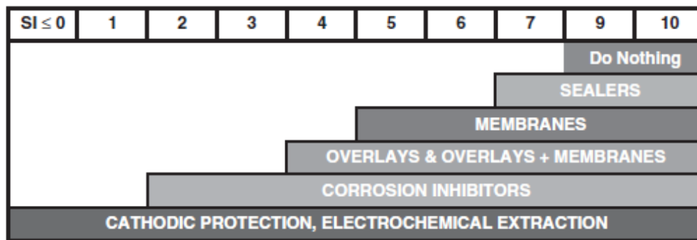
Figure 5-1: Corrosion control measures suggested by NCHRP558
