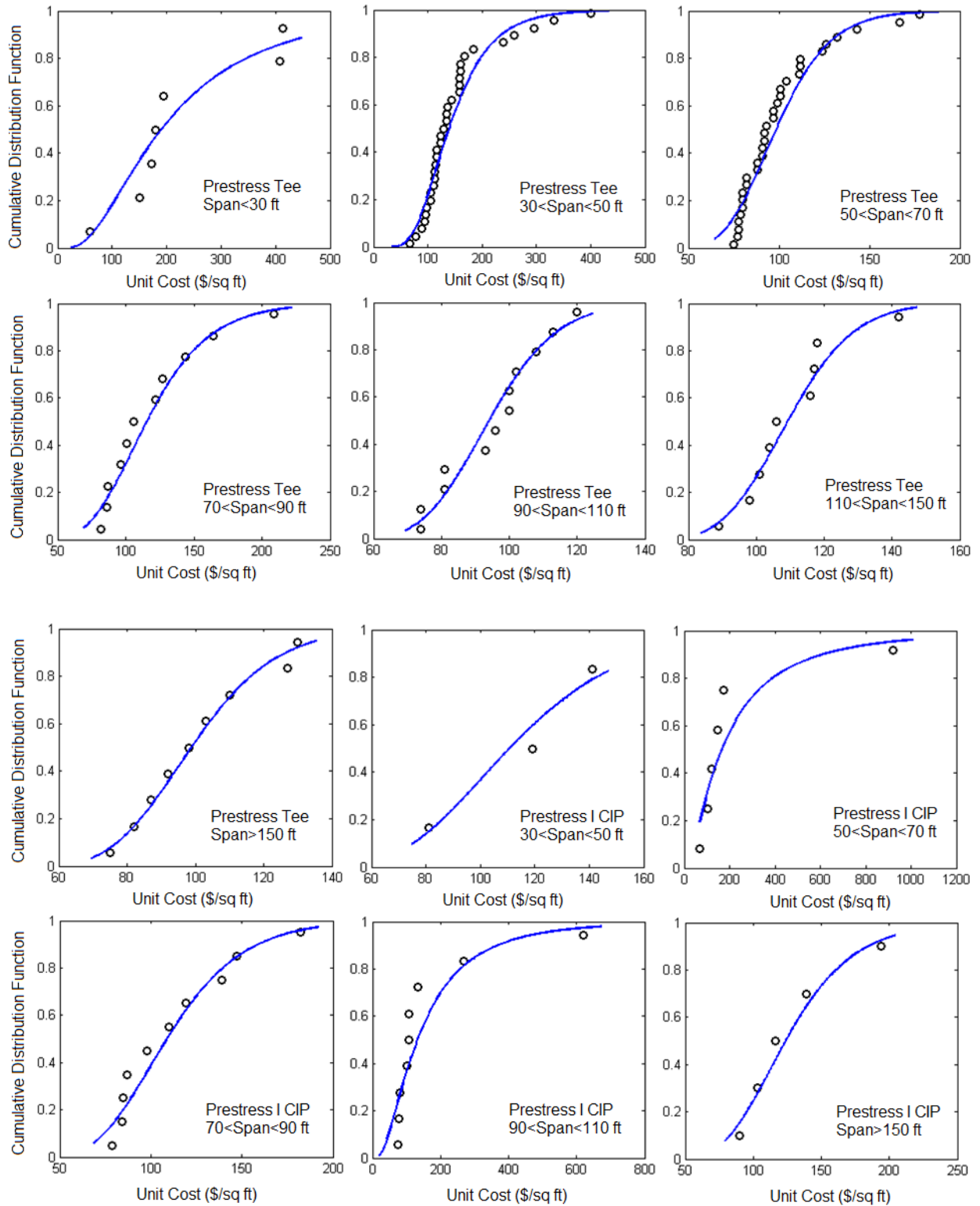
Figure 7-10: Bridge cost data and fitted Lognormal distribution curves
