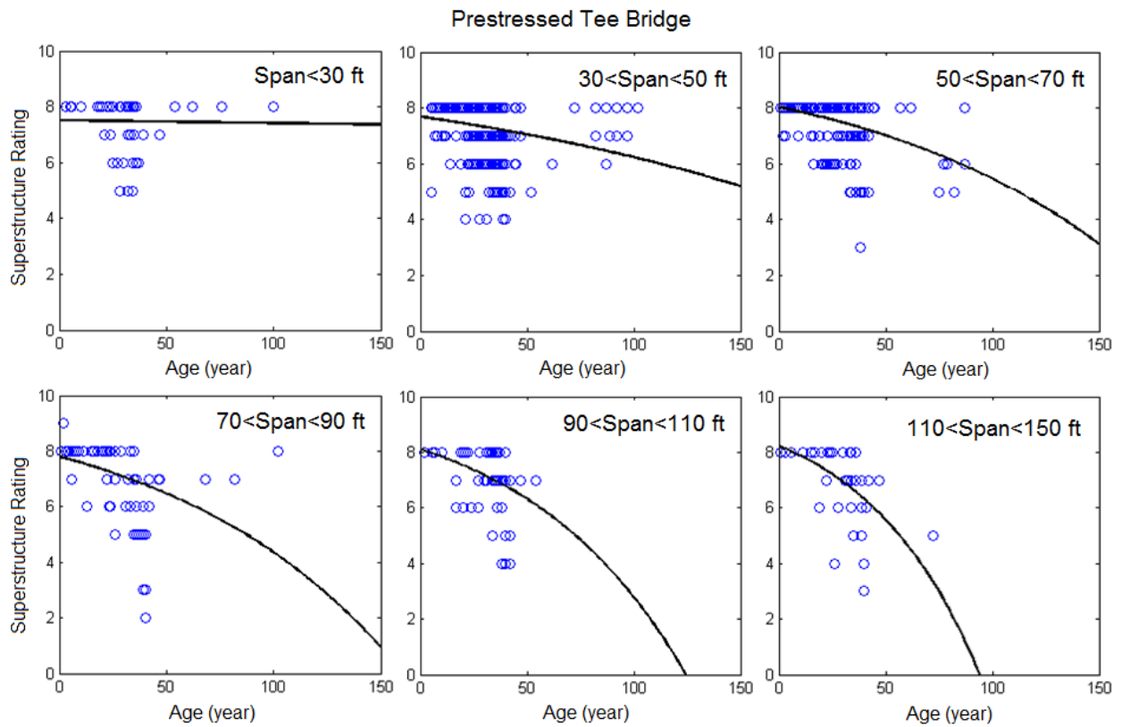
Figure 7-14: Regression analysis on structure rating for service life prediction (Prestressed Tee bridge)
