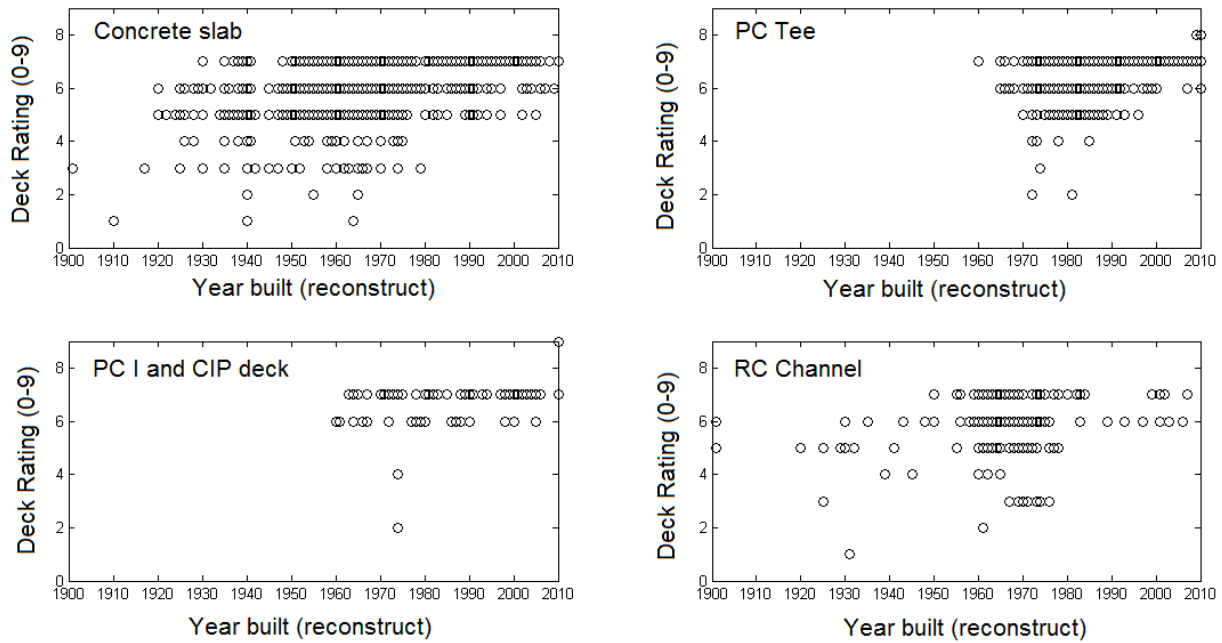
Figure 7-2: Bridge Deck rating comparison break down
