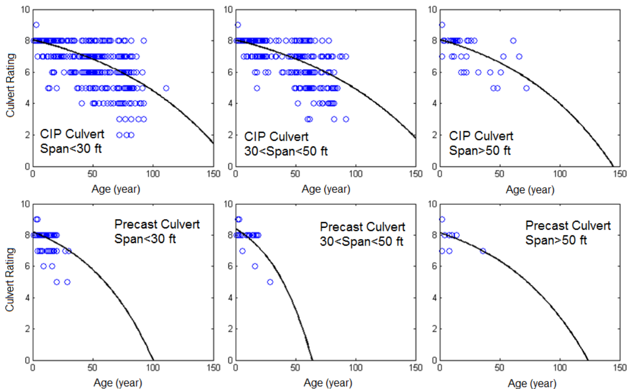
Figure 7-12: Regression analysis on structure rating for service life prediction (Culverts)
