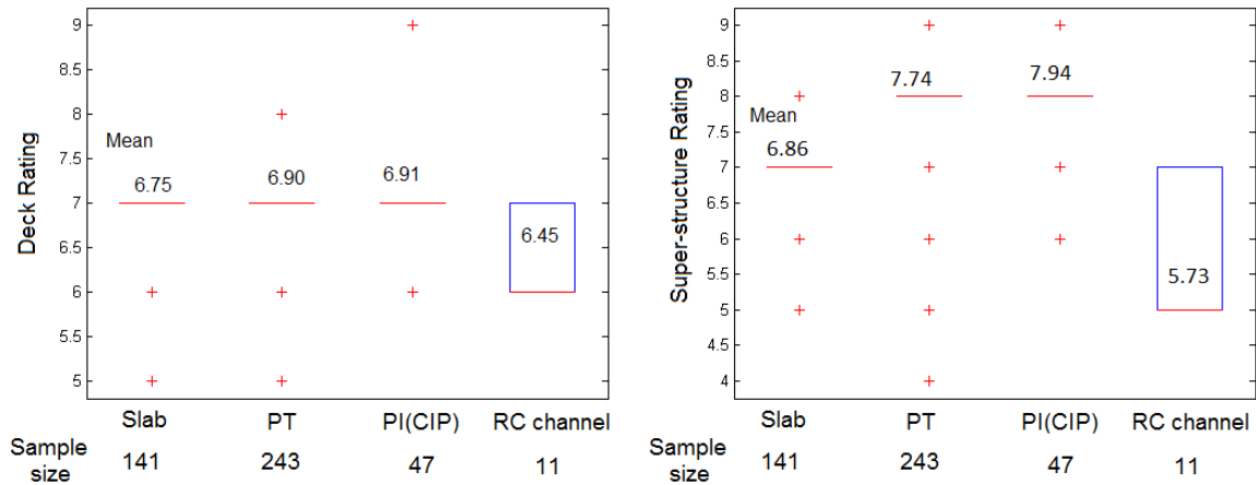
Figure 7-5: Group 1 comparison between bridge types
