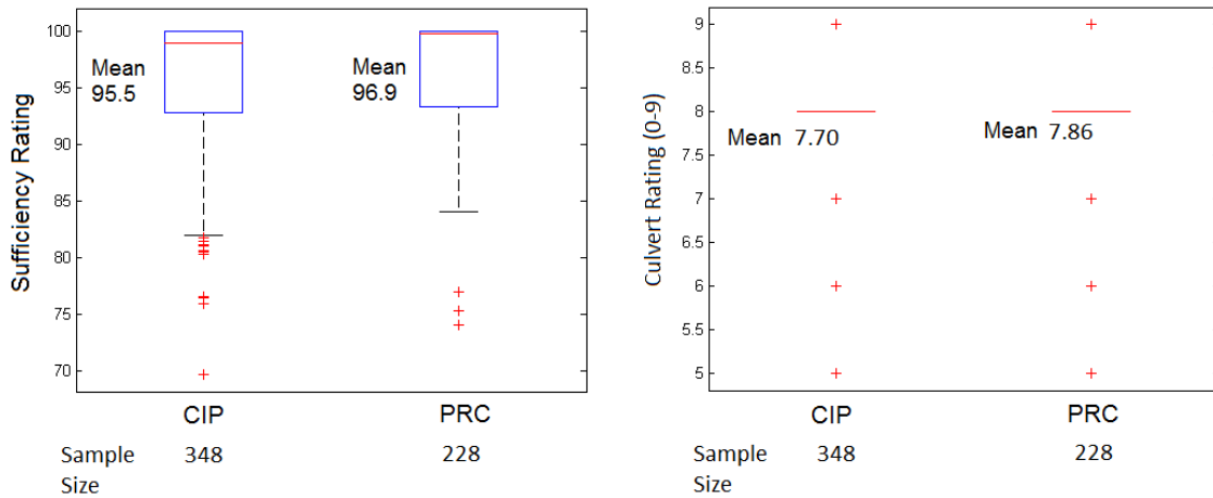
Figure 7-8: Culvert sufficiency rating box plot
