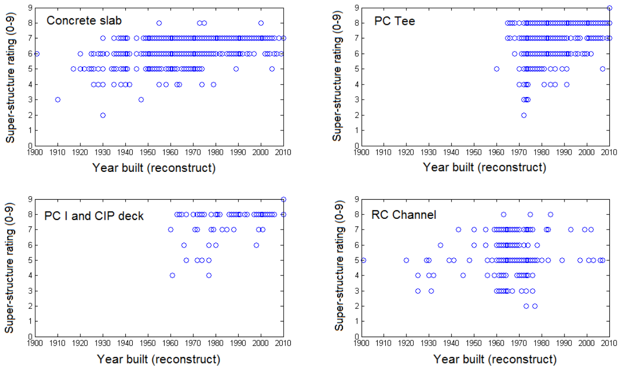
Figure 7-3: Bridge super-structure rating comparison break down
