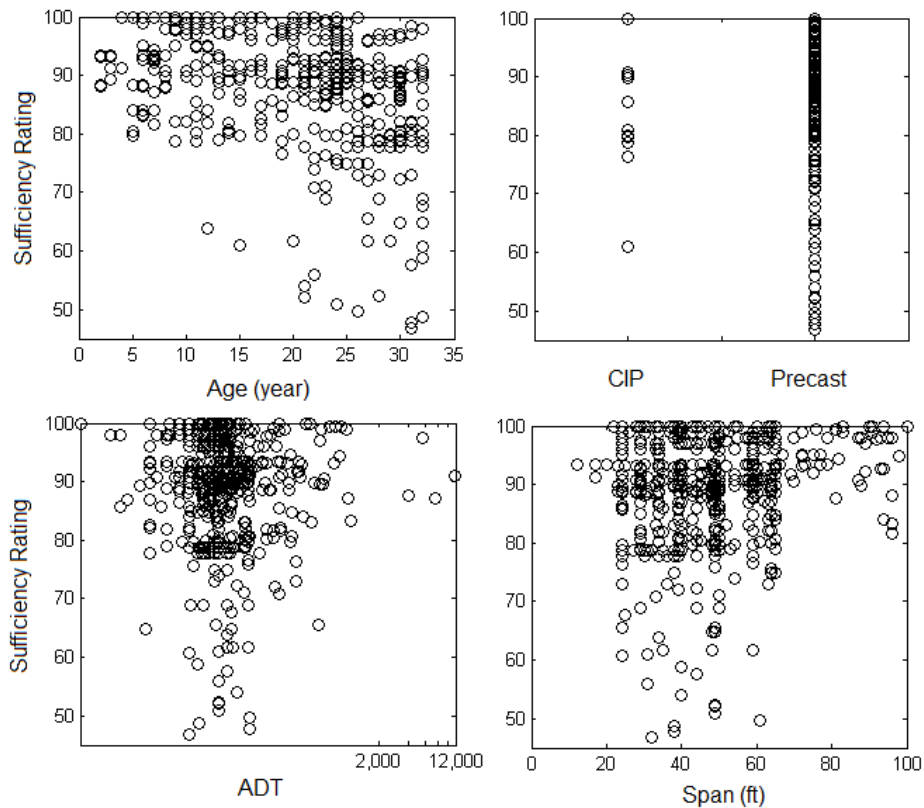
Figure 6-8: Correlation between control variables and current sufficiency rating for short span concrete bridges
