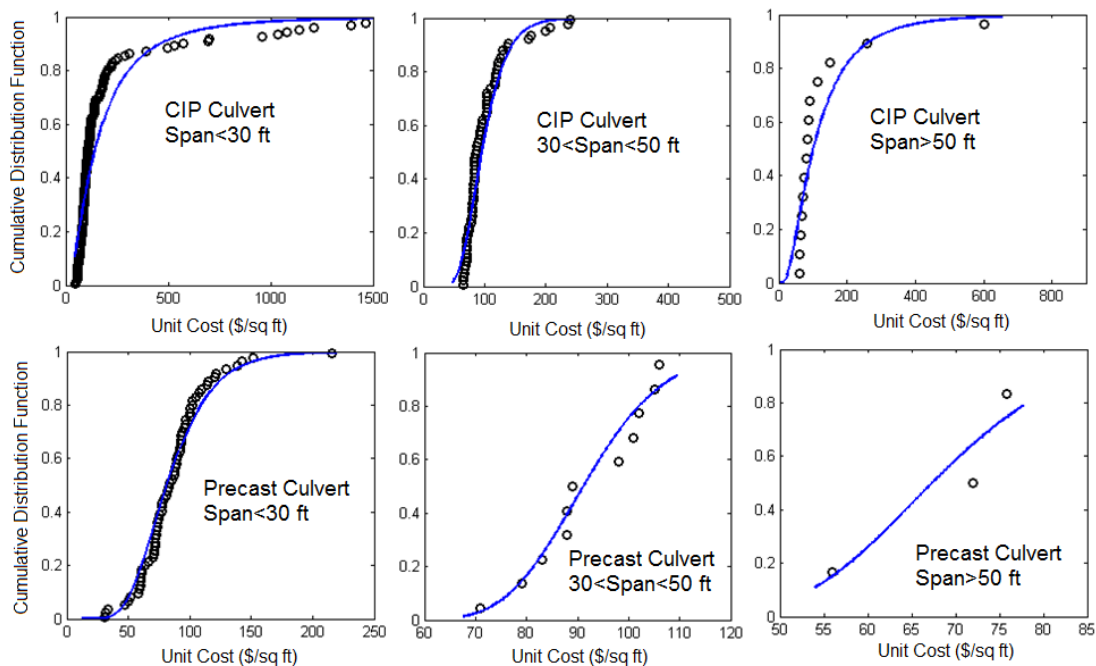
Figure 7-9: Culvert cost data and fitted Lognormal distribution curves
