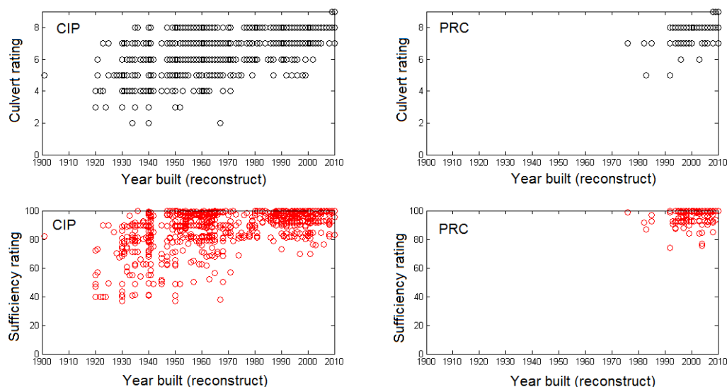
Figure 7-7: Culvert rating comparison break down
