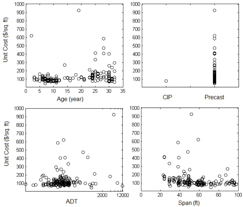
Figure 6-7: Correlation between control variables and unit cost (2010 value) for short span concrete bridges
