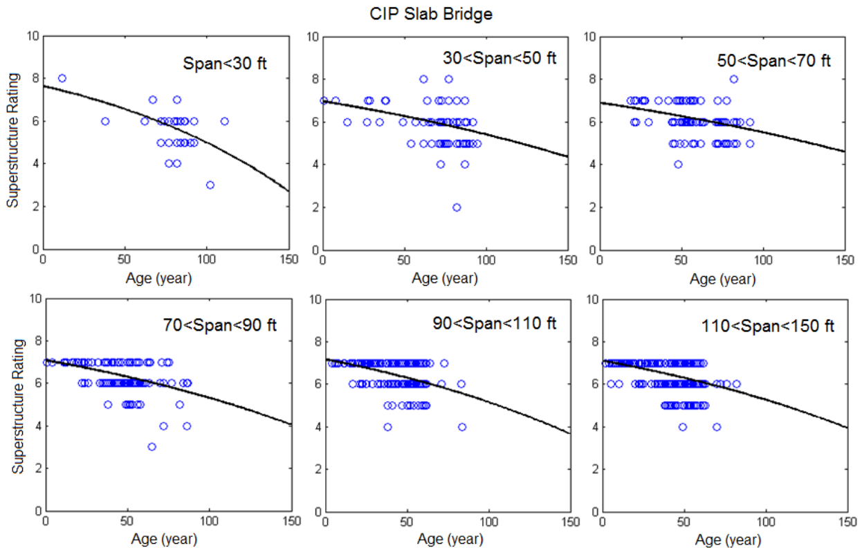
Figure 7-13: Regression analysis on structure rating for service life prediction (CIP slab bridge)
