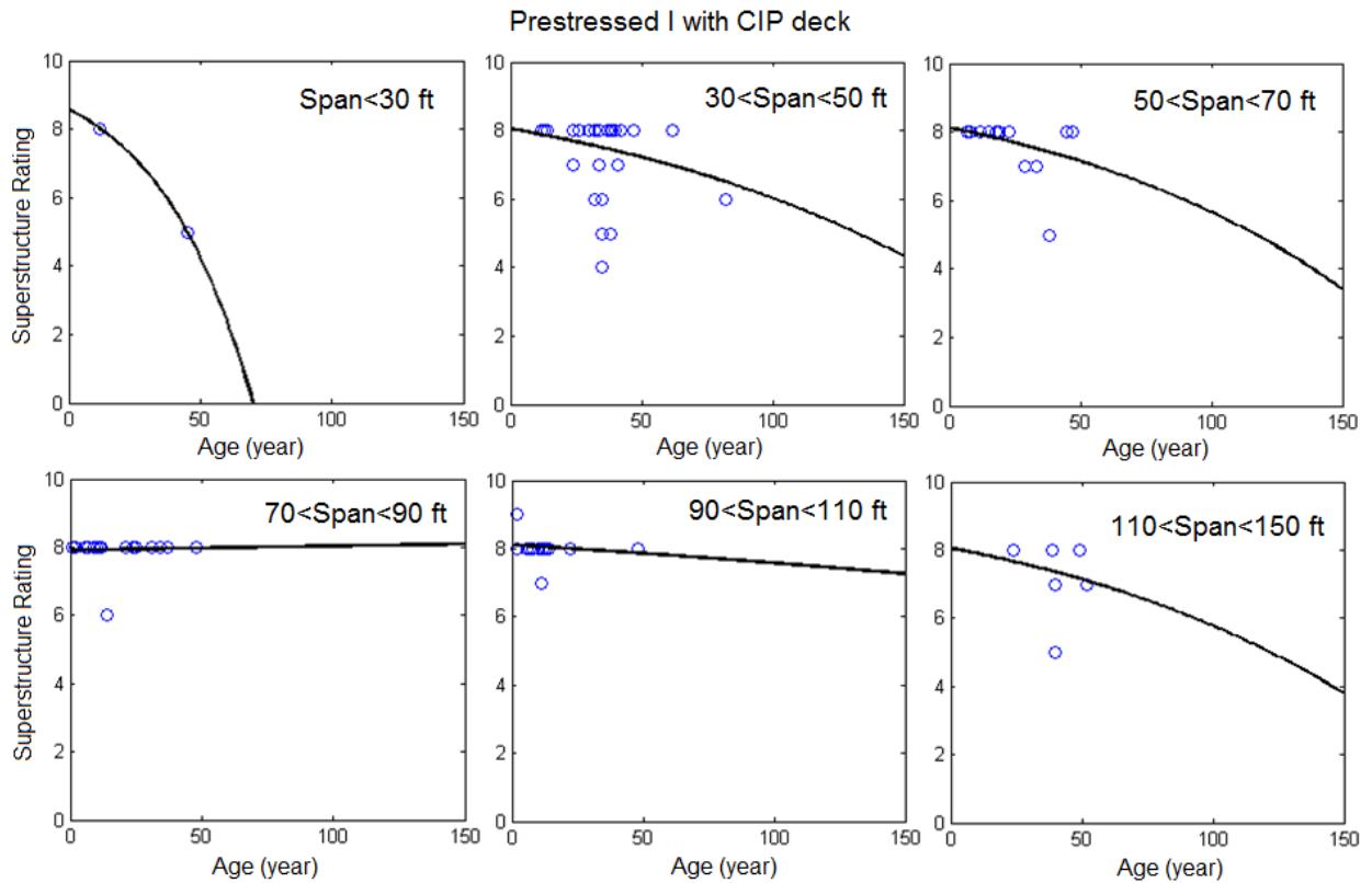
Figure 7-15: Regression analysis on structure rating for service life prediction (Prestressed I and CIP deck bridge)
