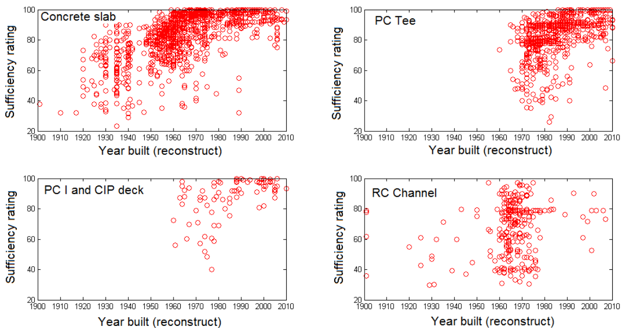
Figure 7-4: Bridge Sufficiency rating comparison break down
