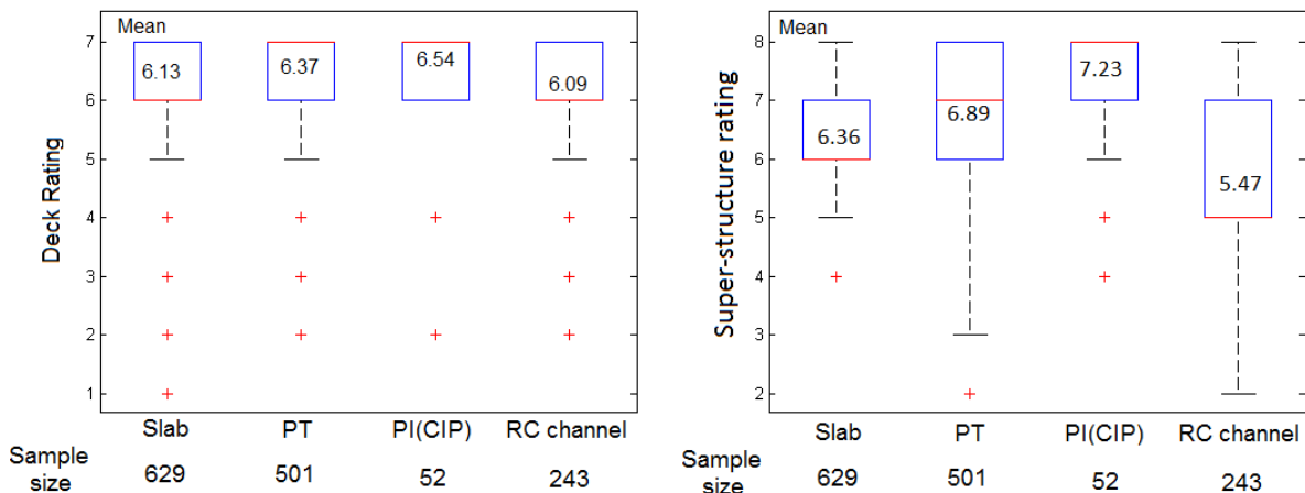
Figure 7-6: Group 2 comparison between bridge types
