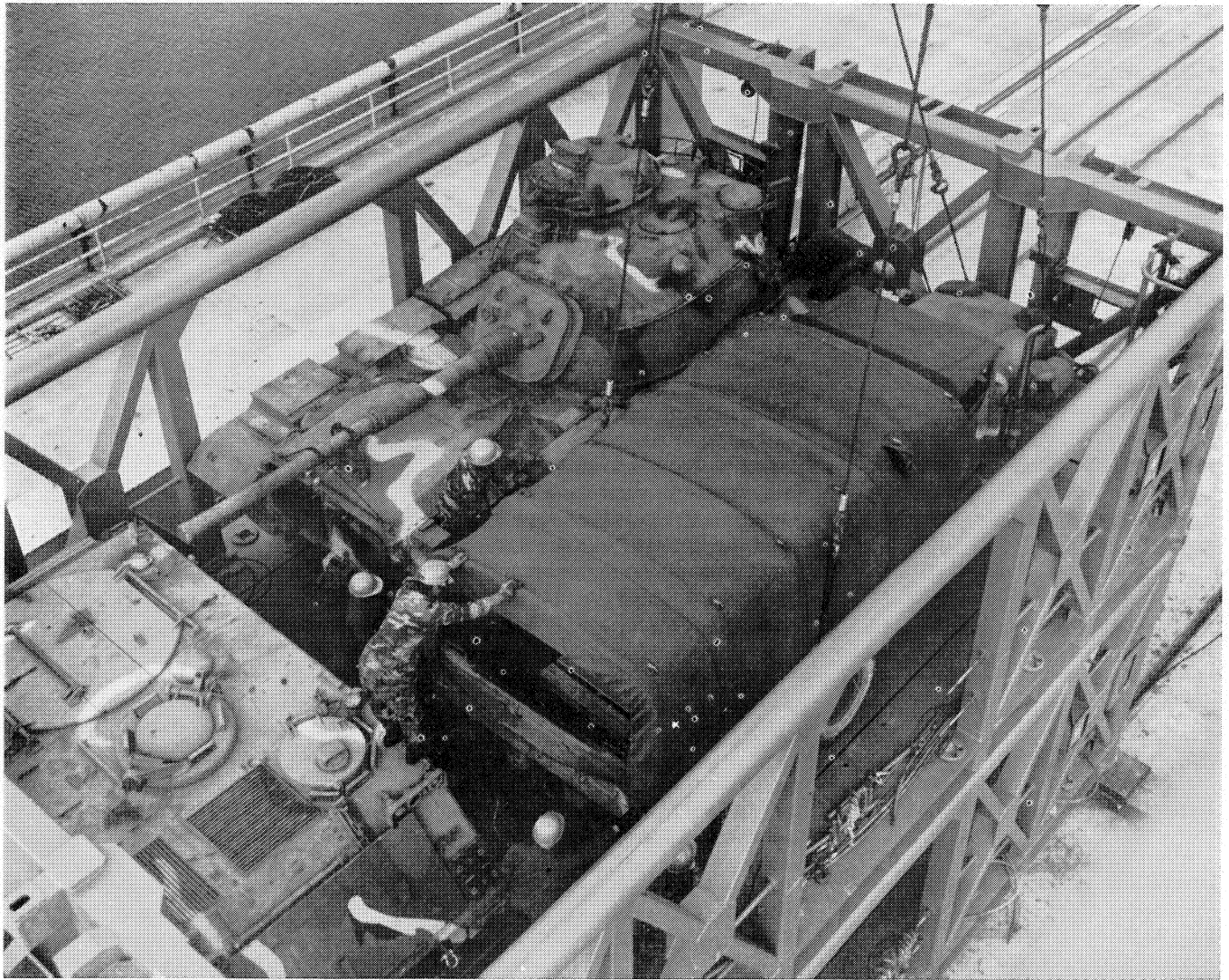
SEA SHEDs provide good stowage capability aboard containerships for large vehicles and equipment. Shown are an M-60 tank, a 5-ton truck and an armored personnel carrier during operational tests at Sunny Point, N.C. See also photo, page vi.
