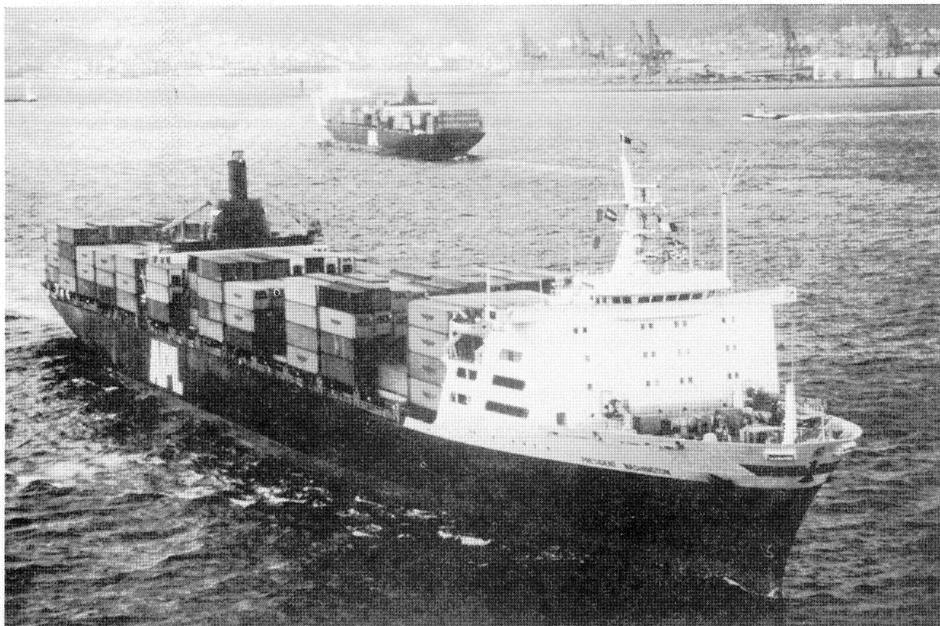
Two of American President Lines' three new containerships pass in Kobe, Japan. Built by Avondale Shipyards, Inc., and delivered in FY 1983, each vessel can carry 2,500 twenty foot containers.
