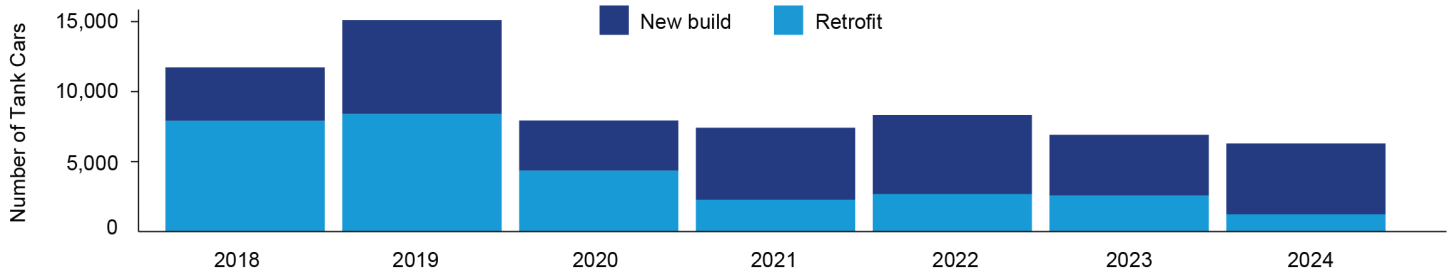
Figure 2 Projected Number of New and Retrofitted DOT-117 Tank Cars Completed by Year: 2018–2024
