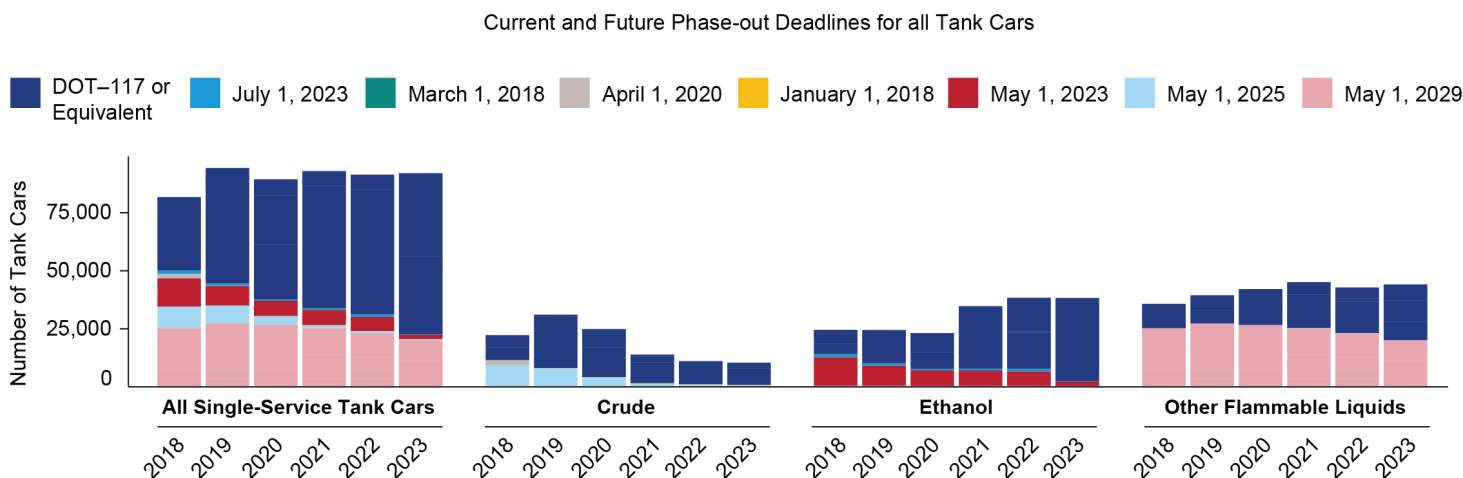
Figure 1 FAST Act Phase-Out Deadlines for Tank Cars by Number and Class 3 Flammable Liquid: 2018–2023
